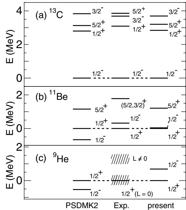
FIG. 3. Energy levels for (a) ^{13}\text{C} , (b) ^{11}\text{Be} , and (c) ^9\text{He} , relative to the state corresponding to the experimental ground state. The results by the PSDMK2 and present Hamiltonians are compared to experiments. Hatched areas indicate continuum states with resonance(like) structures.
