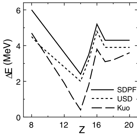
FIG. 2. The effective 1s_{1/2} - 0d_{3/2} gap in N = 16 isotones as a function of Z . The shell-model Hamiltonians, SDPF, USD, and “Kuo,” are used. See the text.
