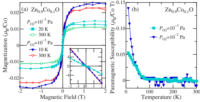
FIG. 1. (Color online) Magnetic properties of \text{Zn}_{0.9}\text{Co}_{0.1}\text{O} thin films measured by a SQUID magnetometer. (a) Magnetic-field ( H ) dependence of the magnetization. The H -linear components deduced from high H data have been subtracted. The inset shows raw data containing the diamagnetic signals from the substrates. (b) Temperature ( T ) dependence of the paramagnetic component of the magnetization represented in the form of magnetic susceptibility, where the T -independent component deduced from high- T data have been subtracted.
