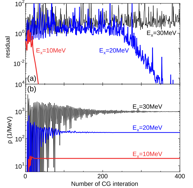
Fig. 3. (Color online.) Convergence patterns of the COCG and stochastic estimation of the total level density of ^{28}\text{Si} as a function of the number of iterations of the BCOCG method. (a) Residual of the BCOCG iteration |r_n|/|v_s| at z = E_{\text{gs}} + E_x with E_{\text{gs}} being the ground-state energy. (b) Total level densities at E_x = 10 (red), 20 (blue), 30 (black) MeV.
