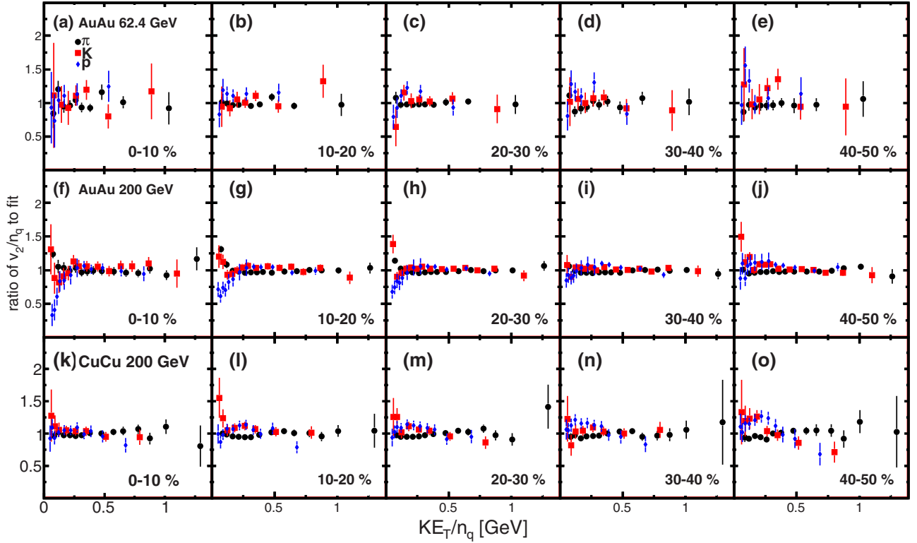
FIG. 19. (Color online) The ratio of v_2/n_q vs KE_T/n_q to the fit for \pi/K/p emitted from Au + Au at 62.4- and 200-GeV collisions and Cu + Cu at 200-GeV collisions for the centralities indicated. The lines for each point indicate the statistical uncertainties.
