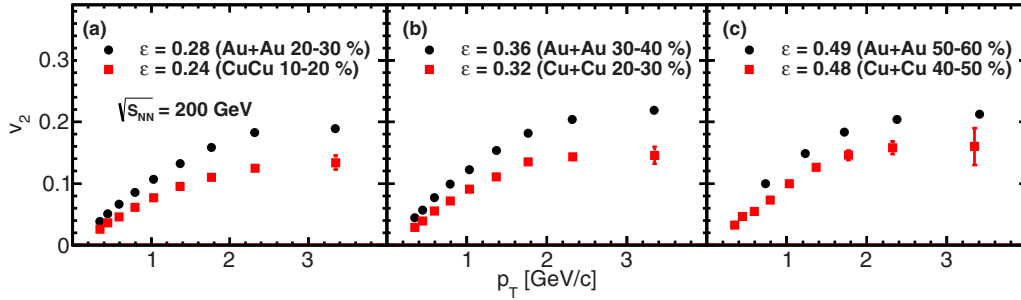
FIG. 12. (Color online) Comparison of v_2(p_T) at 200 GeV for two example systems with different collision size (Au + Au or Cu + Cu) but approximately the same \epsilon . Black symbols indicate Au + Au and red symbols indicate Cu + Cu. The average number of participants N_{\text{part}} is 166.6 for 20%–30%, 114.2 for 30%–40%, and 45.5 for 50%–60% at Au + Au collisions, and N_{\text{part}} is 73.6 for 10%–20%, 53.0 for 20%–30%, and 25.4 for 40%–50% at Cu + Cu collisions.
