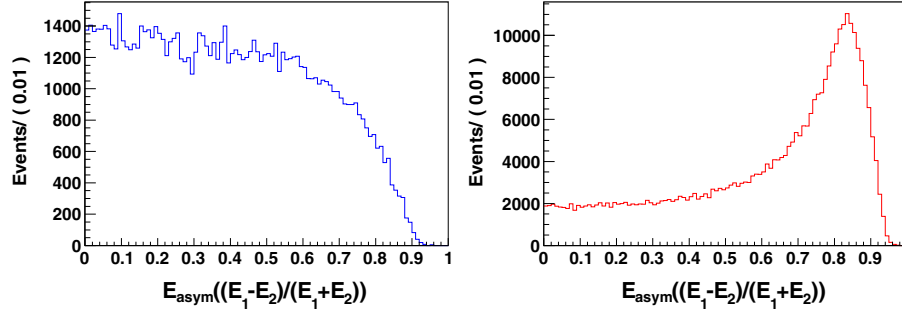
FIG. 1 (color online). The E_{\text{asym}} distributions for signal MC events for correctly (left) and incorrectly (right) assigned photons.
