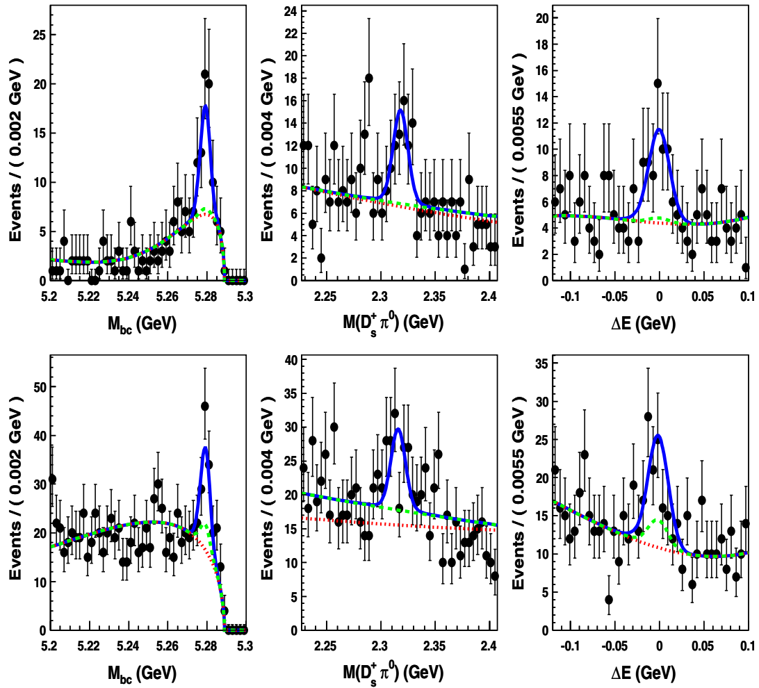
FIG. 5 (color online). Top: The M_{bc} (left), M(D_s^+ \pi^0) (center) and \Delta E (right) distributions for the B^+ \rightarrow \bar{D}^0 D_{s0}^{*+} candidate events for the \bar{D}^0 \rightarrow K^+ \pi^- subdecay mode, with the results of the fit superimposed. The events in each distribution are in the signal regions of the two quantities not being plotted. Bottom: The corresponding distributions for \bar{D}^0 \rightarrow K^+ \pi^+ \pi^- \pi^- decays. (See text for curves.)
