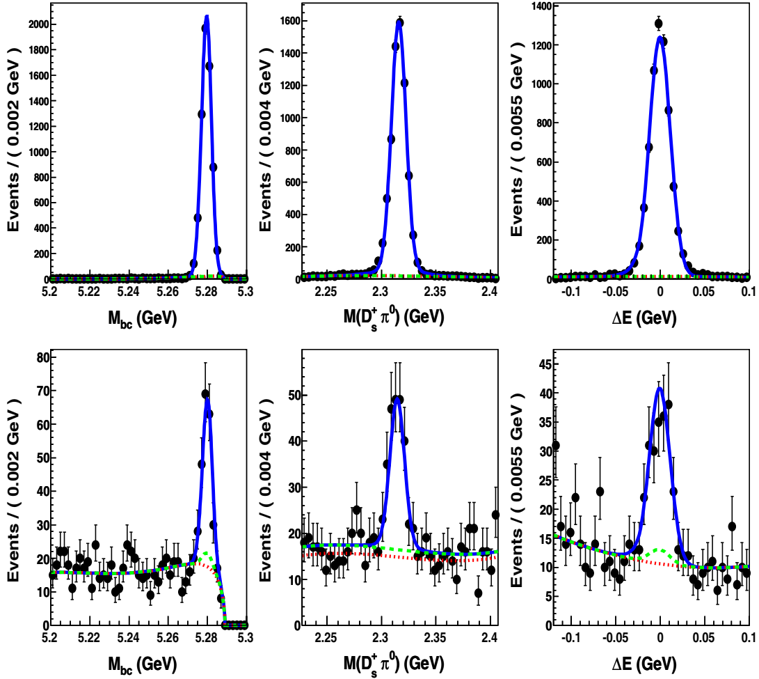
FIG. 3 (color online). Top: The M_{bc} (left), M(D_s^+ \pi^0) (center) and \Delta E (right) distributions for the B^0 \rightarrow D^- D_{s0}^{*+} signal MC events with the results of the fit superimposed. The events in each distribution are in the signal regions of the two quantities not being plotted. Bottom: The corresponding distributions for the generic MC event sample ( \sim 3 times the data). (See text for curves.)
