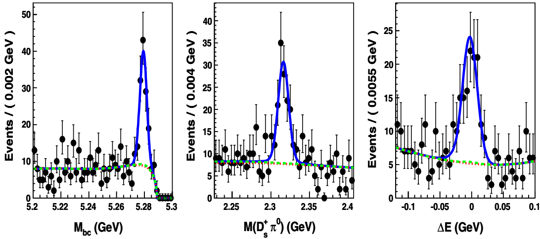
FIG. 4 (color online). The M_{bc} (left), M(D_s^+ \pi^0) (center) and \Delta E (right) distributions for projections of the B^0 \rightarrow D^- D_{s0}^{*+} candidate events that are in the signal regions of the two quantities not being plotted. The results of the fit described in the text are superimposed. (See text for curves.)
