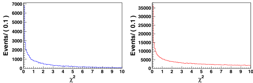
FIG. 2 (color online). The \chi^2 distributions from the \pi^0 \rightarrow \gamma\gamma fit for signal MC events for correctly (left) and incorrectly (right) assigned photons.
