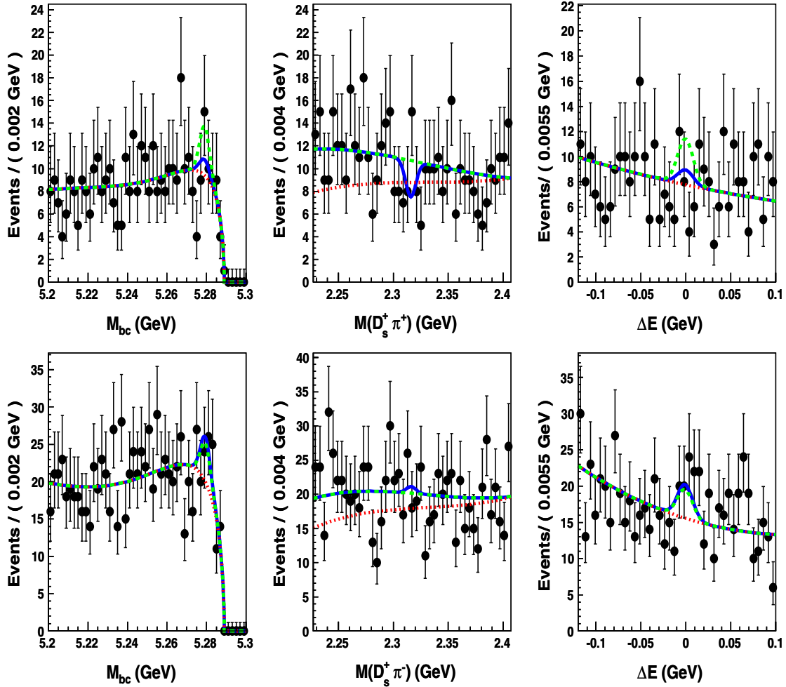
FIG. 7 (color online). The M_{bc} (left), M(D_s^+ \pi^+) (center) and \Delta E (right) distributions for selected B^+ \rightarrow D^- D_s^+ \pi^+ (top) and B^0 \rightarrow \bar{D}^0 D_s^+ \pi^- (bottom) event candidates for the fit with the signal peak mass restricted to a 5 MeV region centered at M(D_s^+ \pi^+) = 2317.8 MeV. In the lower plots, the \bar{D}^0 \rightarrow K^+ \pi^- and K^+ \pi^+ \pi^- \pi^- samples are combined. (See text for curves.)
