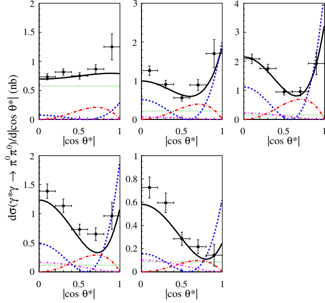
FIG. 23. |\cos \theta^*| dependence in five W bins: 0.9, 1.15, 1.25, 1.35, and 1.45 GeV from left to right and top to bottom and fitted results of the \varphi^* nominal fit. The legend of lines is: solid lines show the total (black), dotted |S|^2 (green), dashed |D_0|^2 (blue), long dashed |D_1|^2 (red), and dash-dotted |D_2|^2 (purple).
