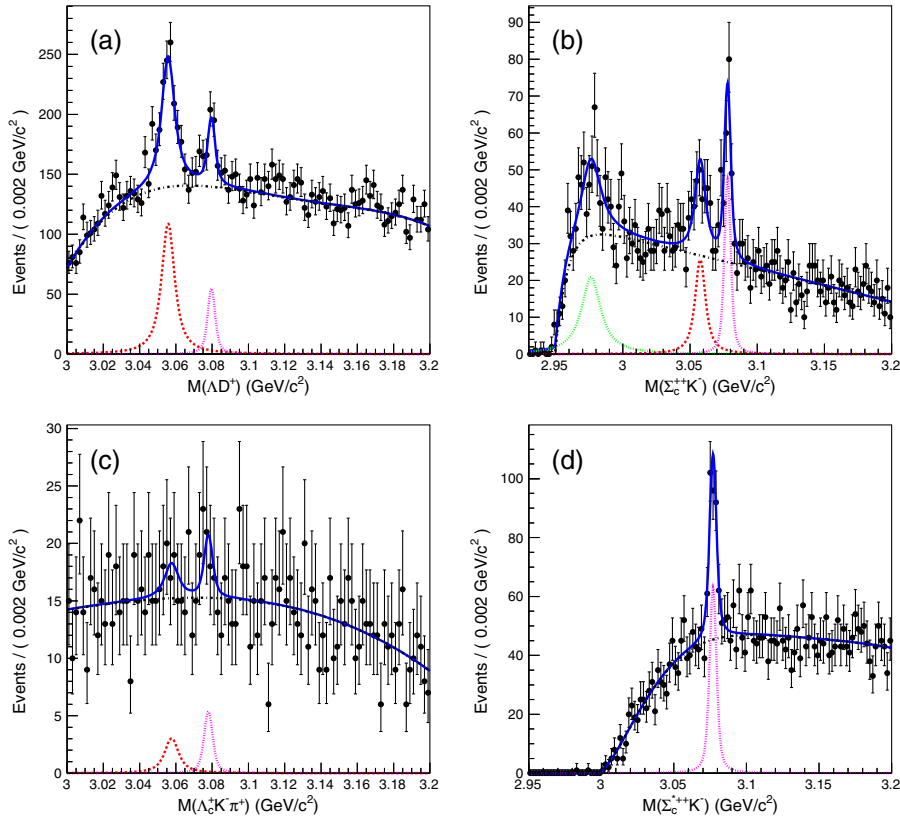
FIG. 2. The simultaneous fit results: (a) M(\Lambda D^+) , (b) M(\Sigma_c^{++} K^-) , (c) M(\Lambda_c^+ K^- \pi^+) for the \Sigma_c^{++} sideband region, and (d) M(\Sigma_c^{*++} K^-) . Points with error bars are data. The blue solid lines show the fit result. The red dashed, magenta dotted, green dotted, and black dash-dotted lines show the contributions from the \Xi_c(3055)^+ , \Xi_c(3080)^+ , \Xi_c(2980)^+ , and background, respectively.
