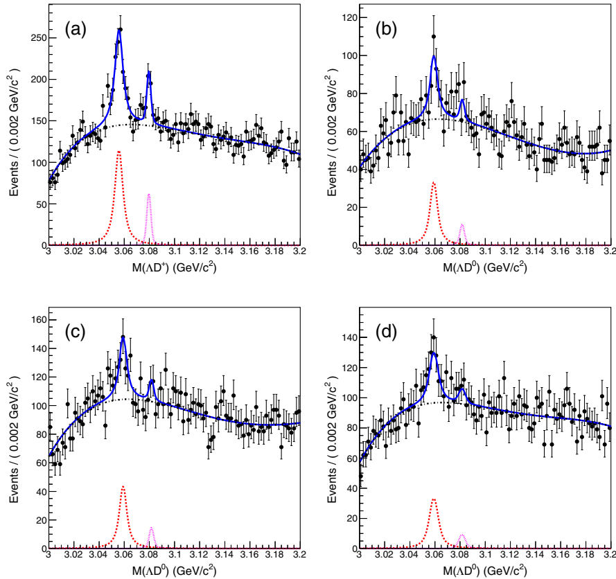
FIG. 1. M(\Lambda D) distributions: (a) M(\Lambda D^+) distribution; M(\Lambda D^0) distributions for the (b) K^-\pi^+ , (c) K^-\pi^+\pi^+\pi^- , and (d) K^-\pi^+\pi^0 D^0 decay modes. Points with statistical error bars are data. Blue solid lines show the fit results. The red dashed, magenta dotted, and black dashed-dotted lines show the \Xi_c(3055) signal, the \Xi_c(3080) signal, and the background components, respectively.
