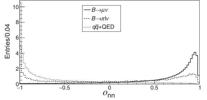
FIG. 1. The distributions of the neural network output variable for the signal and major background processes predicted by MC in the signal-enhanced region 2.644 \text{ GeV}/c < p_\mu^* < 2.812 \text{ GeV}/c (the relative normalization of these distributions is arbitrary).
