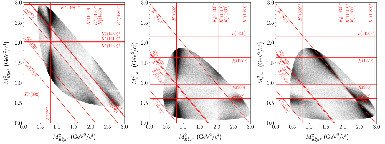
FIG. 4. Dalitz plot data distributions for all three combinations of M^2_{K_S^0 \pi^-} , M^2_{K_S^0 \pi^+} , and M^2_{\pi^+ \pi^-} for D^0 \rightarrow K_S^0 \pi^+ \pi^- from D^{*+} \rightarrow D^0 \pi_s^+ decays reconstructed from Belle e^+ e^- \rightarrow c \bar{c} data. For illustration purposes, the approximate locations of various intermediate two-body resonances are indicated by horizontal, vertical, and diagonal lines.
