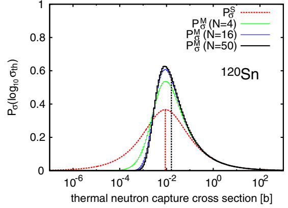
FIG. 1. Probability distributions P_\sigma^M(\log_{10} \sigma_{\text{th}}) and P_\sigma^S(\log_{10} \sigma_{\text{th}}) . For P_\sigma^M(\log_{10} \sigma_{\text{th}}) , calculations using the number of resonance N=4, 16, 50 are compared.
