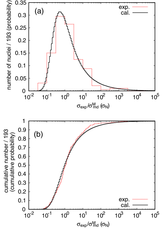
FIG. 6. (a) Distribution [(b) cumulative distribution] of the nuclei as a function of the experimental \sigma_{\text{th}} normalized to \sigma_{\text{md}}^M compared with P_\sigma^M(\log \sigma_N) . The vertical axis is the number (cumulative number) of nuclei divided by the total number of nuclei, which are comparable to the probability (cumulative probability).
