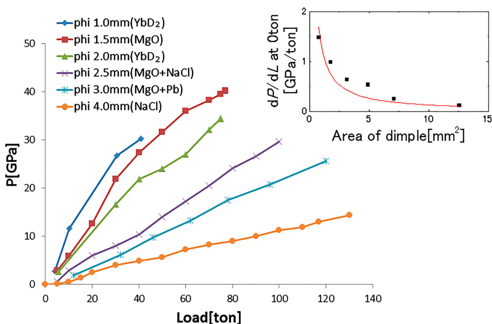
Figure 4. Pressure-load relations when using anvils with different dimple diameters (DDs). (Inset) Comparison of the initial slope of the pressure generation curves against the area of the dimple.
