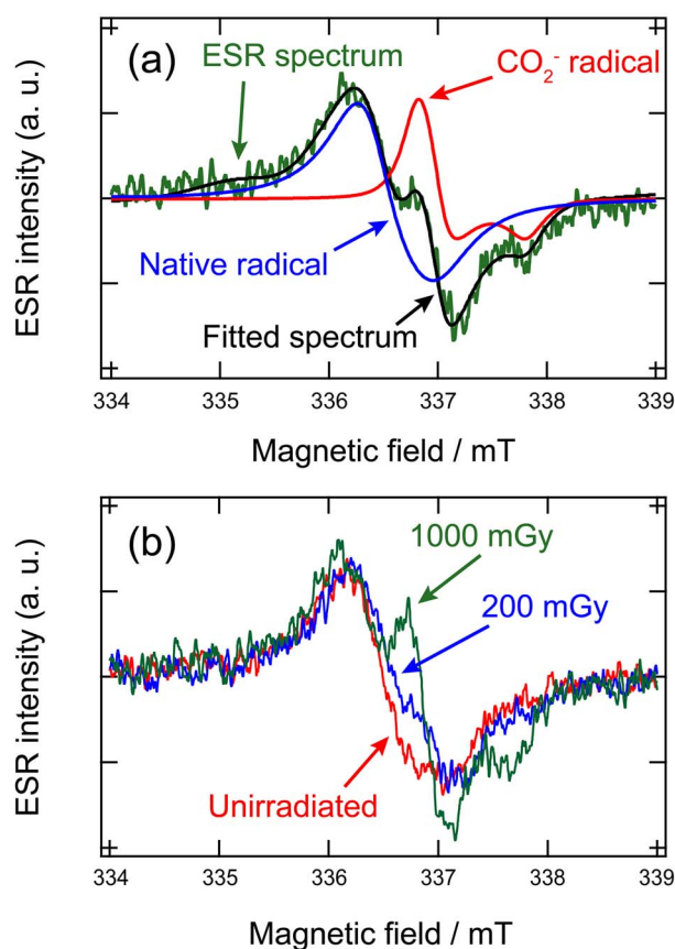
Fig. 2. (a) Typical ESR spectrum, deconvoluted spectra and a fitted spectrum for a 500 mGy-irradiated deciduous tooth from a Japanese child. (b) ESR spectra for the same deciduous tooth irradiated with different dose.
