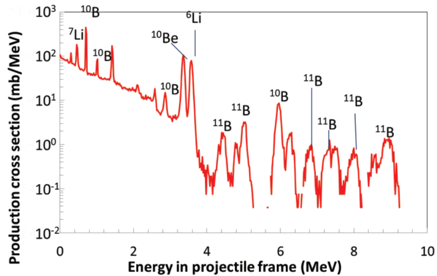
Figure 3: Energy spectrum of gamma-rays from ^{11}\text{B} interacting with nitrogen.
