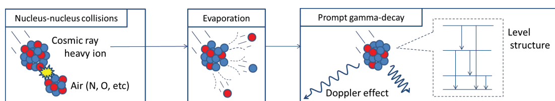
Figure 1: Calculation scheme of prompt gamma-rays from cosmic heavy ion fragments.
