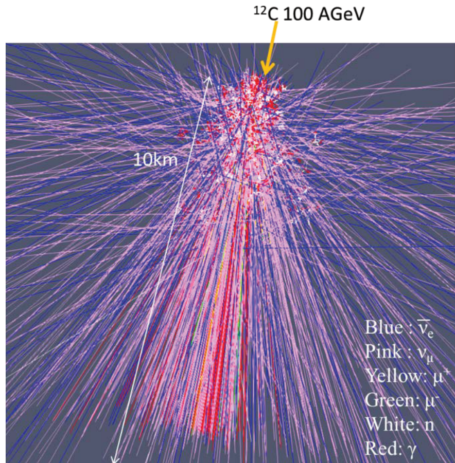
Figure 2: Secondary particle trajectories in one reaction.
