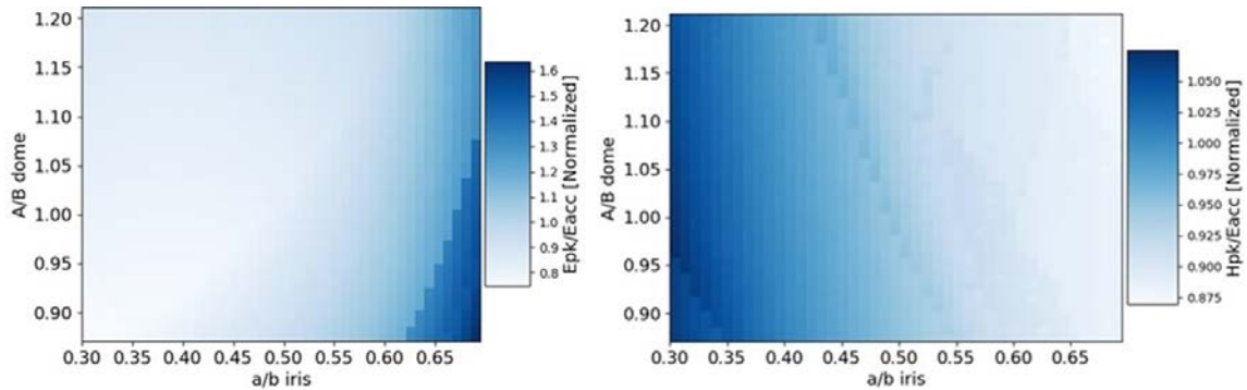
Figure 4. The surface plot by changing the iris and the dome ratio to select the parameters to minimize the E_{pk}/E_{acc} (left) and H_{pk}/E_{acc} (right).
