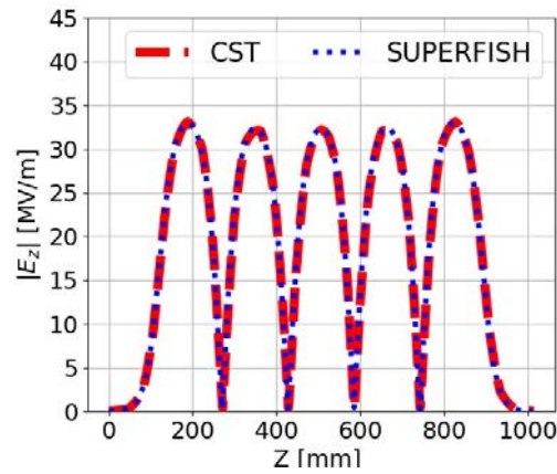
Figure 5. The comparison of the absolute value of the longitudinal electric field between SF and CST for the EllipR1 models.
