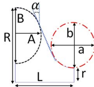
Figure 2. Parametrization of the half cell geometry. R is the cavity radius, L half of the cell length, r is beam pipe radius, A and B are the semi-axis of the ellipse dome, a and b are the semi axis of the ellipse iris and \alpha is the wall angle.
