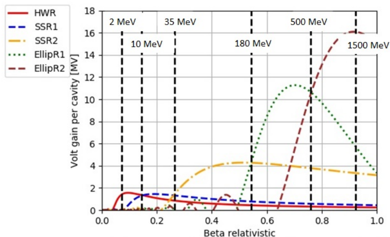
Figure 1. Voltage gain per cavity as a function of relativistic beta for the JAEA-ADS project.
