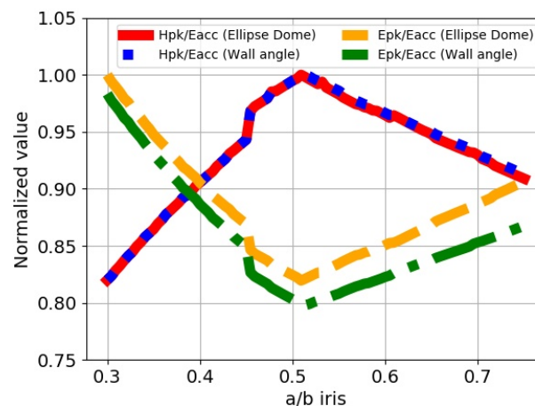
Figure 3. The electromagnetic peaks as a function of the iris ratio by adjusting the ellipse dome ratio (solid red line and dashed orange line) and adjusting \alpha (dotted blue line and dashed-dotted green line) to tune the frequency. The values were normalized to maximum value of electromagnetic peaks.
