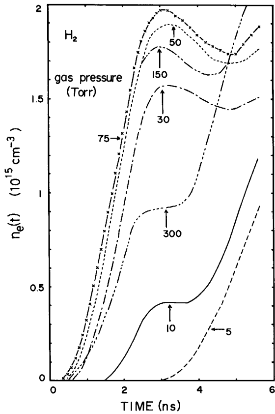
Fig. 8.3 Calculated curves of n_e(t) for various pressures of \text{H}_2 .
