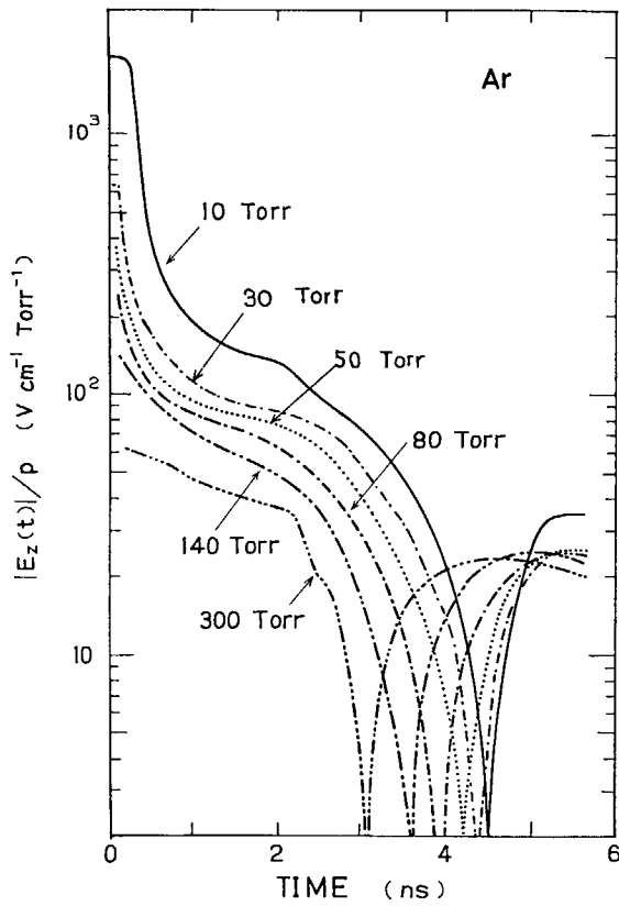
Fig. 7.9 Calculated curves of E_z/p obtained from E_z in Fig. 7.8 for various pressures of Ar.
