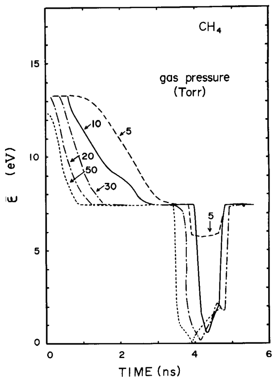
Fig. 9.5 Calculated curves of \bar{\epsilon}(t) for various pressures of \text{CH}_4 .
