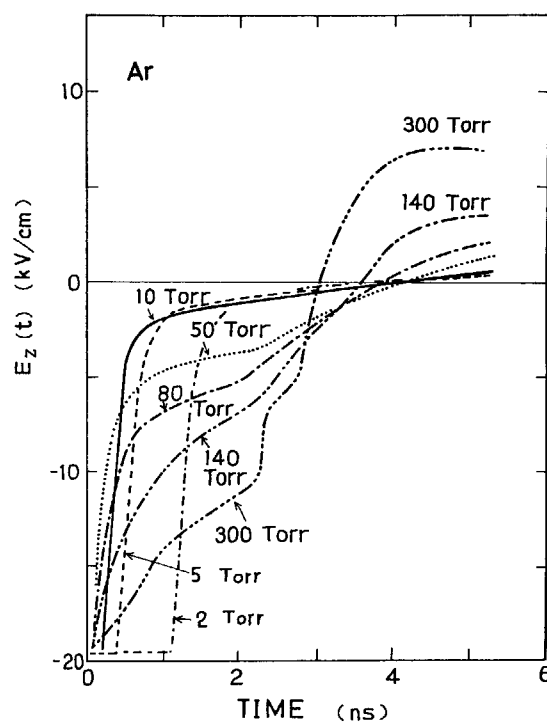
Fig. 7.8 Calculated curves of E_z(t) for various pressures of Ar.
