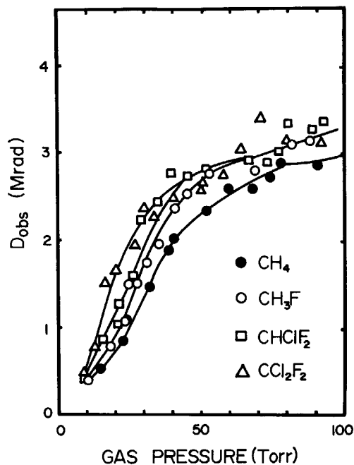
Fig. 9.9 Data on D_{obs} as functions of pressure for halogenomethanes.
