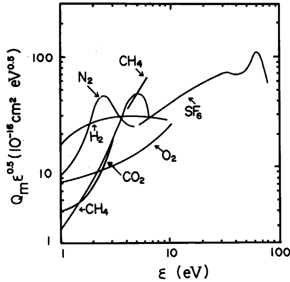
Fig. 8.13 Curves of Q_m \epsilon^{0.5} for some polyatomic gases plotted against \epsilon .
