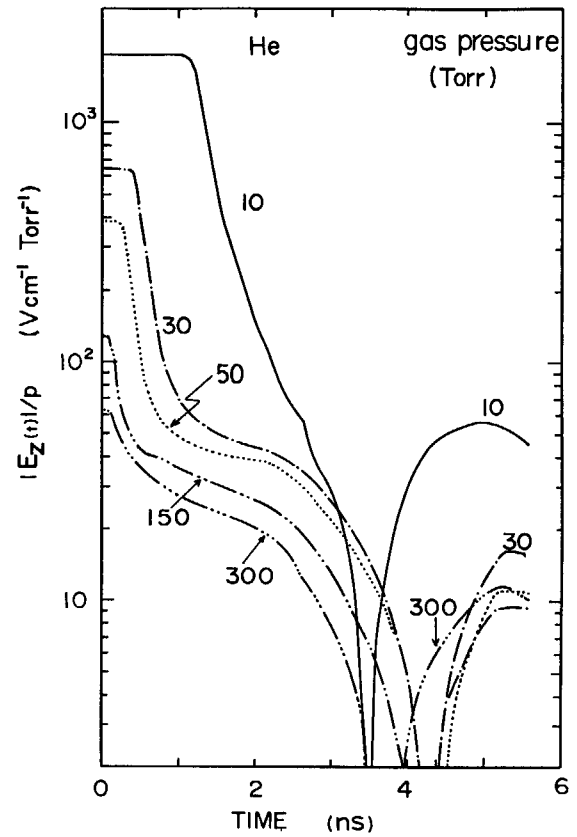
Fig. 7.4 Calculated curves of E_z/p obtained from E_z in Fig. 7.3 for various pressures of He.
