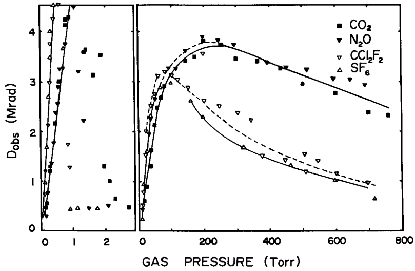
Fig. 3.10 Values of D_{obs} , at 10.4 cm on the beam axis from the cell window in \text{CO}_2 ( \blacksquare ), \text{N}_2\text{O} ( \blacktriangledown ), \text{SF}_6 ( \triangle ), and \text{CCl}_2\text{F}_2 ( \nabla ).
