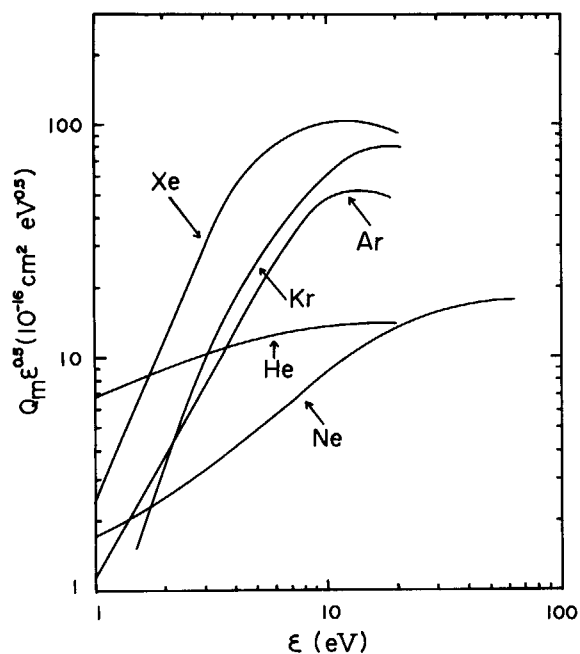
Fig. 7.14 Curves of Q_m(\epsilon)\epsilon^{0.5} for monatomic gases cited from references in text.
