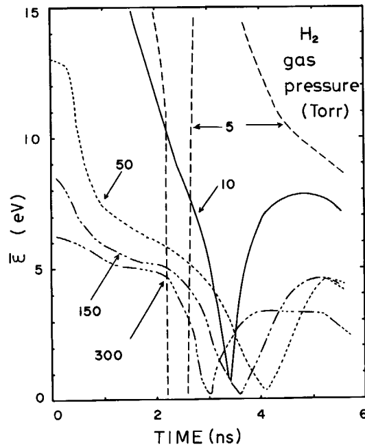
Fig. 8.5 Calculated curves of \bar{\epsilon}(t) for various pressures of \text{H}_2 .
