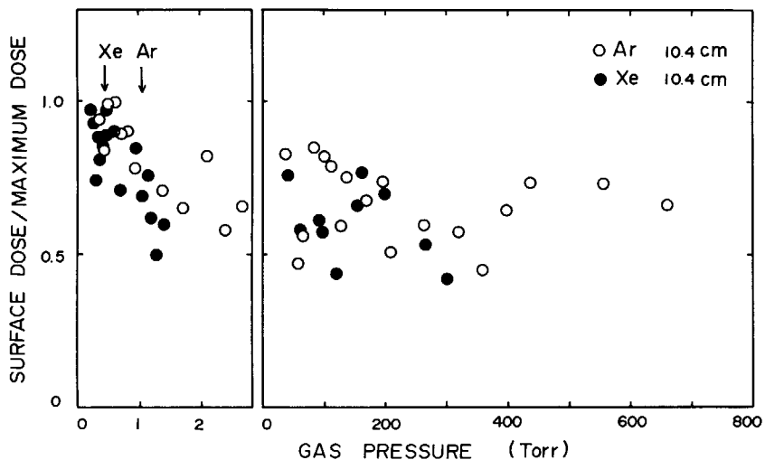
Fig. 4.12 Ratios of the surface dose to the maximum dose in depth-dose curves at 10.4 cm on the beam axis from the cell window as functions of pressure of Ar (○) and Xe (●). Arrows indicate p_{AMrad}
