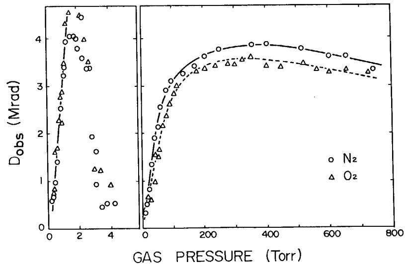
Fig. 3.9 Values of D_{obs} at 10.4 cm on the beam axis from the cell window in N_2 ( \circ ) and O_2 ( \Delta ).
