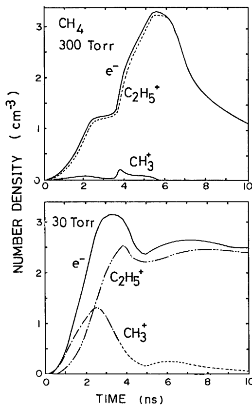
Fig. 9.6 Calculated curves of n_e(t) , n_i(\text{CH}_3^+)(t) , and n_d(\text{C}_2\text{H}_5^+)(t) at 30 and 300 Torr of \text{CH}_4 .
