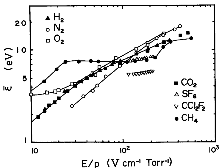
Fig. 8.18 Curves of \bar{\epsilon} as functions of E/p estimated from data on D_L/\mu in references in text.
