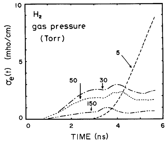
Fig. 8.4 Calculated curves of \sigma_e(t) for various pressures of \text{H}_2 .
