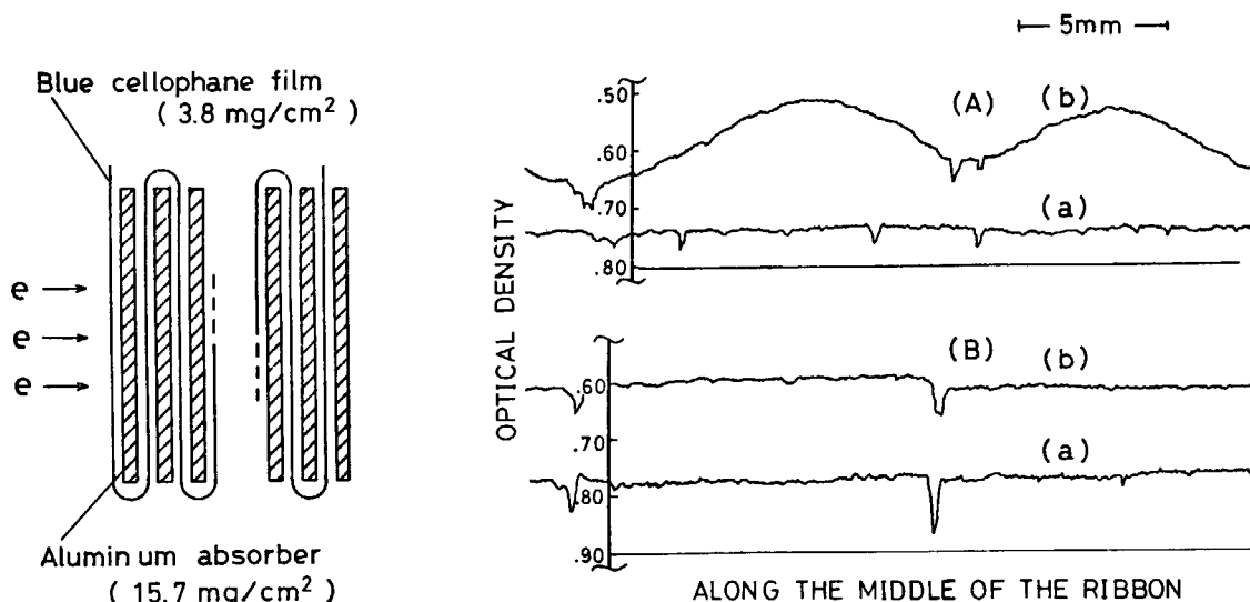
Fig. 3.3 Scanning of the optical density of the blue cellophane ribbon at 655 nm before (a) and after (b) irradiation. The self-focused (A) and defocused beam (B).
