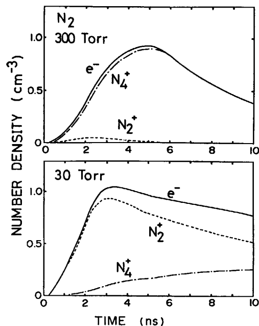
Fig. 8.11 Calculated curves of n_e(t) , n_i(N_2^+)(t) , and n_d(N_4^+)(t) at 30 and 300 Torr of N_2 .
