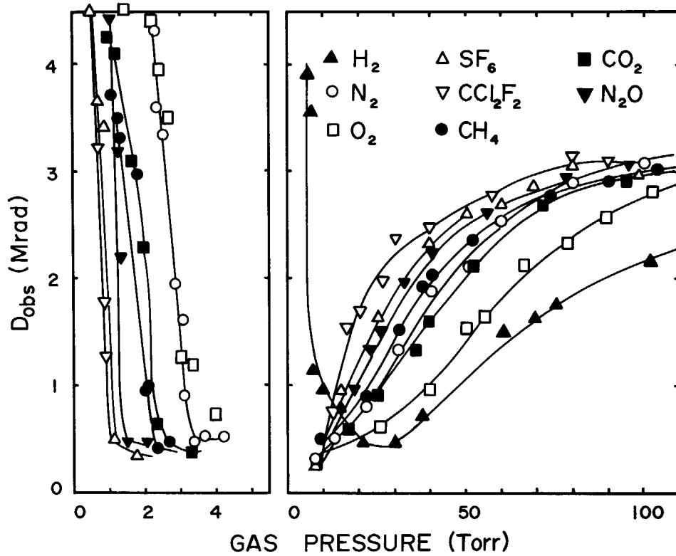
Fig. 8.15 Data on D_{obs}(p) for some polyatomic gases.
