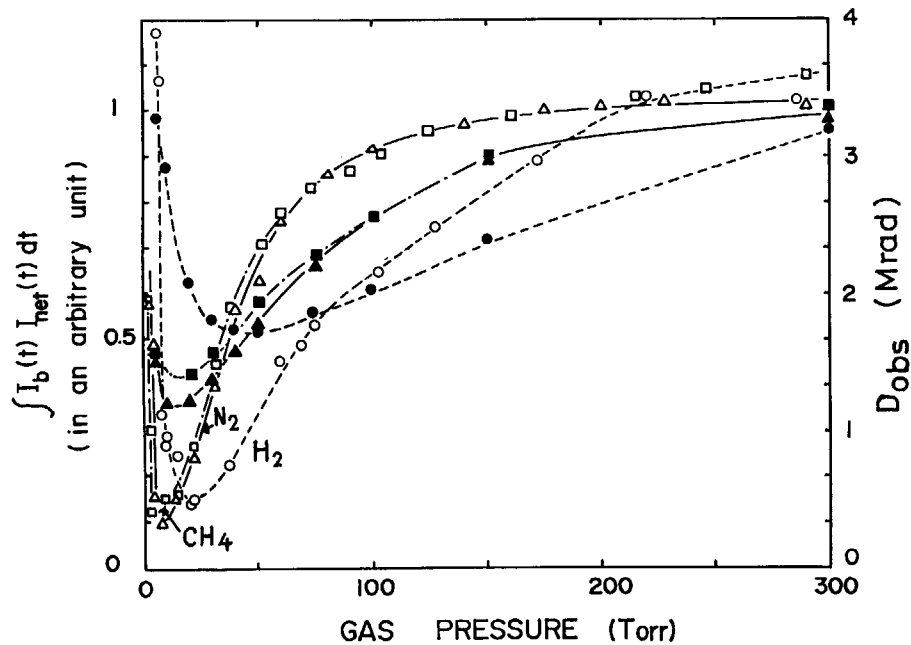
Fig. 8.12 Data on D_{obs}(p) for H_2 ( \circ ), N_2 ( \triangle ), and CH_4 ( \square ) and values of \int_0^p I_b(t) I_{net}(t) dt calculated from I_{net}(t) in Figs. 8.1, 8.6, and 9.1, which are plotted in an arbitrary unit by the corresponding closed marks.
