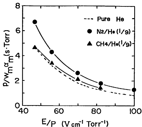
Fig. 10.2 Values of p/(w_m \alpha_m) estimated by the average electron method for \text{N}_2/\text{He} (1/9) and \text{CH}_4/\text{He} (1/9).
