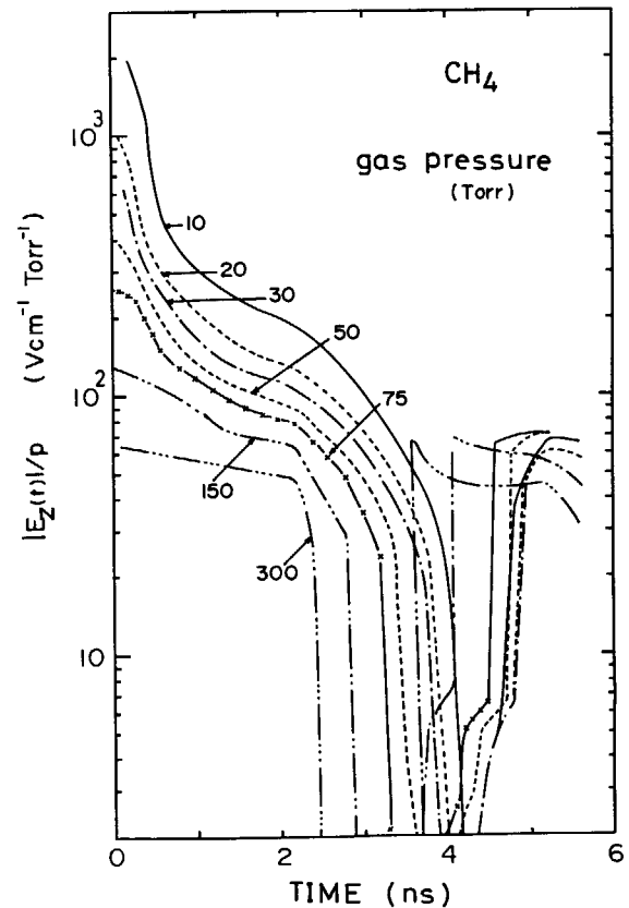
Fig. 9.2 Calculated curves of E_z(t)/p for various pressures of \text{CH}_4 .
