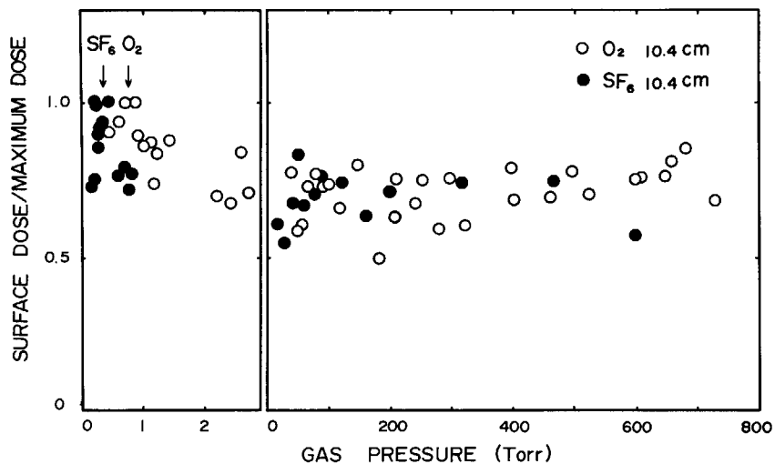
Fig. 4.13 Ratios of the surface dose to the maximum dose in depth-dose curve at 10.4 cm on the beam axis from the cell window as functions of pressure of O 2 (○) and SF 6 (●). Arrows indicate p_{AMrad}
