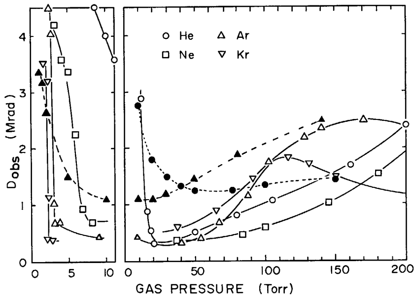
Fig. 7.2 Data on D_{obs}(p) for monatomic gases shown by open marks. Values of \int_0^p I_b(t)I_{net}(t)dt calculated from I_{net}(t) in Fig. 7.1 are also plotted in an arbitrary unit for He (●) and Ar (▲).
