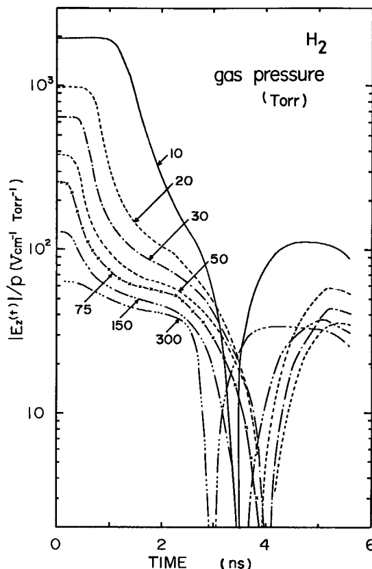
Fig. 8.2 Calculated curves of E_z(t)/p for various pressures of H_2 .
