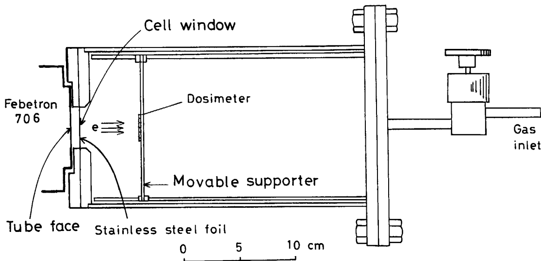
Fig. 3.1 The irradiation cell.
