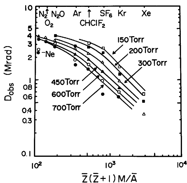
Fig. 11.1 Data on D_{obs} plotted against Z(\bar{Z}+1)M/\bar{A} for various pressures; 150 Torr ( \square ), 200 Torr ( \blacksquare ), 300 Torr ( \triangle ), 450 Torr ( \blacktriangle ), 600 Torr ( \circ ), and 700 Torr ( \bullet ).
