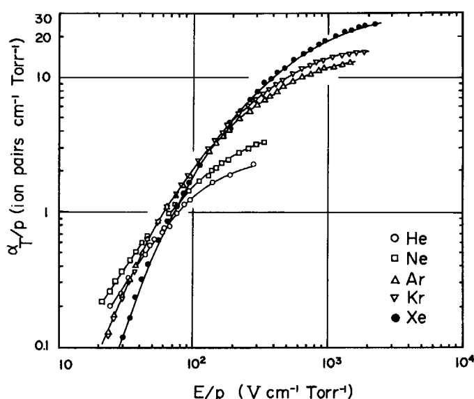
Fig. 7.13 Curves of \alpha_T/p as functions of E/p for monatomic gases.
