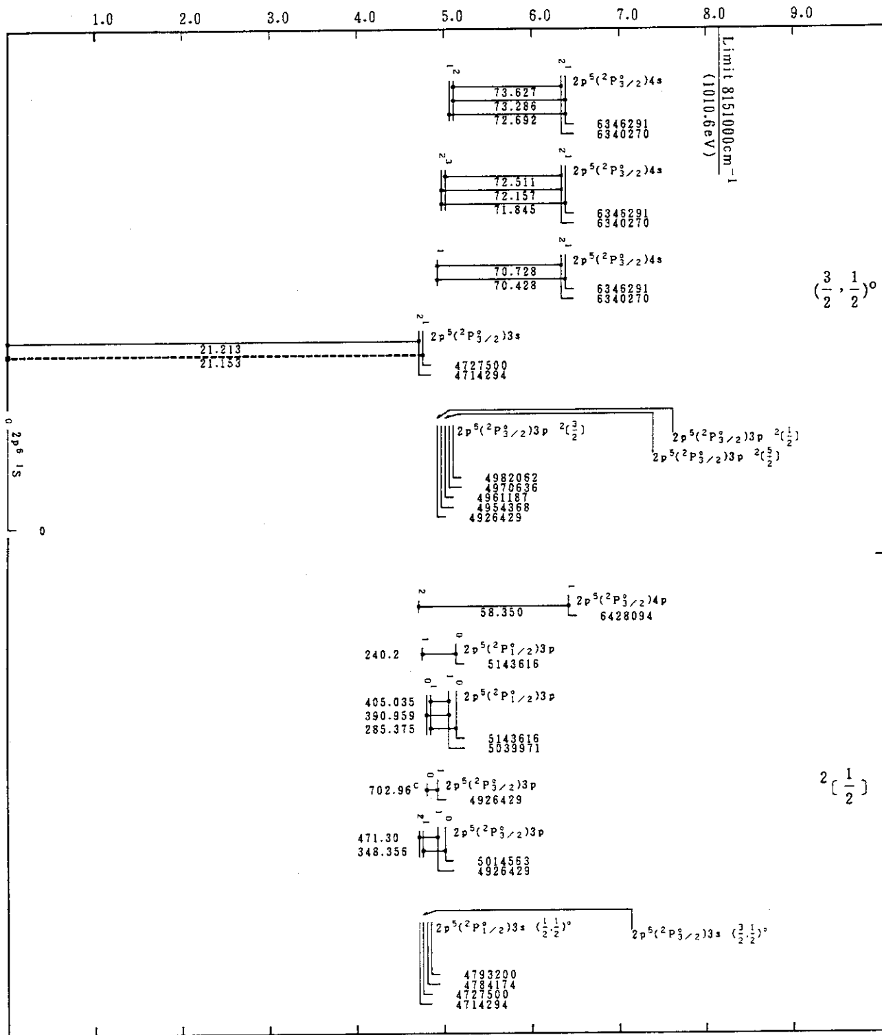
Cr XV(Ne-Sequence)
