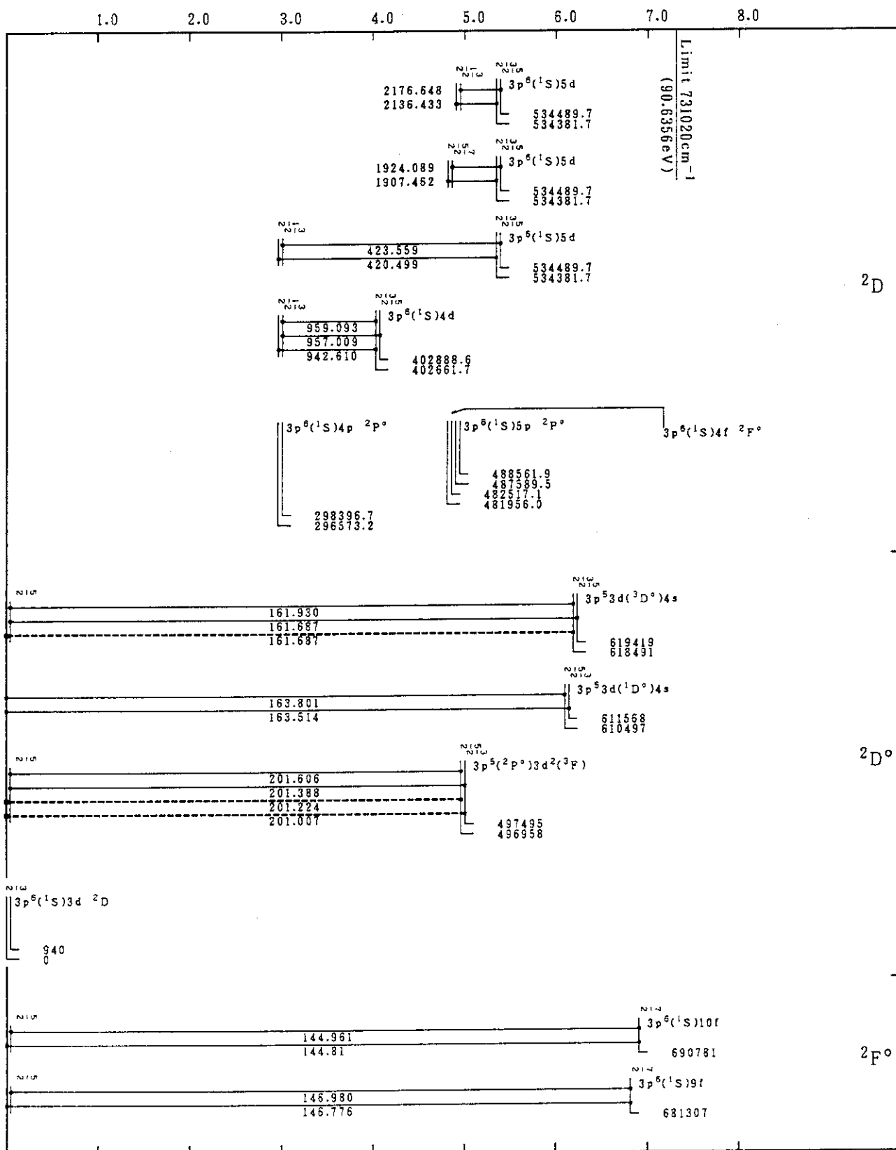
Cr VI(K-Sequence)
