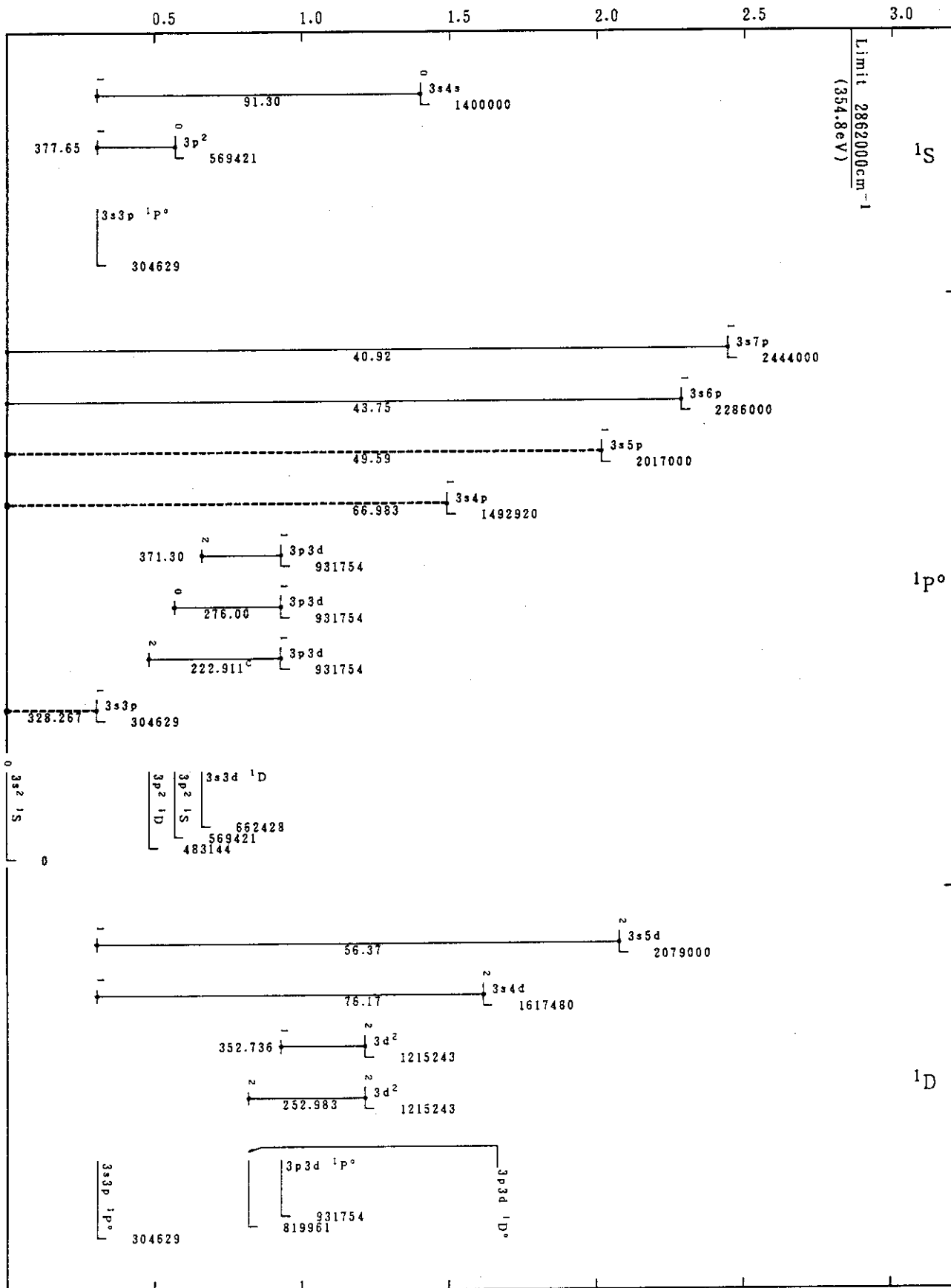
Cr XIII(Mg-Sequence)
