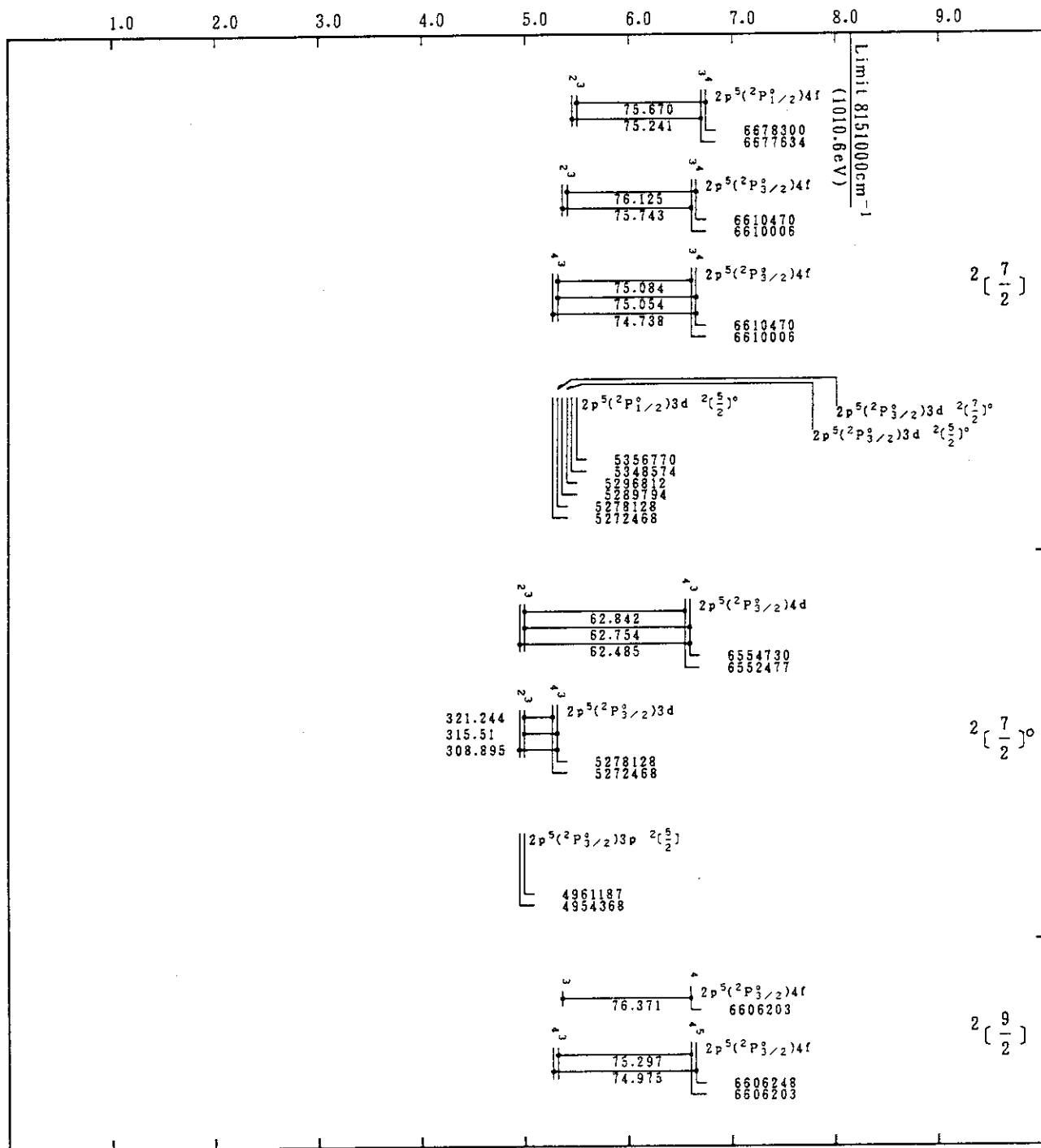
Cr XV(Ne-Sequence)
