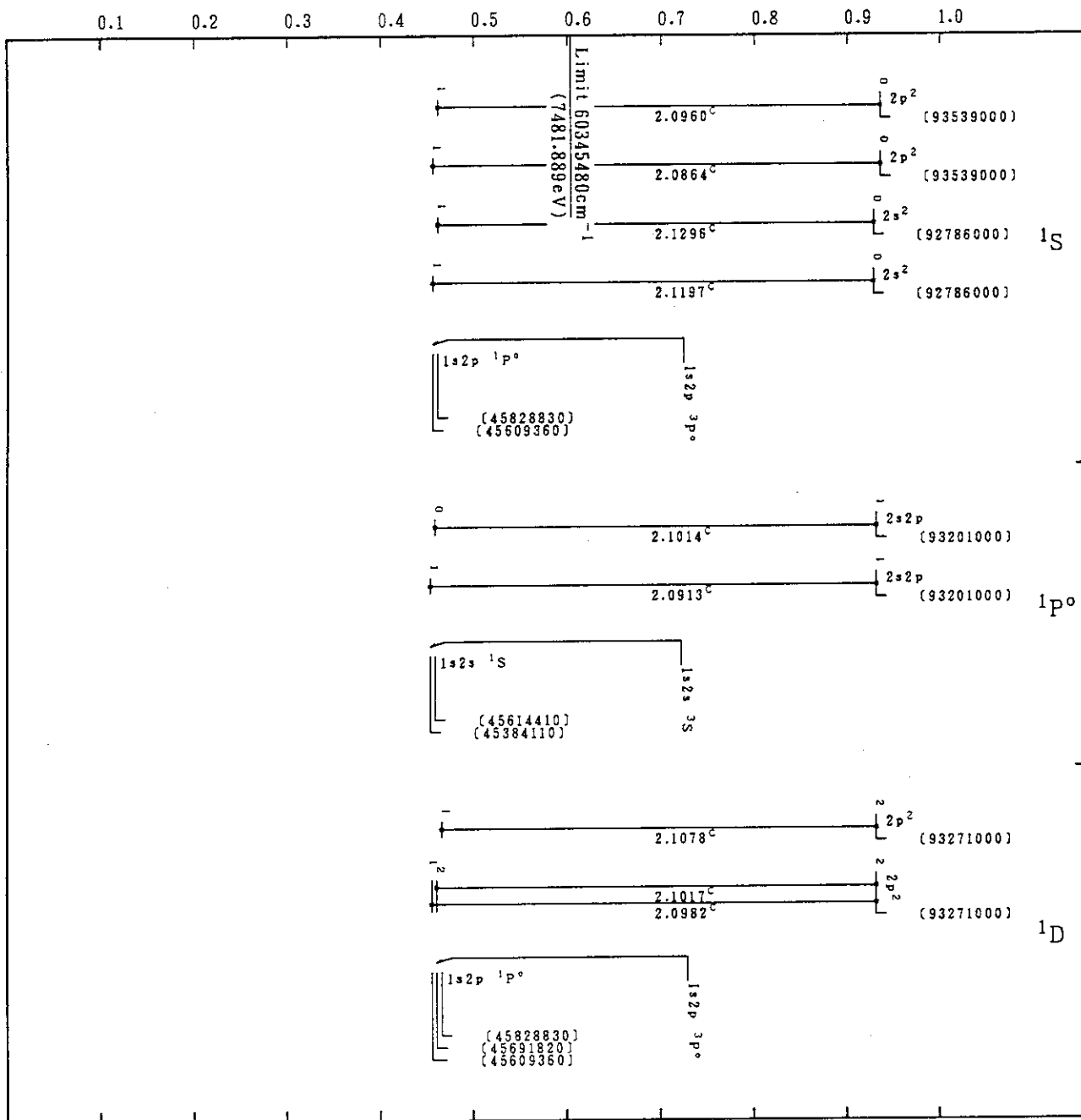
Cr XXIII(He-Sequence)
