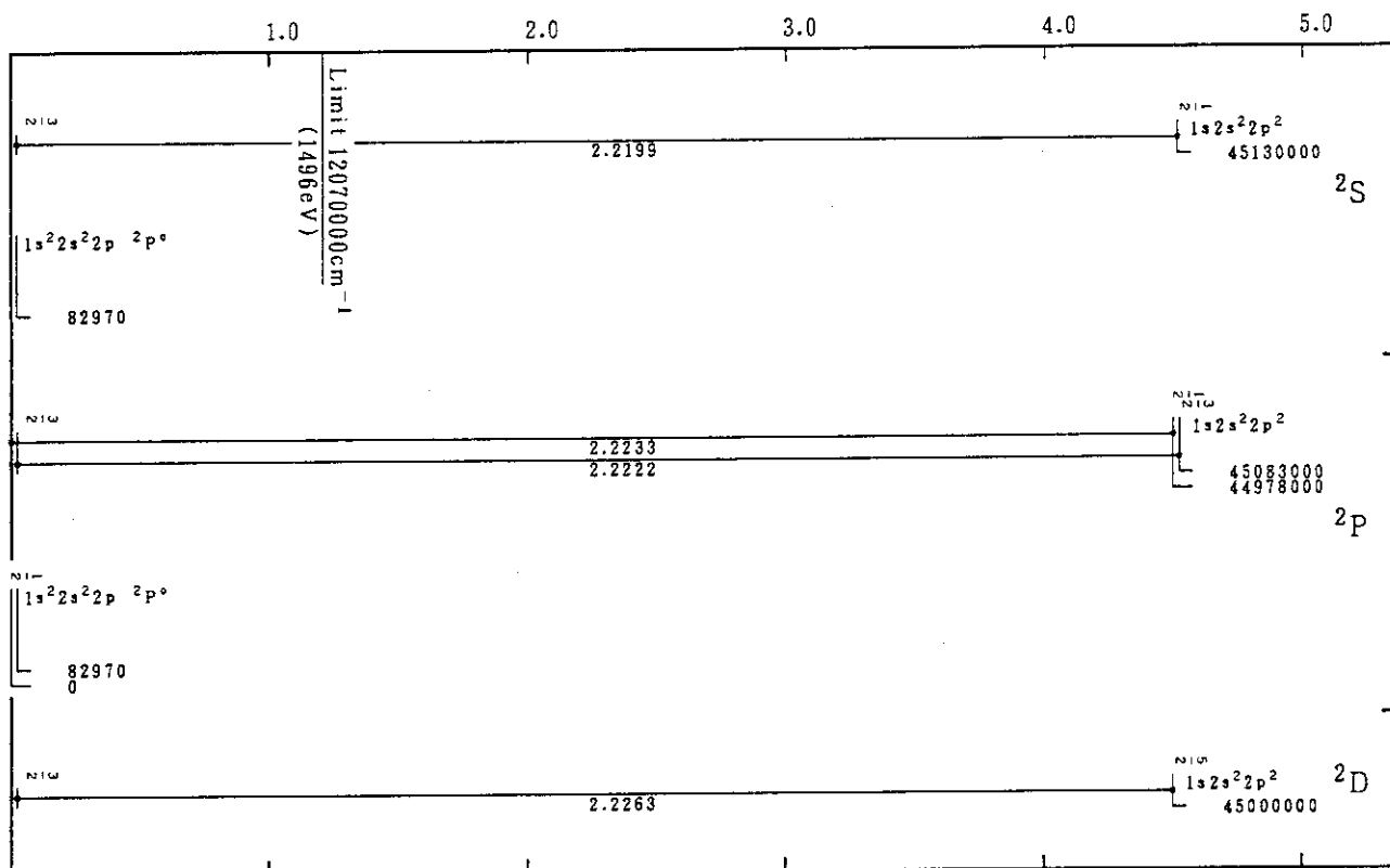
Cr XX(B-Sequence)
