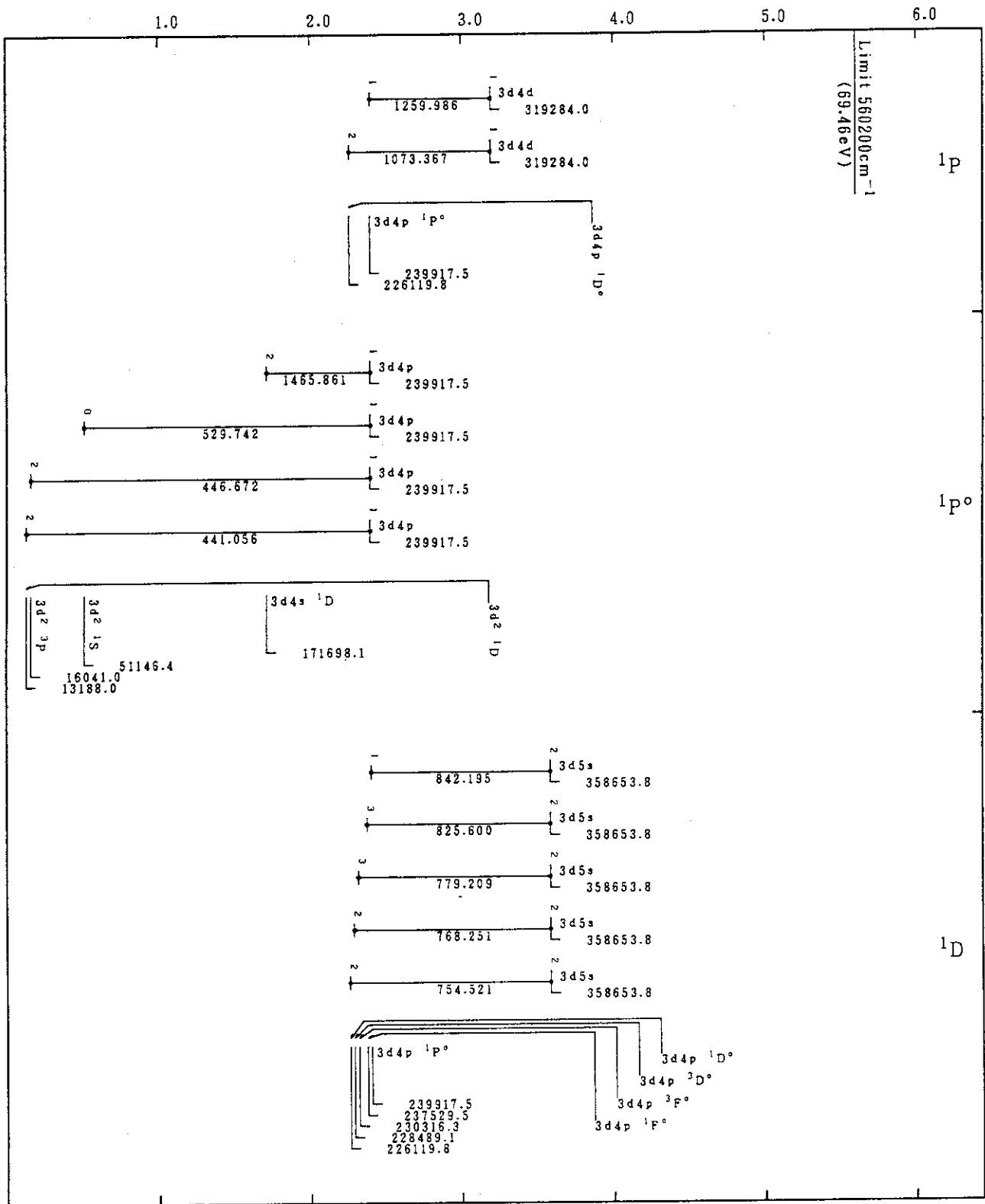
Cr V(Ca-Sequence)
