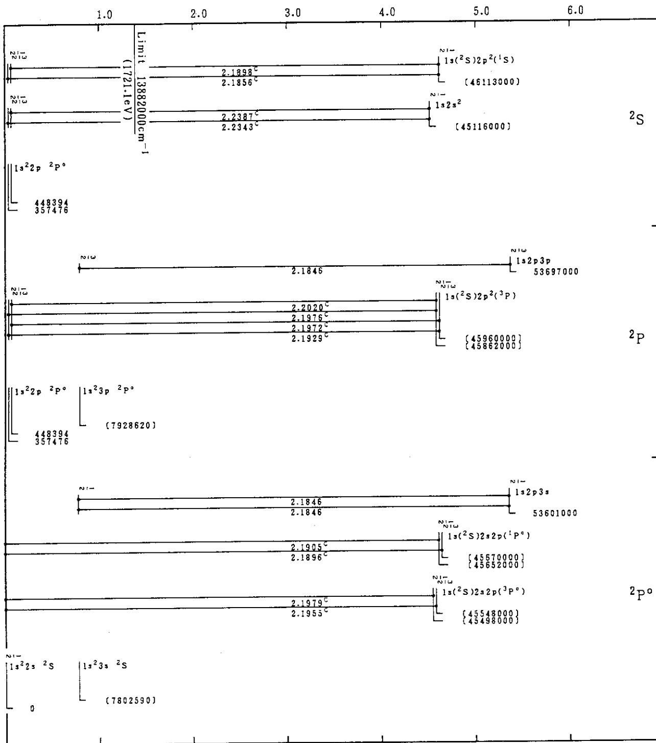
Cr XXII(Li-Sequence)
