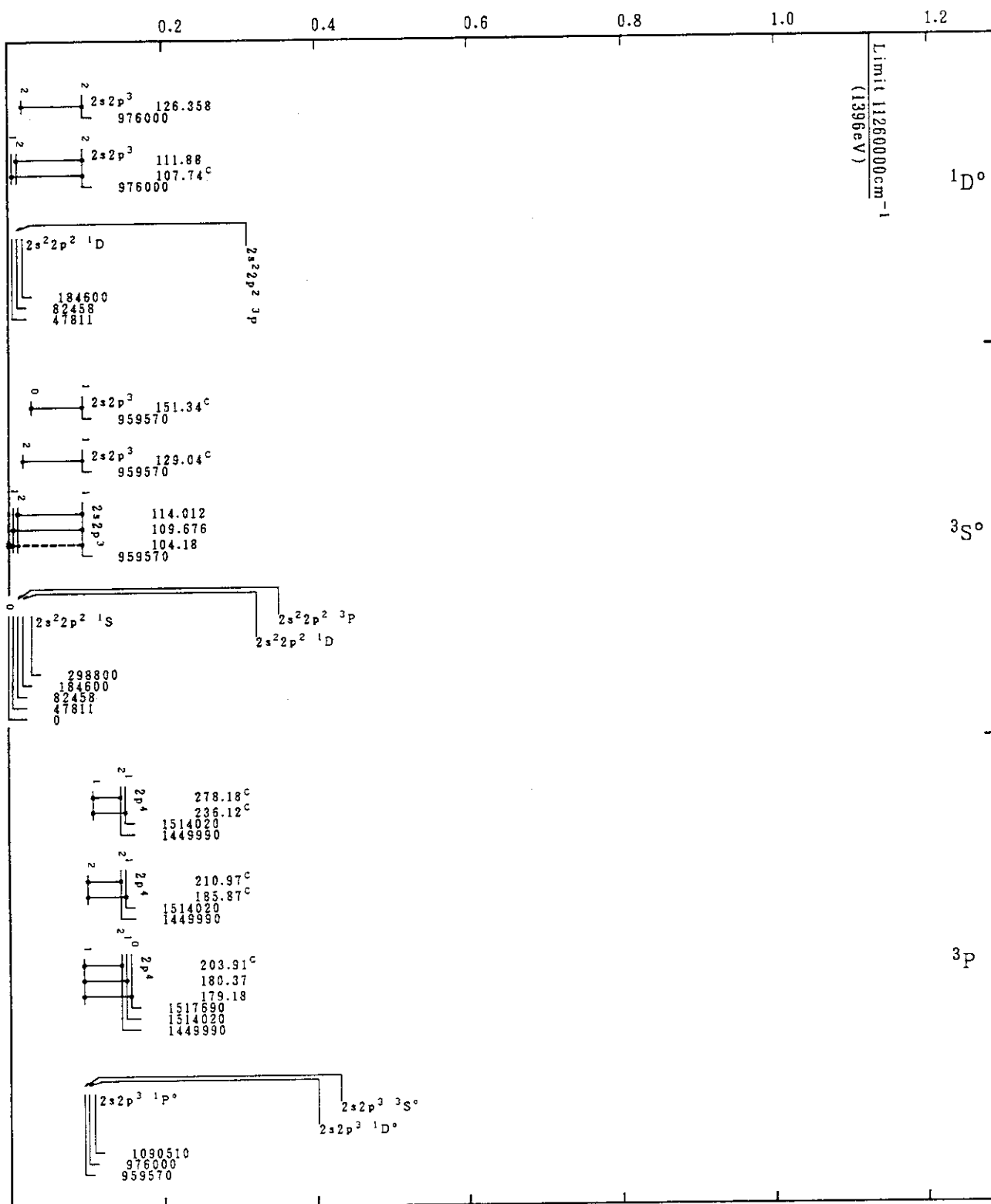
Cr XIX(C-Sequence)
