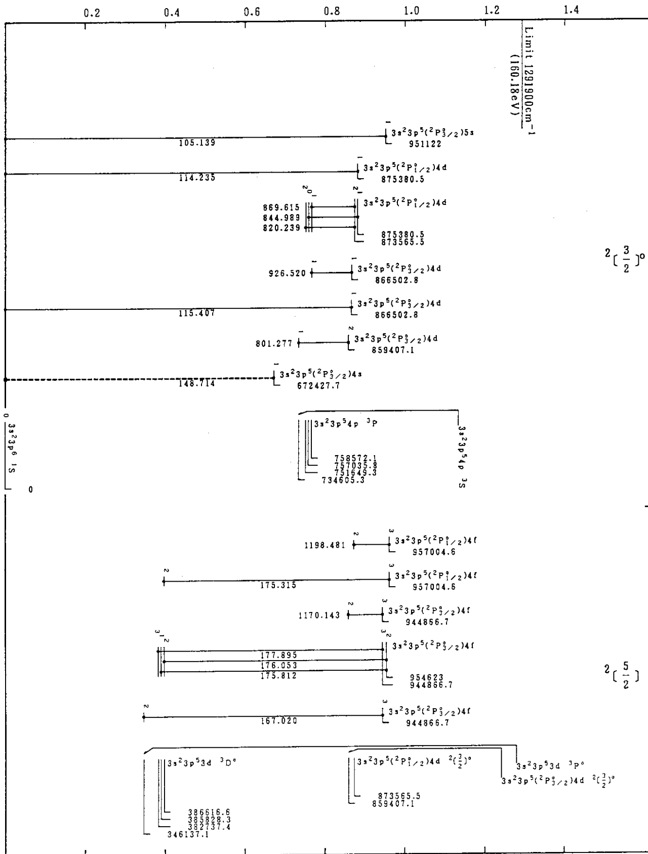
Cr VII(Ar-Sequence)
