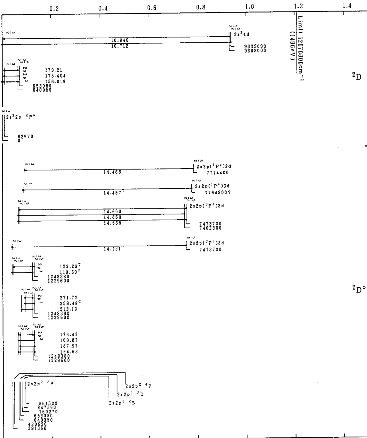
Cr XX(B-Sequence)
