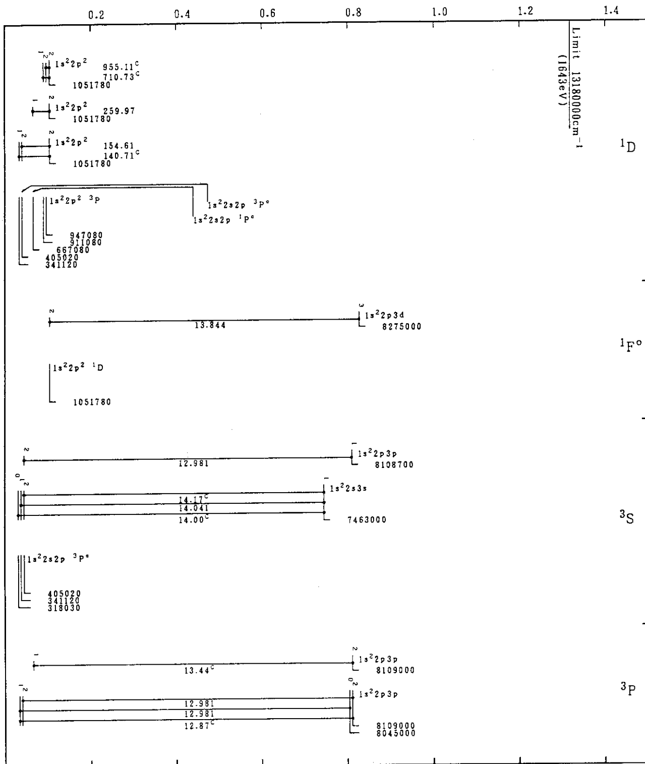
Cr XXI(Be-Sequence)
