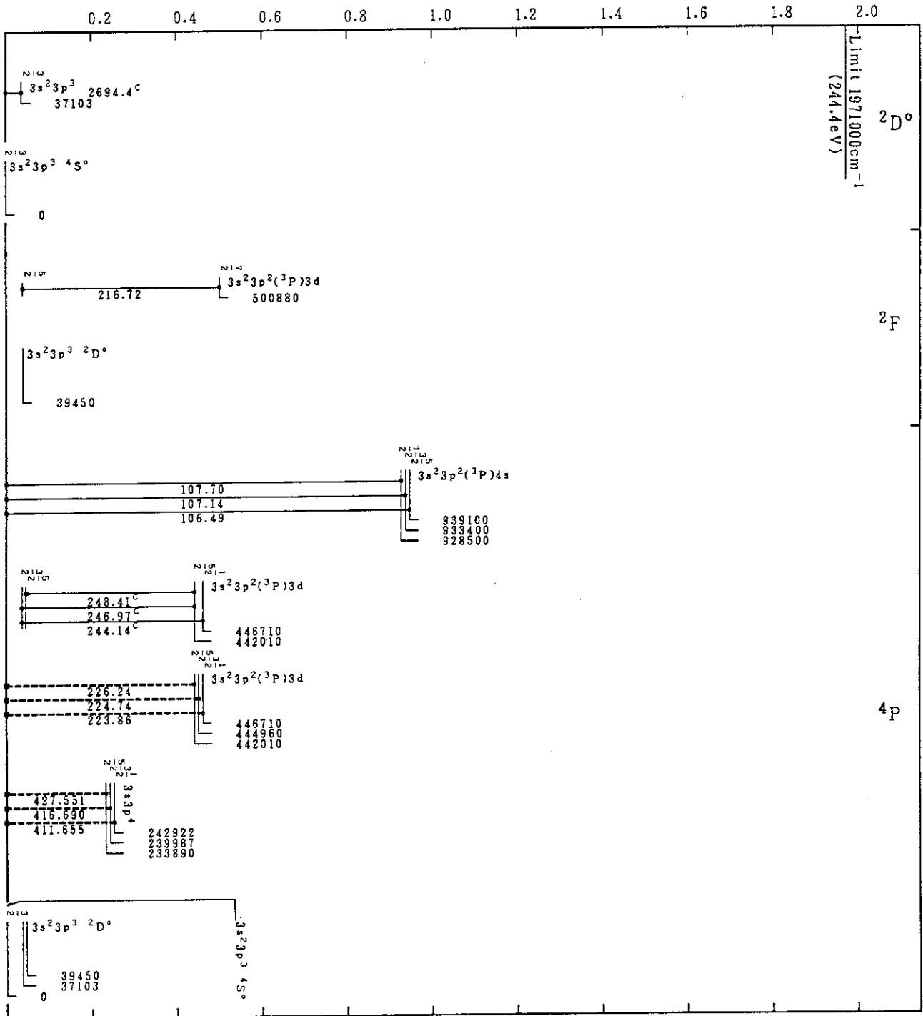
Cr X(P-Sequence)
