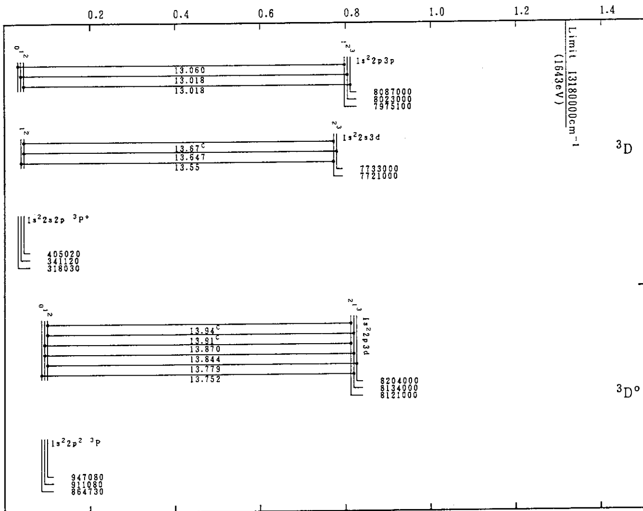
Cr XXI(Be-Sequence)
