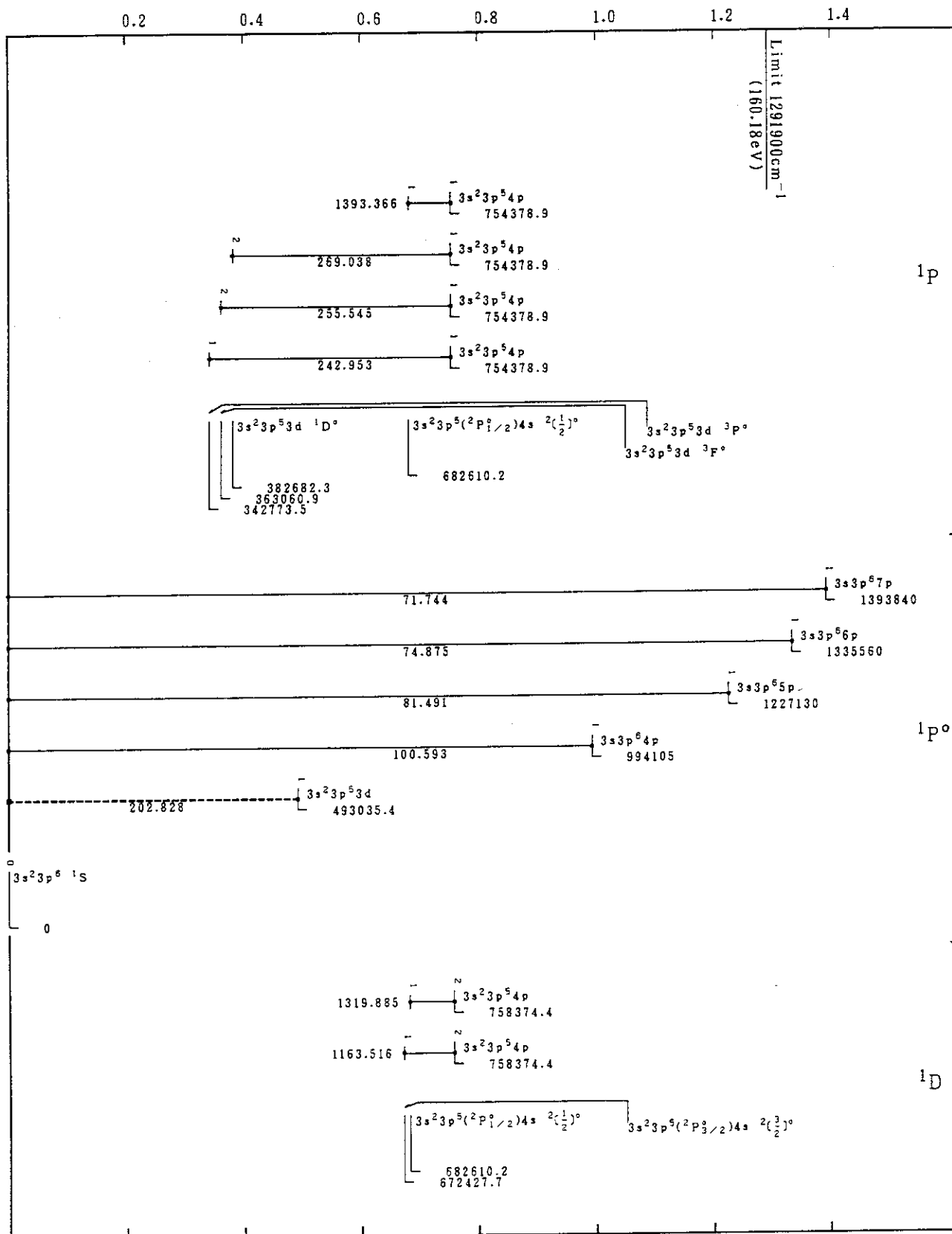
Cr VII(Ar-Sequence)
