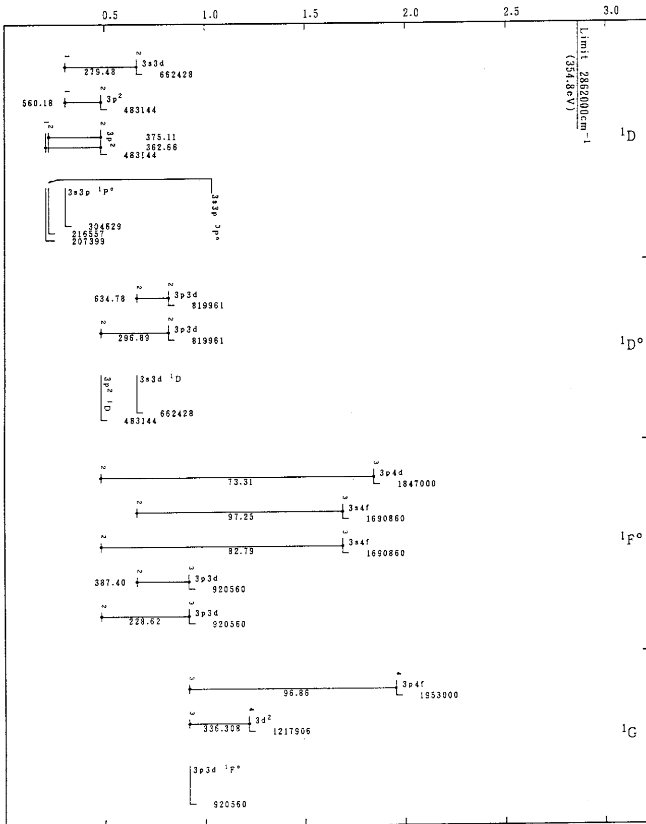
Cr XIII(Mg-Sequence)
