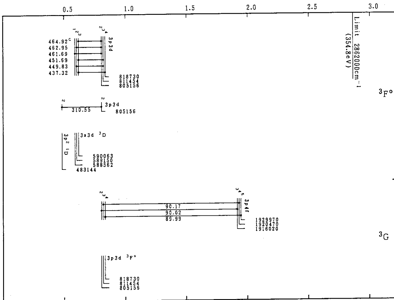
Cr XIII(Mg-Sequence)
