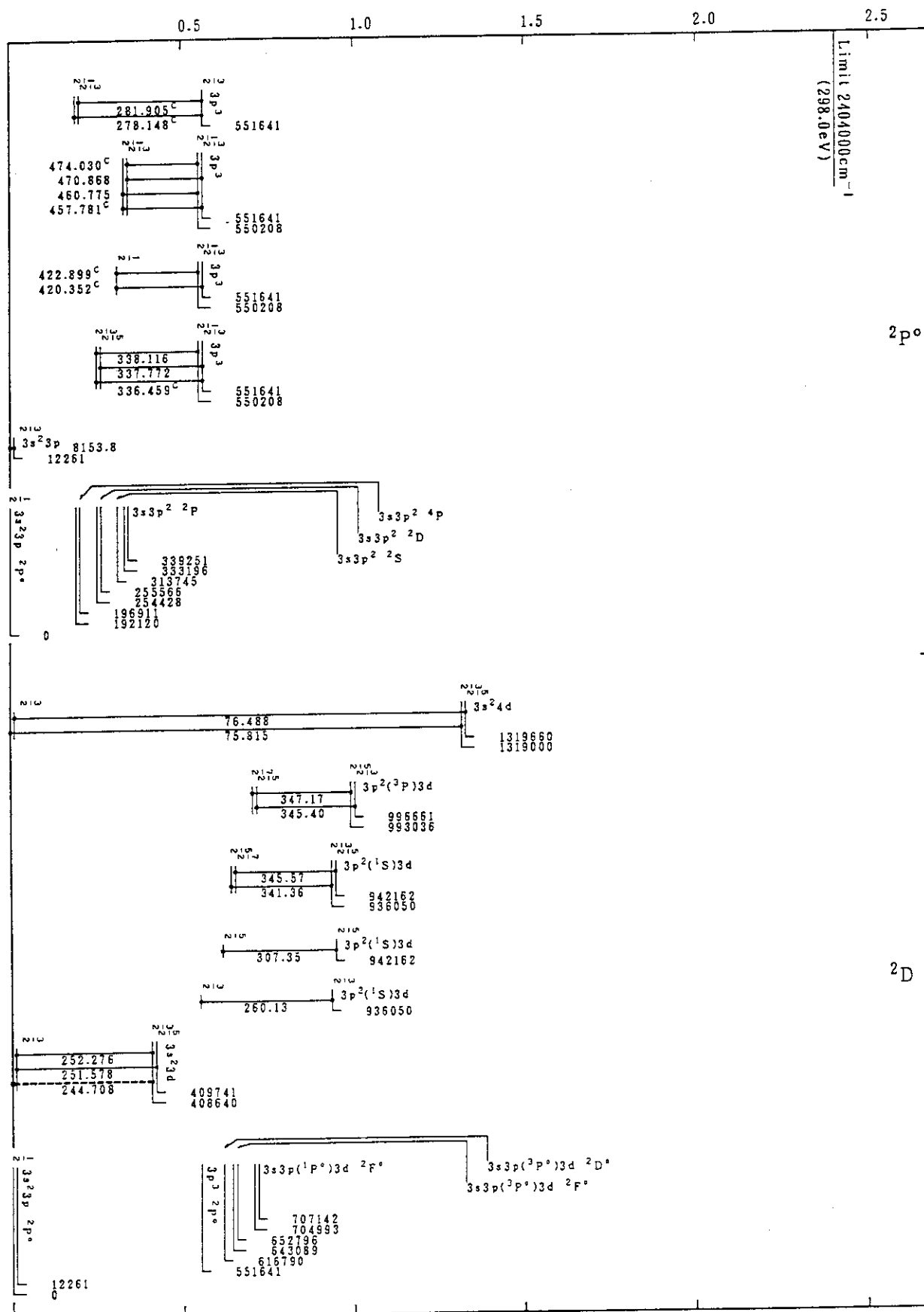
Cr XII(Al-Sequence)
