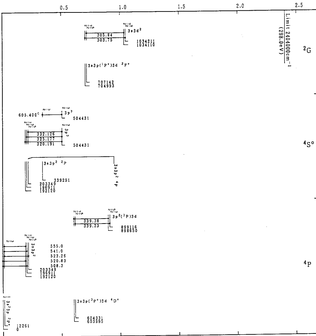
Cr XII(Al-Sequence)
