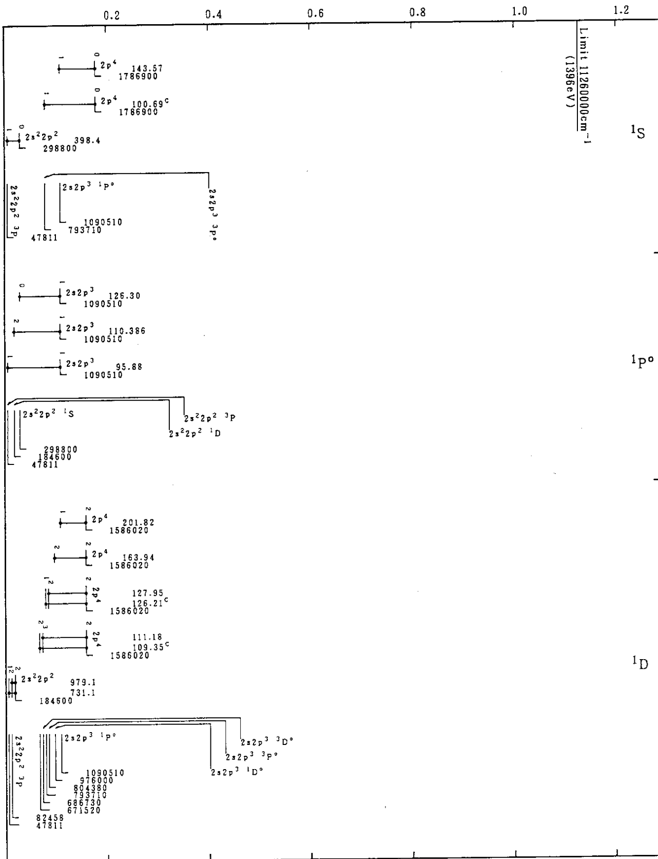
Cr XIX(C-Sequence)
