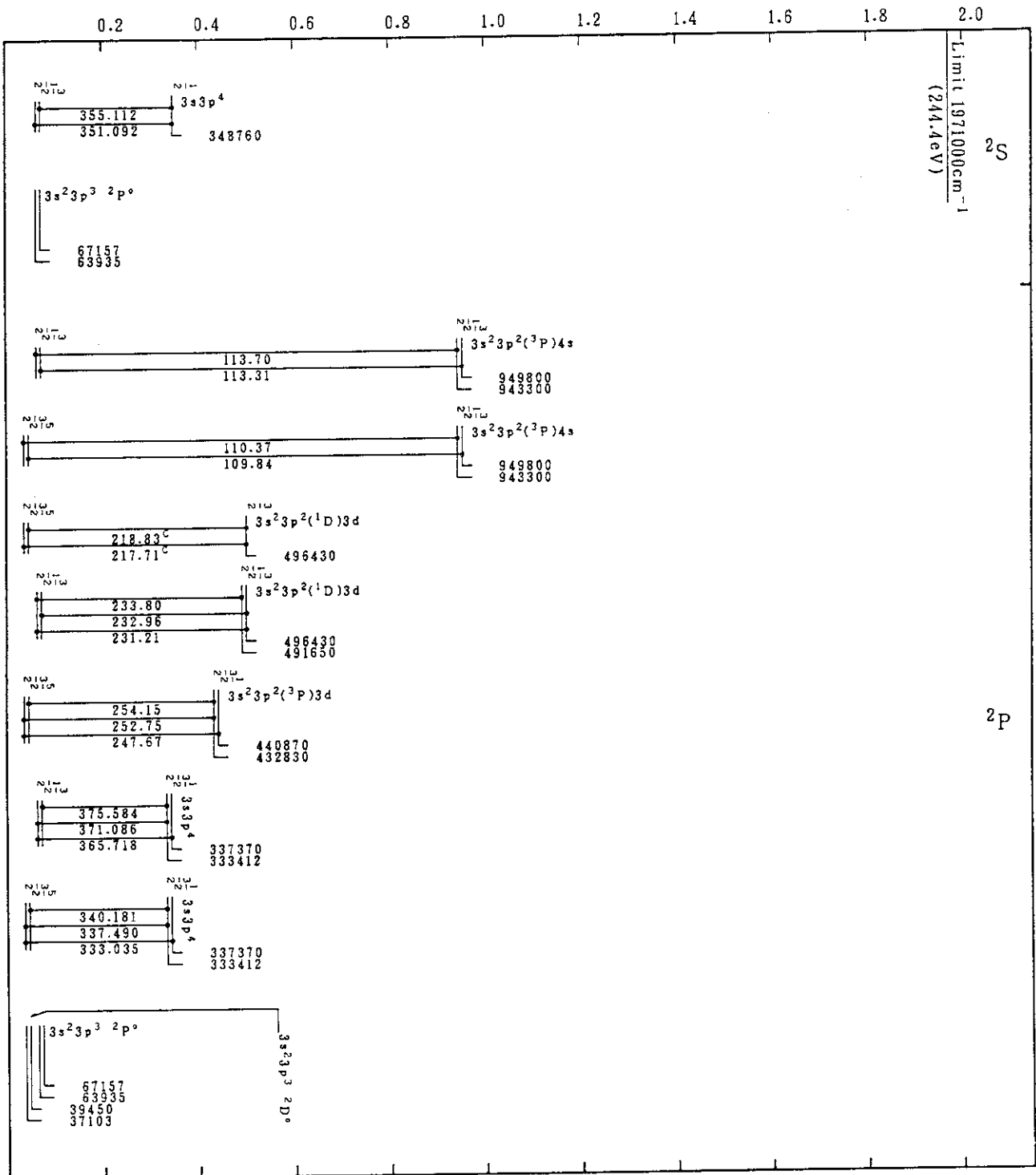
Cr X(P-Sequence)
