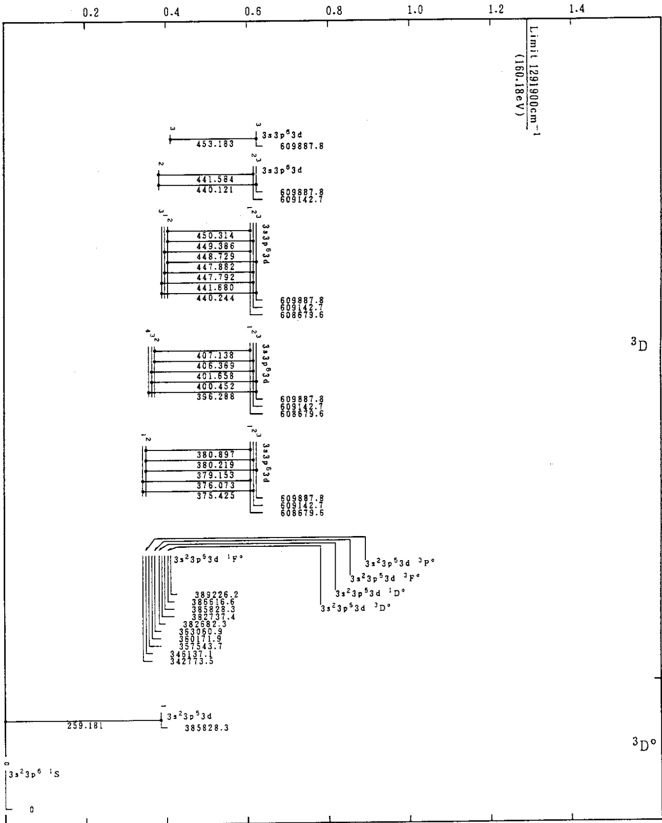
Cr VII(Ar-Sequence)
