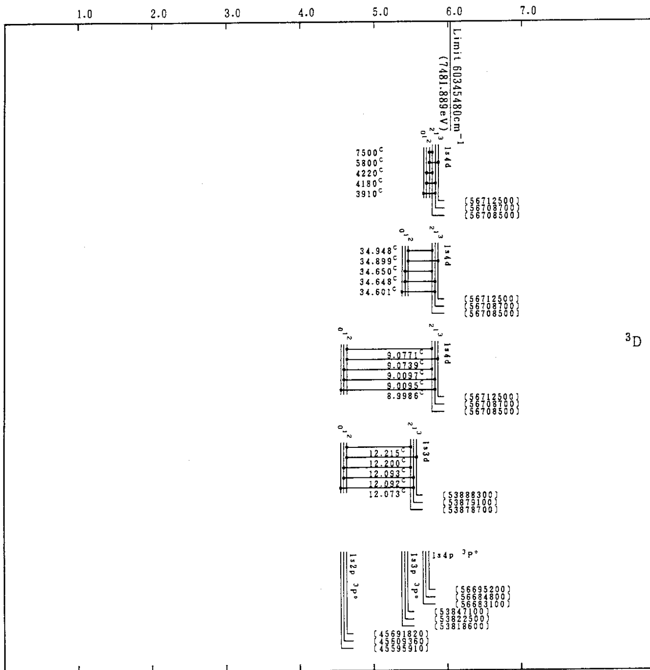
Cr XXIII(He-Sequence)
