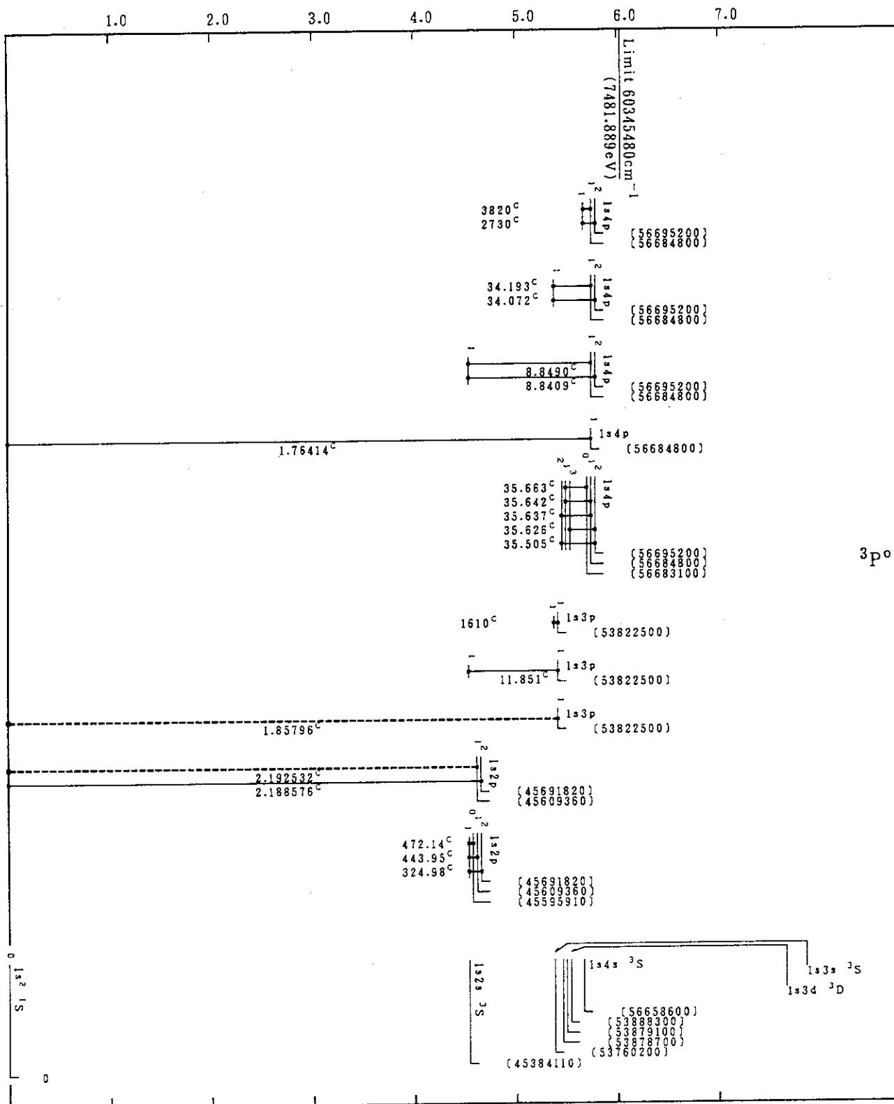
Cr XXIII(He-Sequence)
