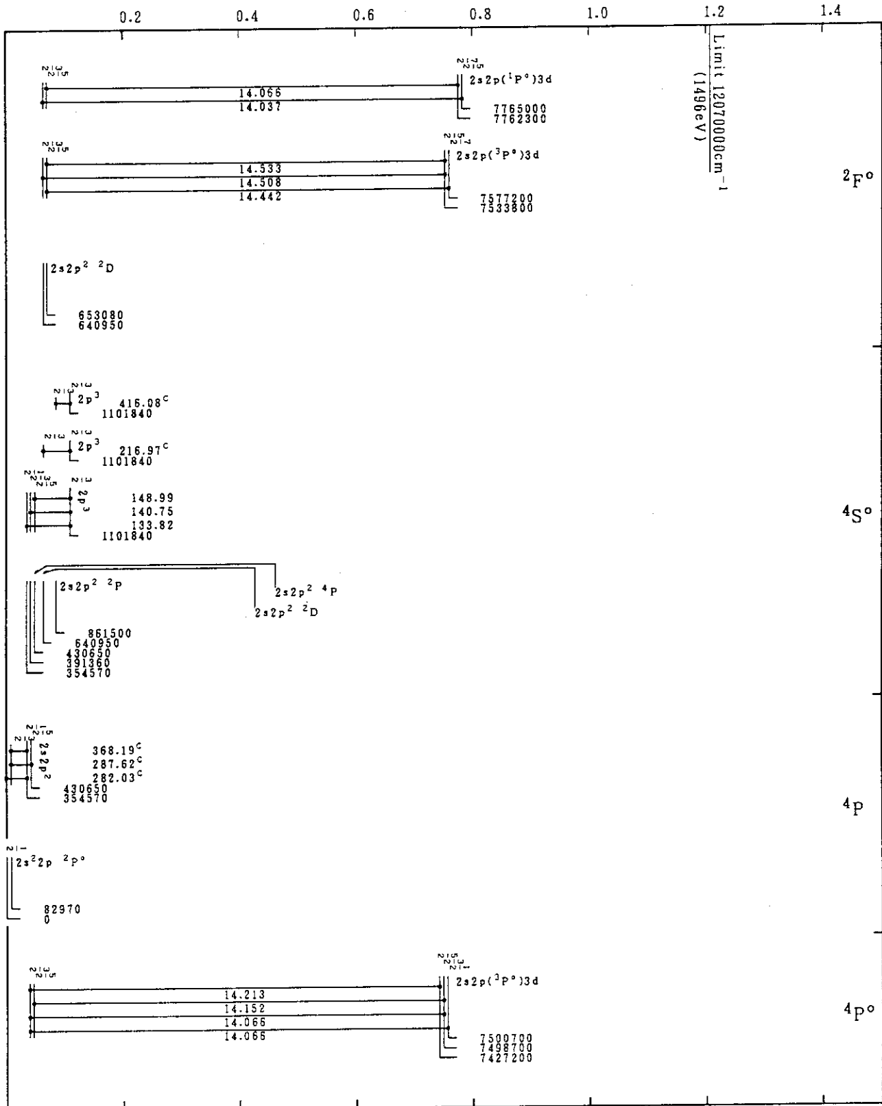
Cr XX(B-Sequence)
