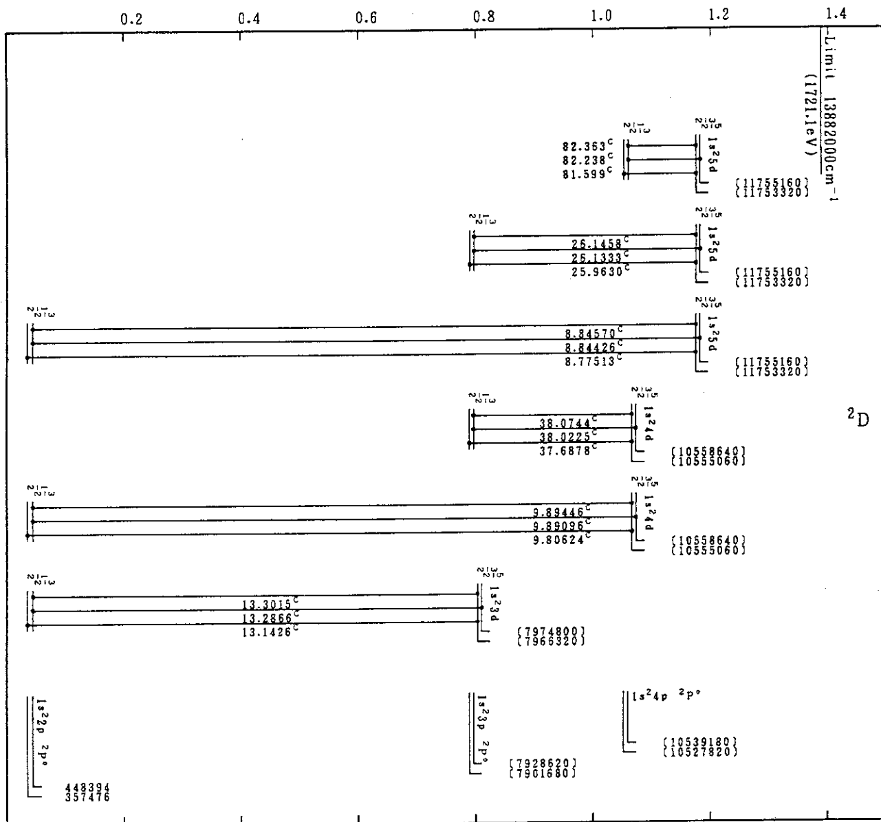
Cr XXII(Li-Sequence)
