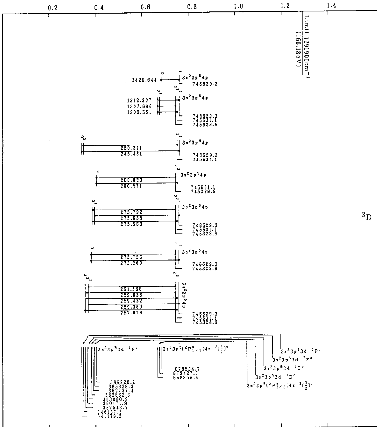
Cr VII(Ar-Sequence)
