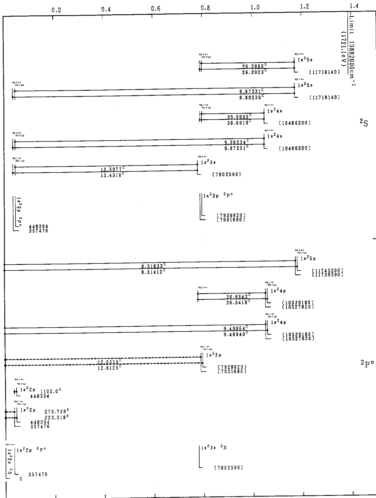
Cr XXII(Li-Sequence)
