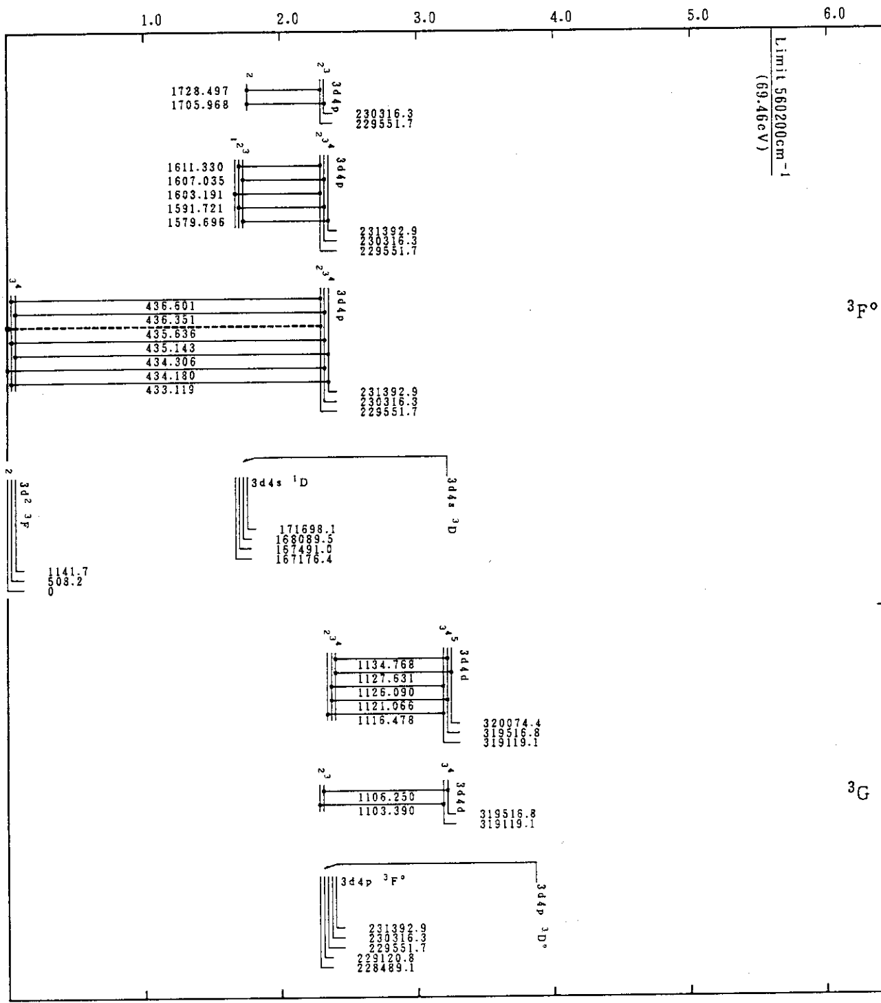
Cr V(Ca-Sequence)
