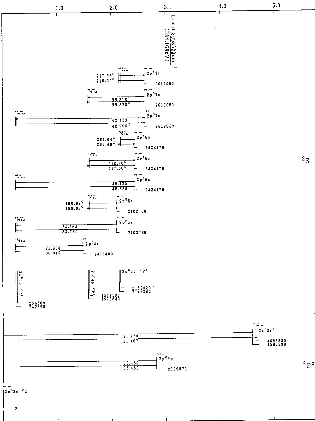
Cr XIV(Na-Sequence)
