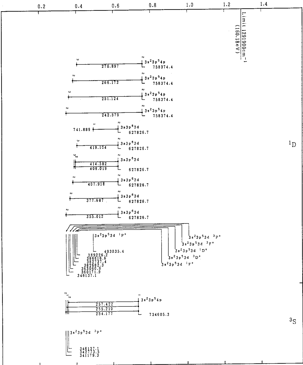
Cr VII(Ar-Sequence)
