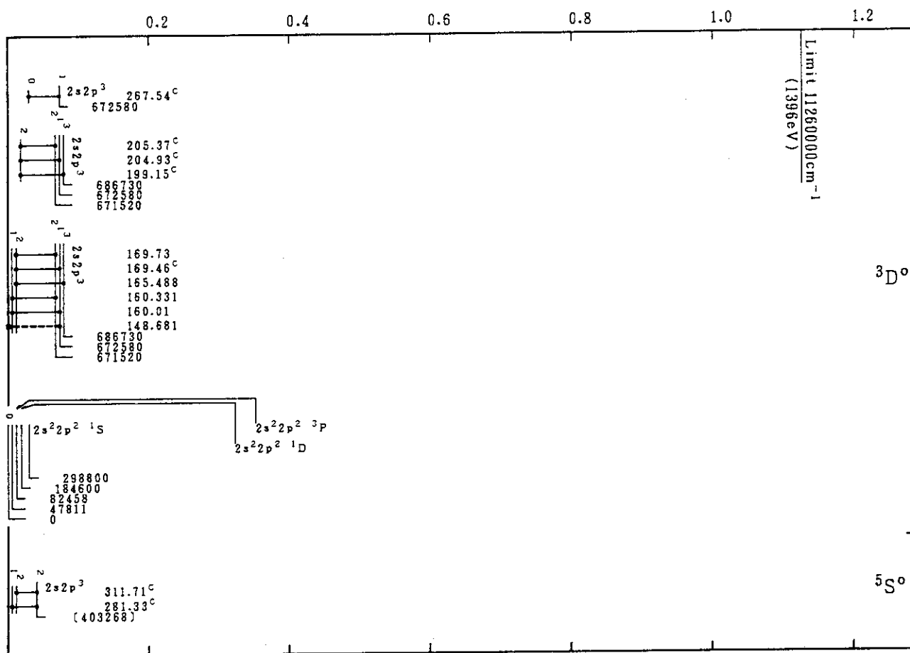
Cr XIX(C-Sequence)
