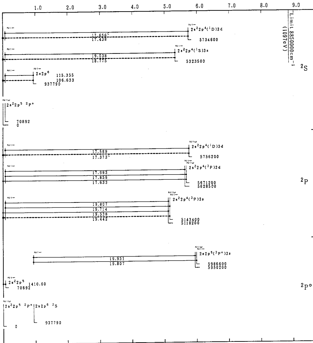
Cr XVI(F-Sequence)
