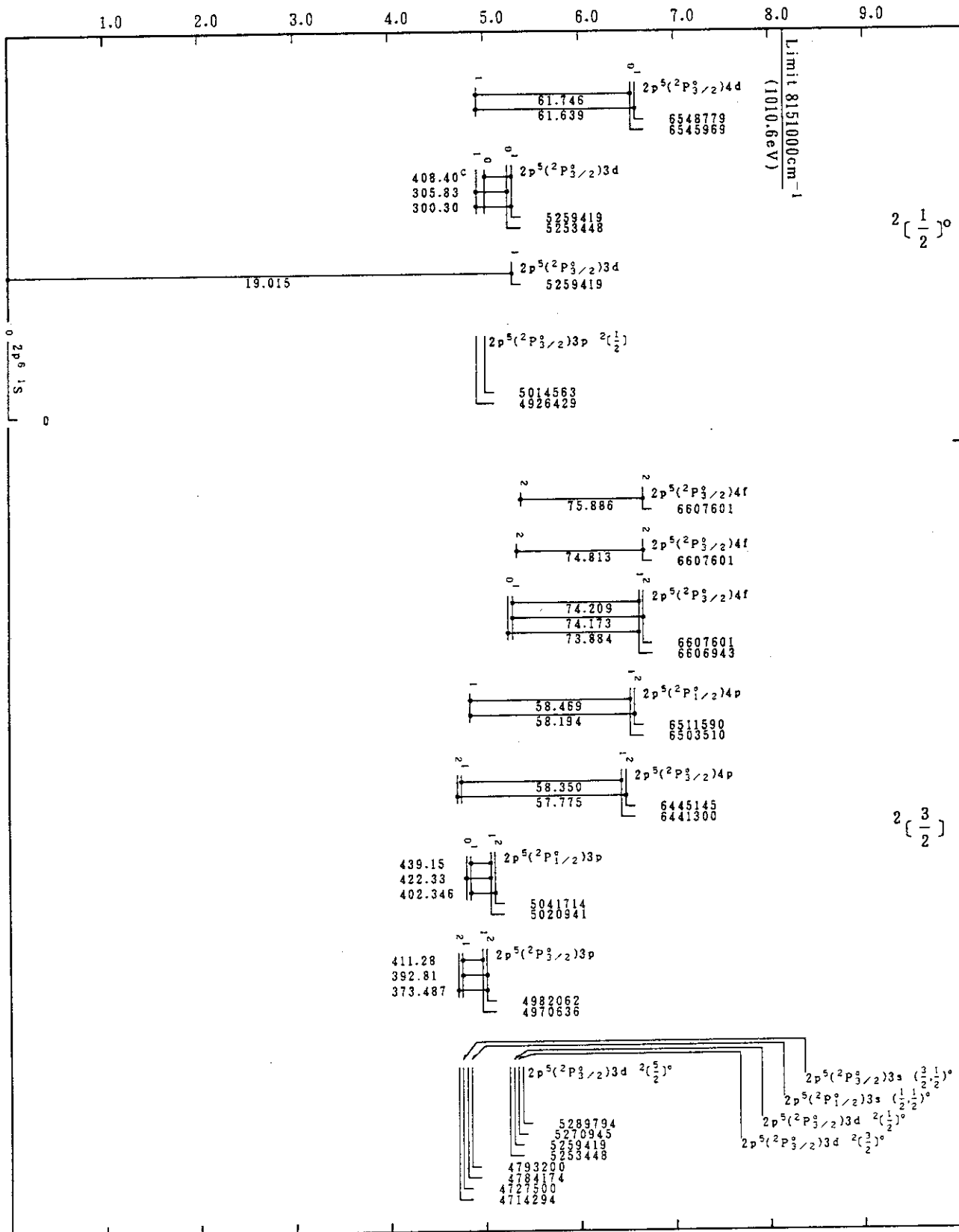
Cr XV(Ne-Sequence)
