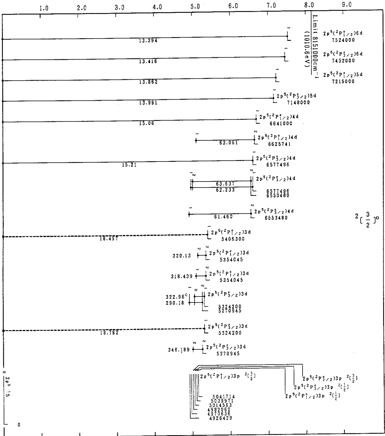
Cr XV(Ne-Sequence)
