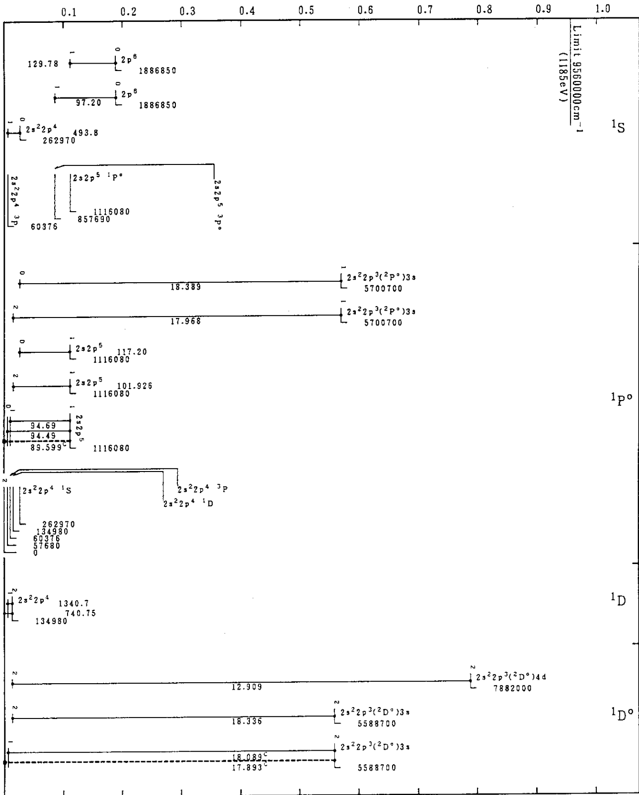
Cr XVII(O-Sequence)
