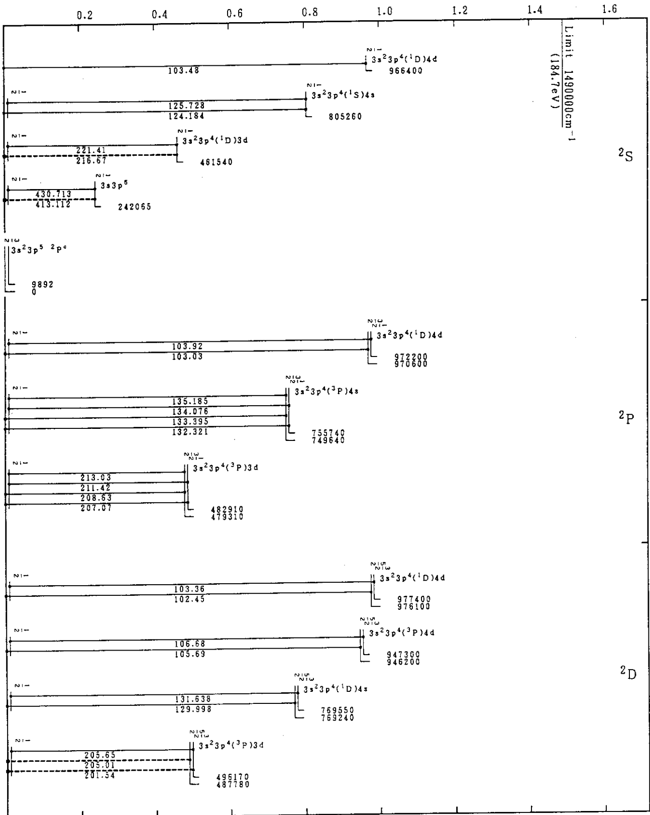
Cr VIII(Cl-Sequence)
