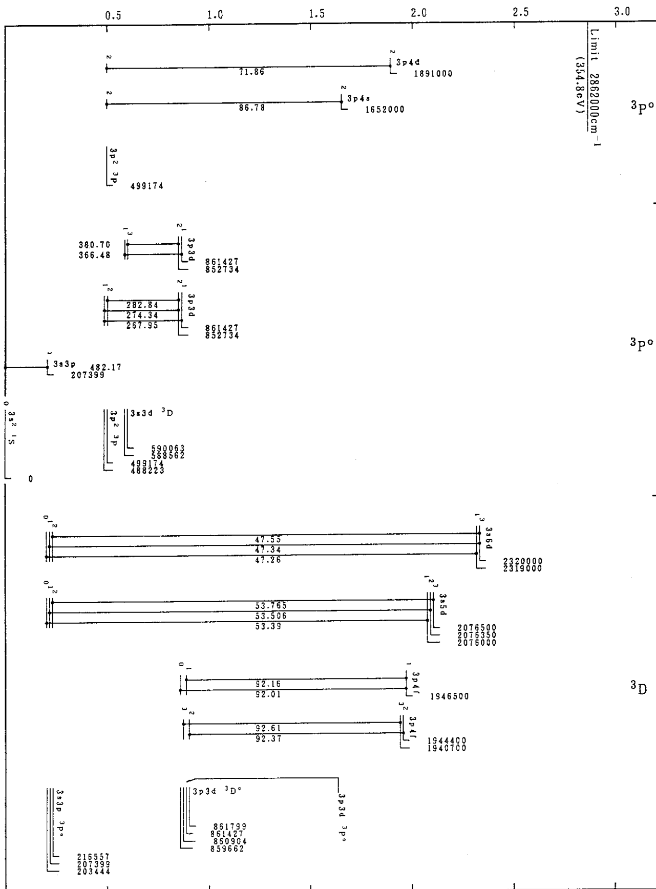
Cr XIII(Mg-Sequence)
