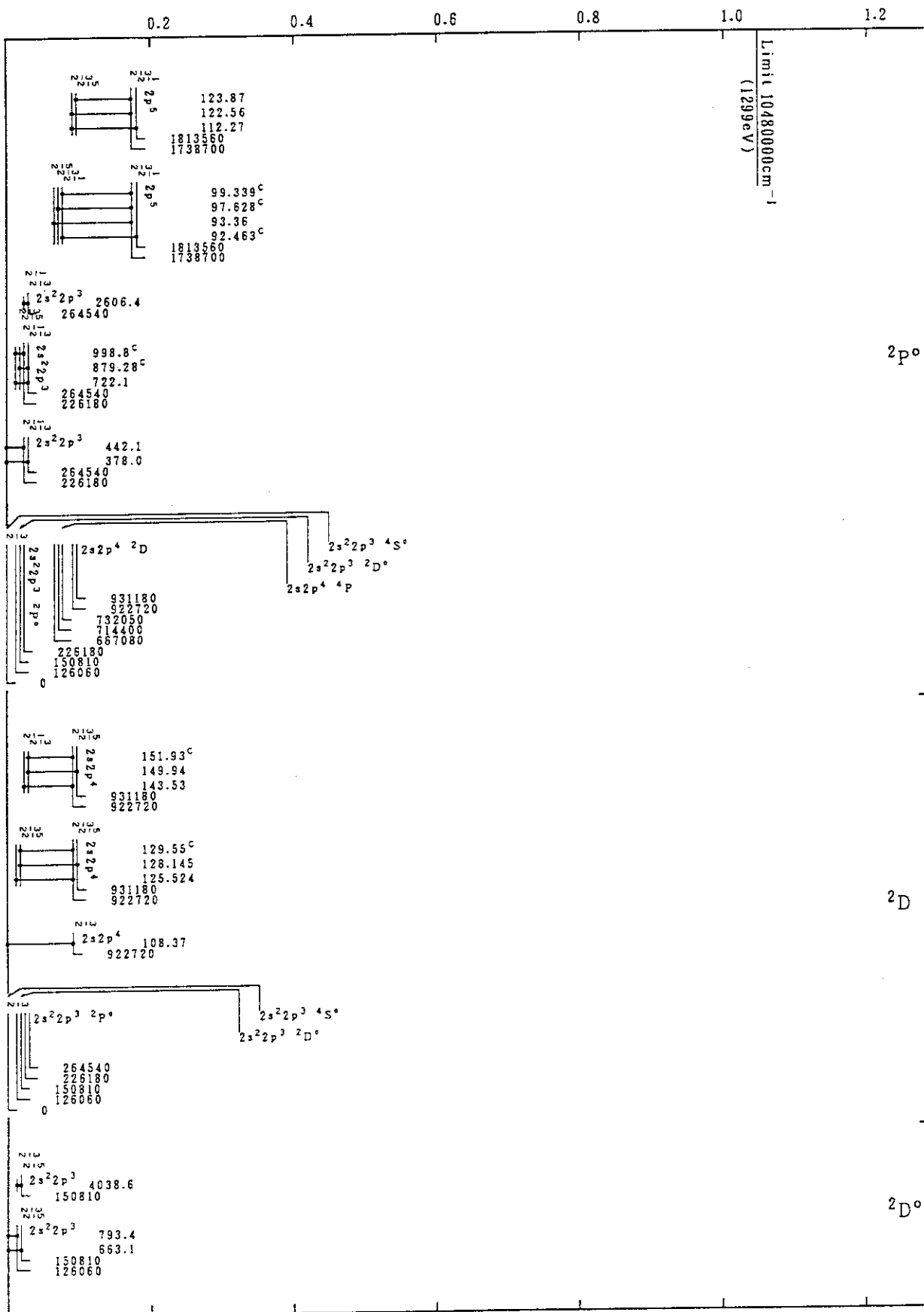
Cr XVIII(N-Sequence)
