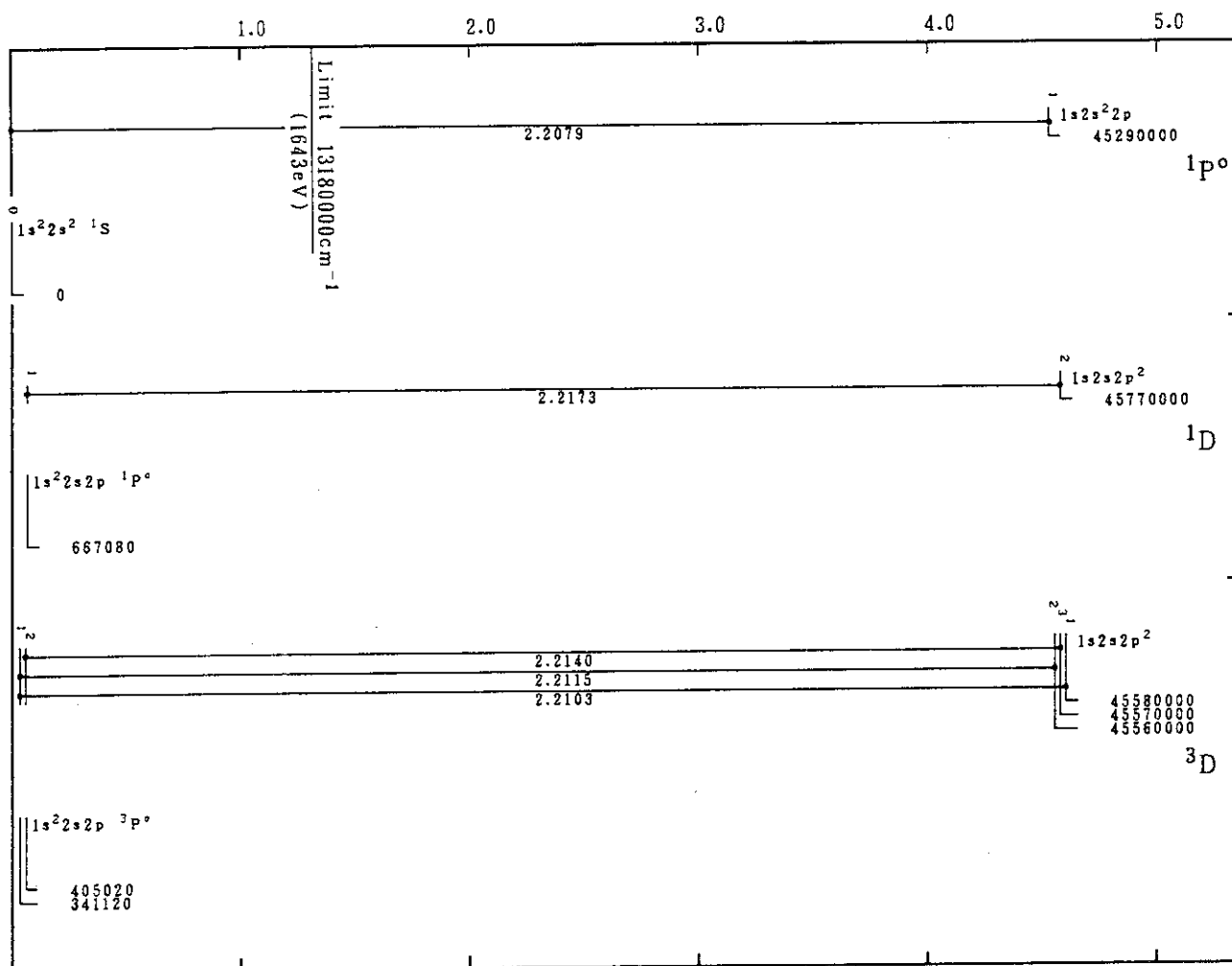
Cr XXI(Be-Sequence)
