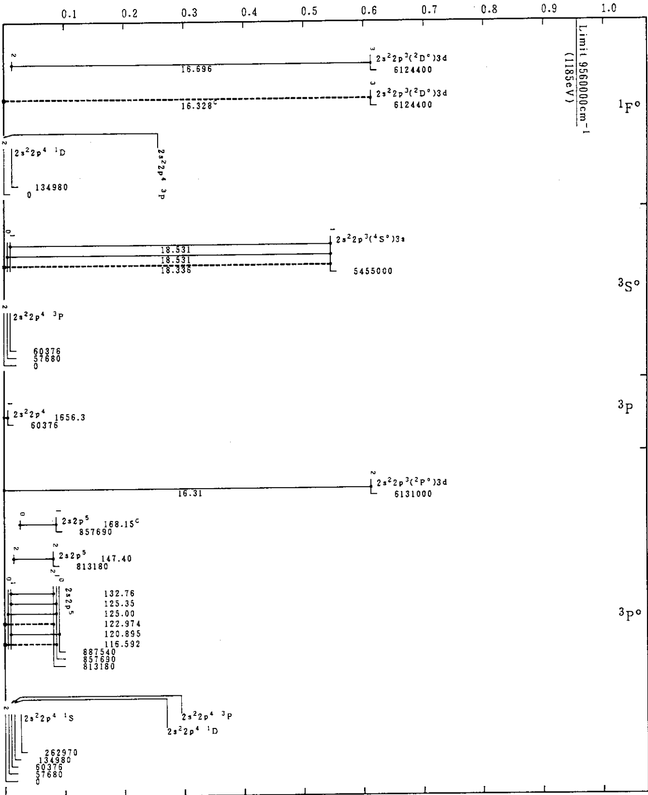
Cr XVII(O-Sequence)
