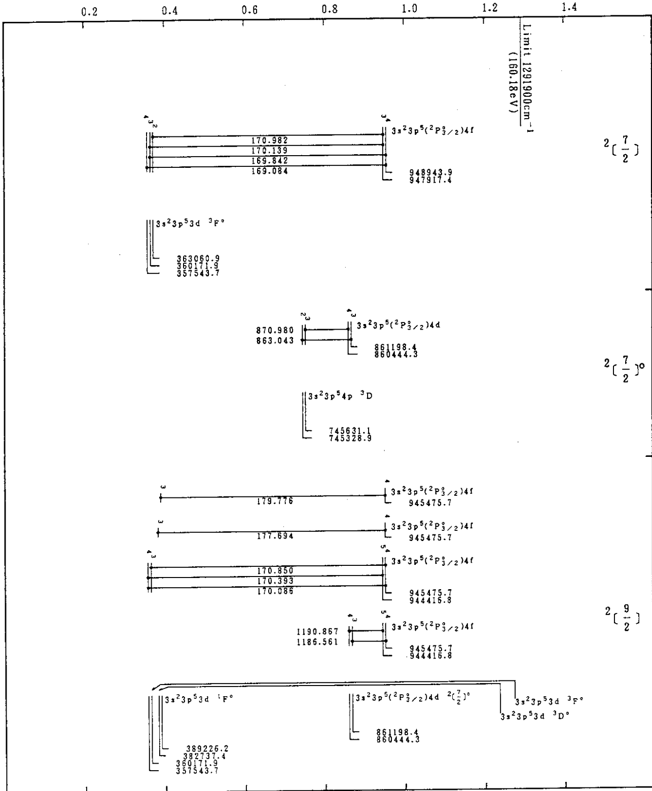
Cr VII(Ar-Sequence)
