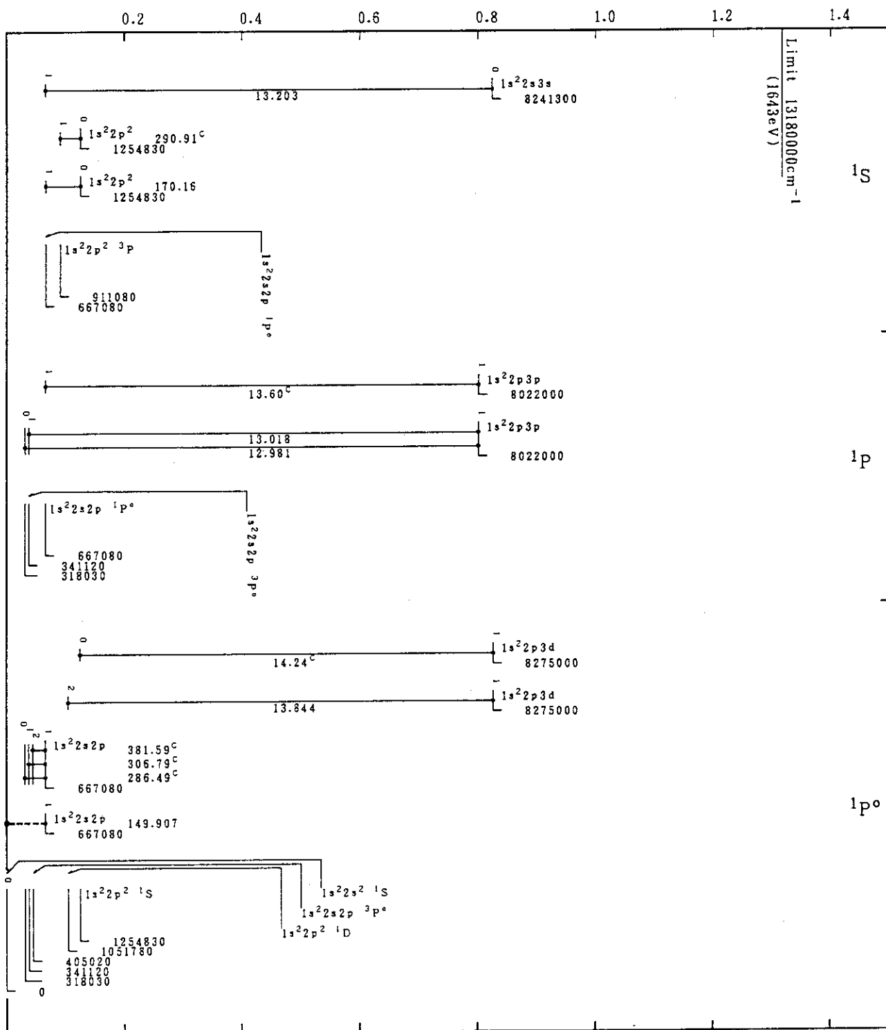
Cr XXI(Be-Sequence)
