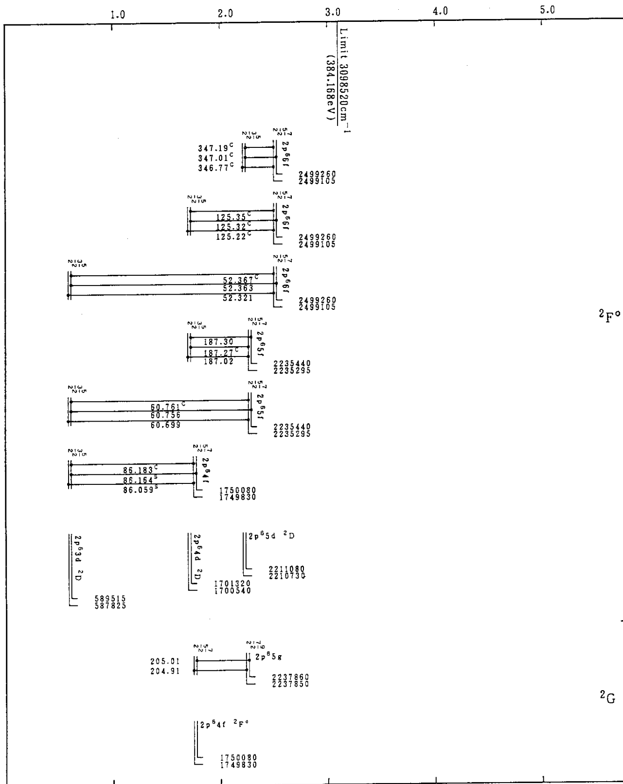
Cr XIV(Na-Sequence)
