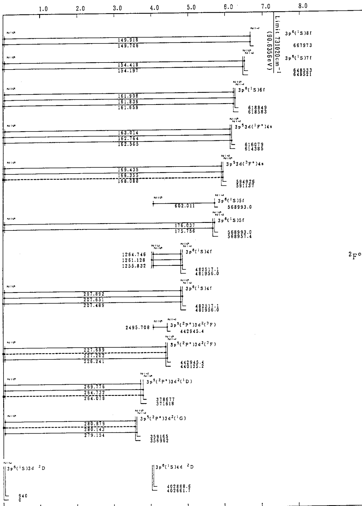
Cr VI(K-Sequence)
