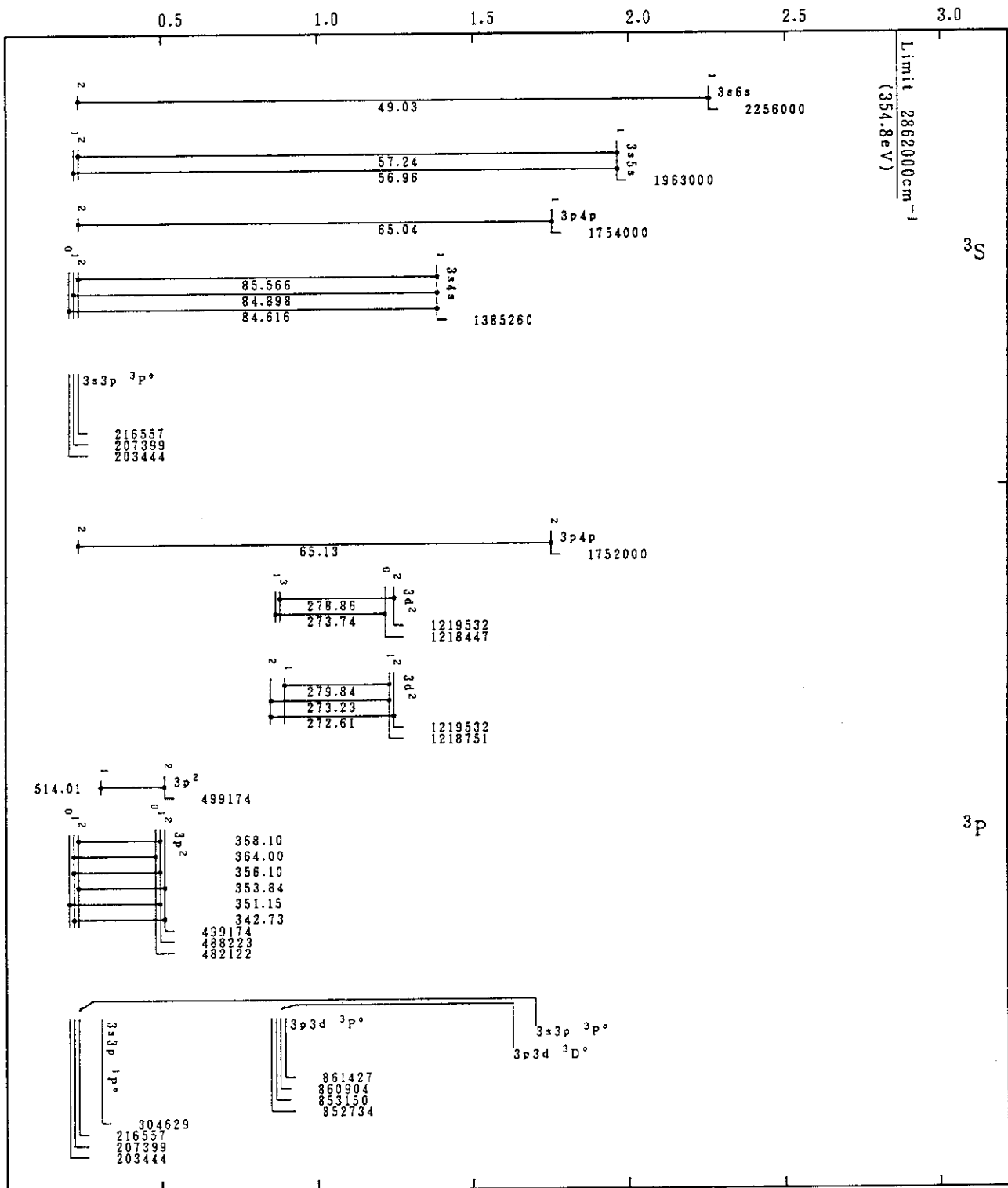
Cr XIII(Mg-Sequence)
