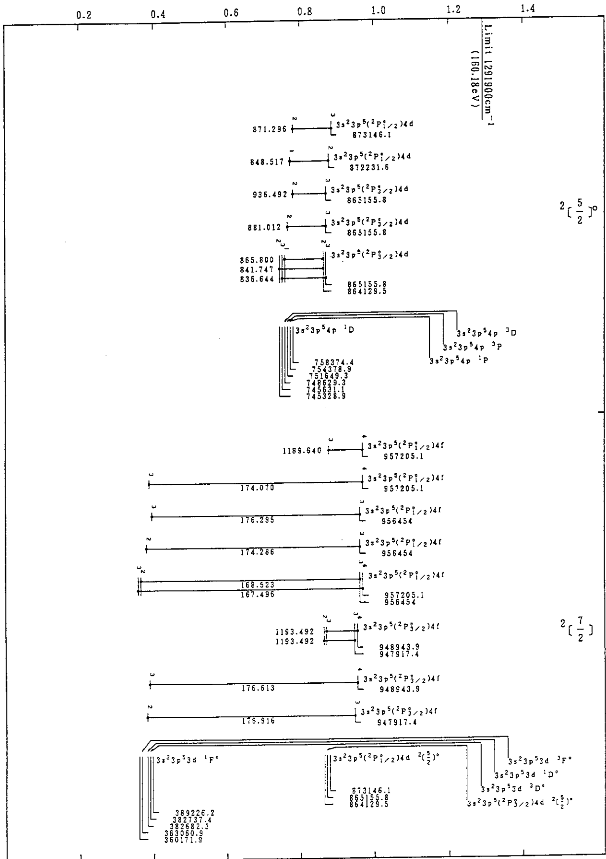
Cr VII(Ar-Sequence)
