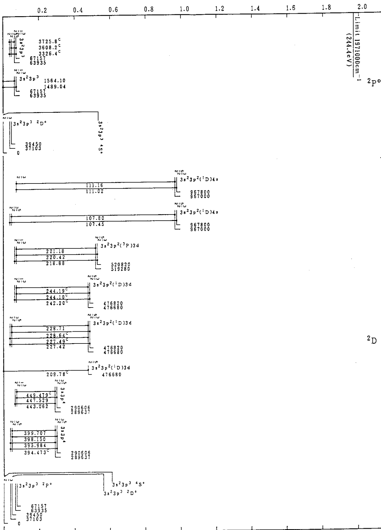
Cr X(P-Sequence)
