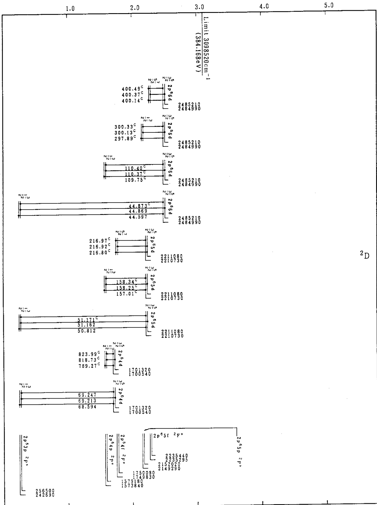
Cr XIV(Na-Sequence)
