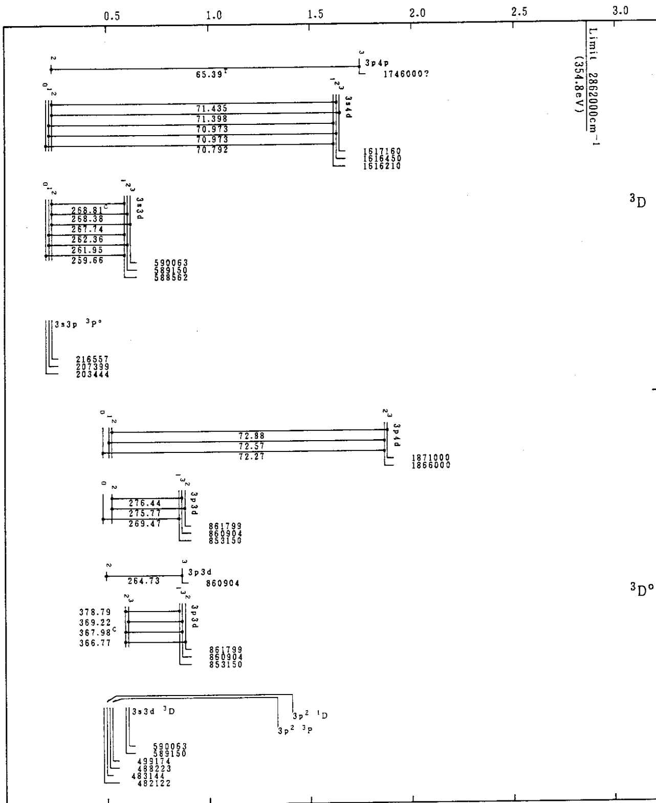
Cr XIII(Mg-Sequence)
