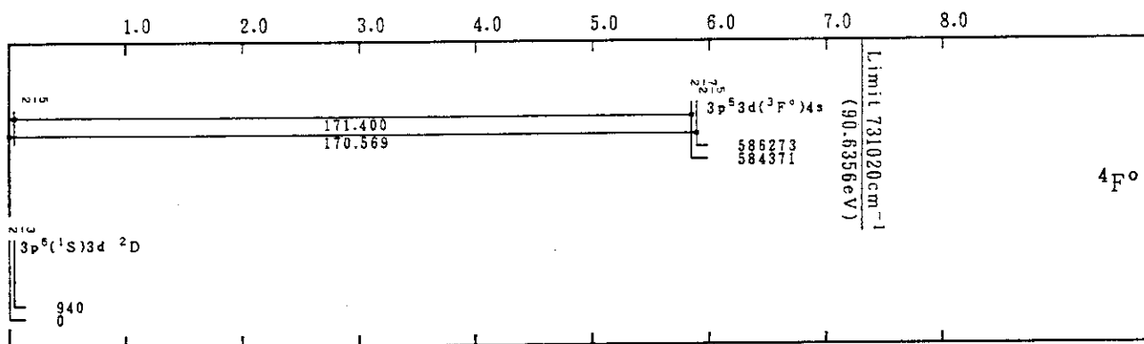
Cr VI(K-Sequence)
