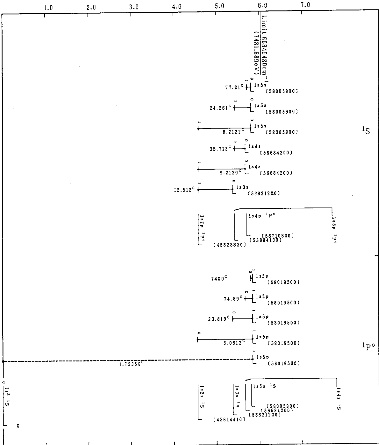
Cr XXIII(He-Sequence)
