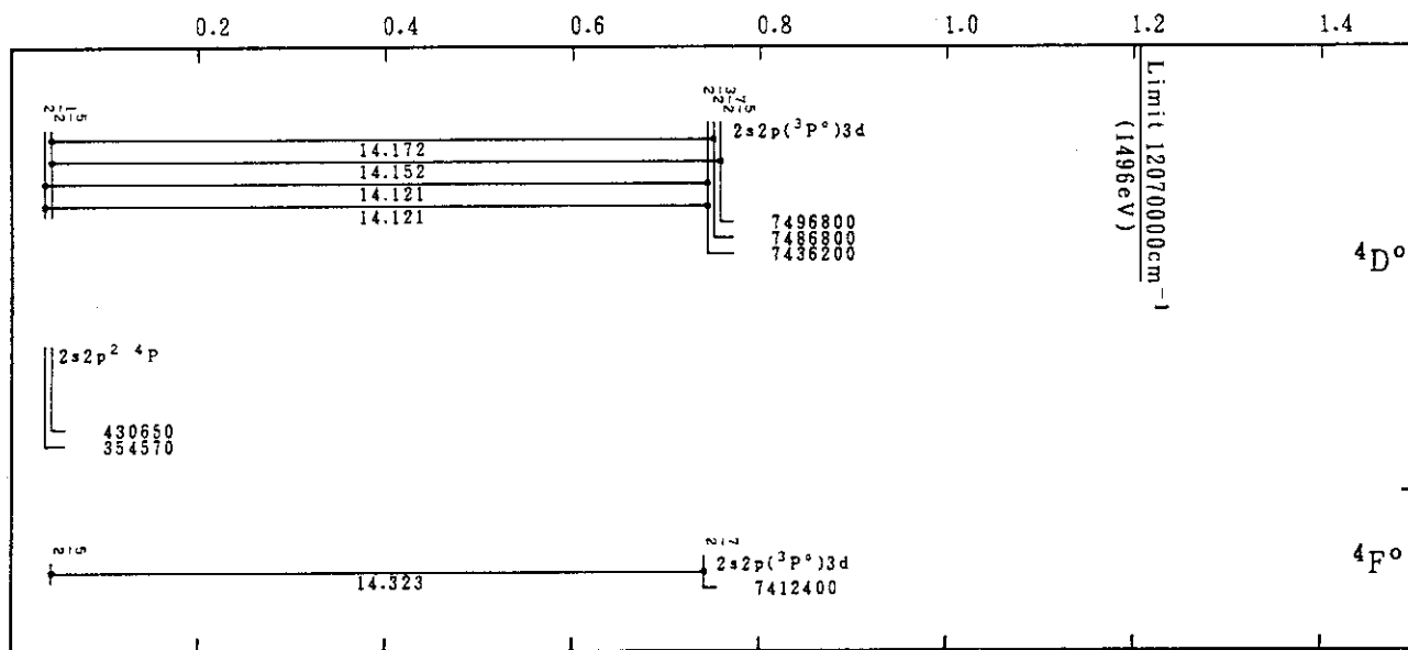
Cr XX(B-Sequence)
