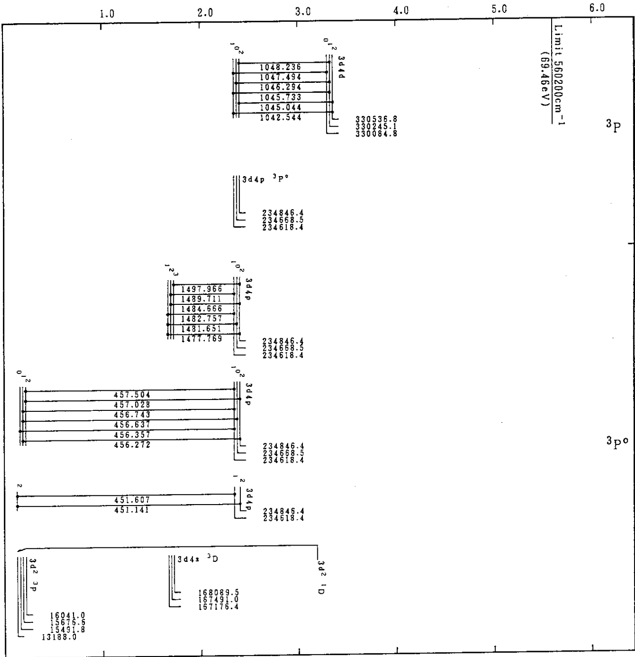
Cr V(Ca-Sequence)
