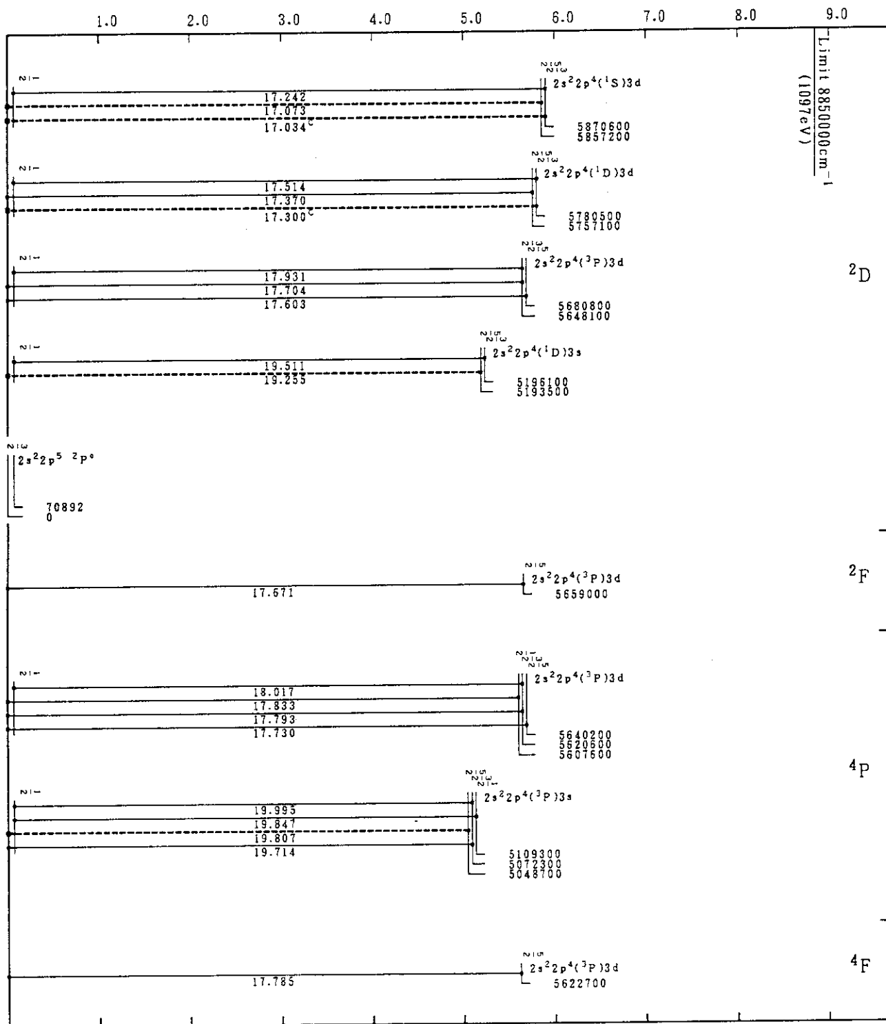
Cr XVI(F-Sequence)
