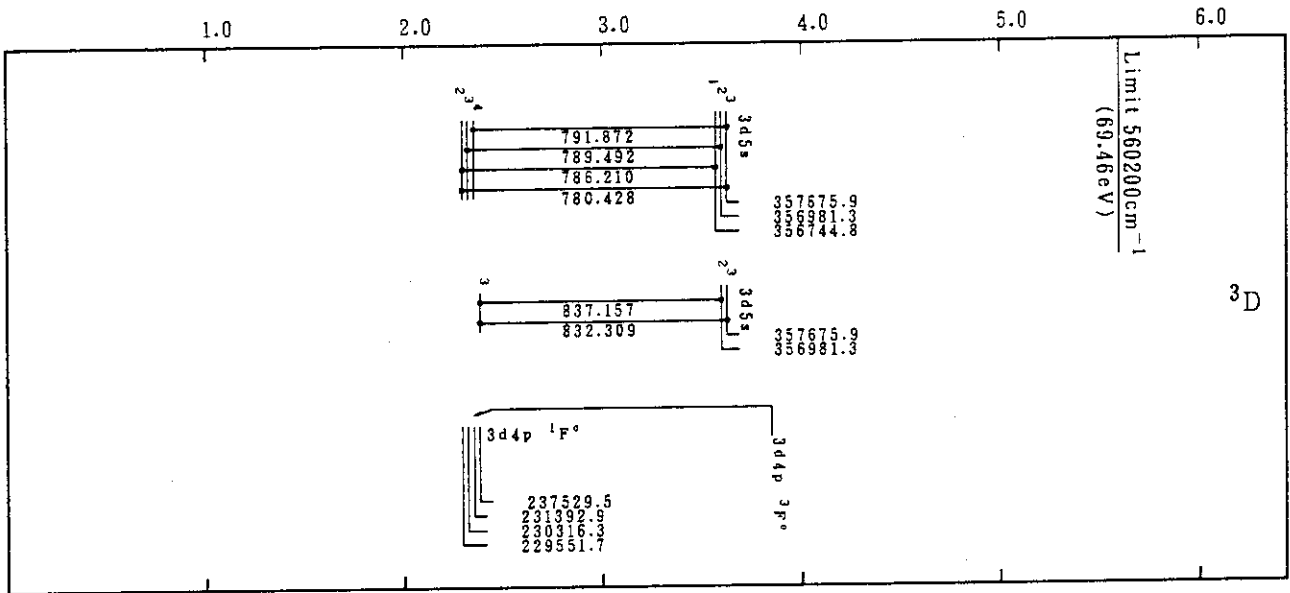
Cr V (Ca-Sequence)
