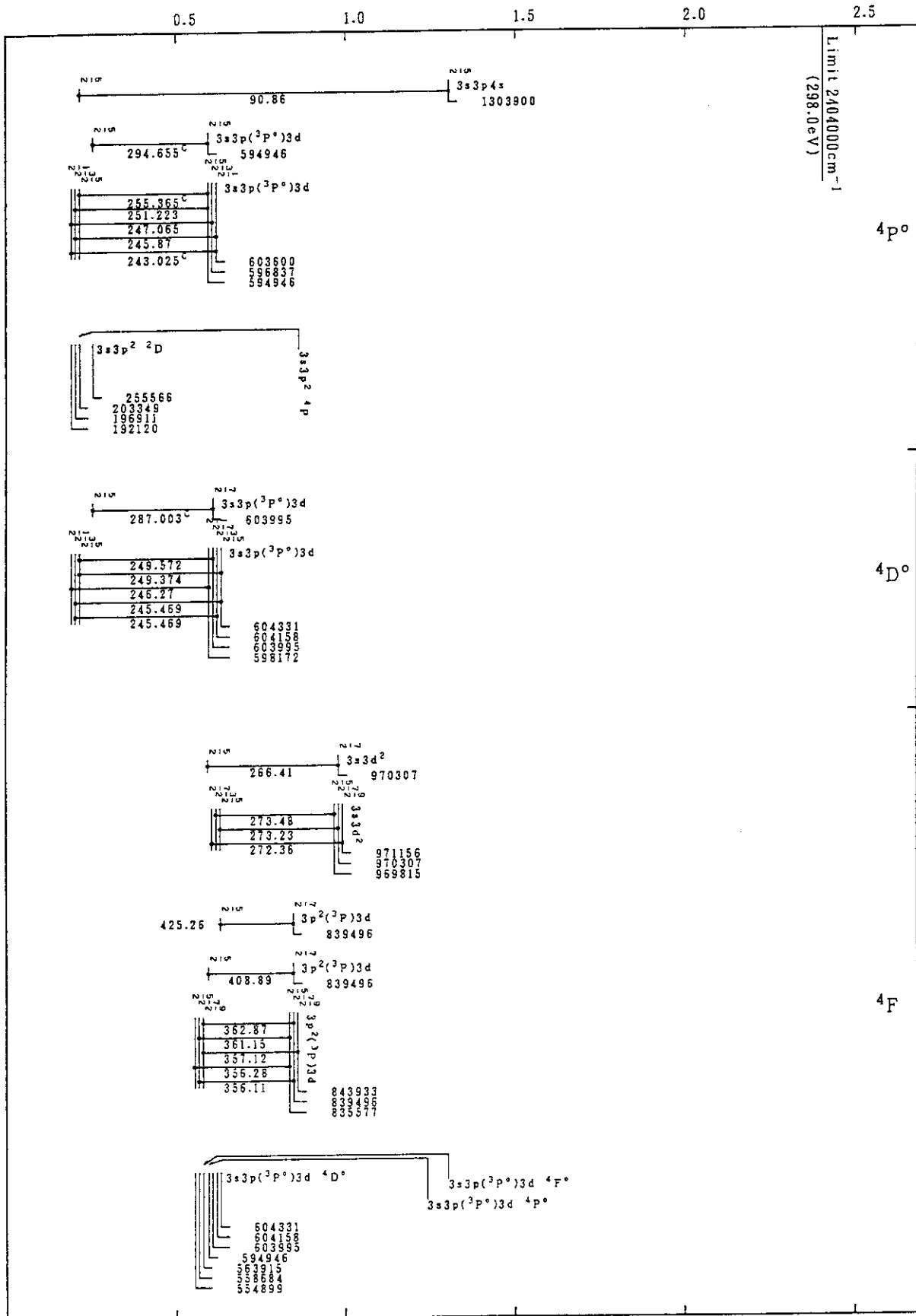
Cr XII(Al-Sequence)
