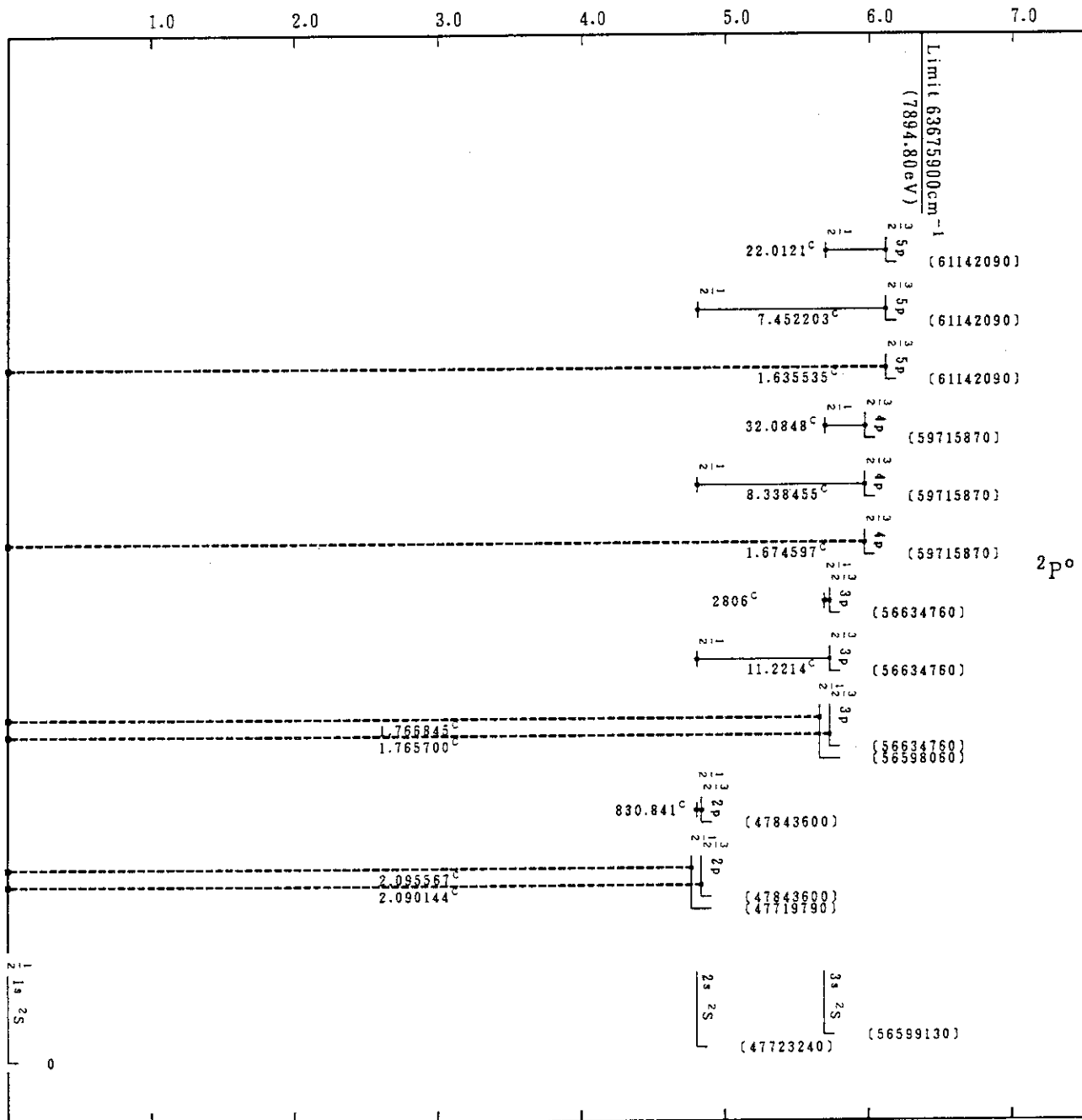
Cr XXIV(H-Sequence)
