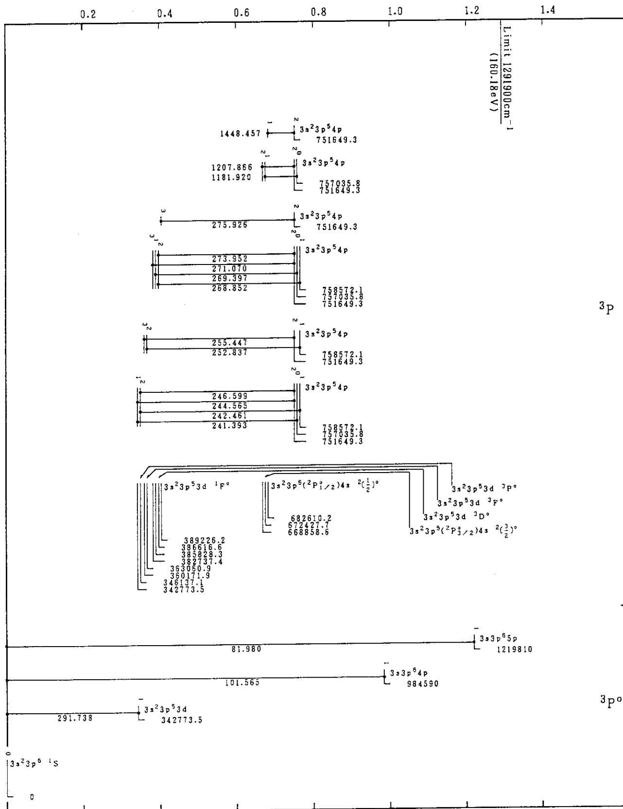
Cr VII (Ar-Sequence)
