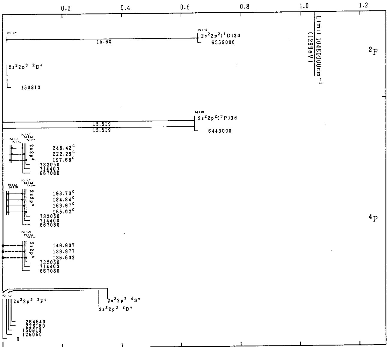
Cr XVIII(N-Sequence)
