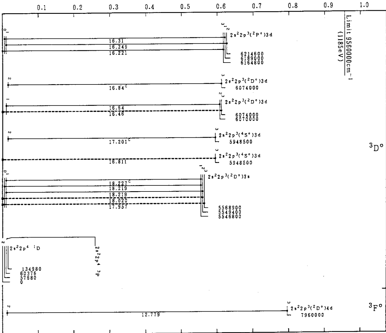
Cr XVII(O-Sequence)
