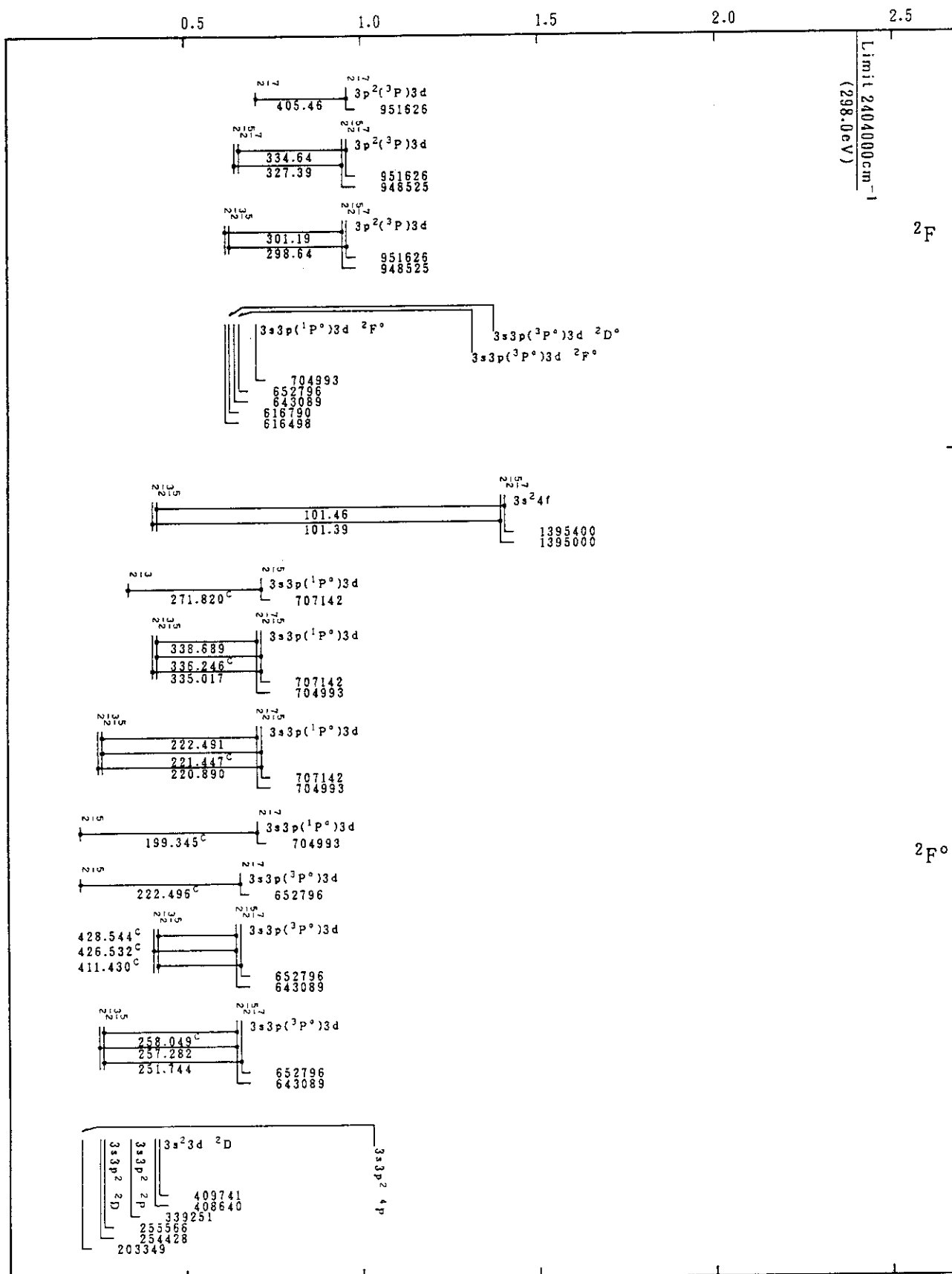
Cr XII(Al-Sequence)
