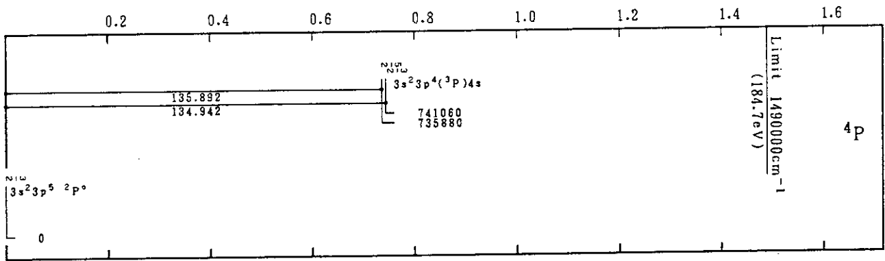
Cr VIII(Cl-Sequence)
