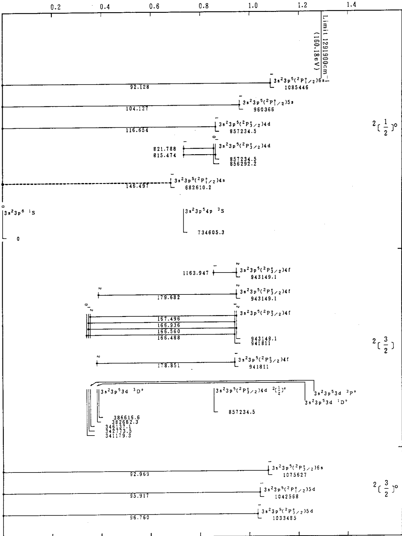
Cr VII(Ar-Sequence)
