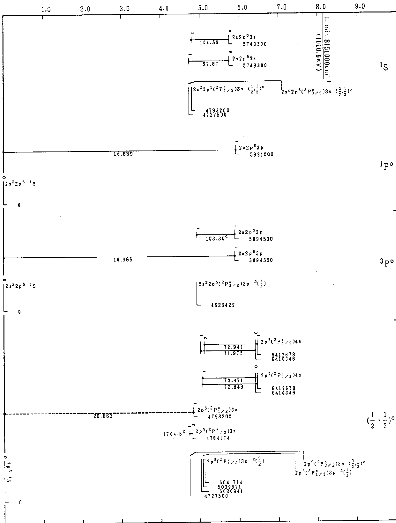
Cr XV (Ne-Sequence)
