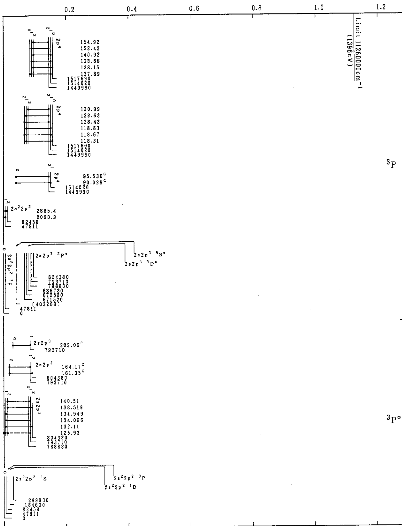
Cr XIX(C-Sequence)
