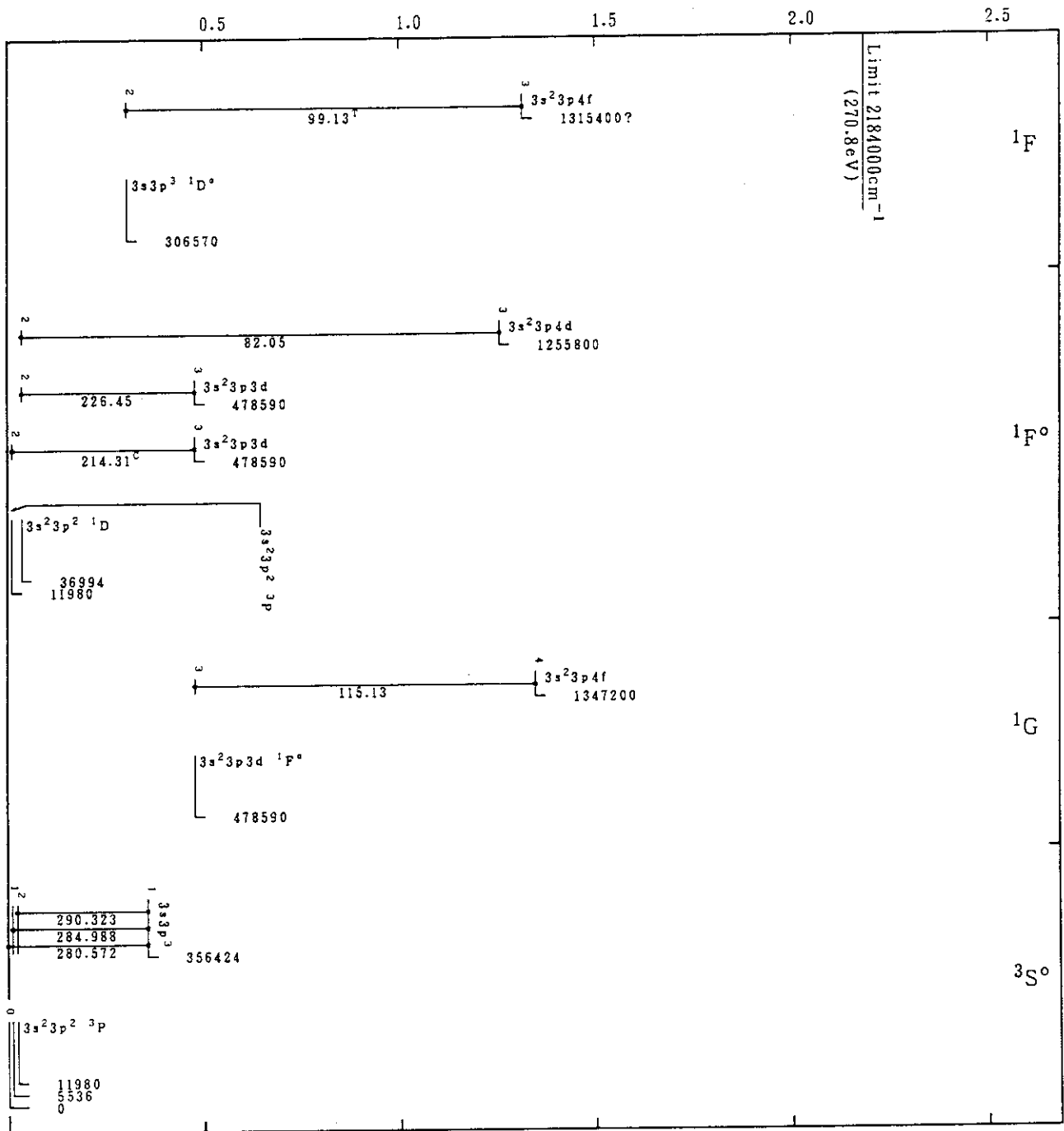
Cr XI(Si-Sequence)
