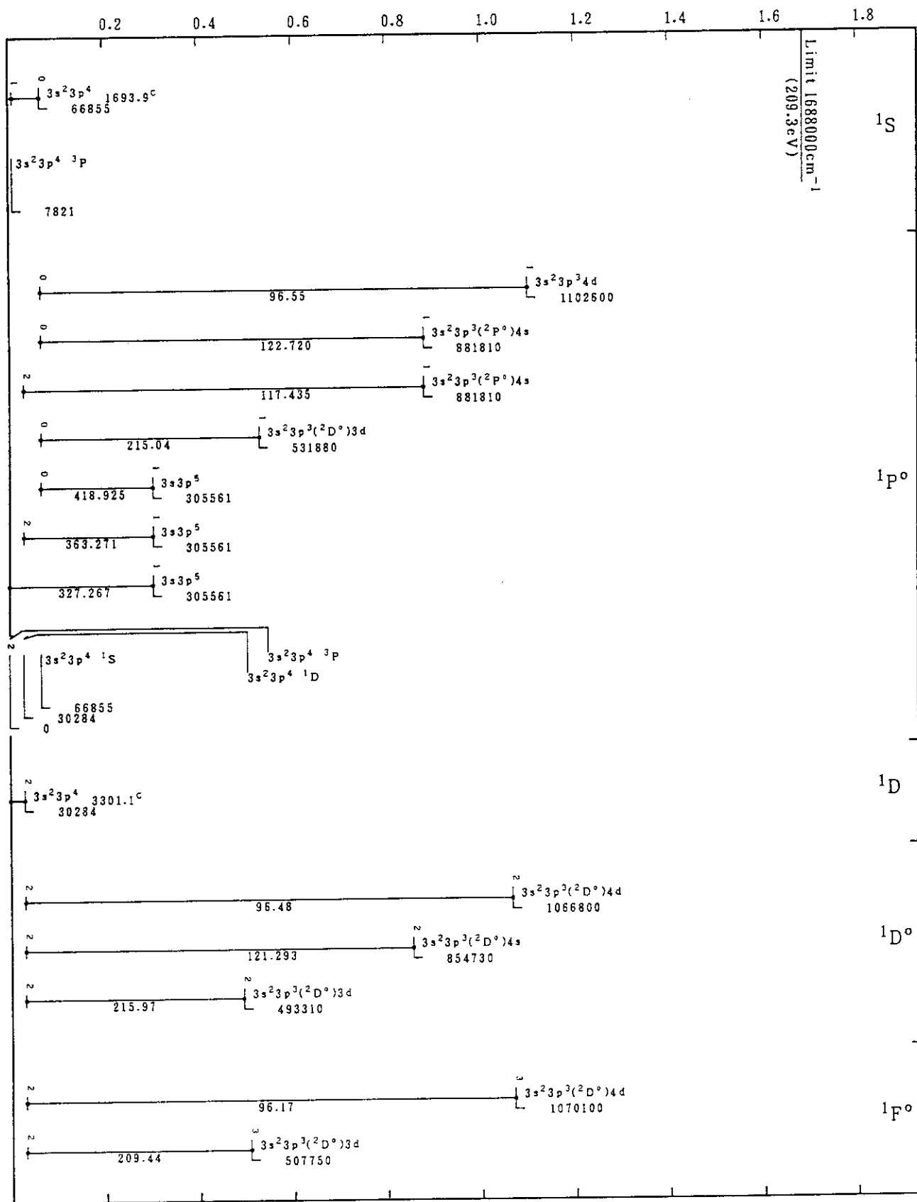
Cr IX(S-Sequence)
