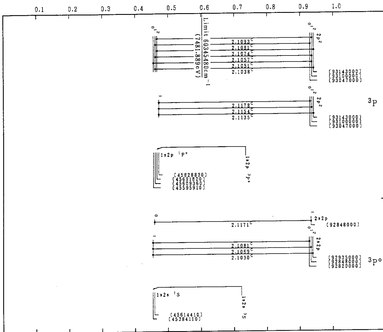
Cr XXIII(He-Sequence)
