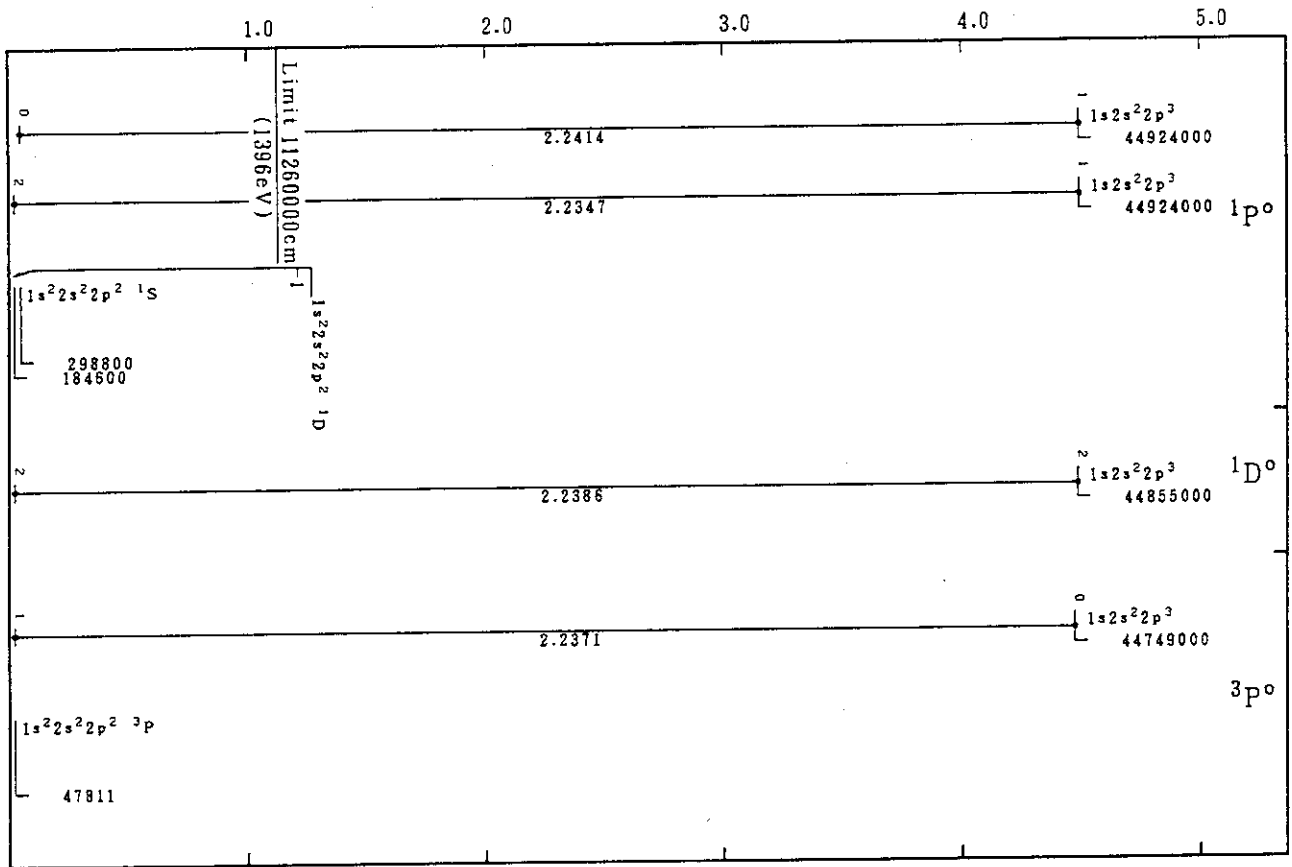
Cr XIX(C-Sequence)
