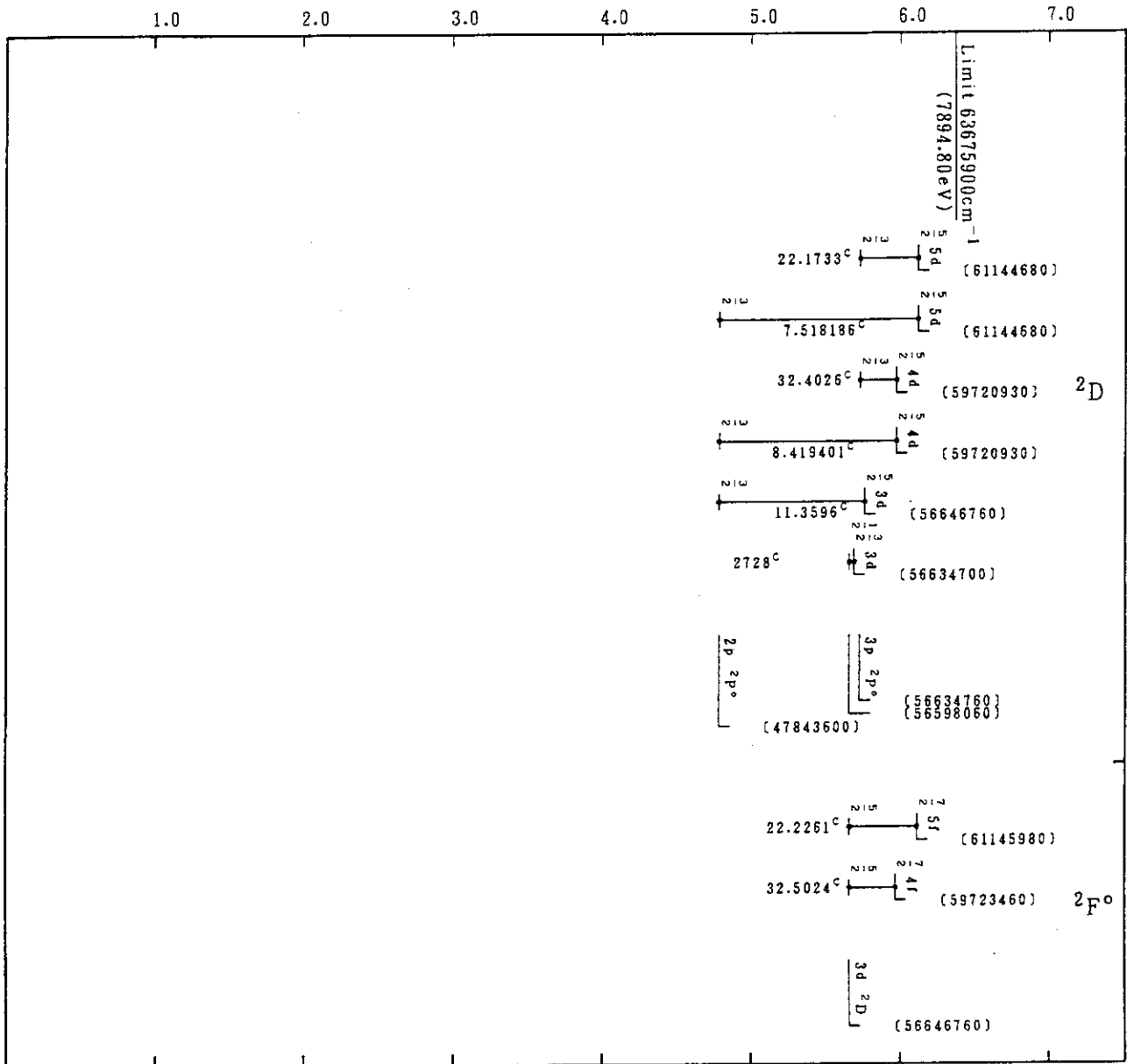
Cr XXIV(H-Sequence)
