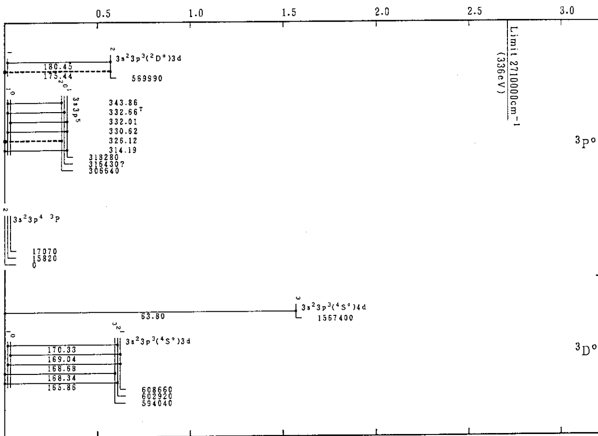
Co XII (S-Sequence)
