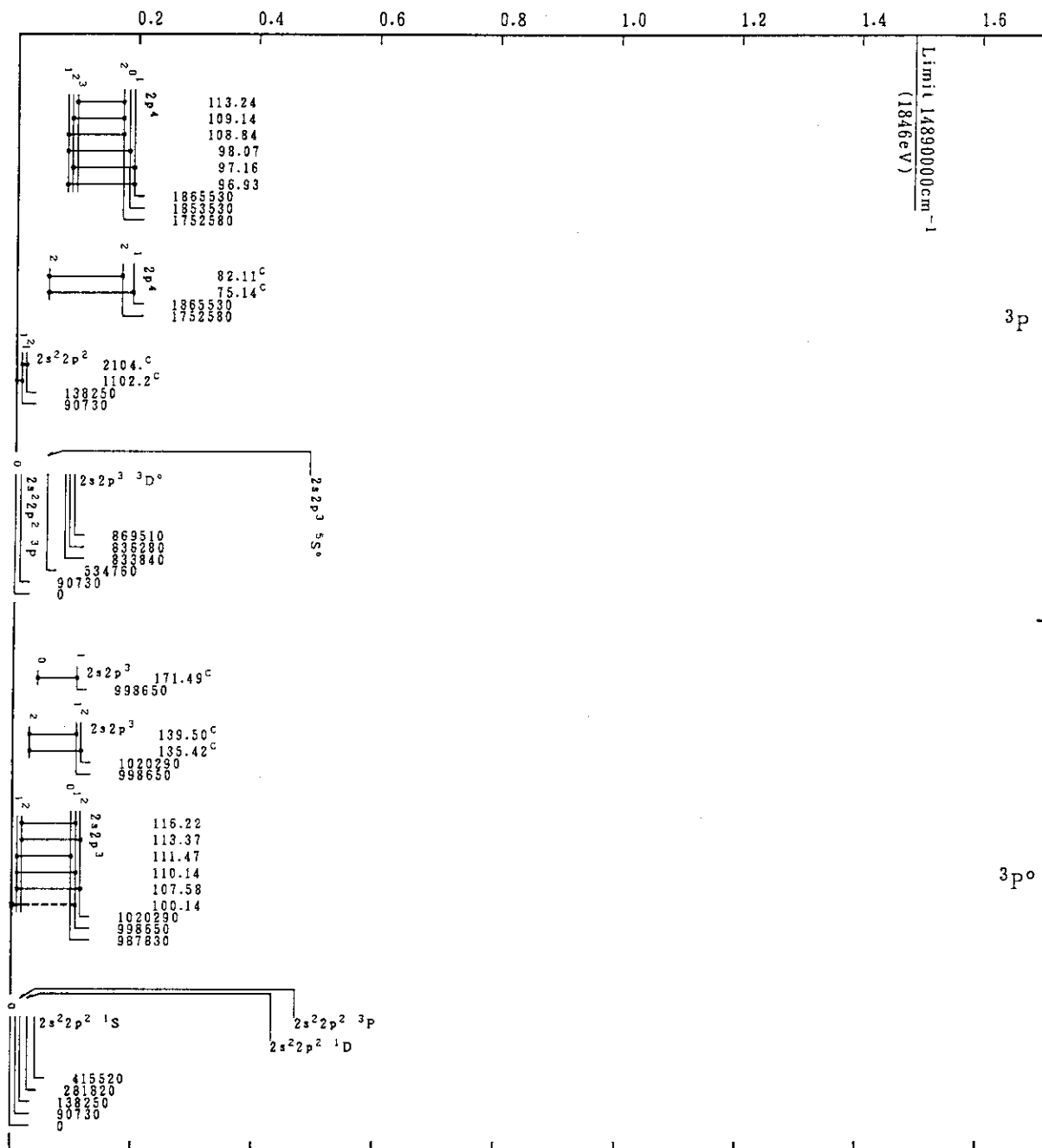
Co XXII (C-Sequence)
