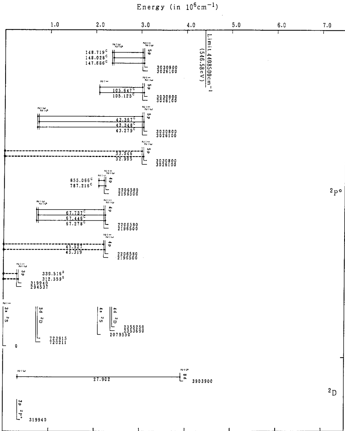
Co XVII (Na-Sequence)
