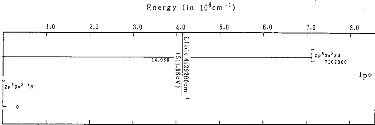
Co XVI (Mg-Sequence)
