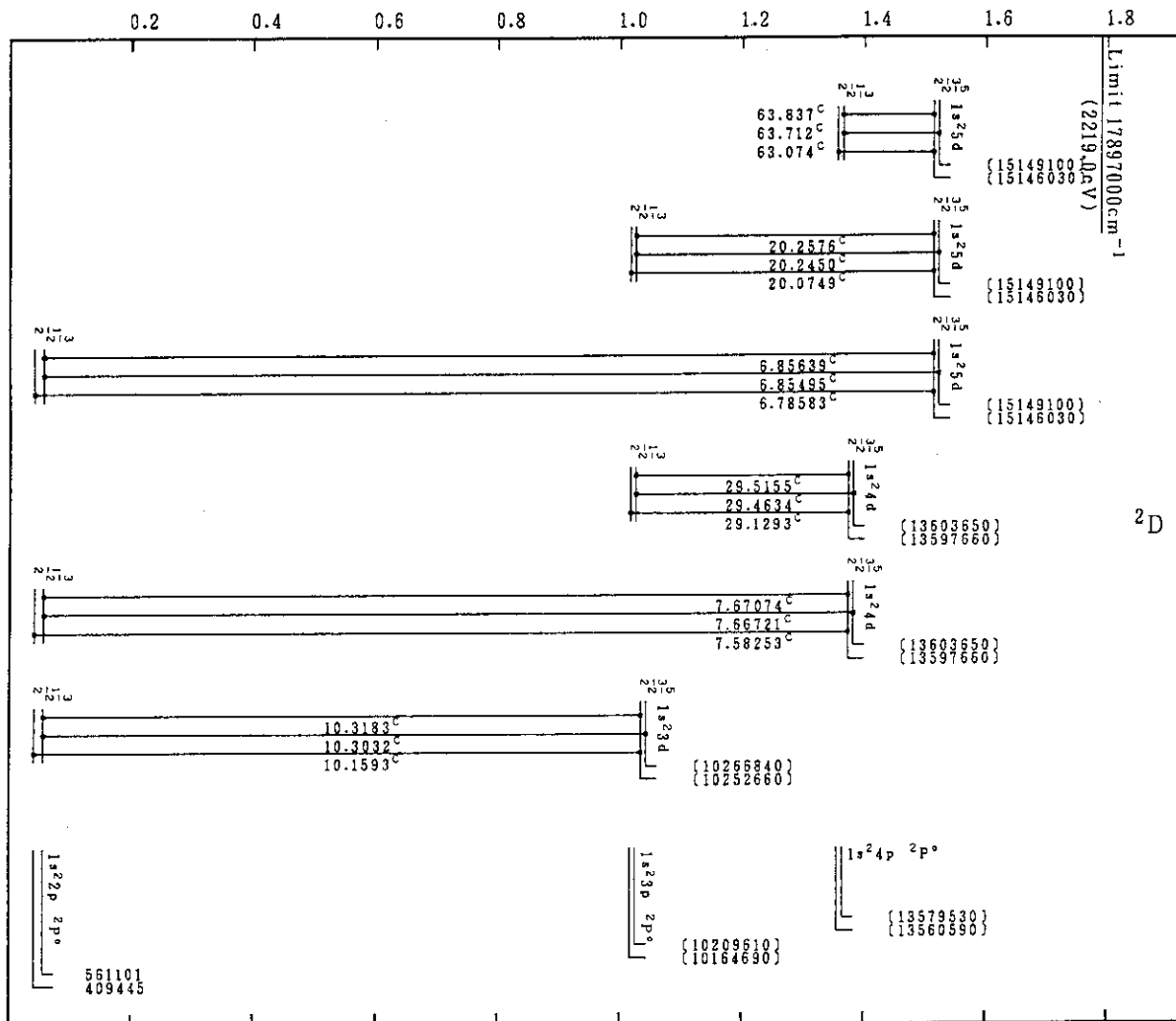
Co XXV (Li-Sequence)
