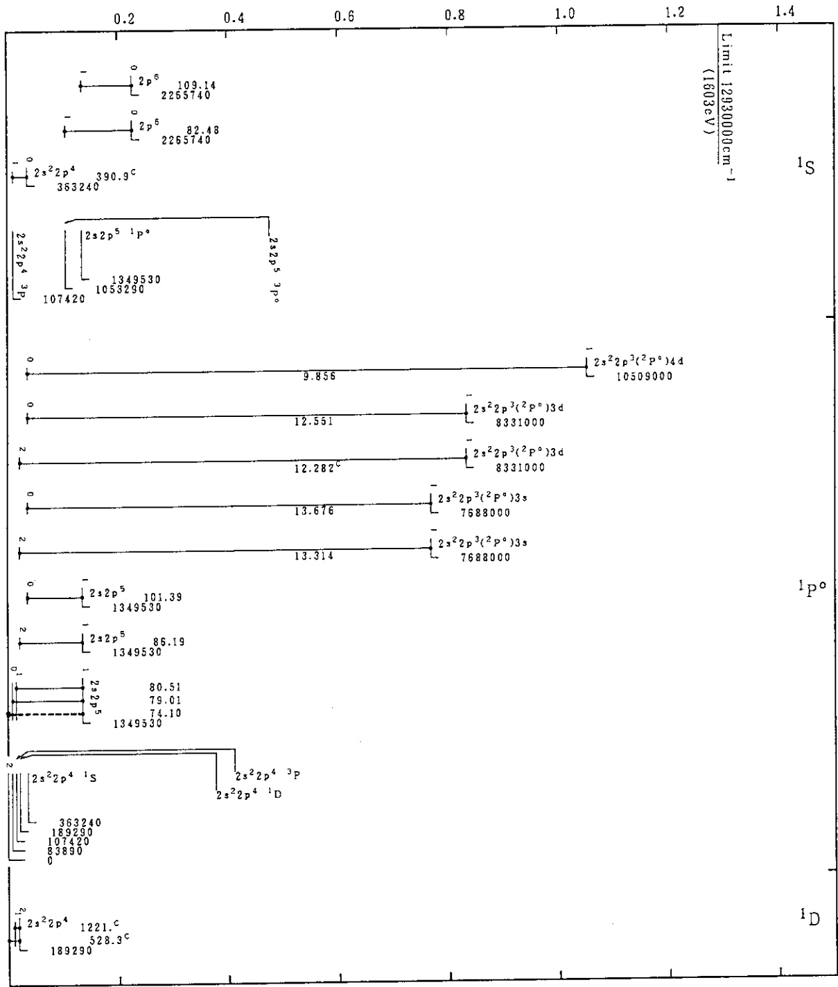
Co XX (O-Sequence)
