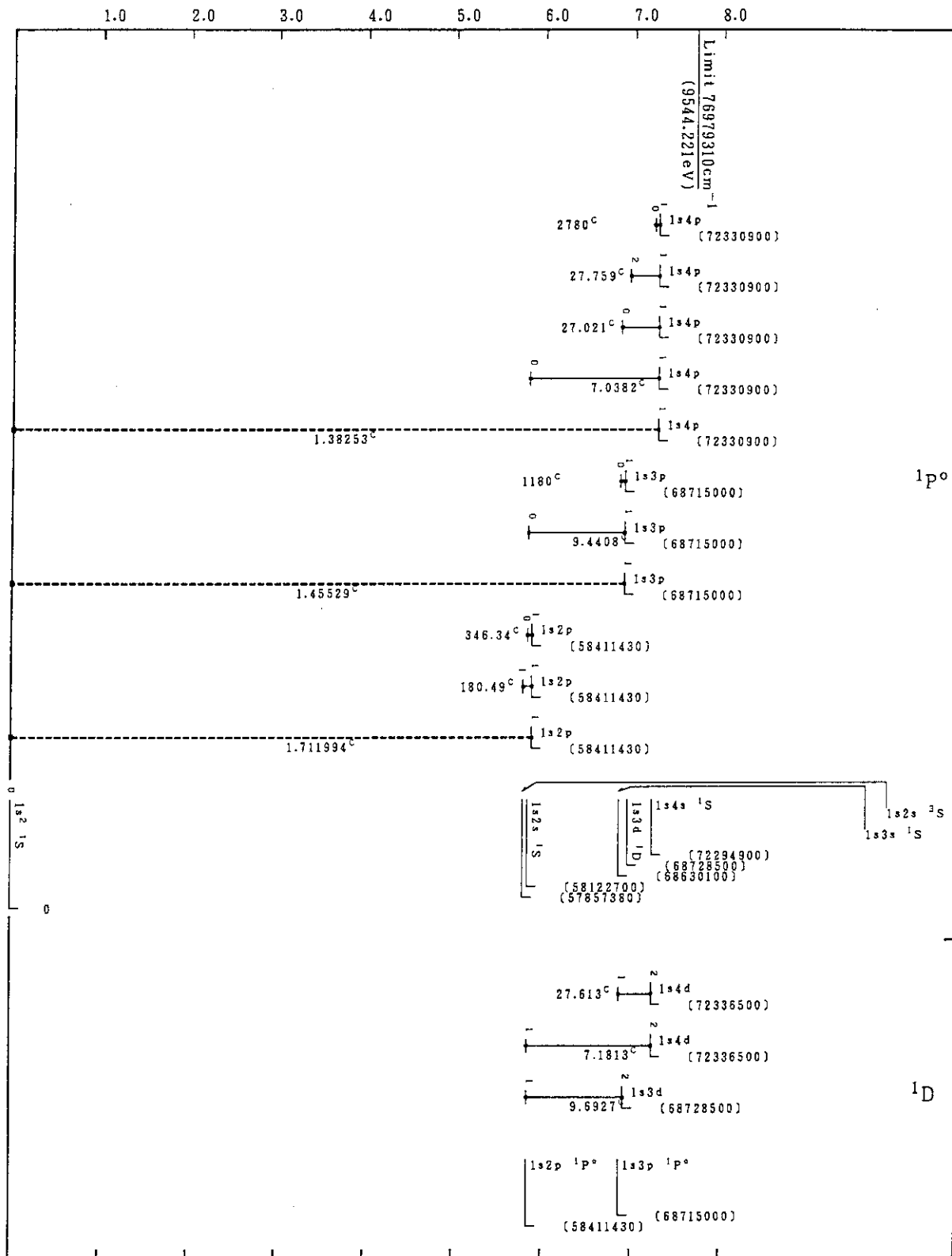
Co XXVI (He-Sequence)
