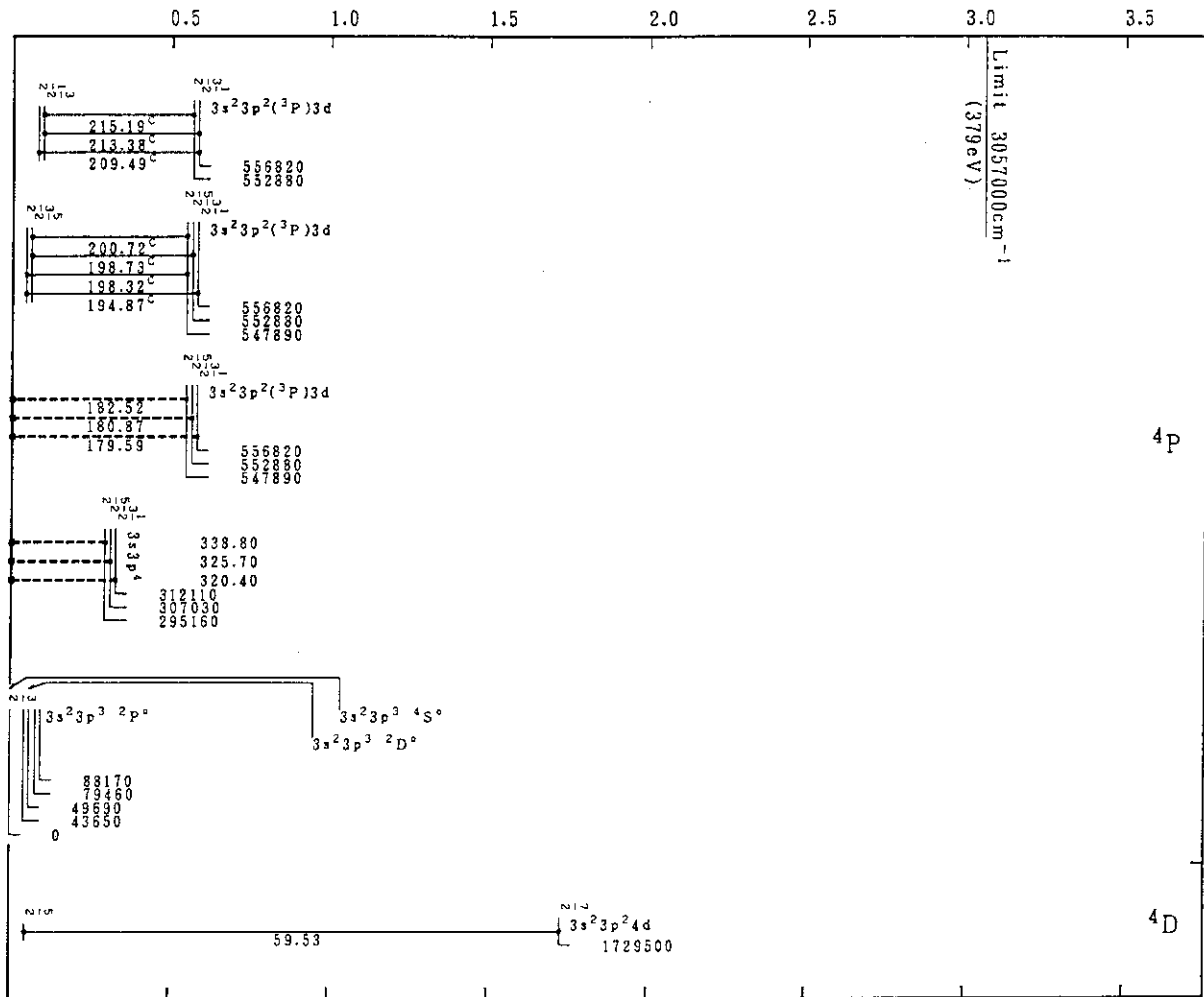
Co XIII (P-Sequence)
