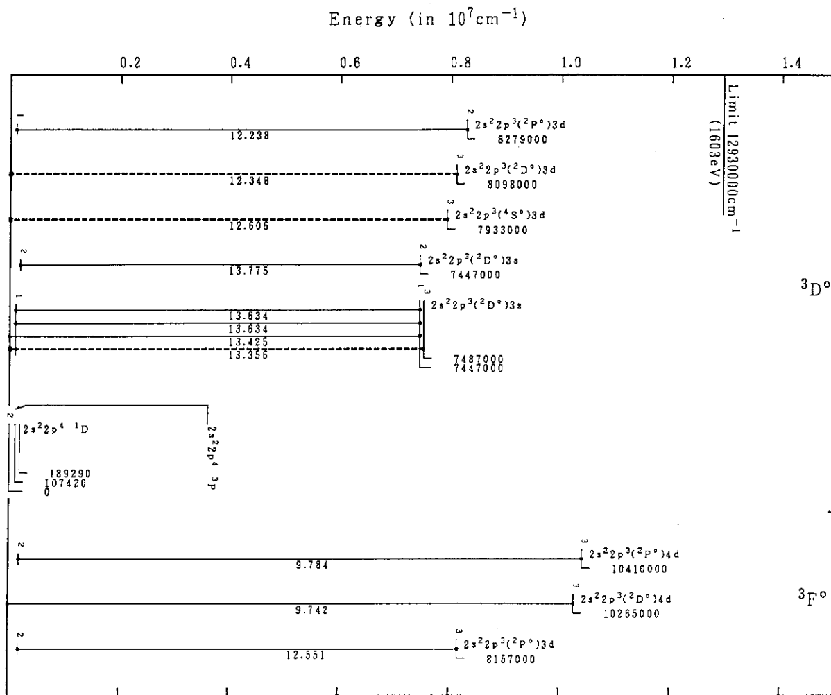
Co XX (O-Sequence)
