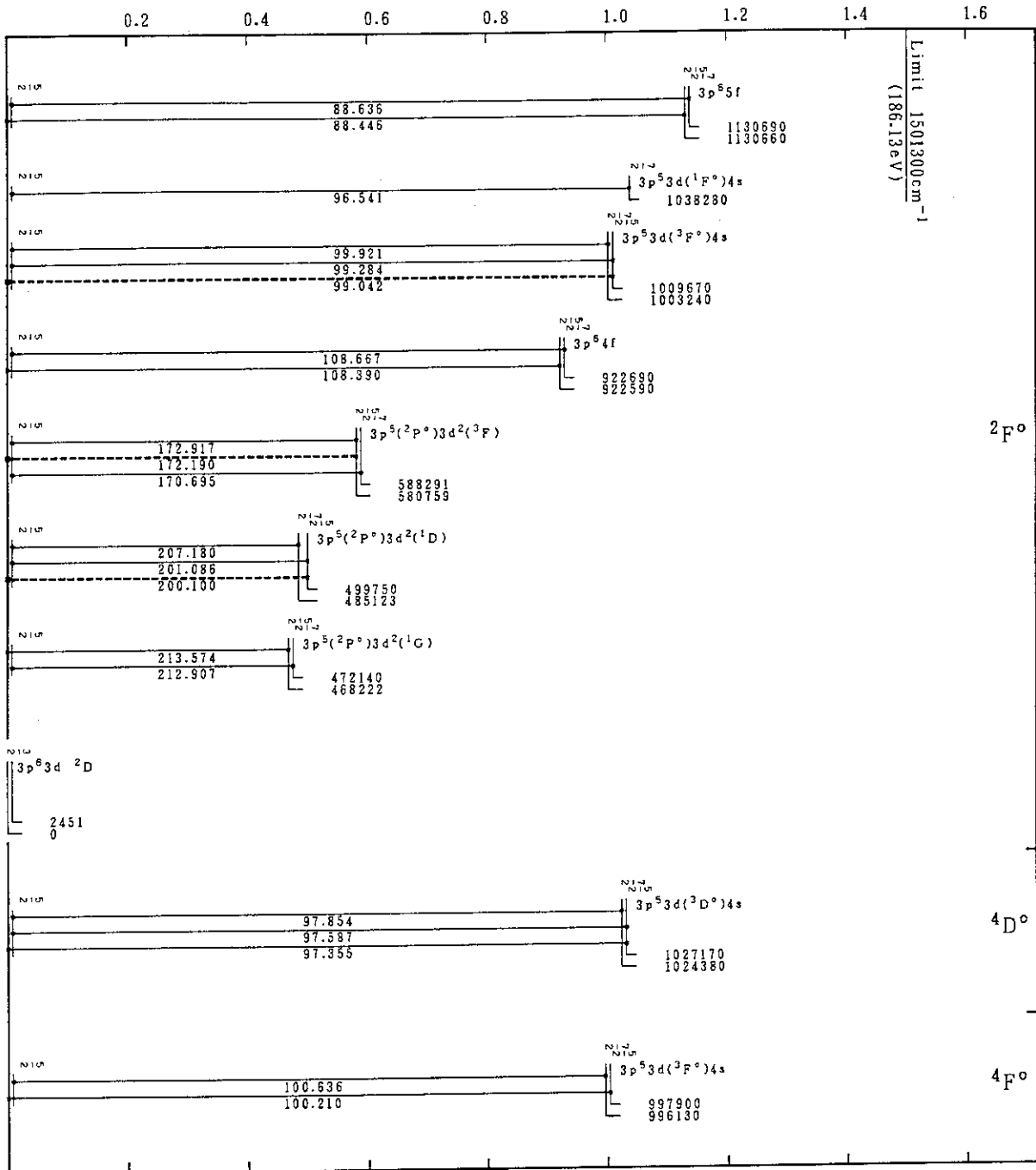
Co IX (K-Sequence)
