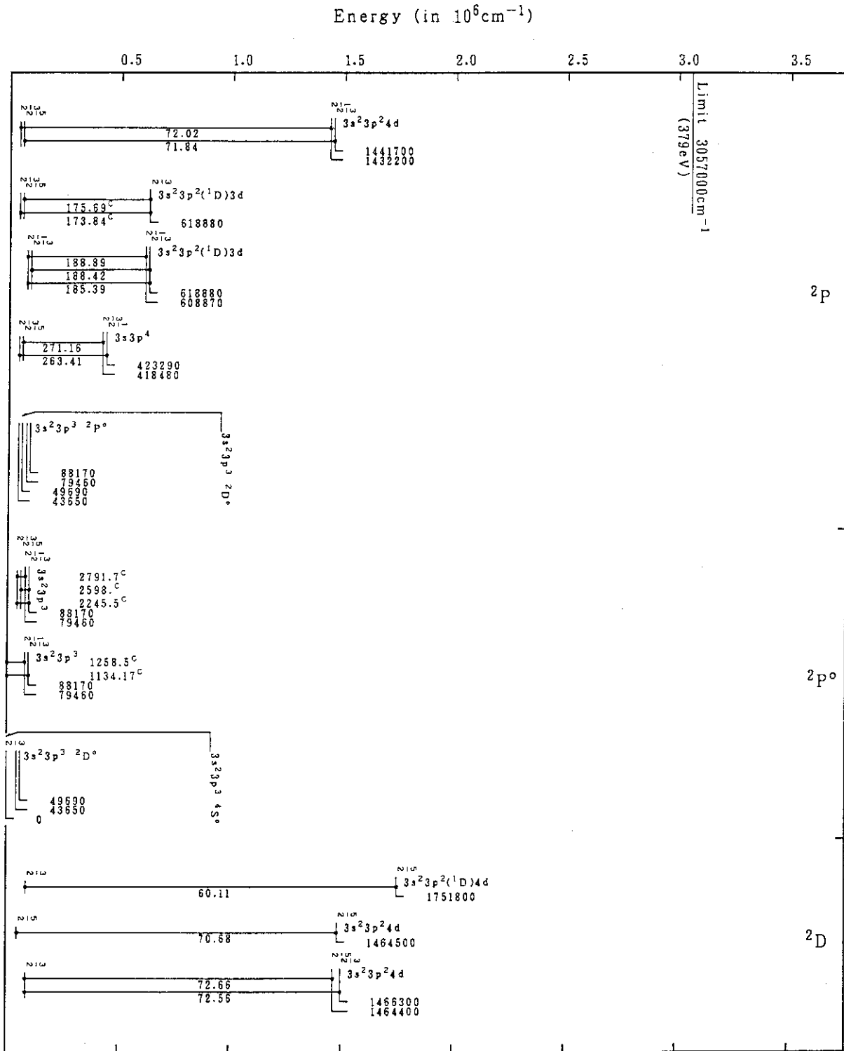
Co XIII (P-Sequence)
