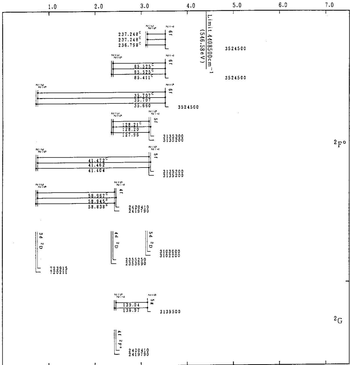
Co XVII (Na-Sequence)
