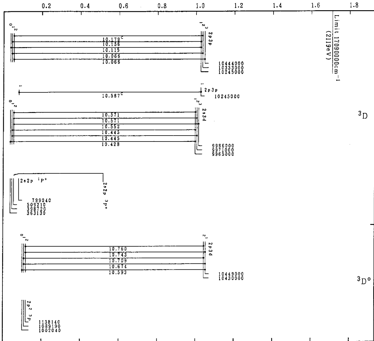
Co XXIV (Be-Sequence)
