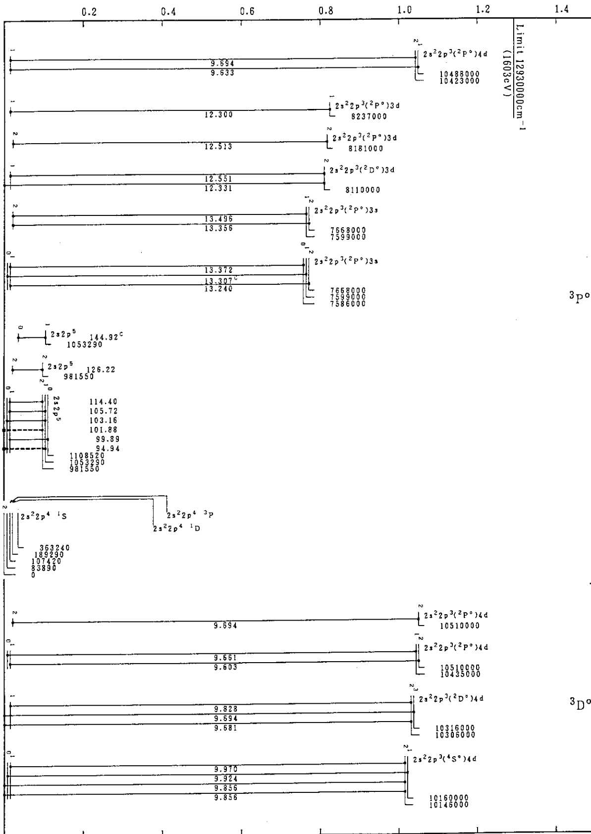
Co XX (O-Sequence)
