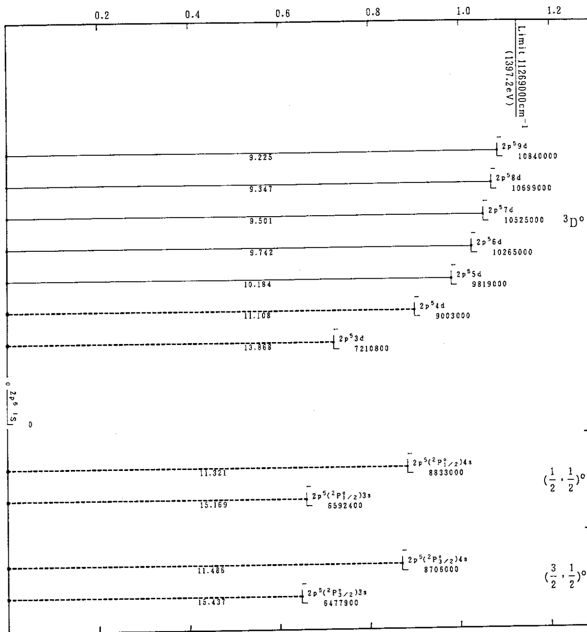
Co XVIII (Ne-Sequence)
