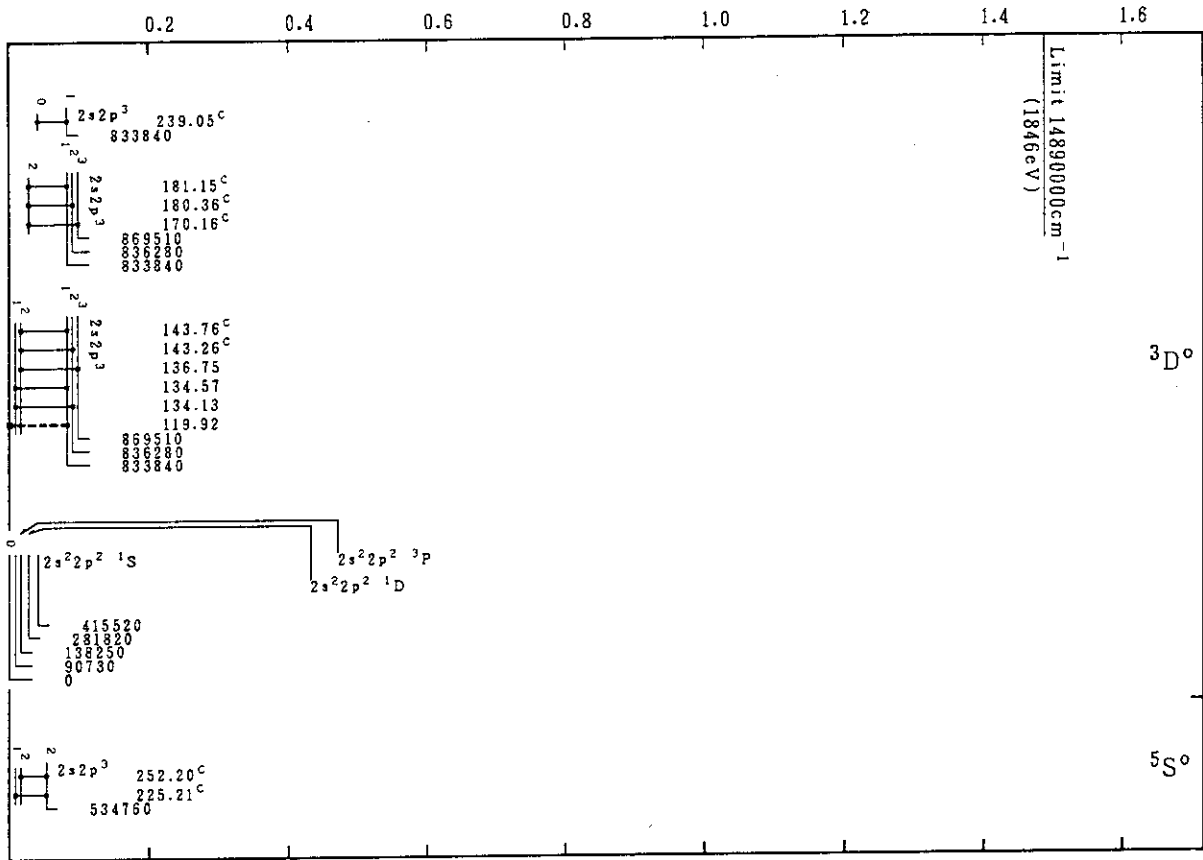
Co XXII (C-Sequence)
