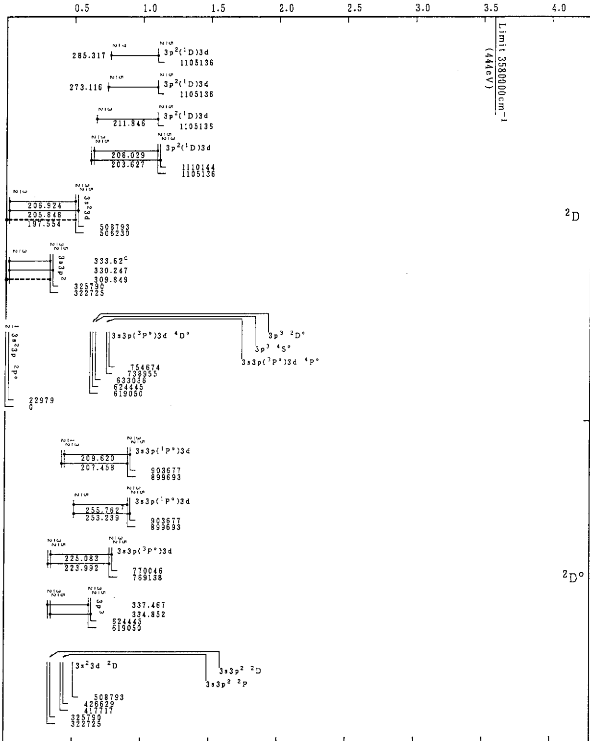
Co XV (Al-Sequence)
