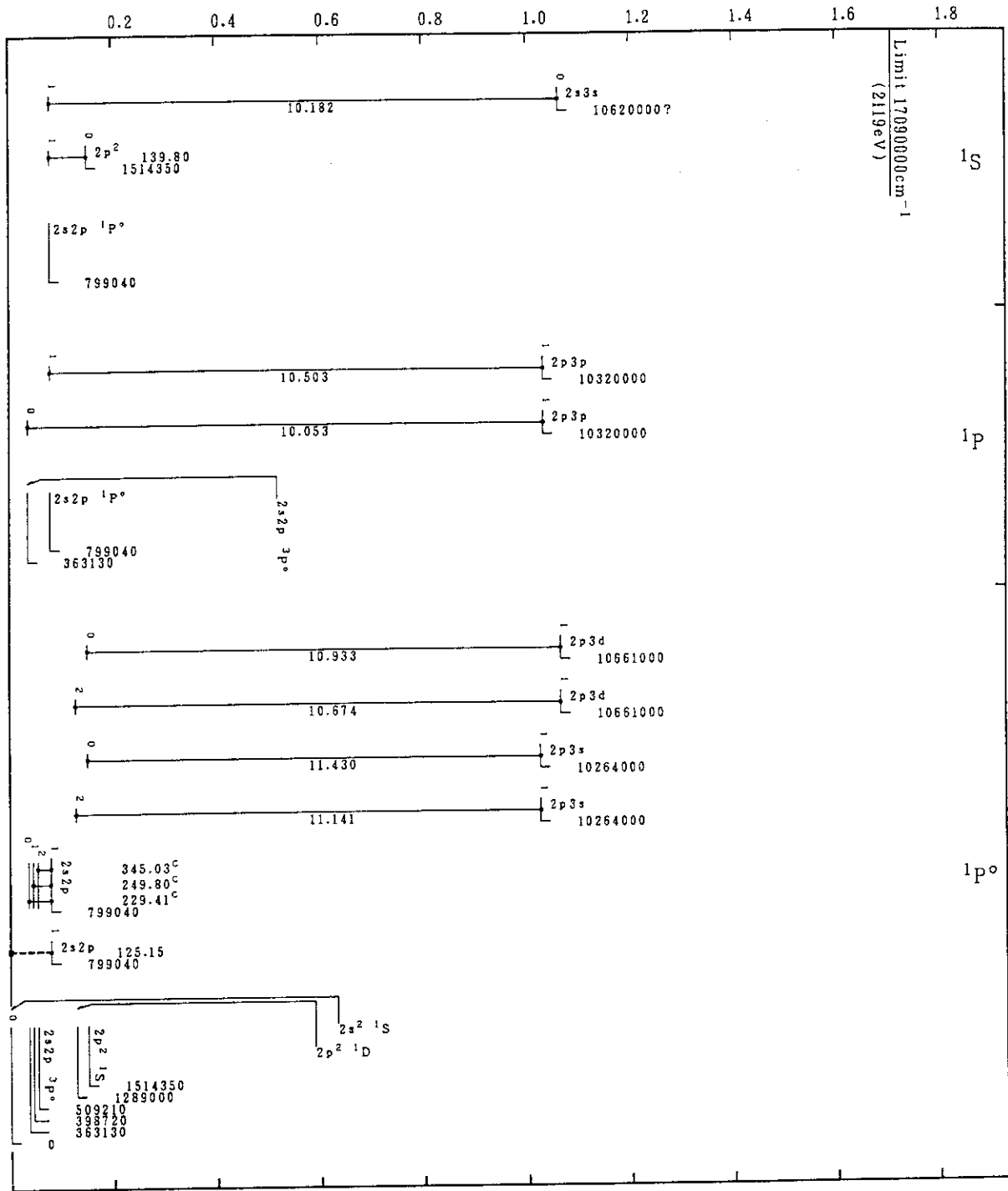
Co XXIV (Be-Sequence)
