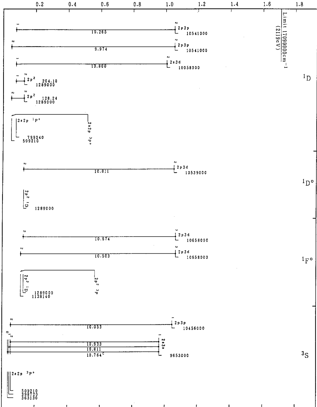
Co XXIV (Be-Sequence)
