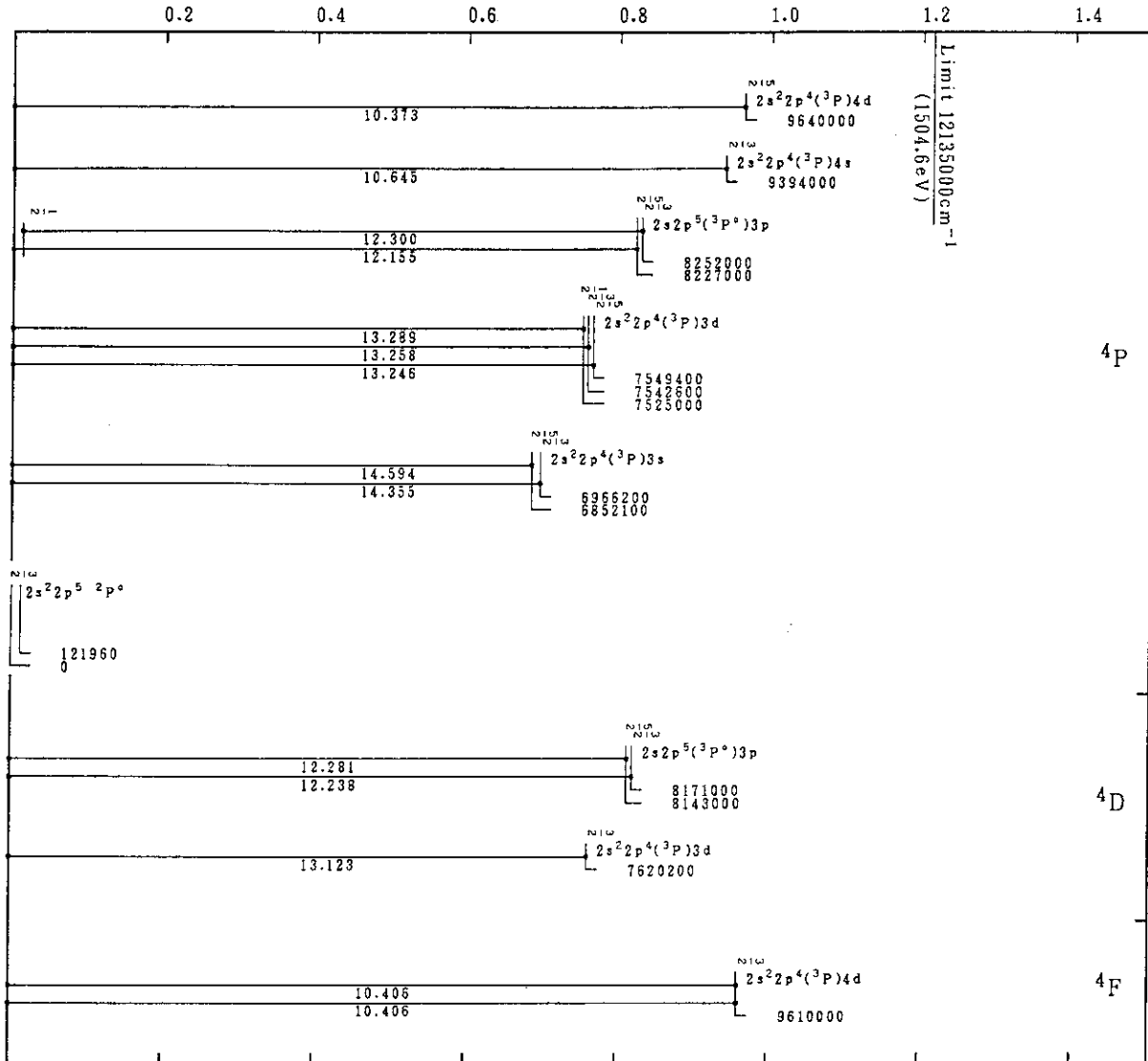
Co XIX (F-Sequence)
