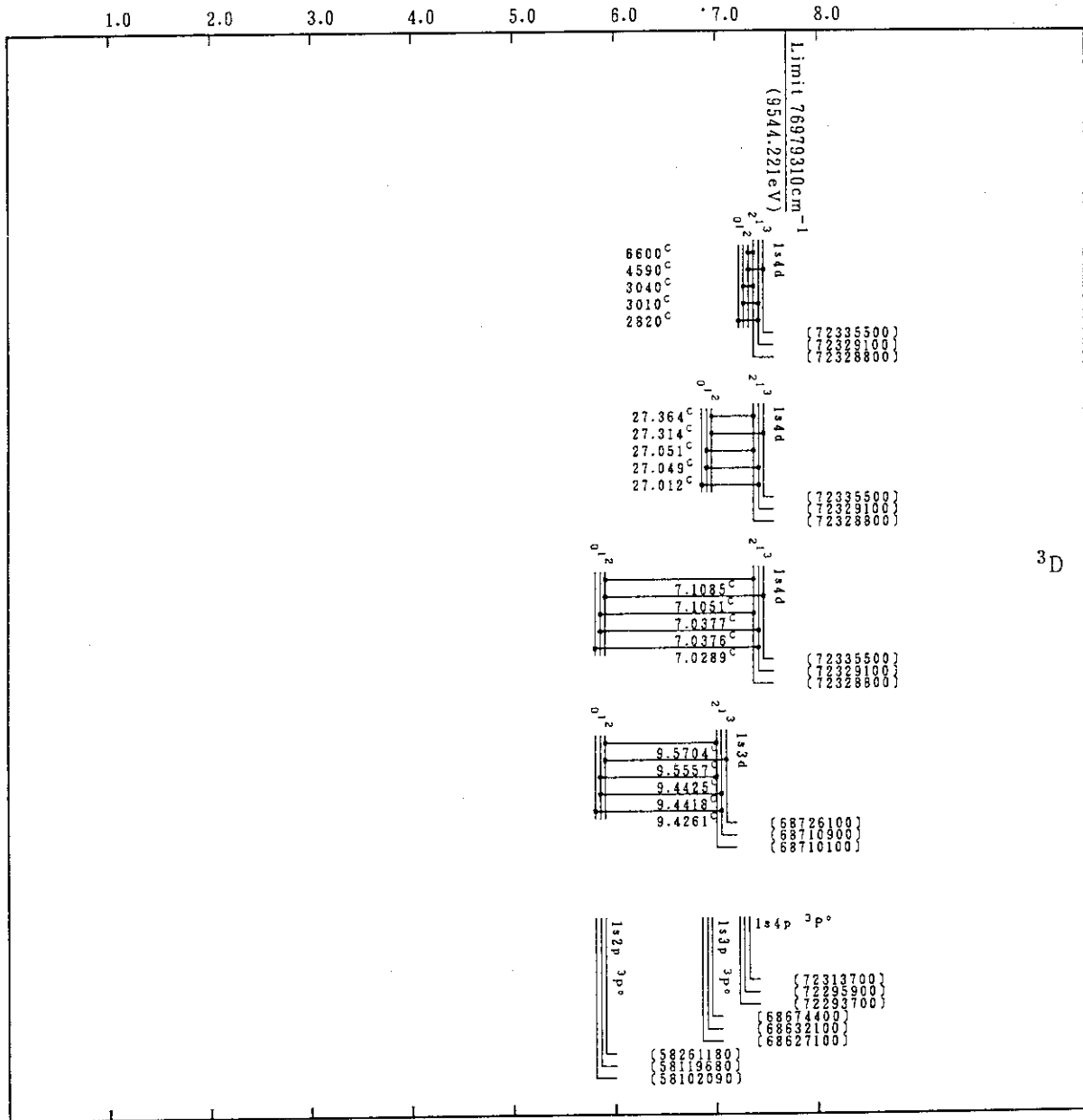
Co XXVI (He-Sequence)
