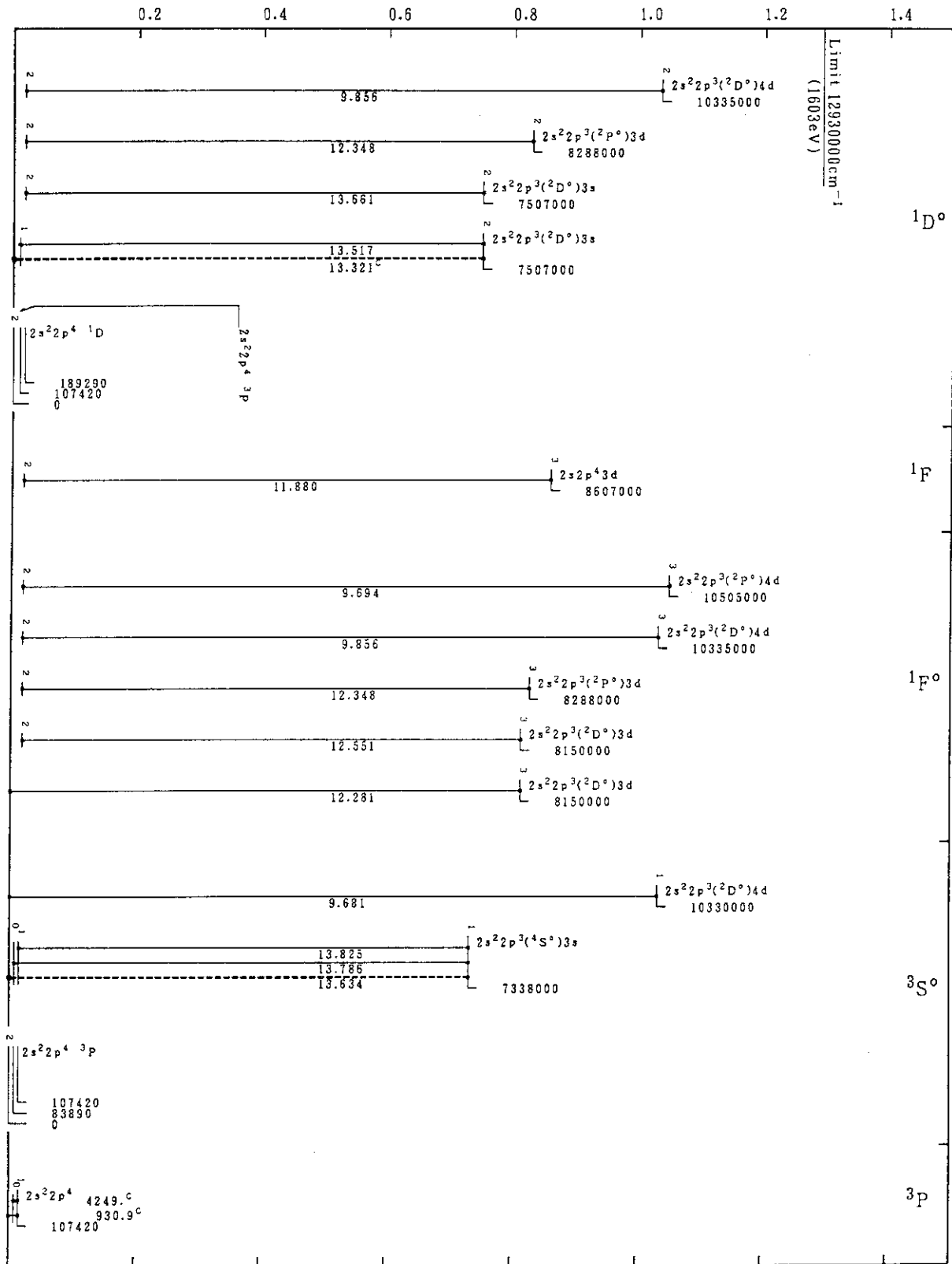
Co XX (O-Sequence)
