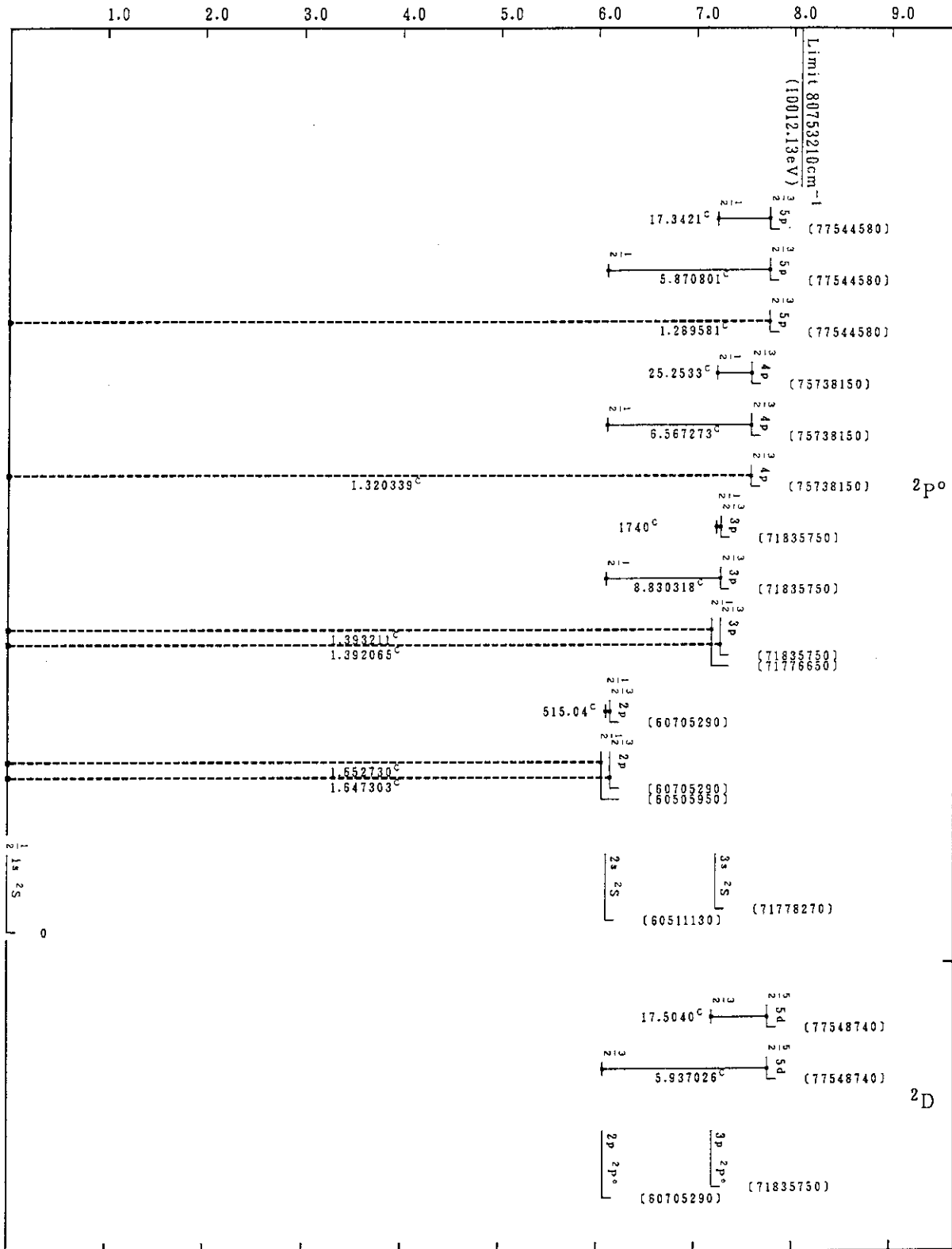
Co XXVII (H-Sequence)
