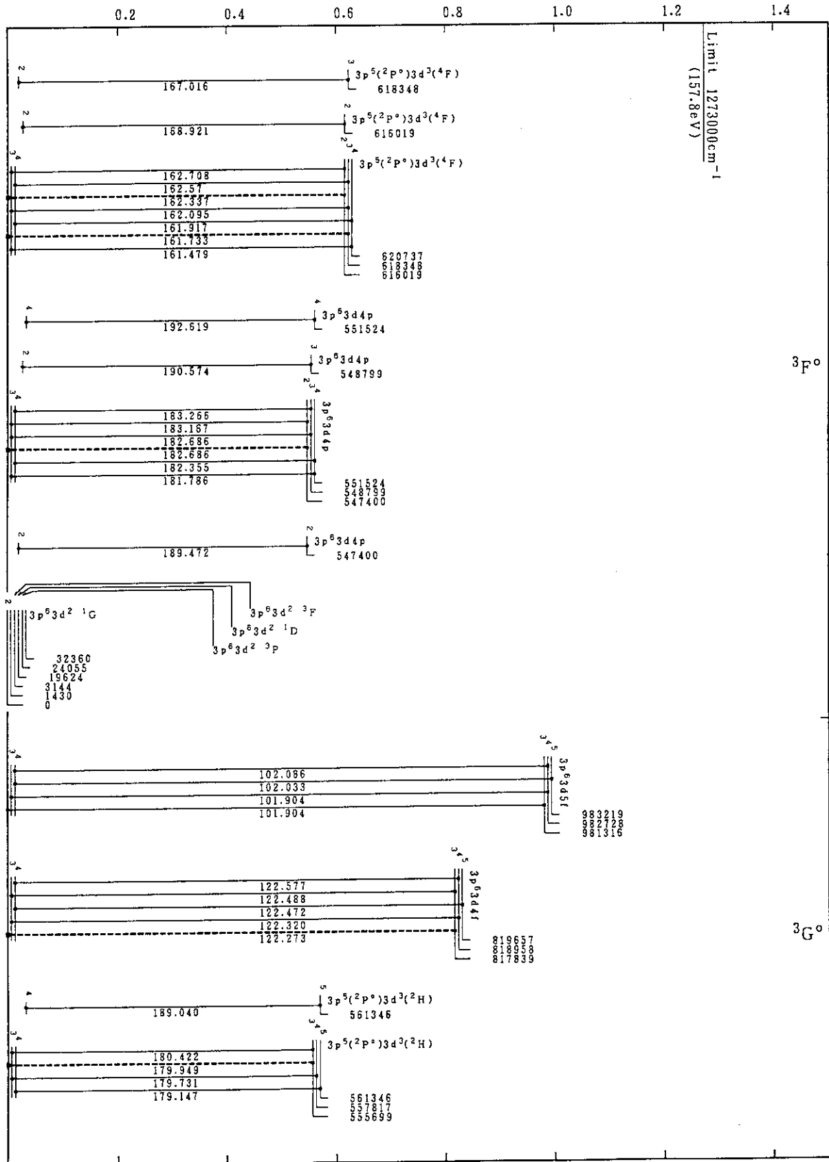
Co VIII (Ca-Sequence)
