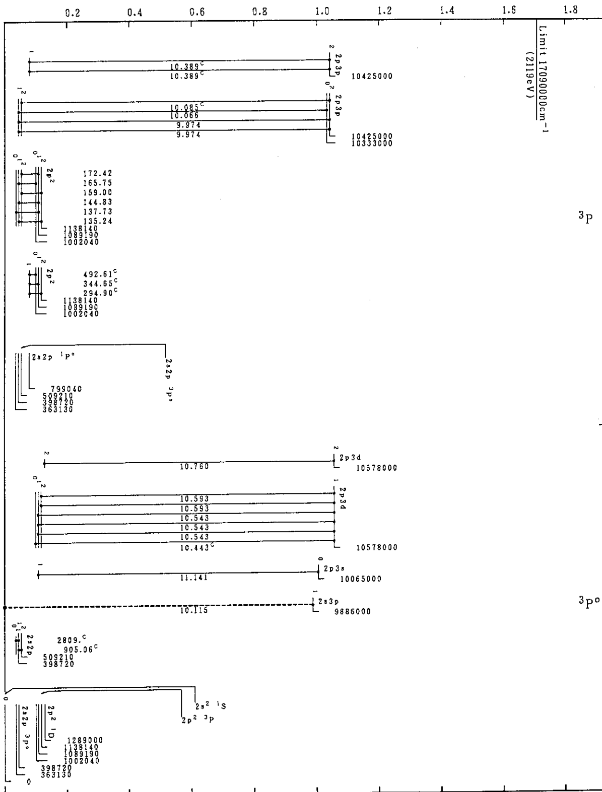
Co XXIV (Be-Sequence)
