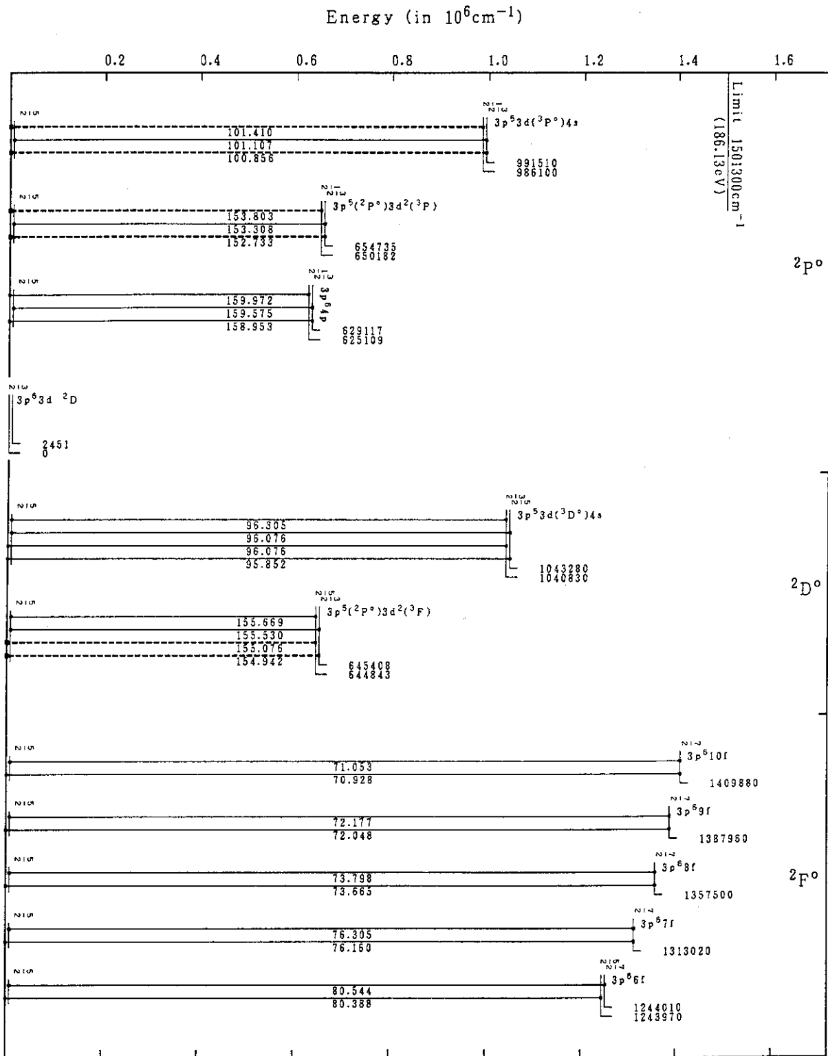
Co IX (K-Sequence)
