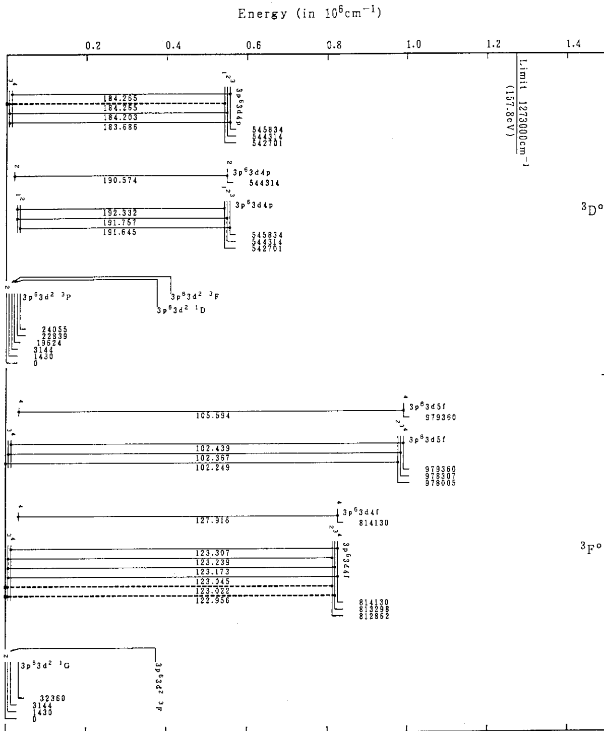
Co VIII (Ca-Sequence)
