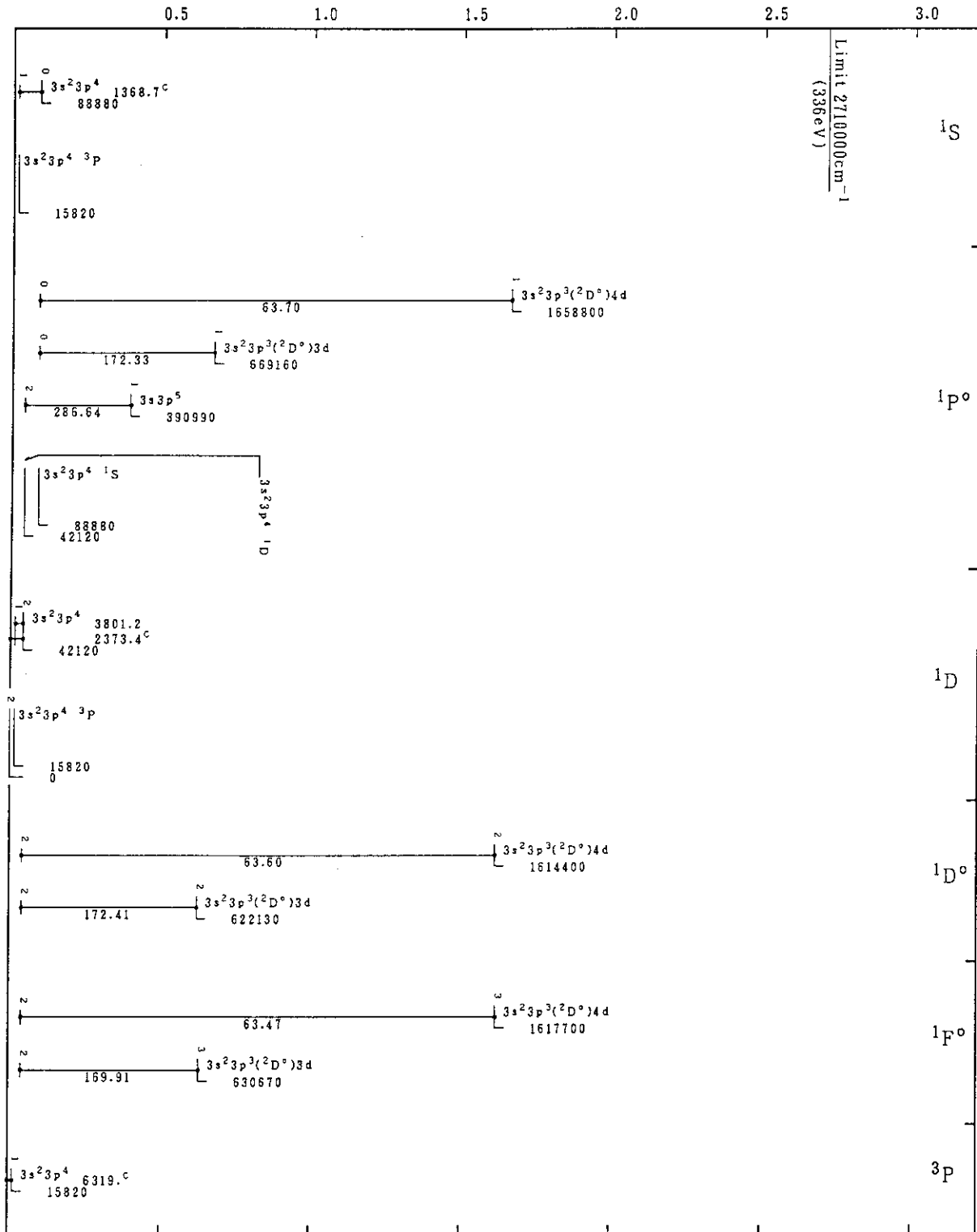
Co XII (S-Sequence)
