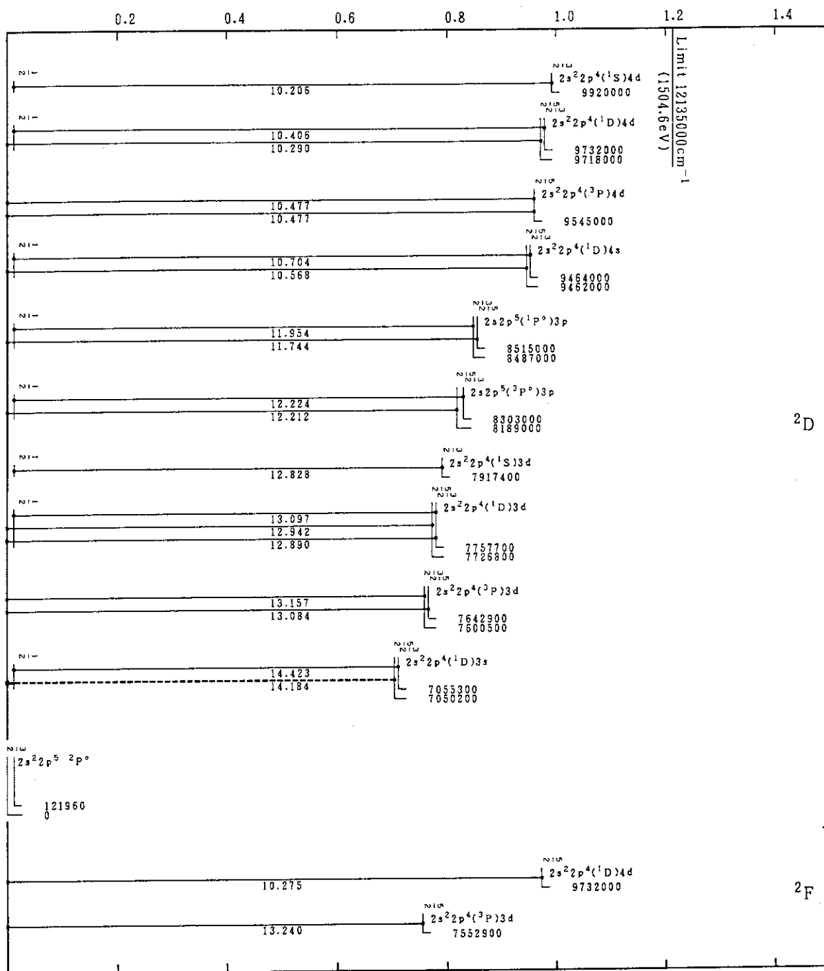
Co XIX (F-Sequence)
