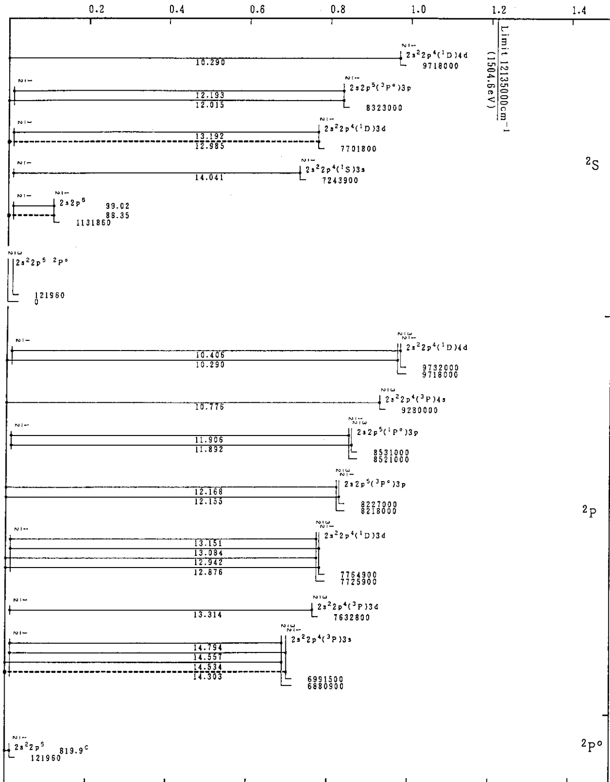
Co XIX (F-Sequence)
