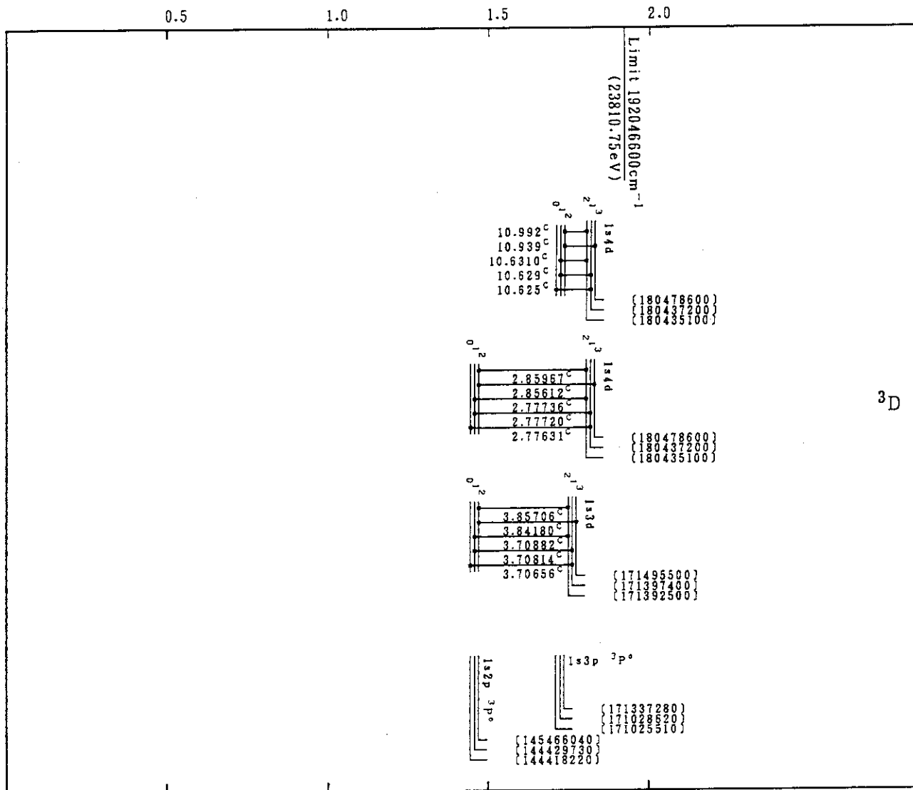
Mo XLI(He-Sequence)
