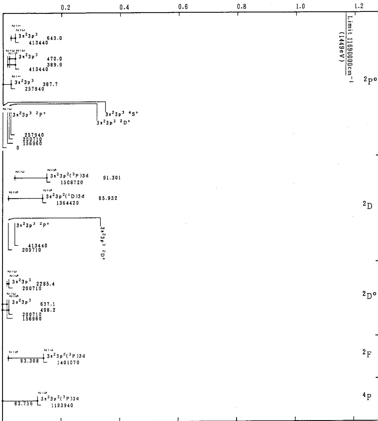
Mo XXVIII(P-Sequence)
