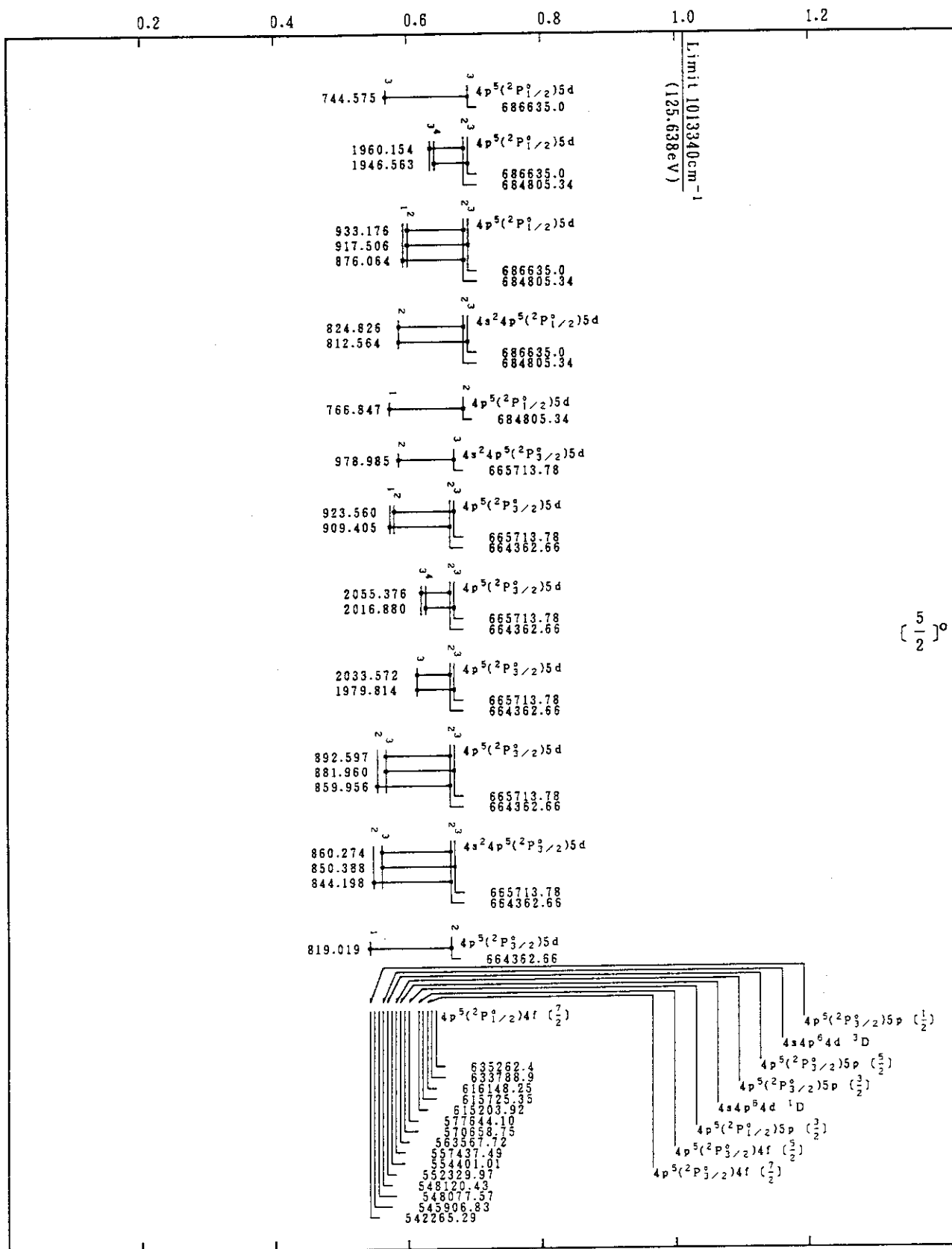
Mo VII(Kr-Sequence)
