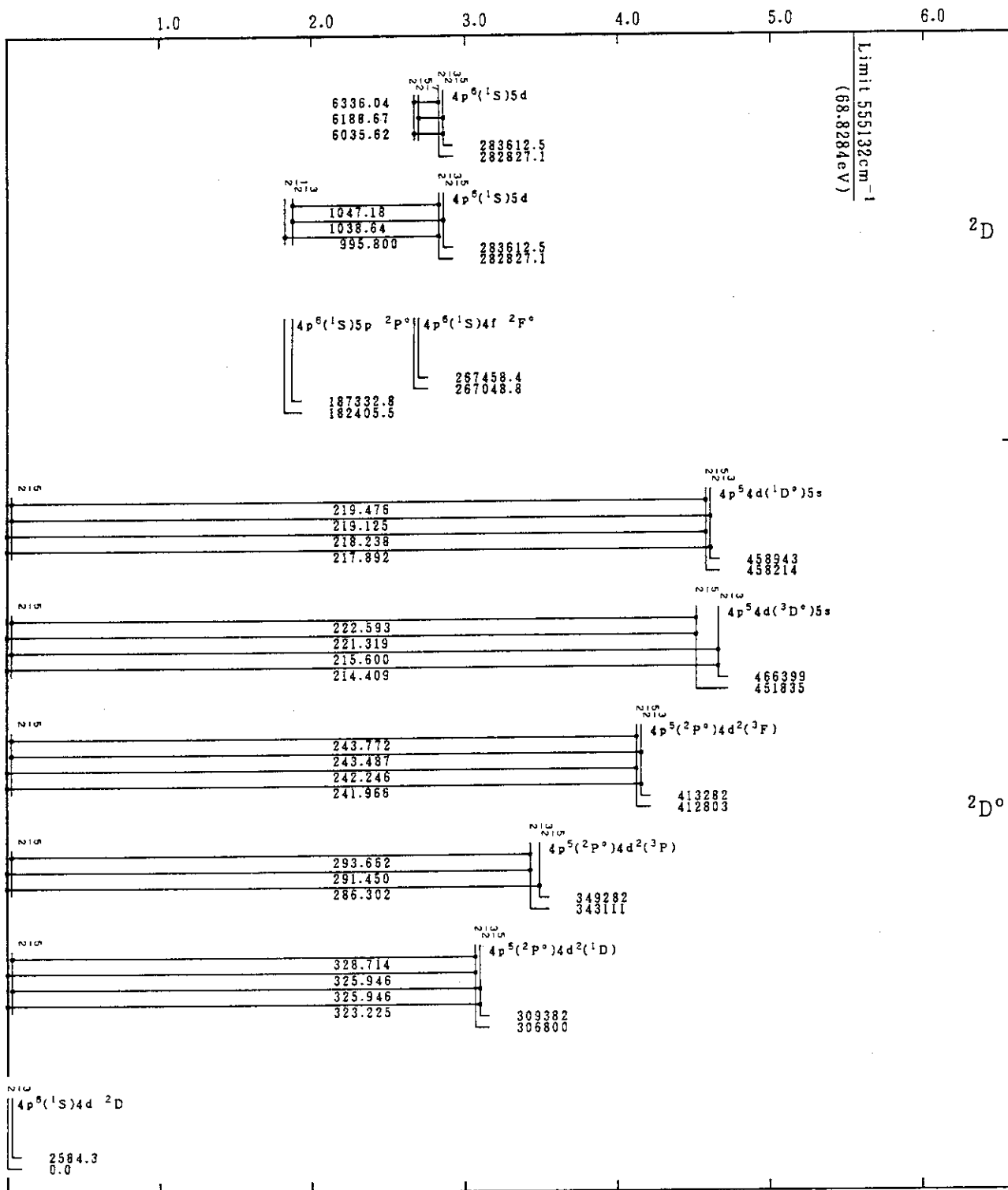
Mo VI(Rb-Sequence)
