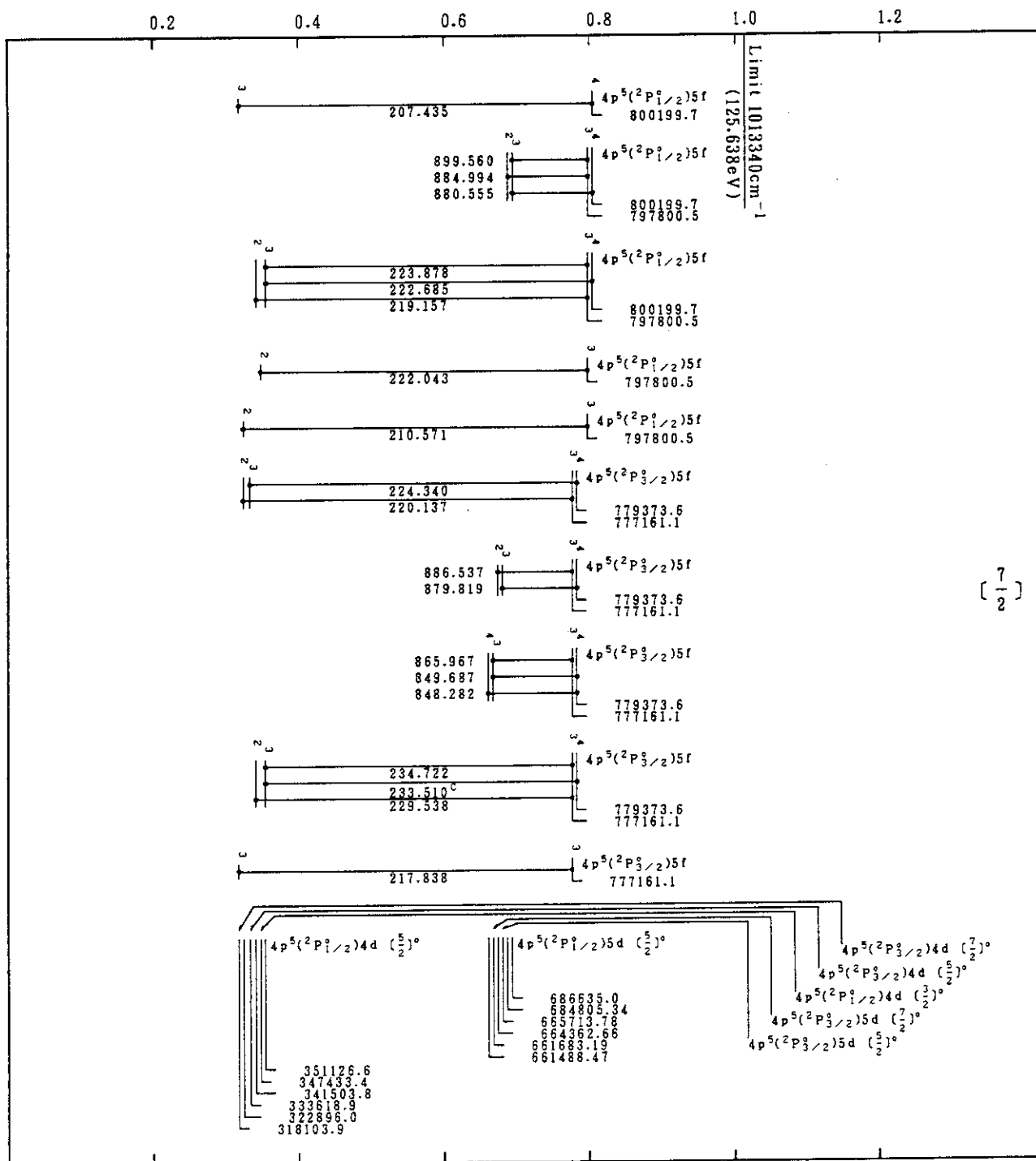
Mo VII(Kr-Sequence)
