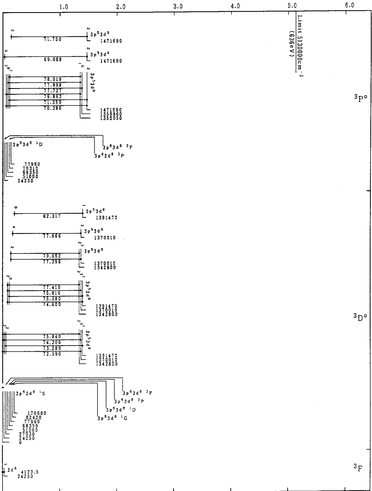
Mo XVII(Fe-Sequence)
