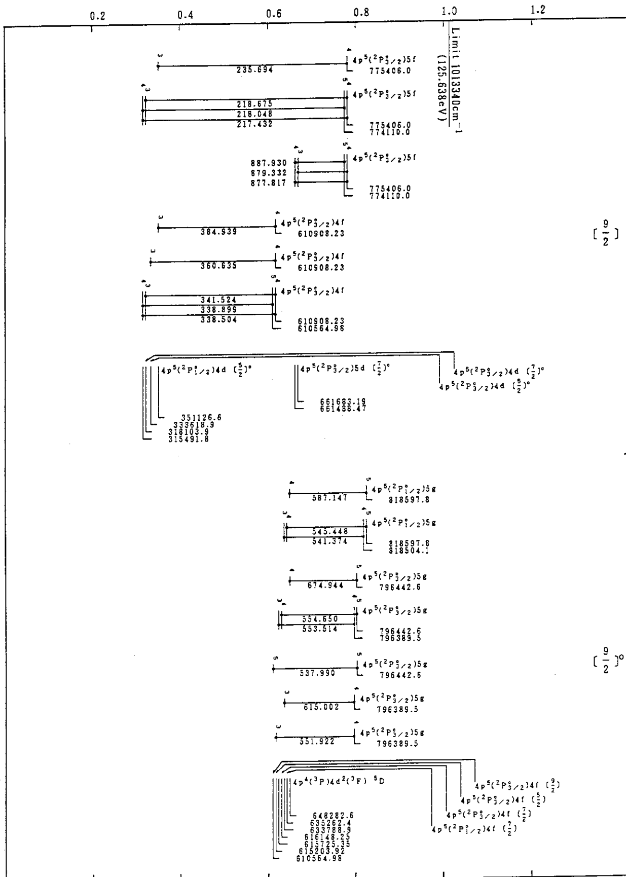
Mo VII(Kr-Sequence)
