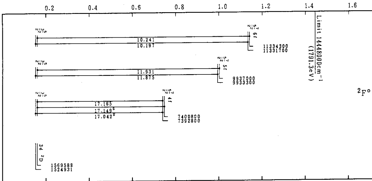
Mo XXXII(Na-Sequence)
