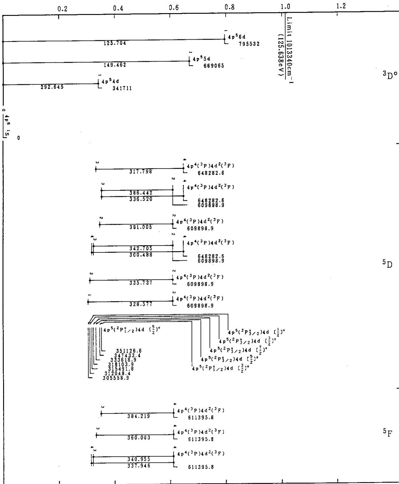
Mo VII(Kr-Sequence)
