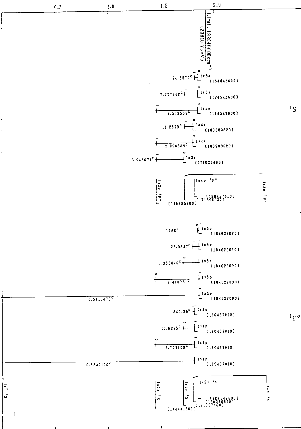
Mo XLI(He-Sequence)
