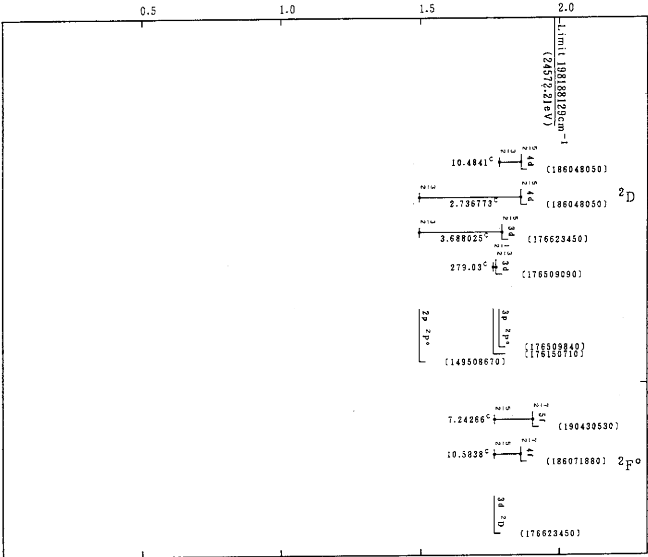
Mo XLII(H-Sequence)
