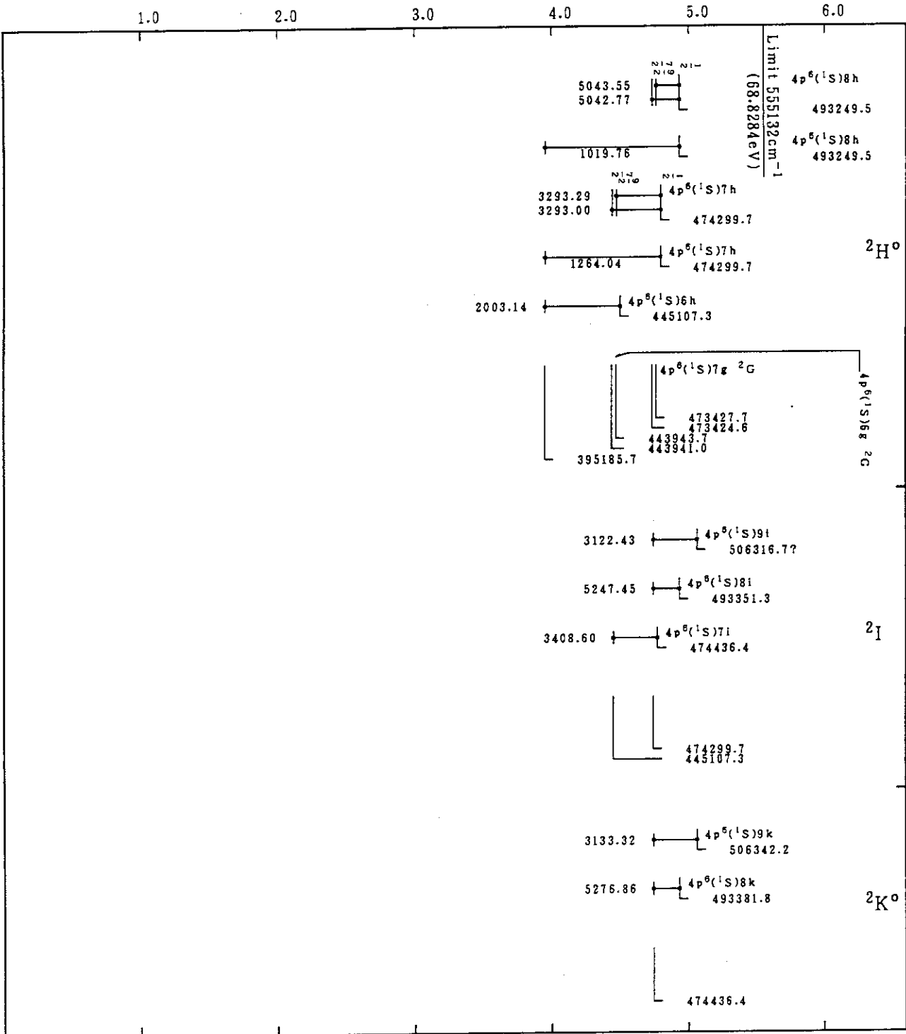
Mo VI(Rb-Sequence)
