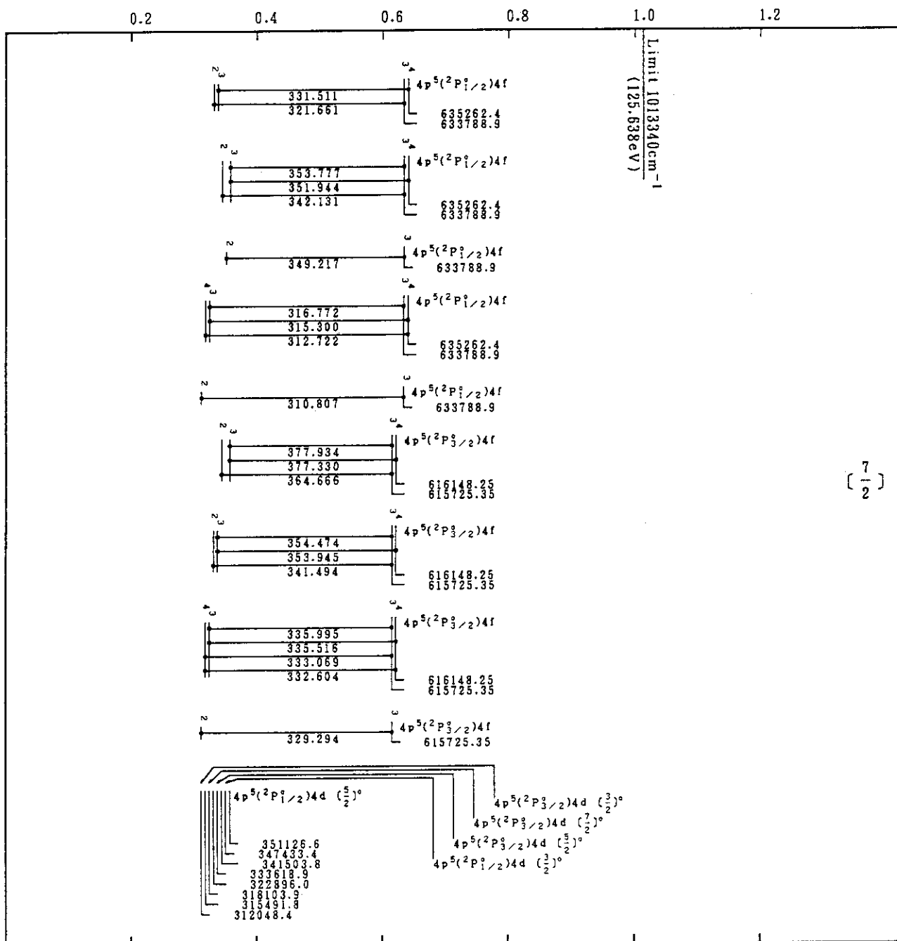
Mo VII(Kr-Sequence)
