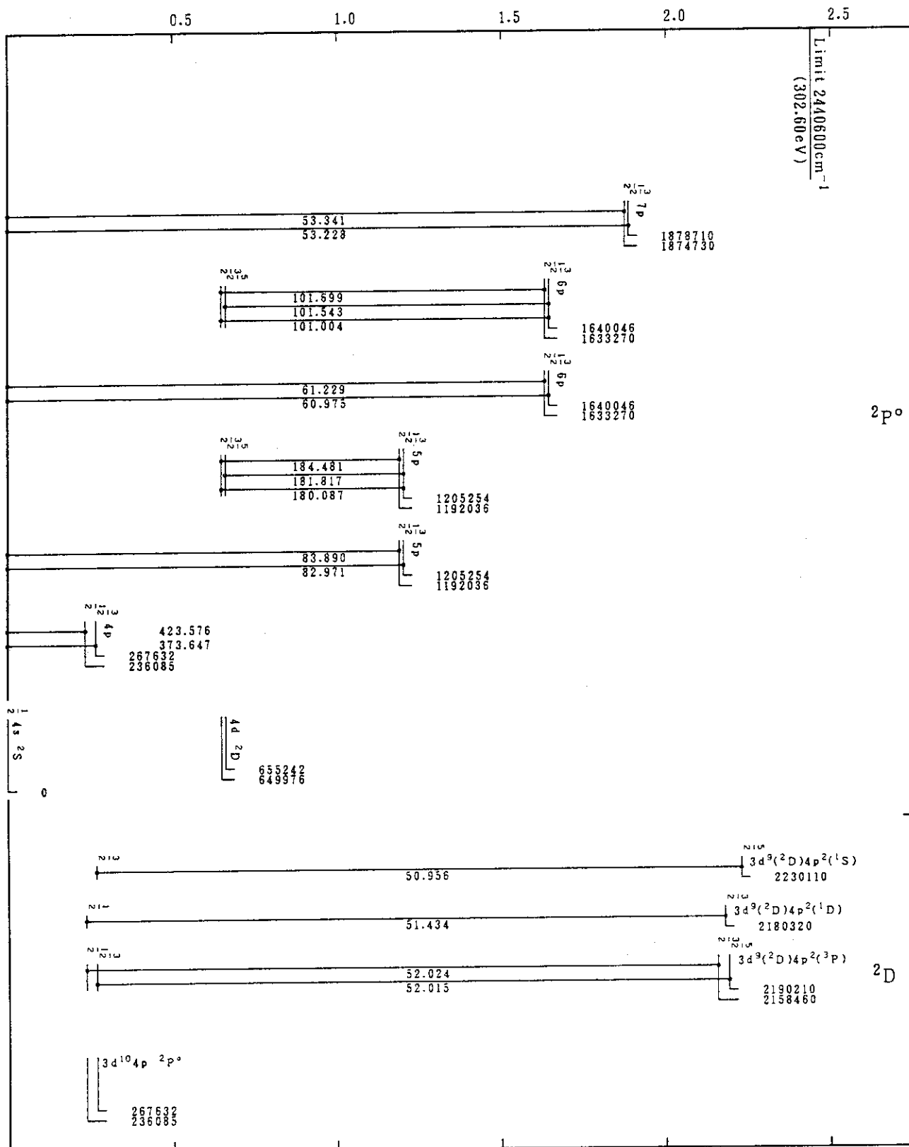
Mo XIV(Cu-Sequence)
