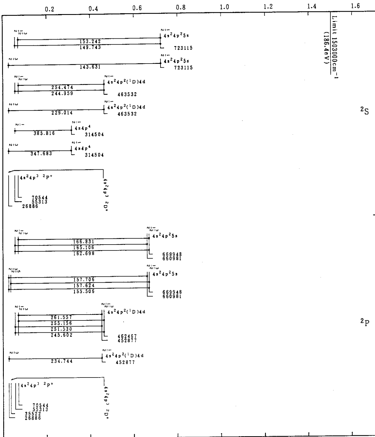
Mo X(As-Sequence)
