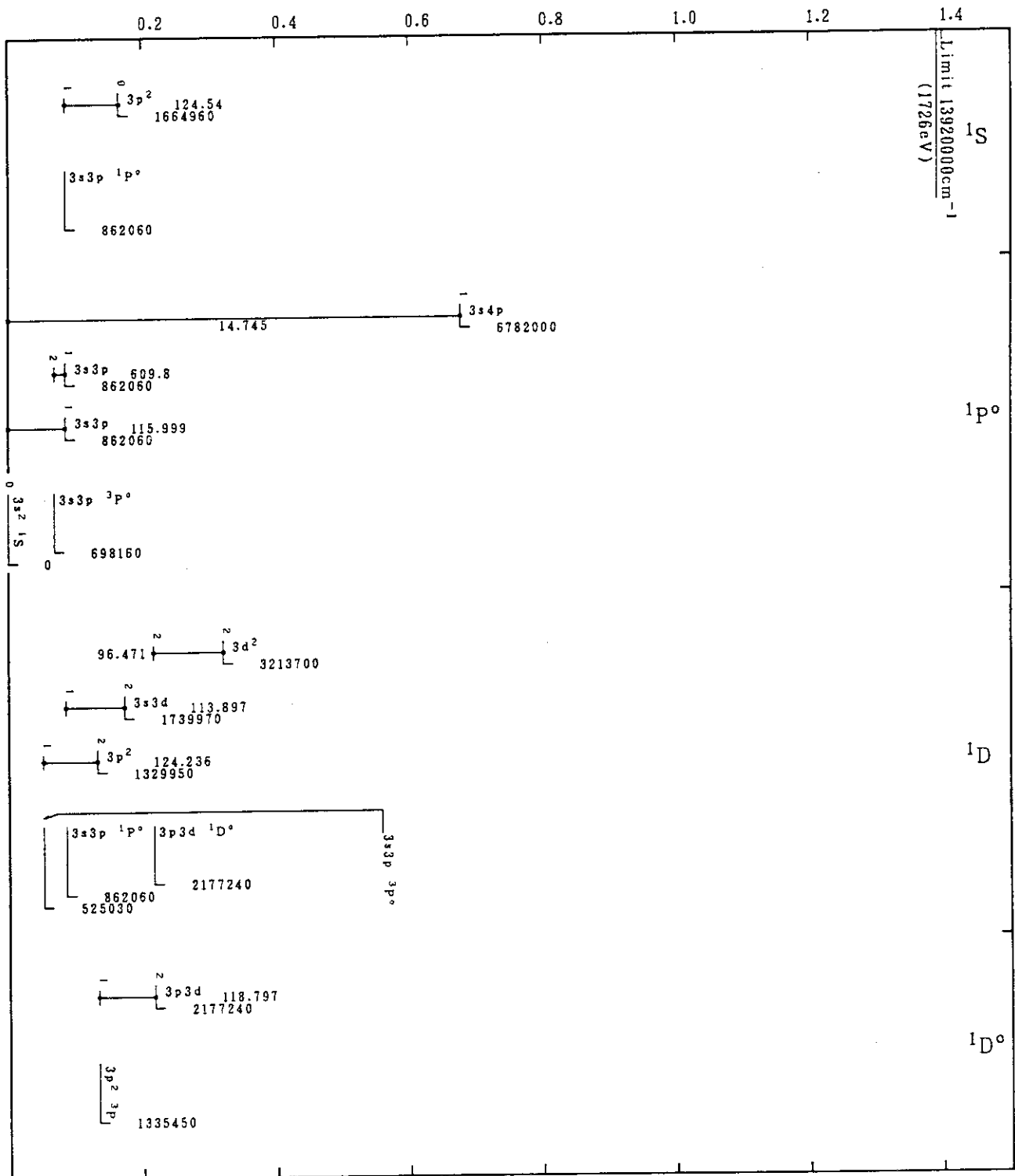
Mo XXXI(Mg-Sequence)
