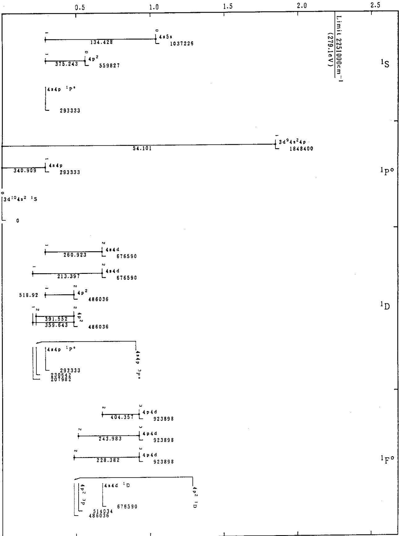
Mo XIII(Zn-Sequence)
