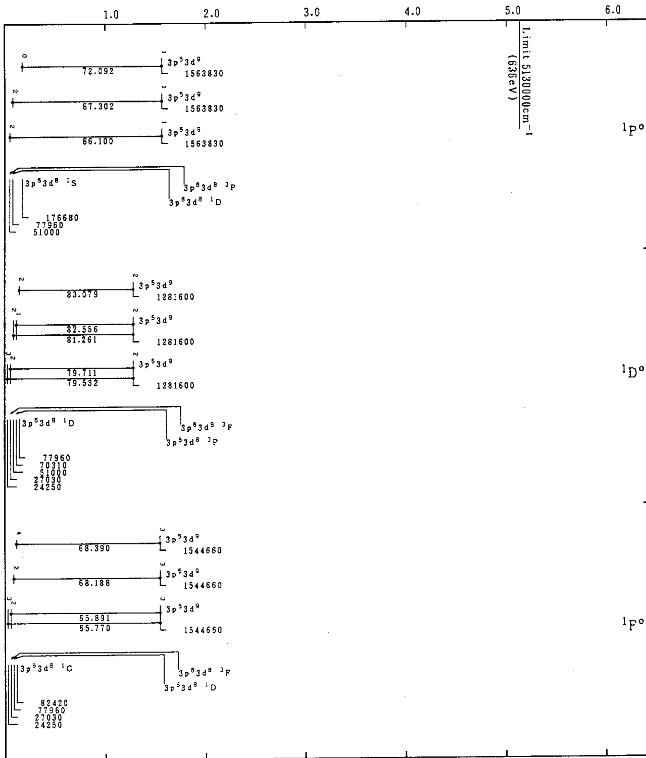
Mo XVII(Fe-Sequence)
