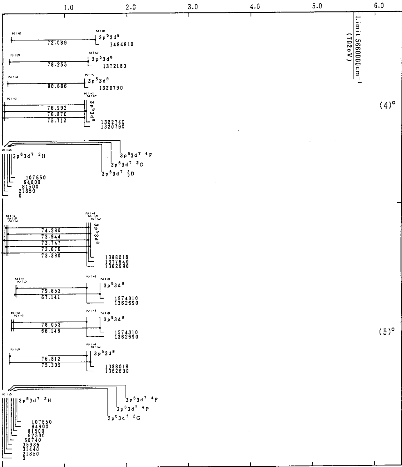
Mo XVIII(Mn-Sequence)
