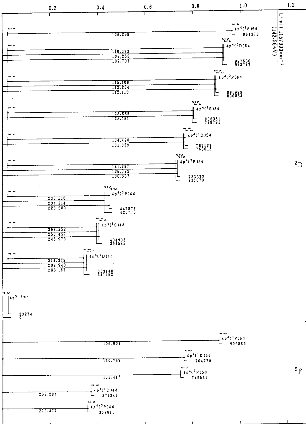
Mo VIII(Br-Sequence)
