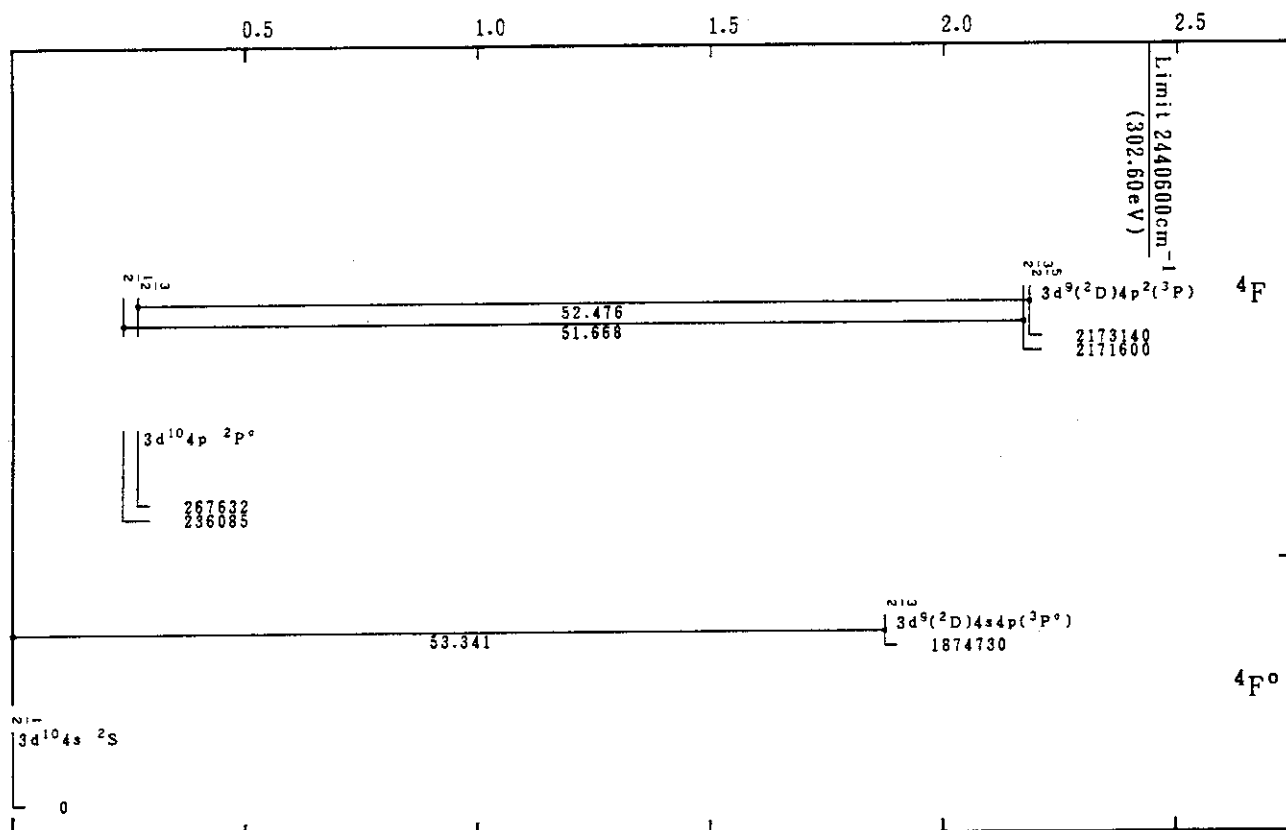
Mo XIV(Cu-Sequence)
