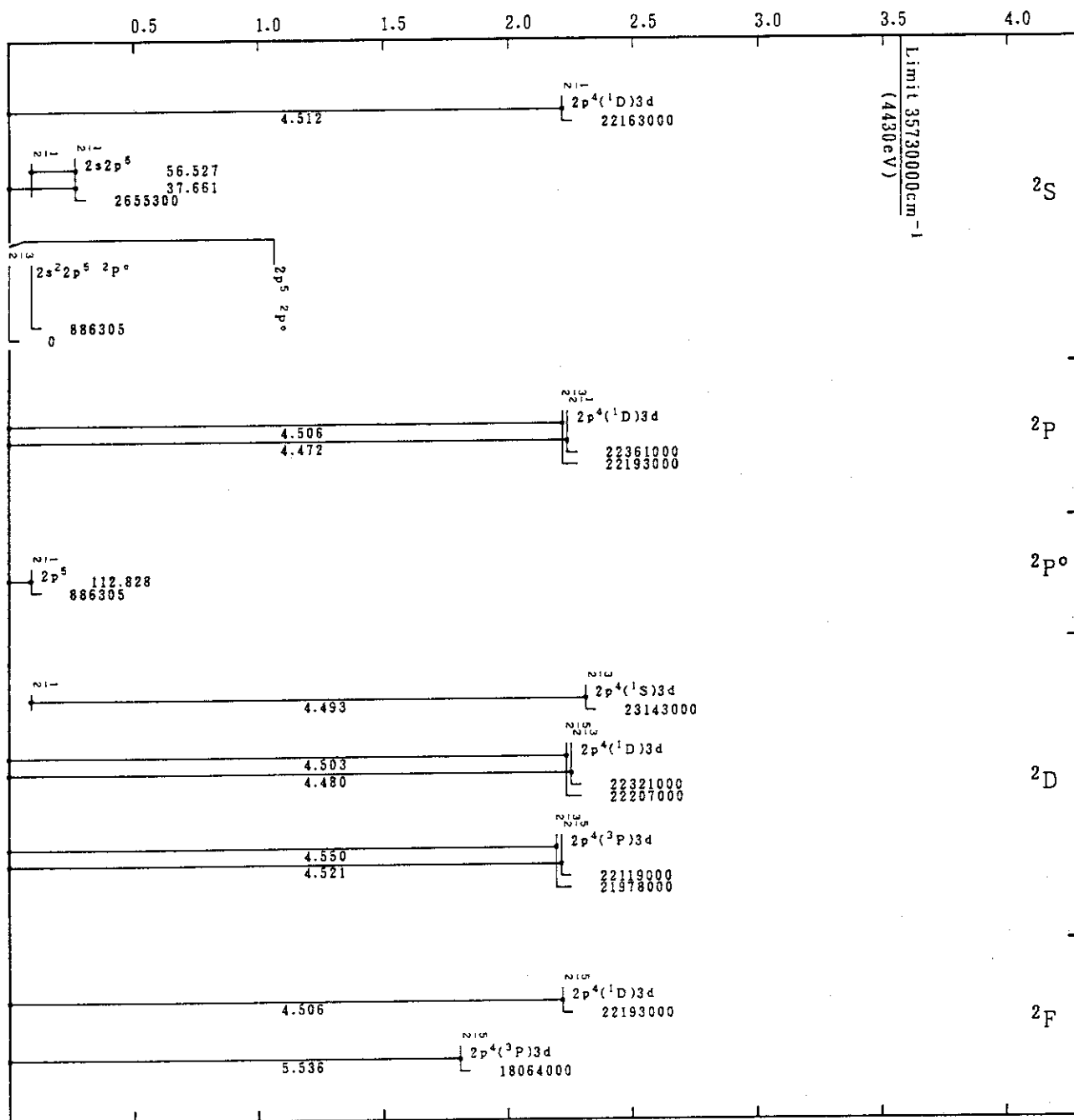
Mo XXXIV(F-Sequence)
