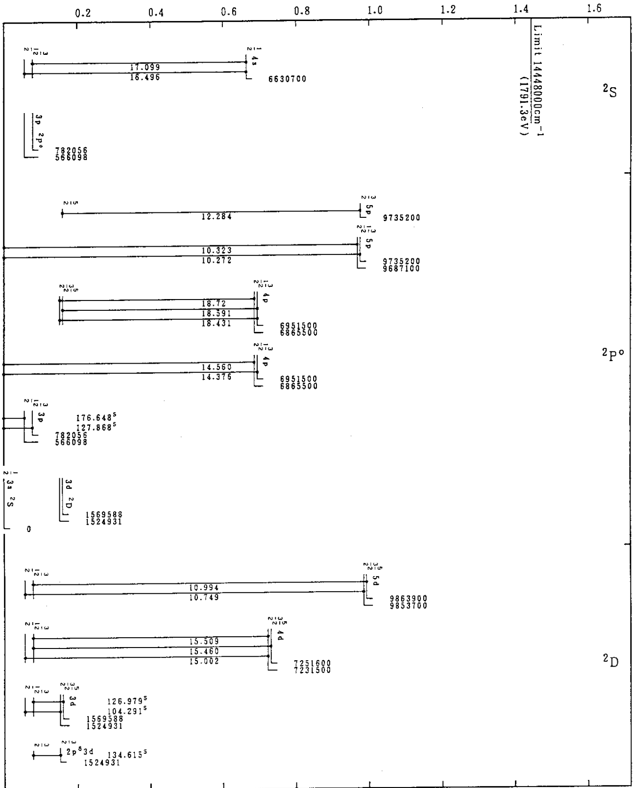
Mo XXXII(Na-Sequence)
