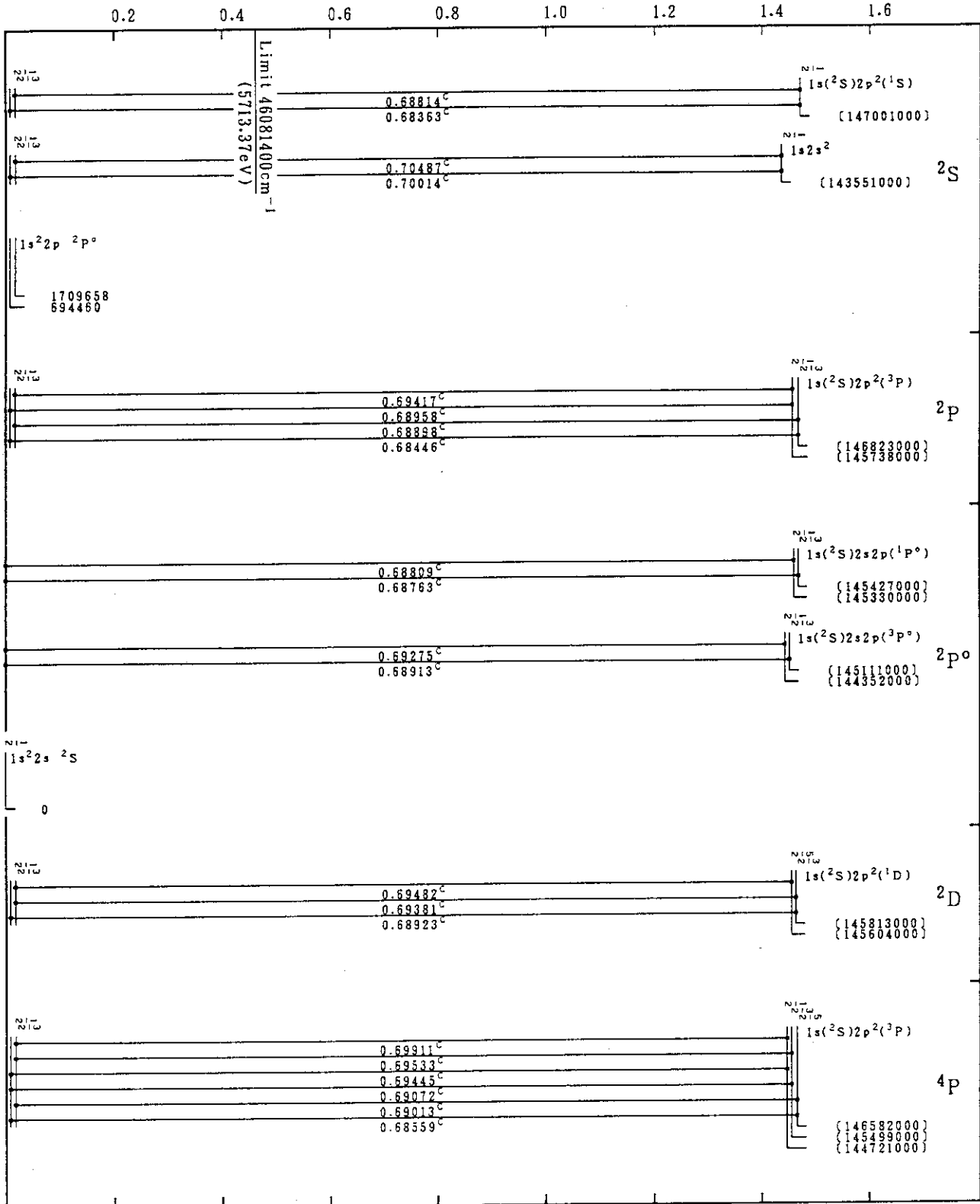
Mo XL(Li-Sequence)
