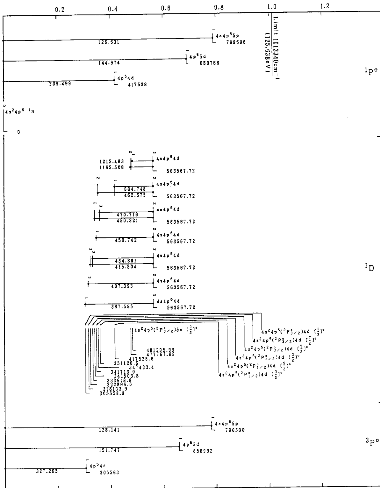
Mo VII(Kr-Sequence)
