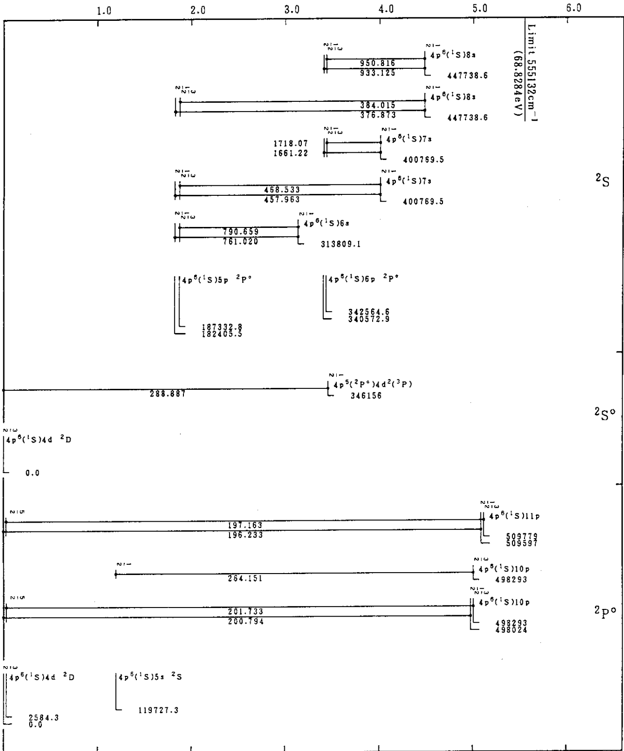
Mo VI(Rb-Sequence)
