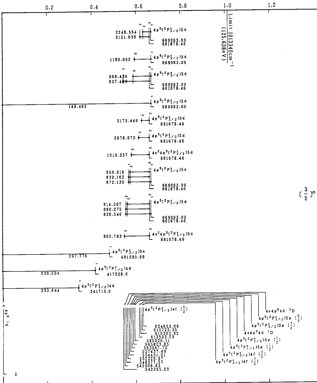
Mo VII(Kr-Sequence)
