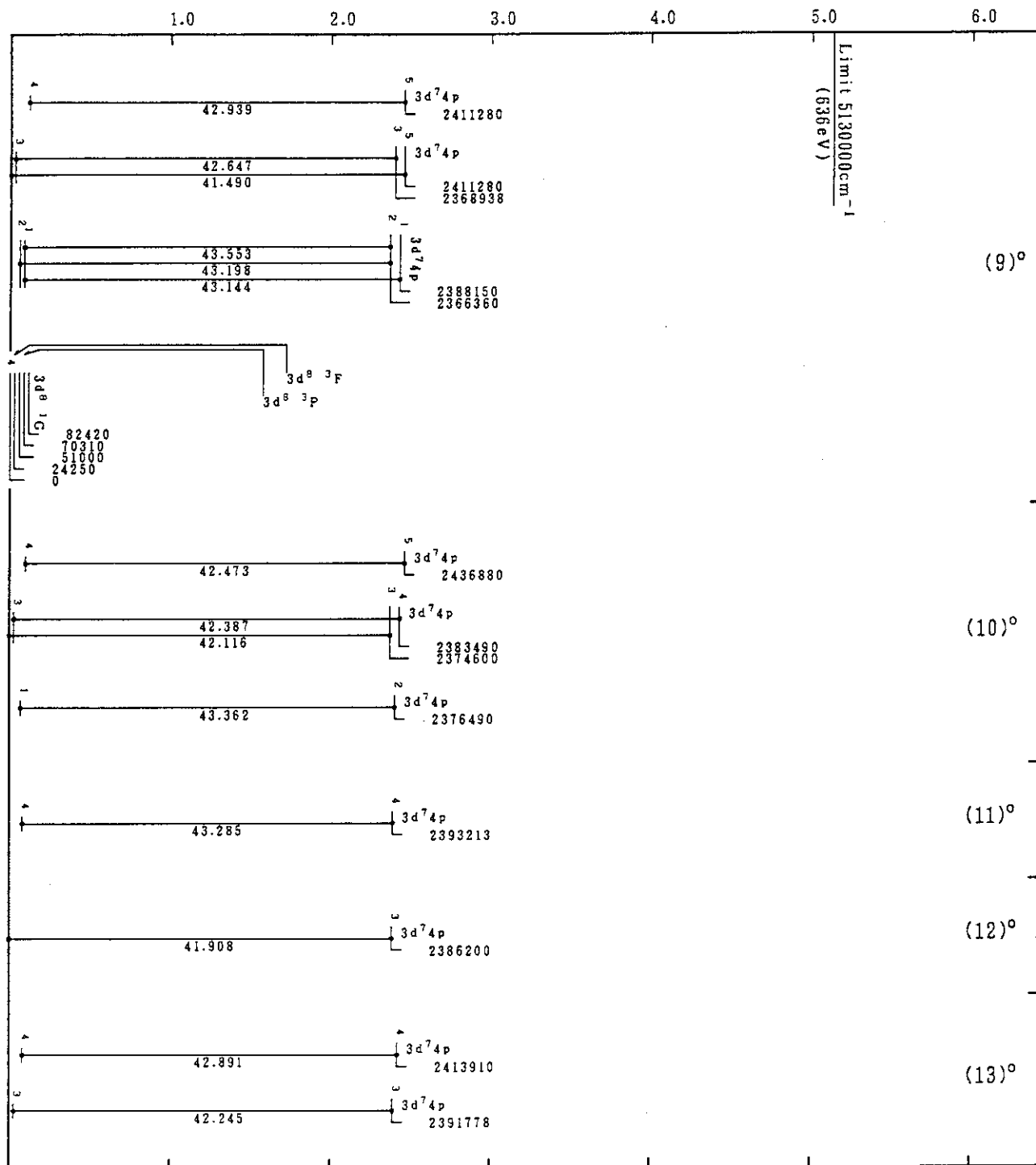
Mo XVII(Fe-Sequence)
