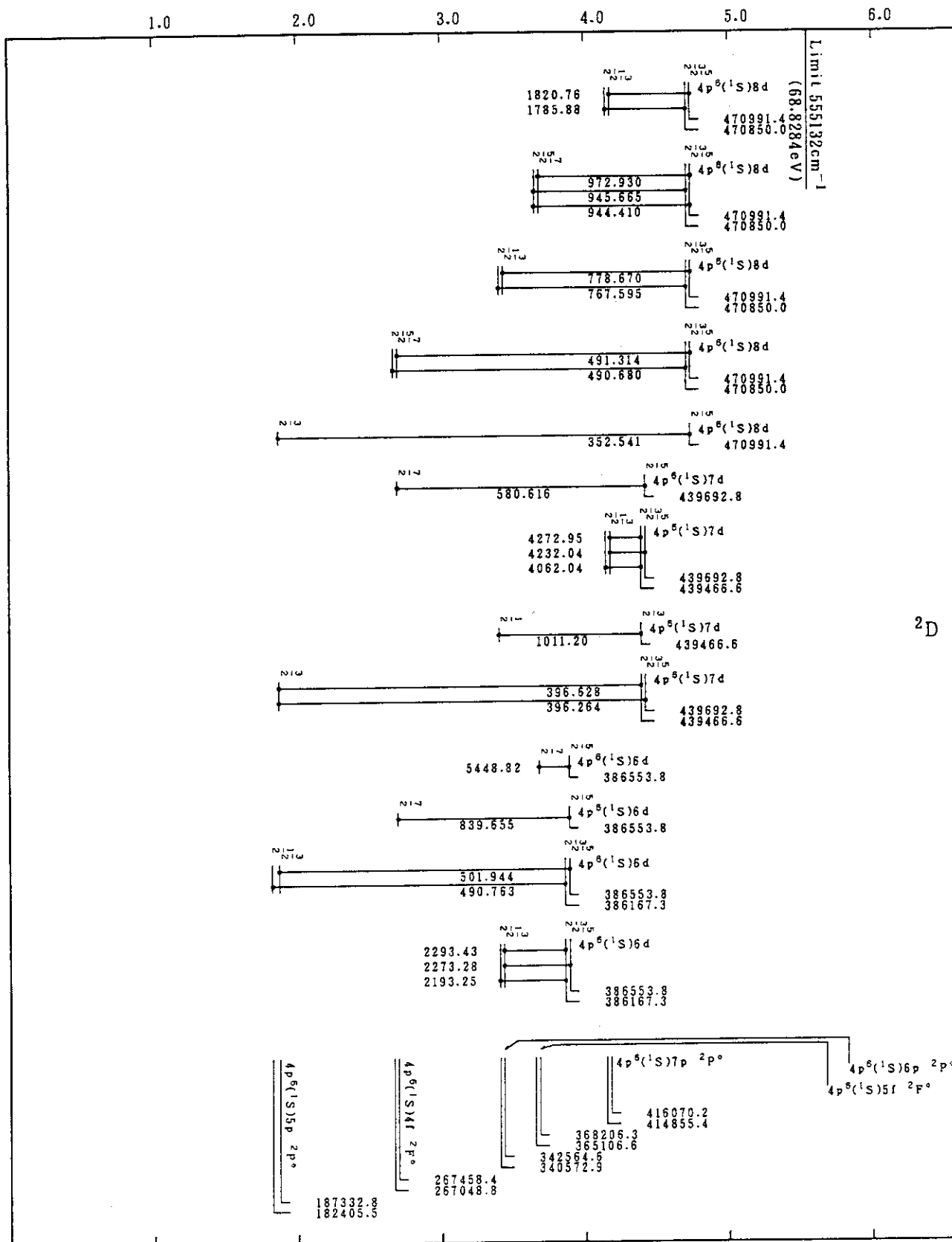
Mo VI(Rb-Sequence)
