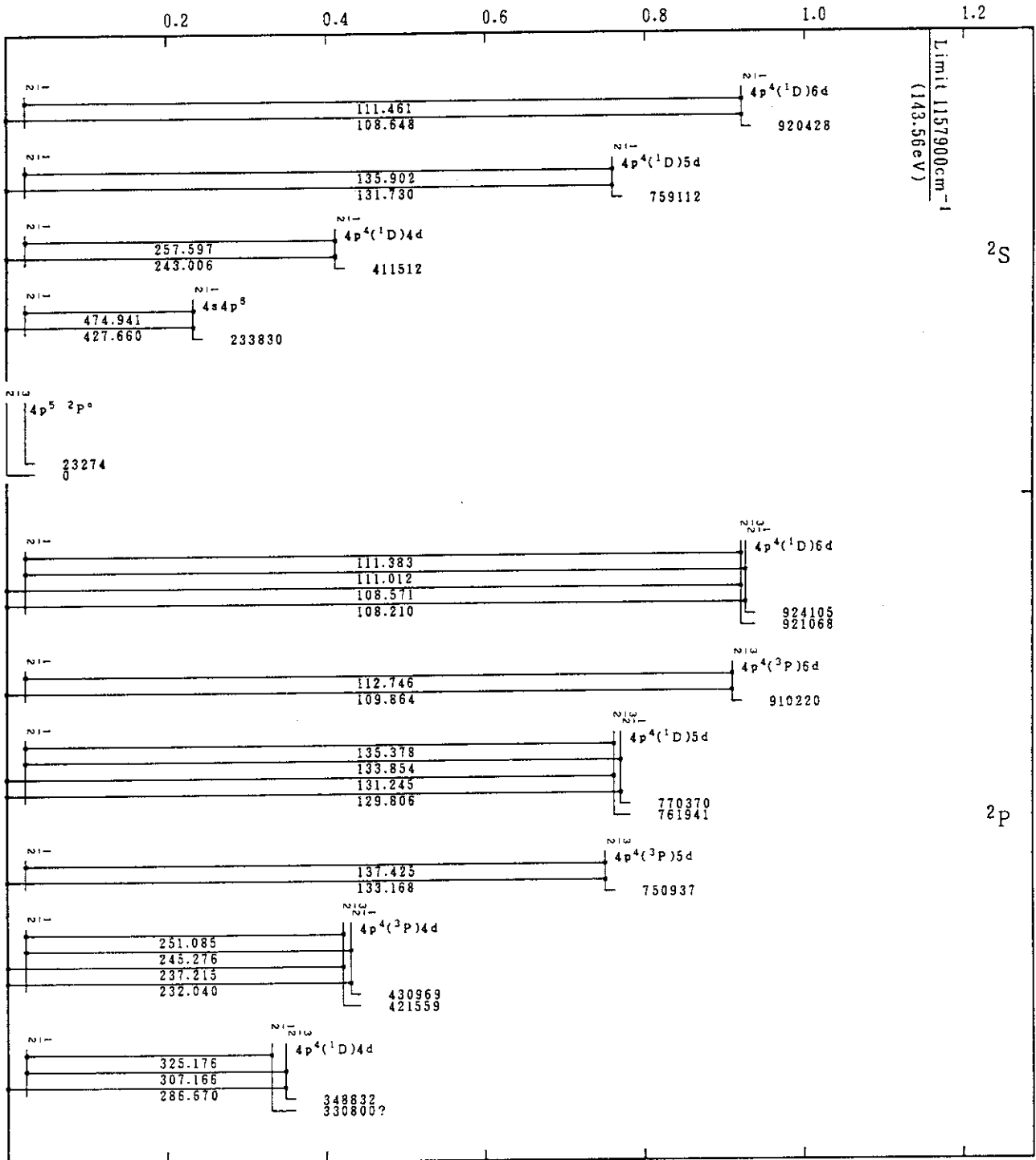
Mo VIII(Br-Sequence)
