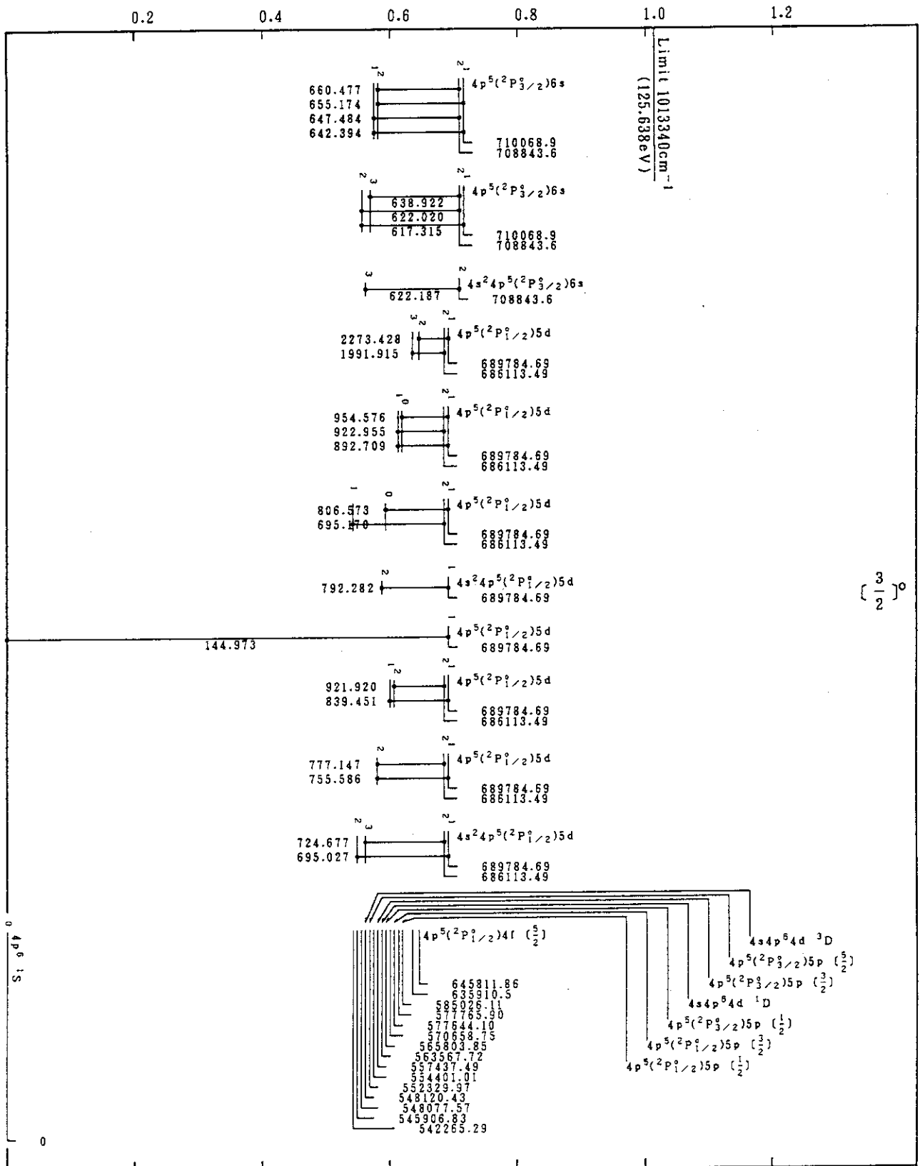
Mo VII(Kr-Sequence)
