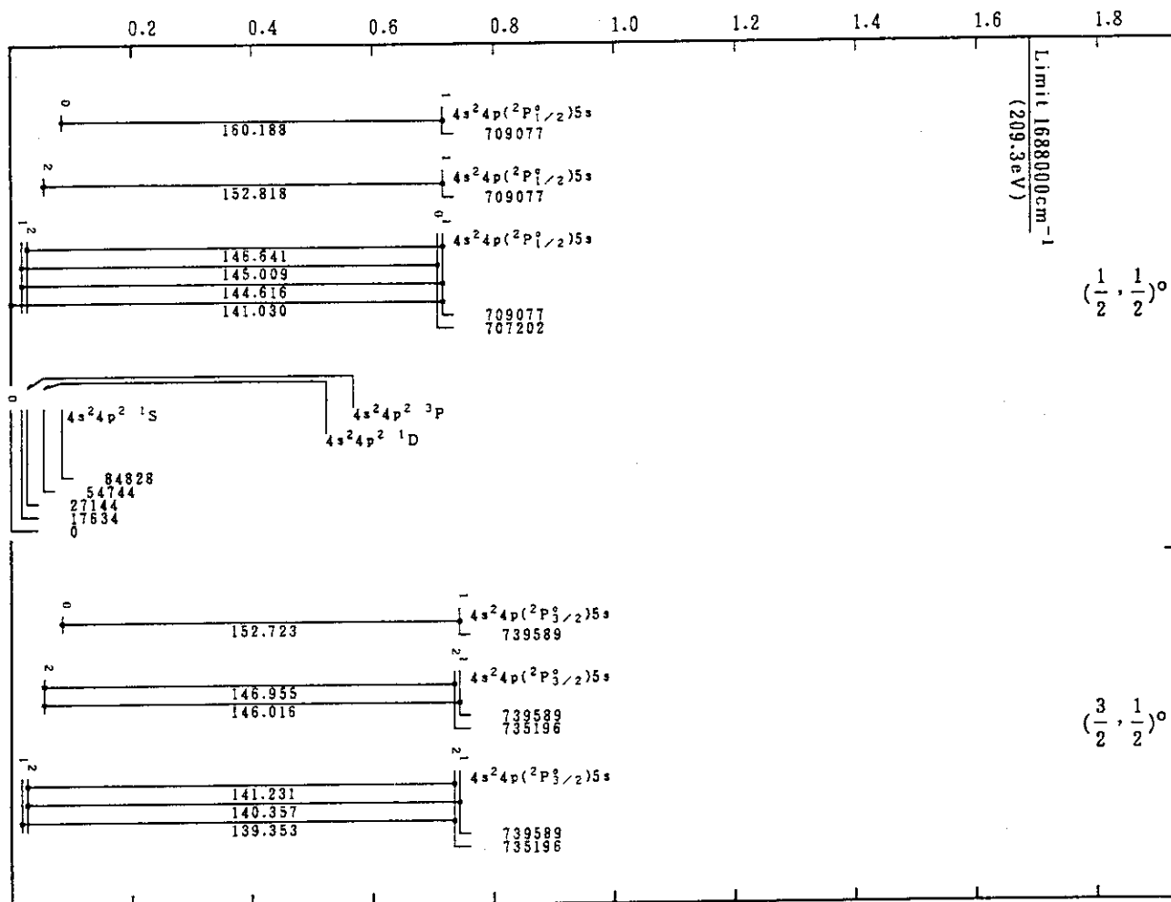
Mo XI(Ge-Sequence)
