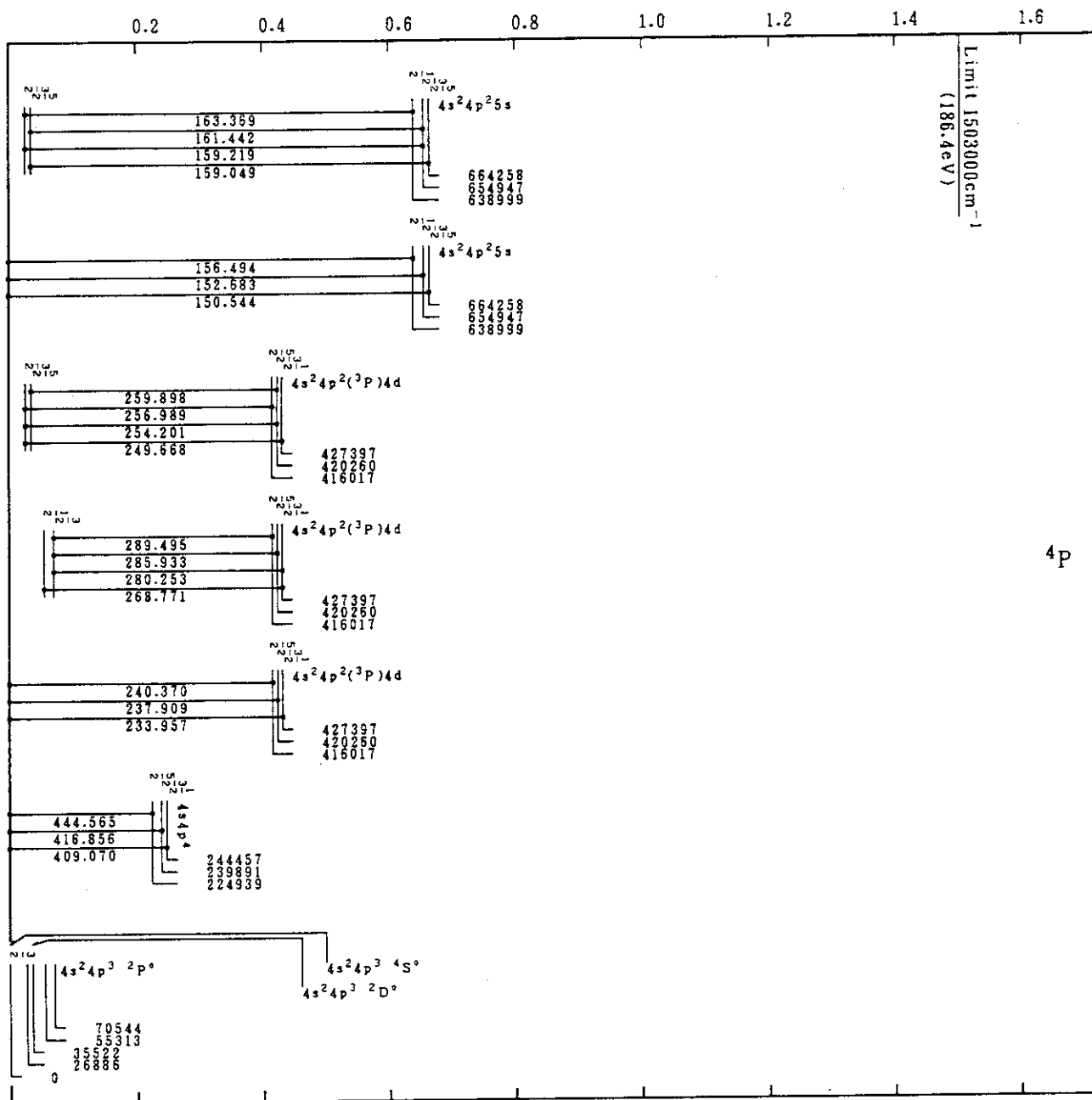
Mo X(As-Sequence)
