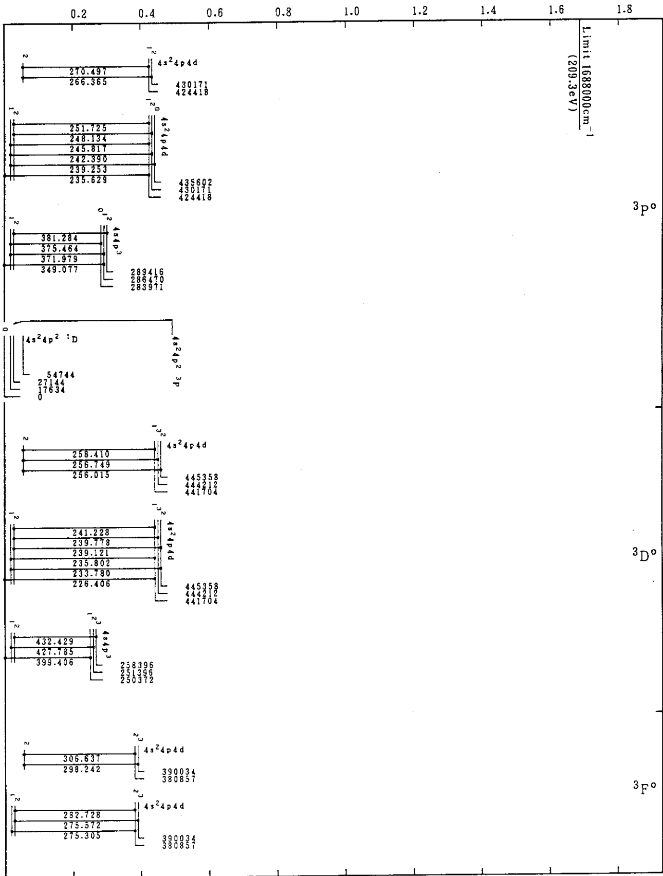
Mo XI(Ge-Sequence)
