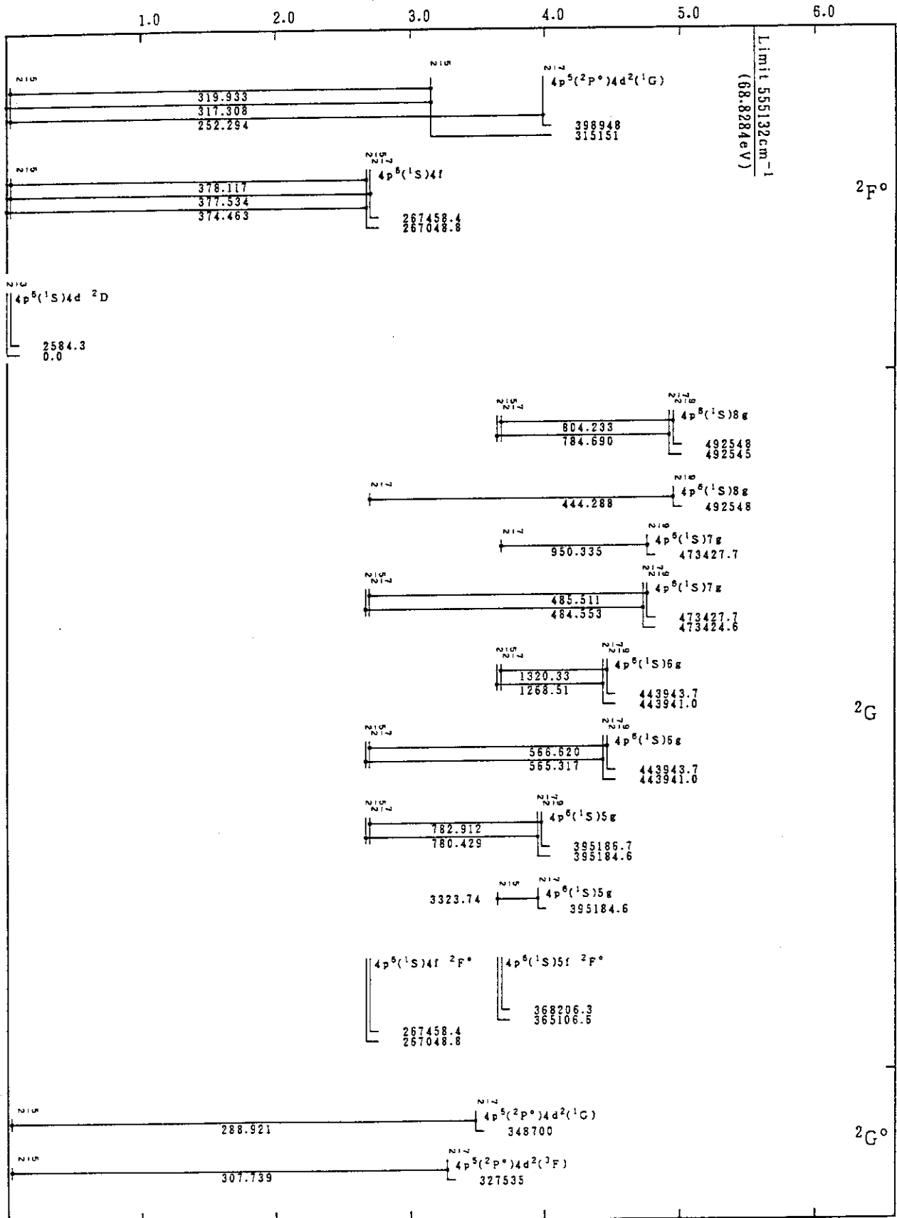
Mo VI(Rb-Sequence)
