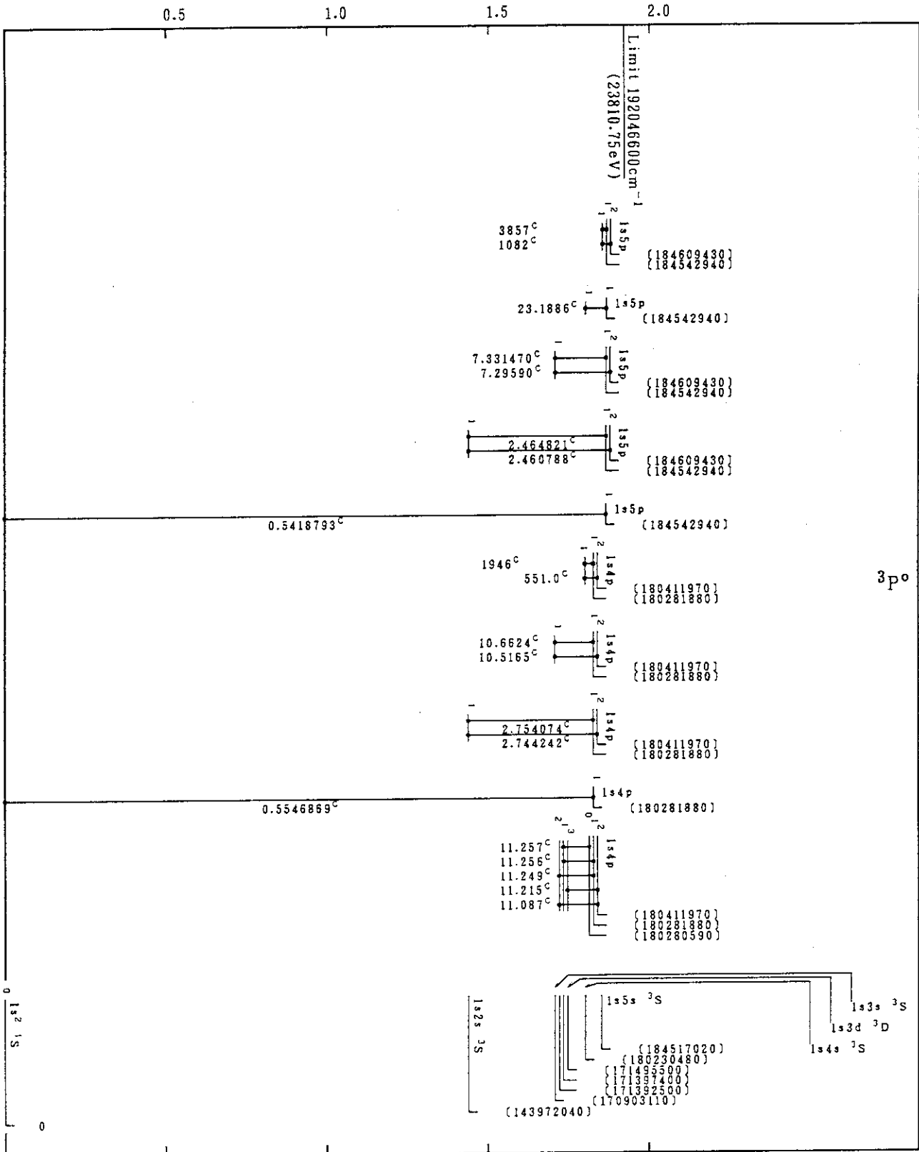
Mo XLI(He-Sequence)
