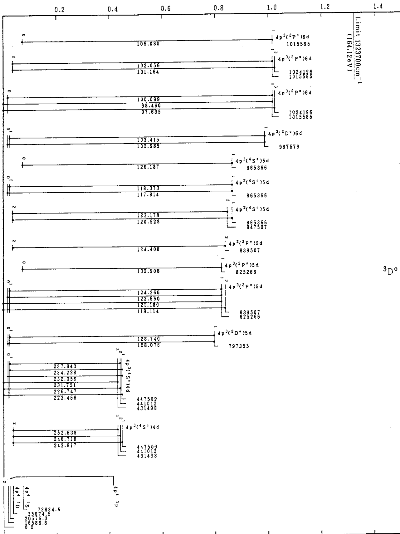
Mo IX(Se-Sequence)
