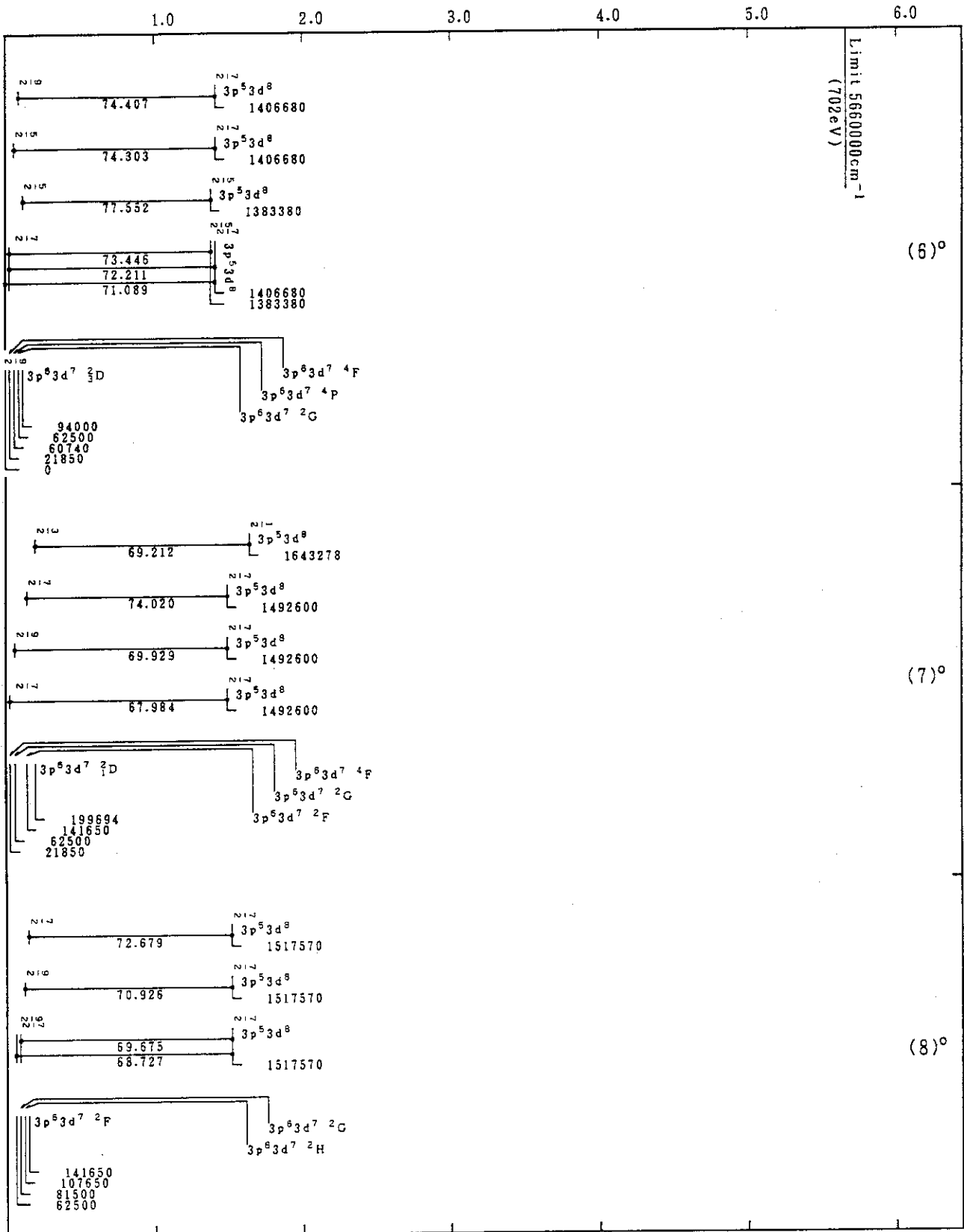
Mo XVIII(Mn-Sequence)
