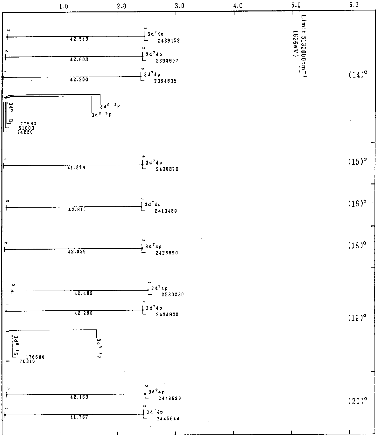
Mo XVII(Fe-Sequence)
