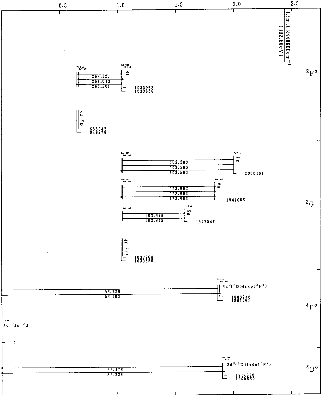
Mo XIV(Cu-Sequence)
