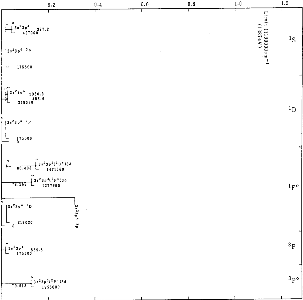
Mo XXVII(S-Sequence)
