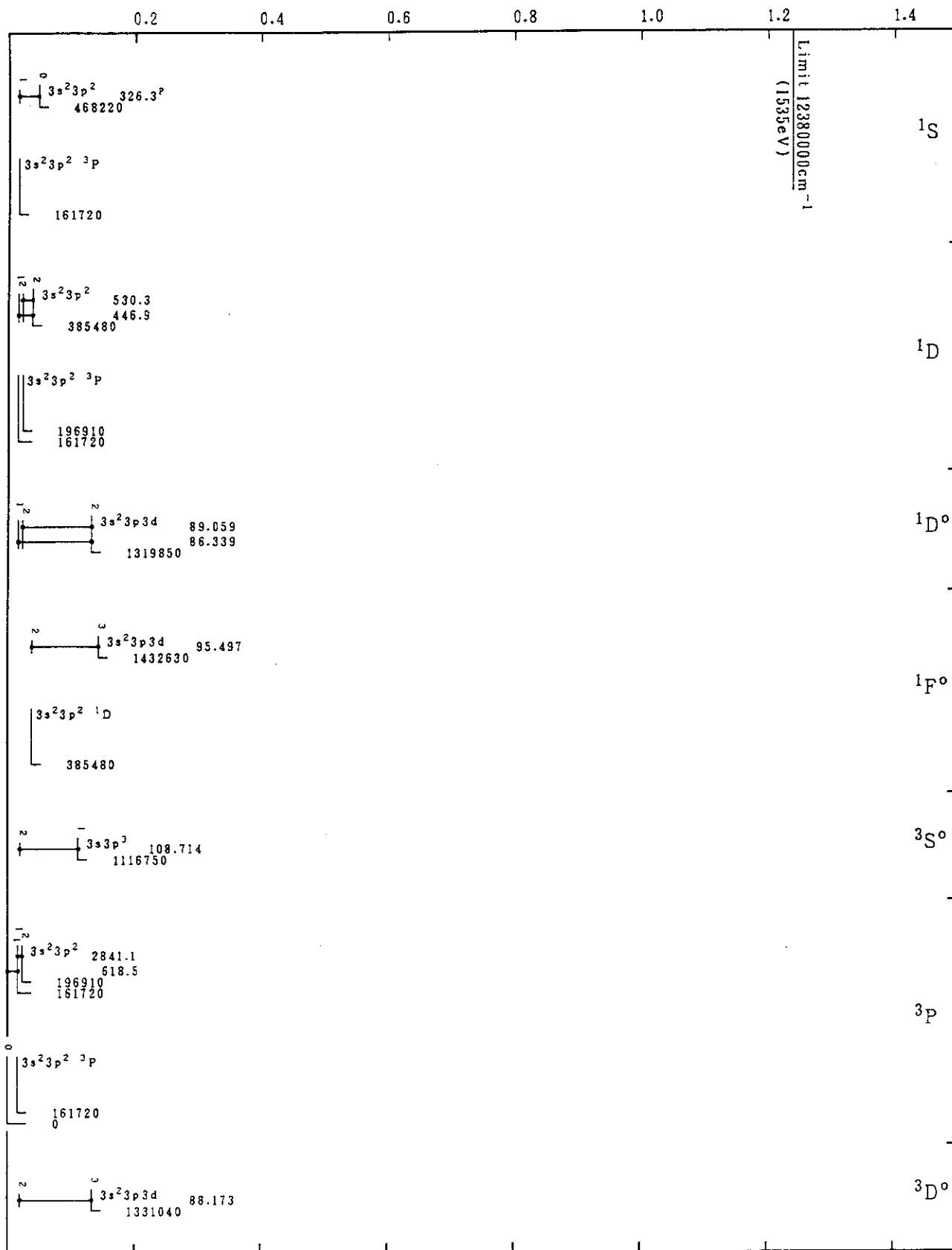
Mo XXIX(Si-Sequence)
