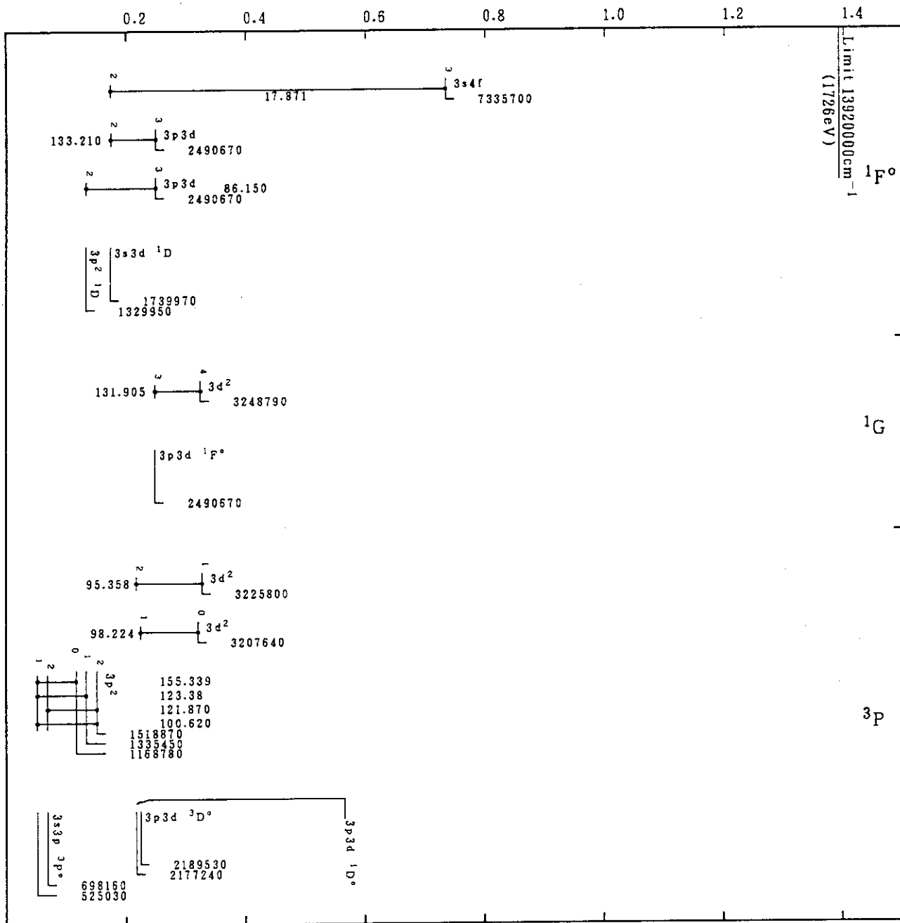
Mo XXXI(Mg-Sequence)
