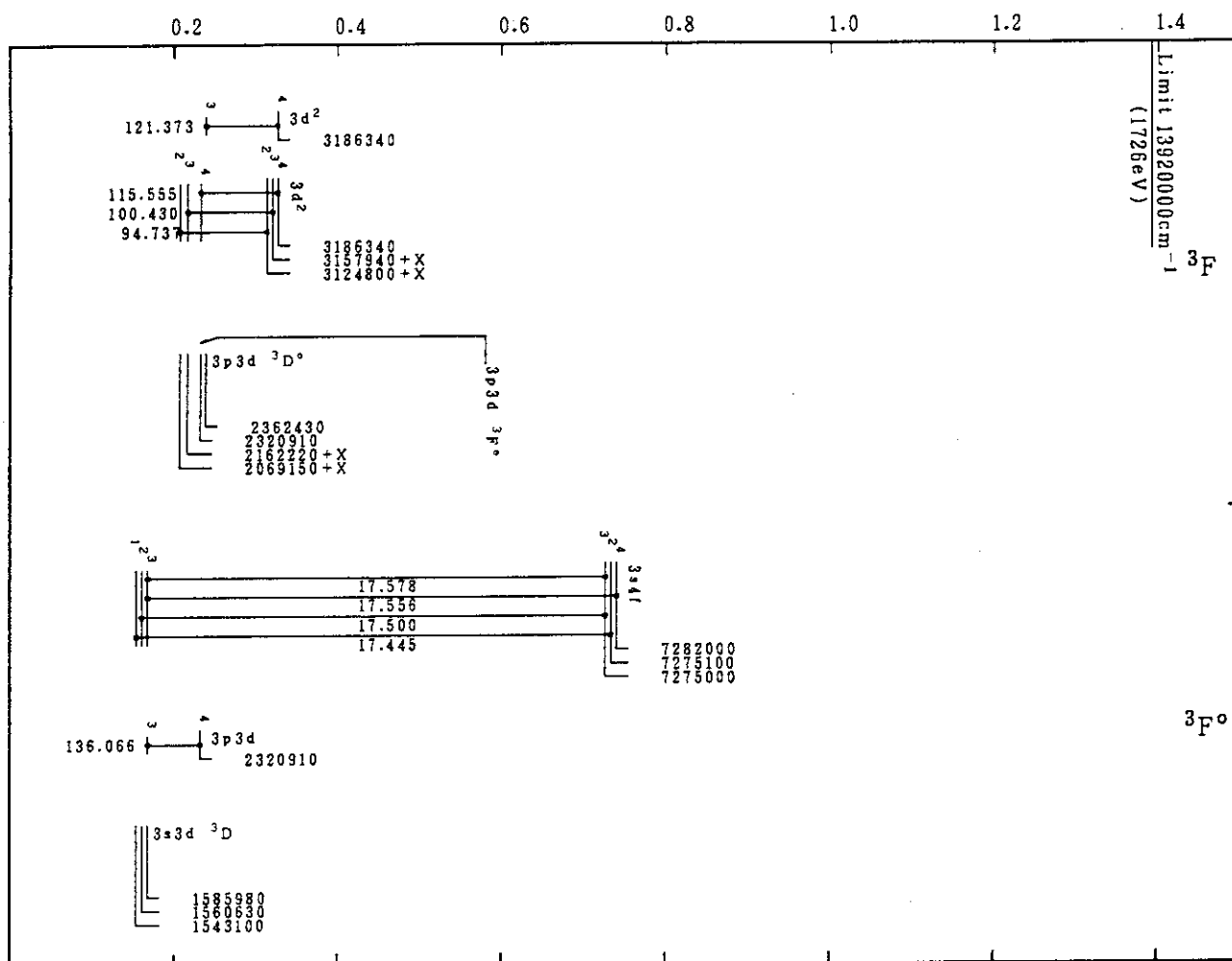
Mo XXXI(Mg-Sequence)
