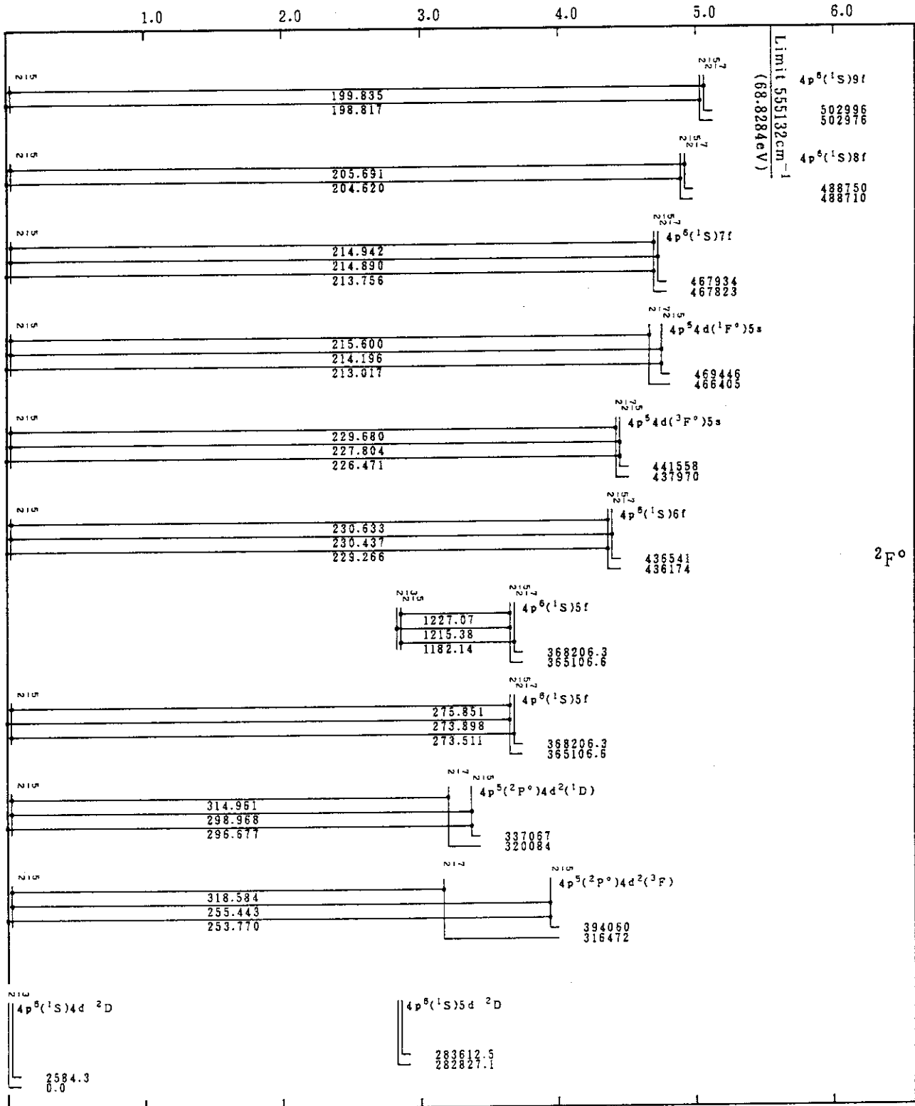
Mo VI(Rb-Sequence)
