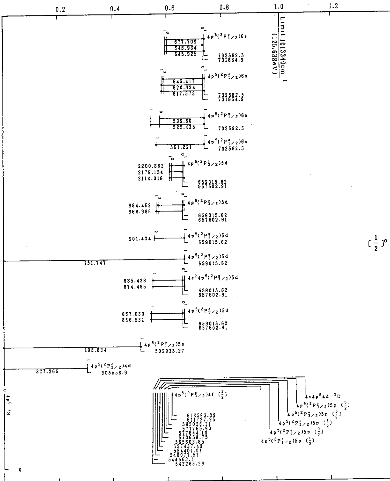
Mo VII(Kr-Sequence)
