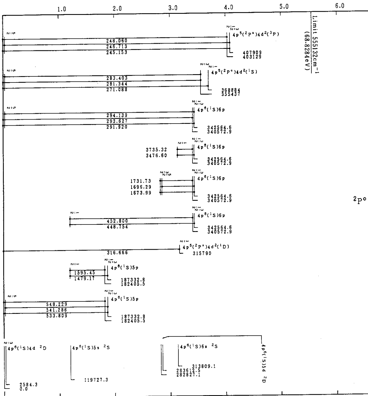
Mo VI(Rb-Sequence)
