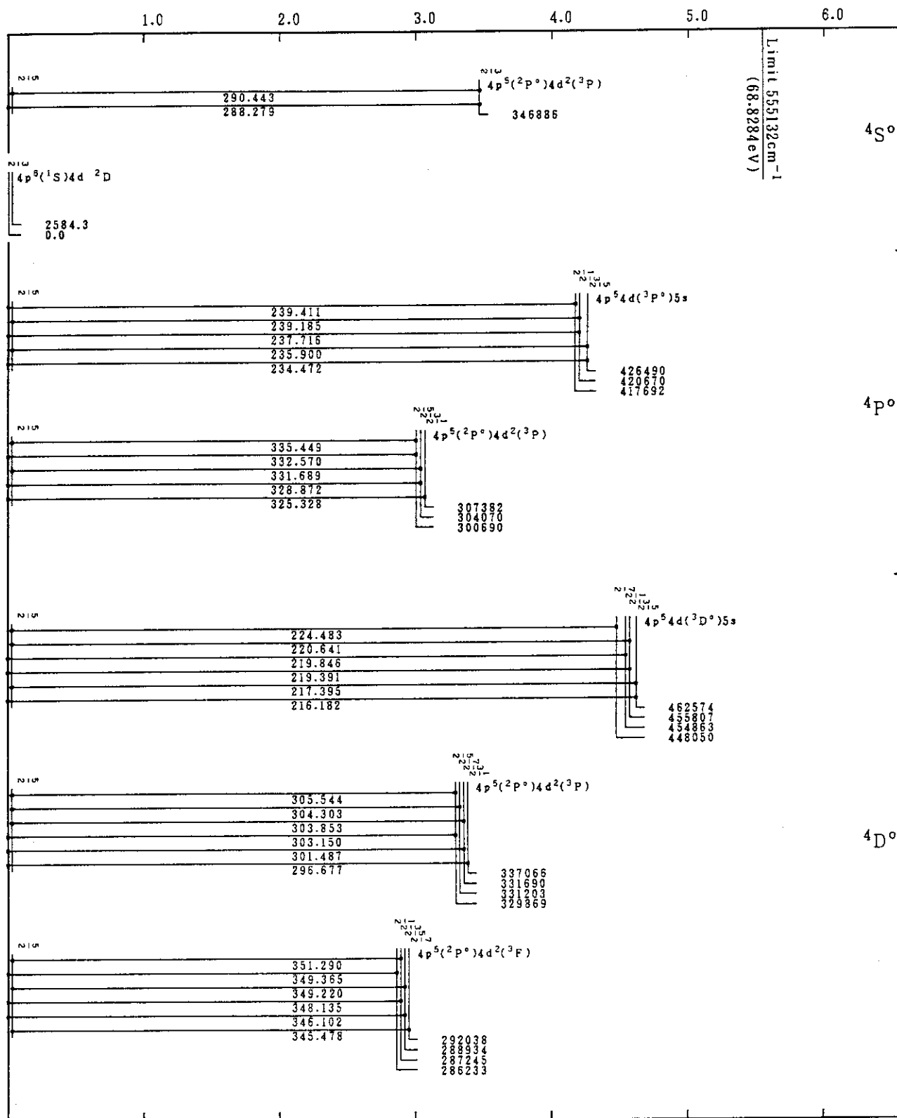
Mo VI(Rb-Sequence)
