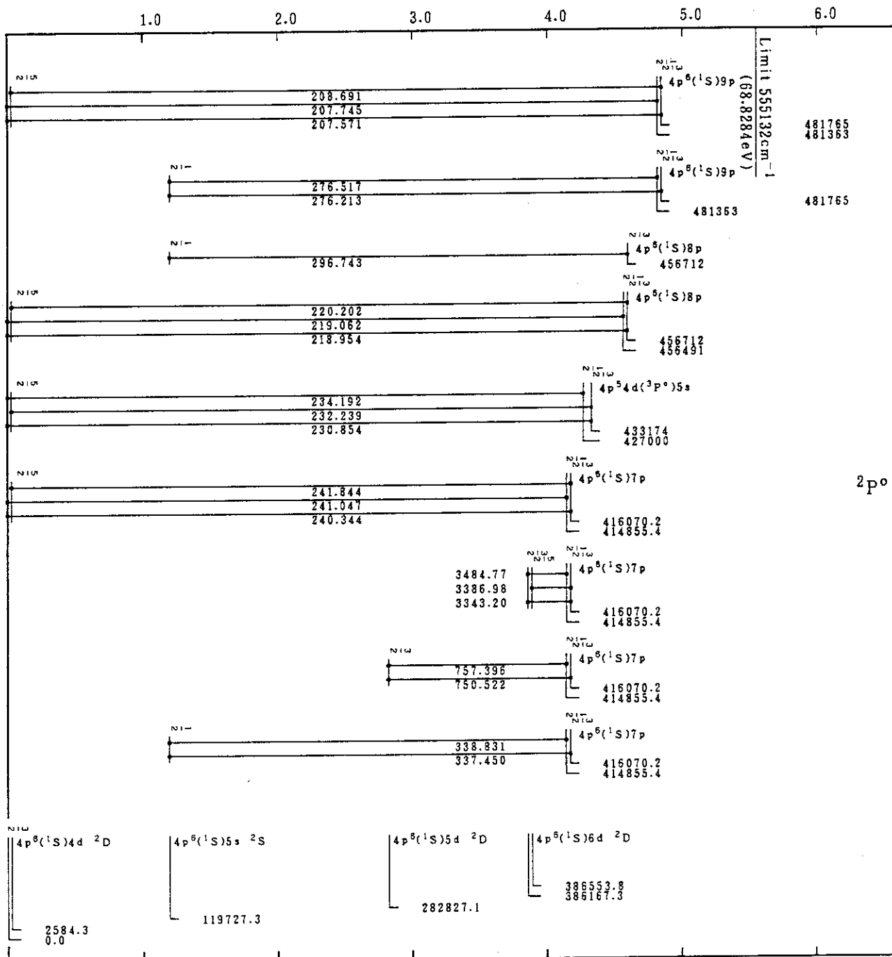
Mo VI(Rb-Sequence)
