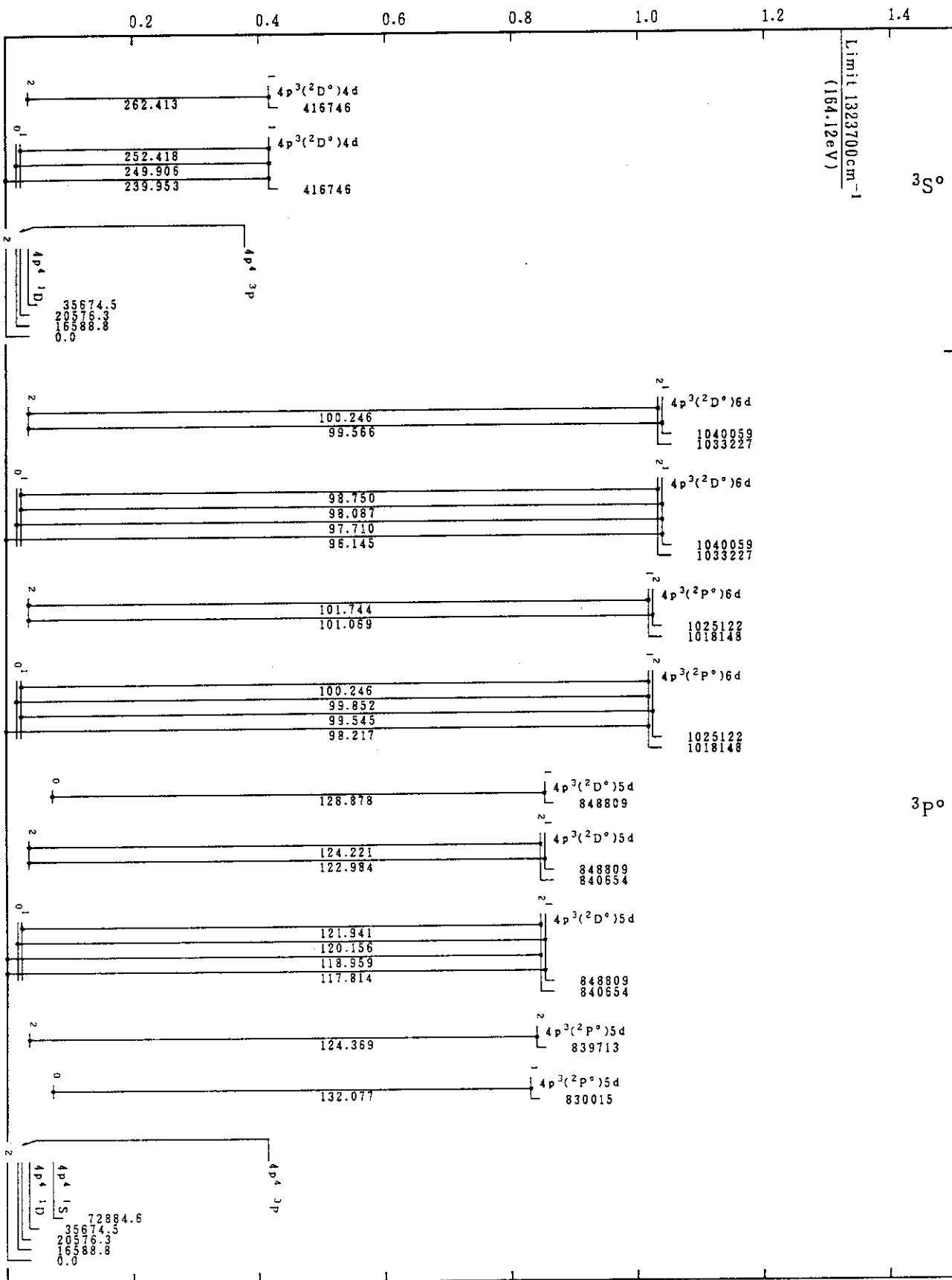
Mo IX(Se-Sequence)
