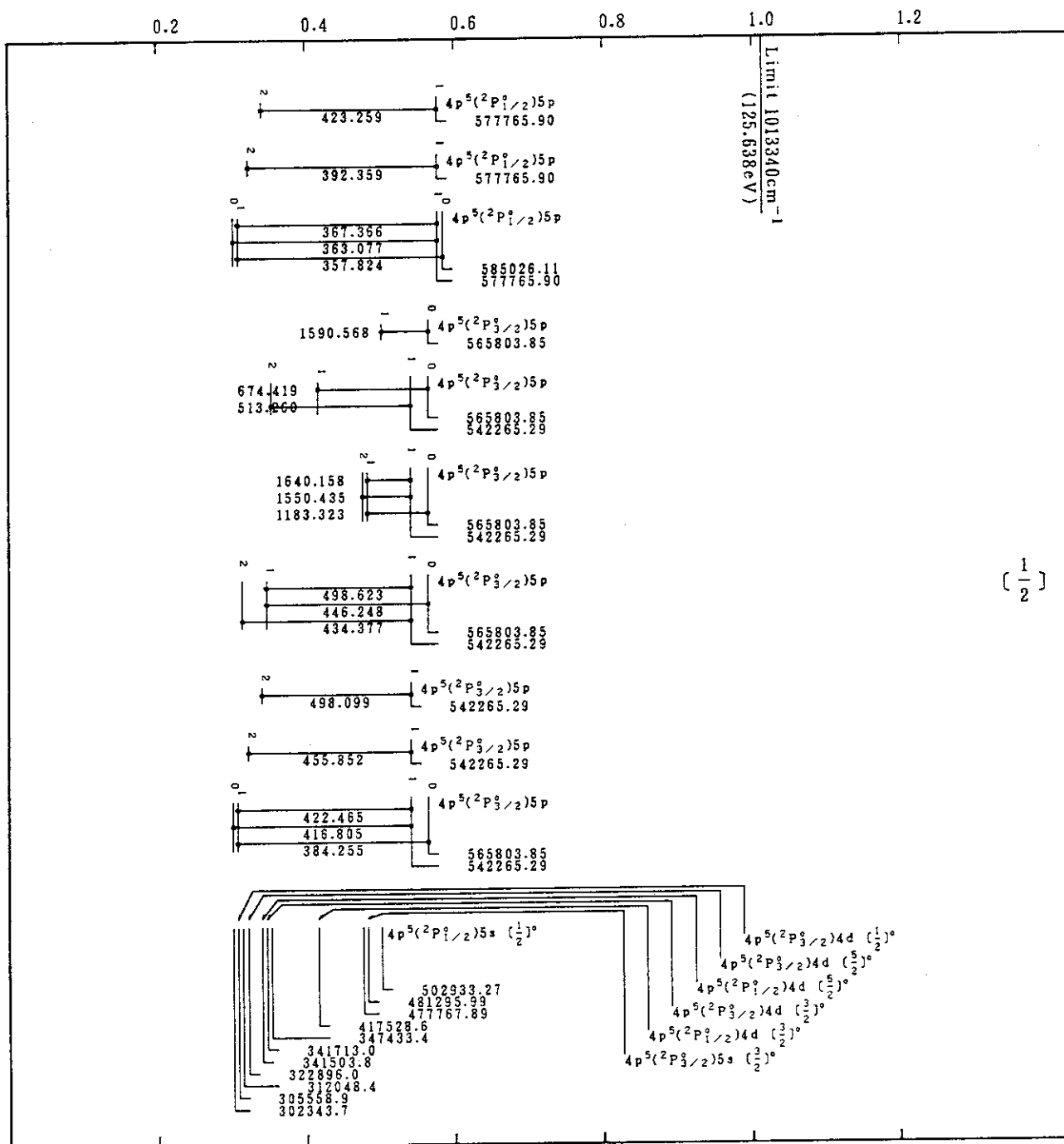
Mo VII(Kr-Sequence)
