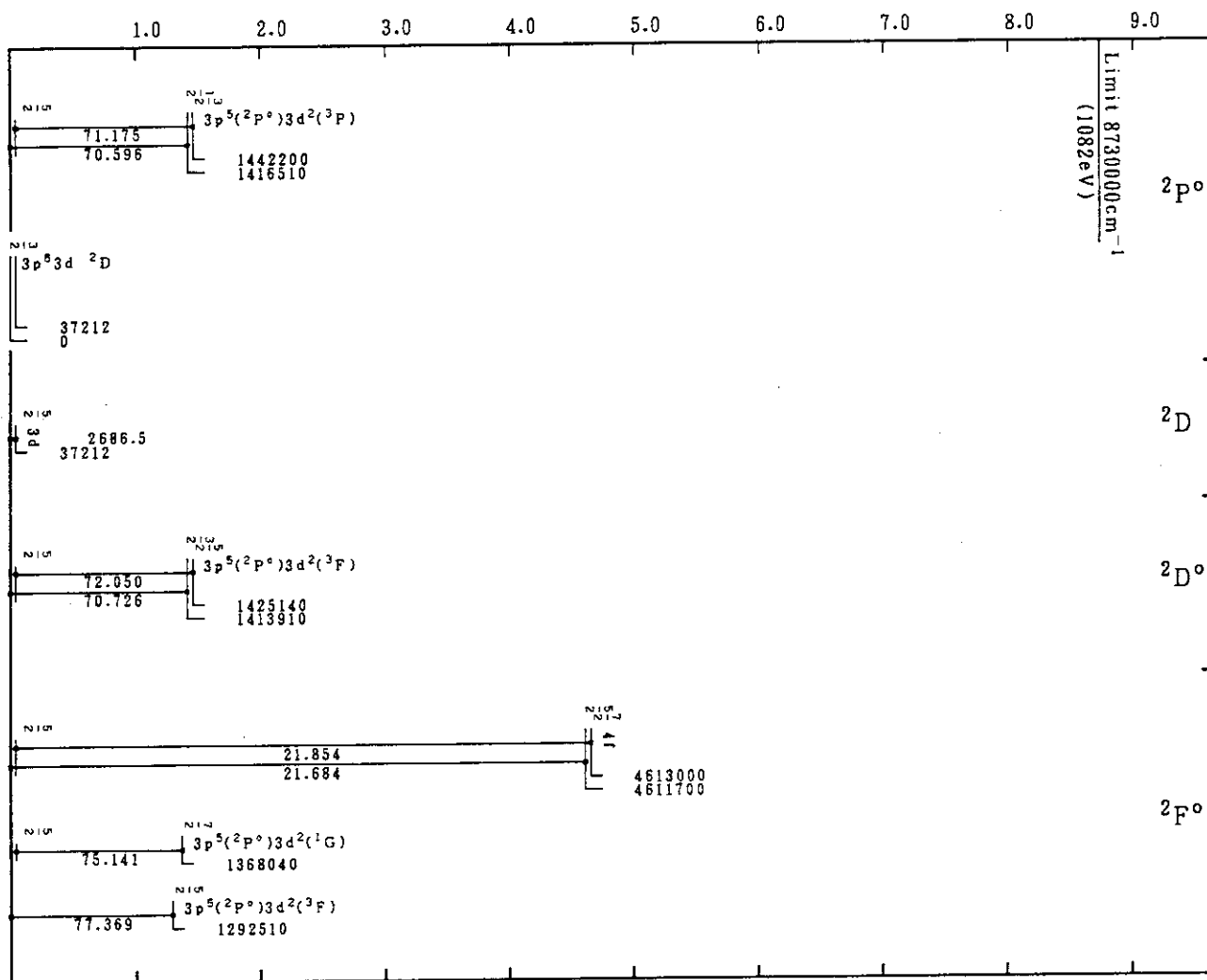
Mo XXIV(K-Sequence)
