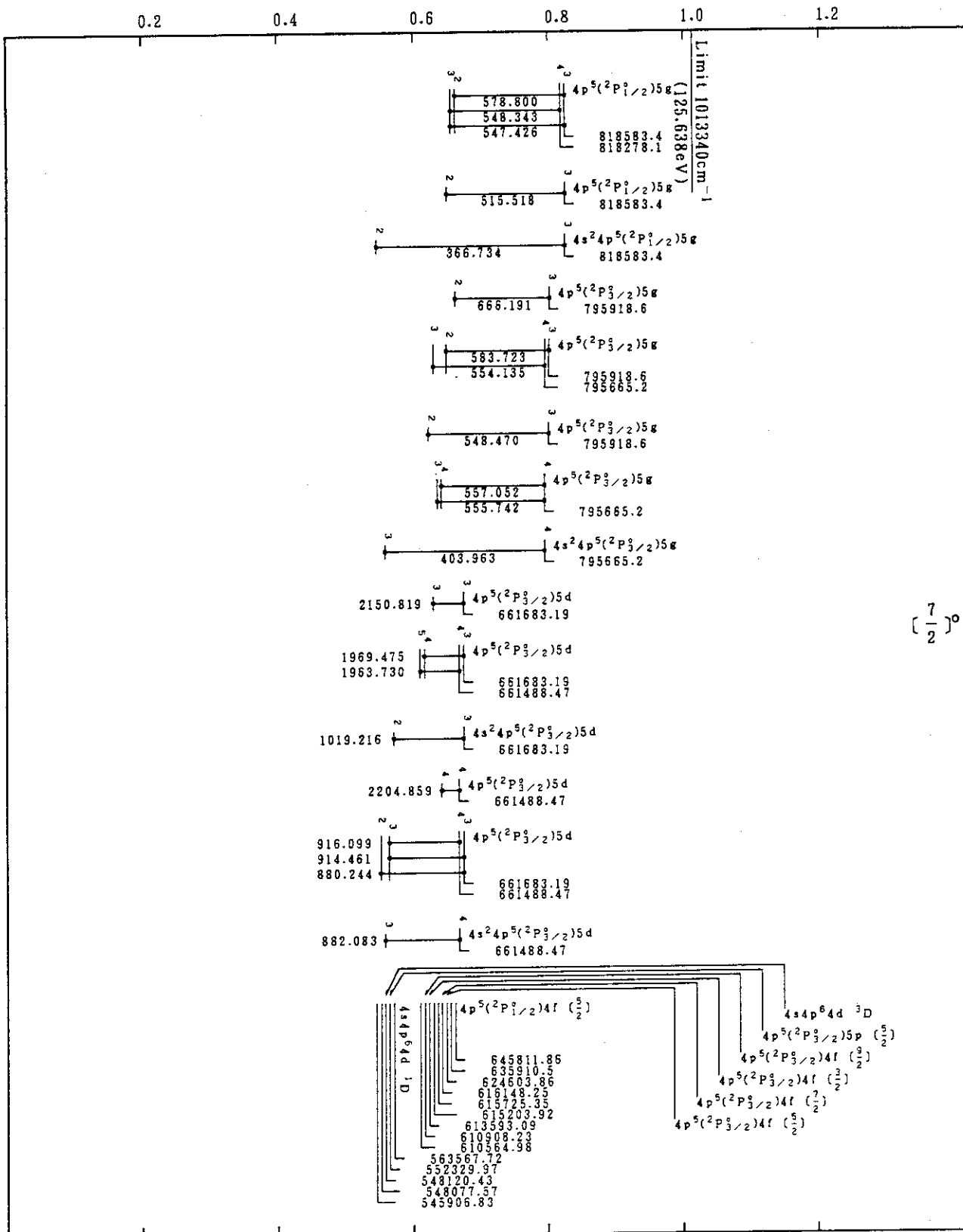
Mo VII(Kr-Sequence)
