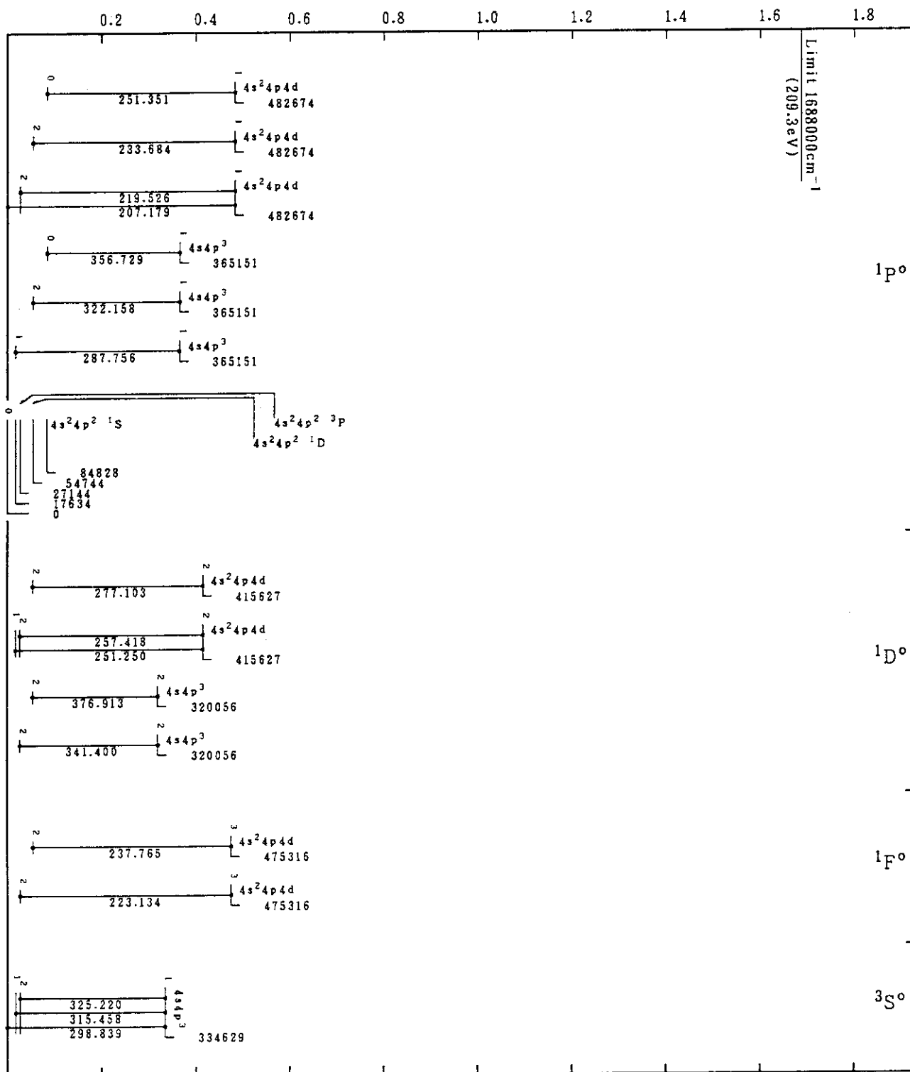
Mo XI(Ge-Sequence)
