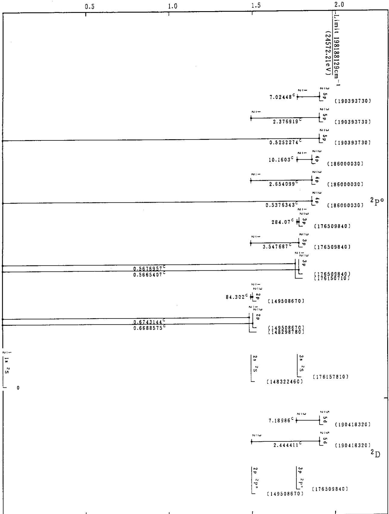
Mo XLII(H-Sequence)
