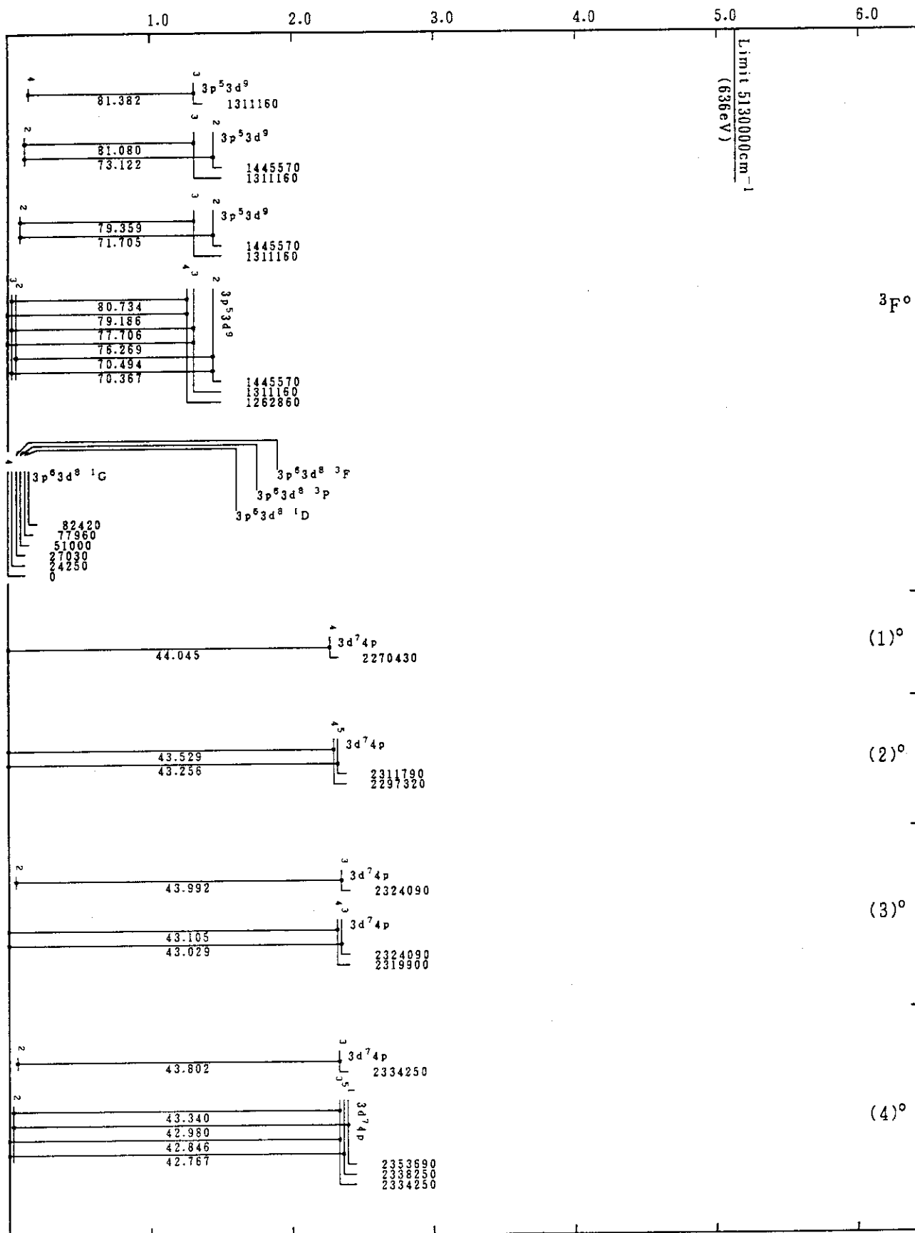
Mo XVII(Fe-Sequence)
