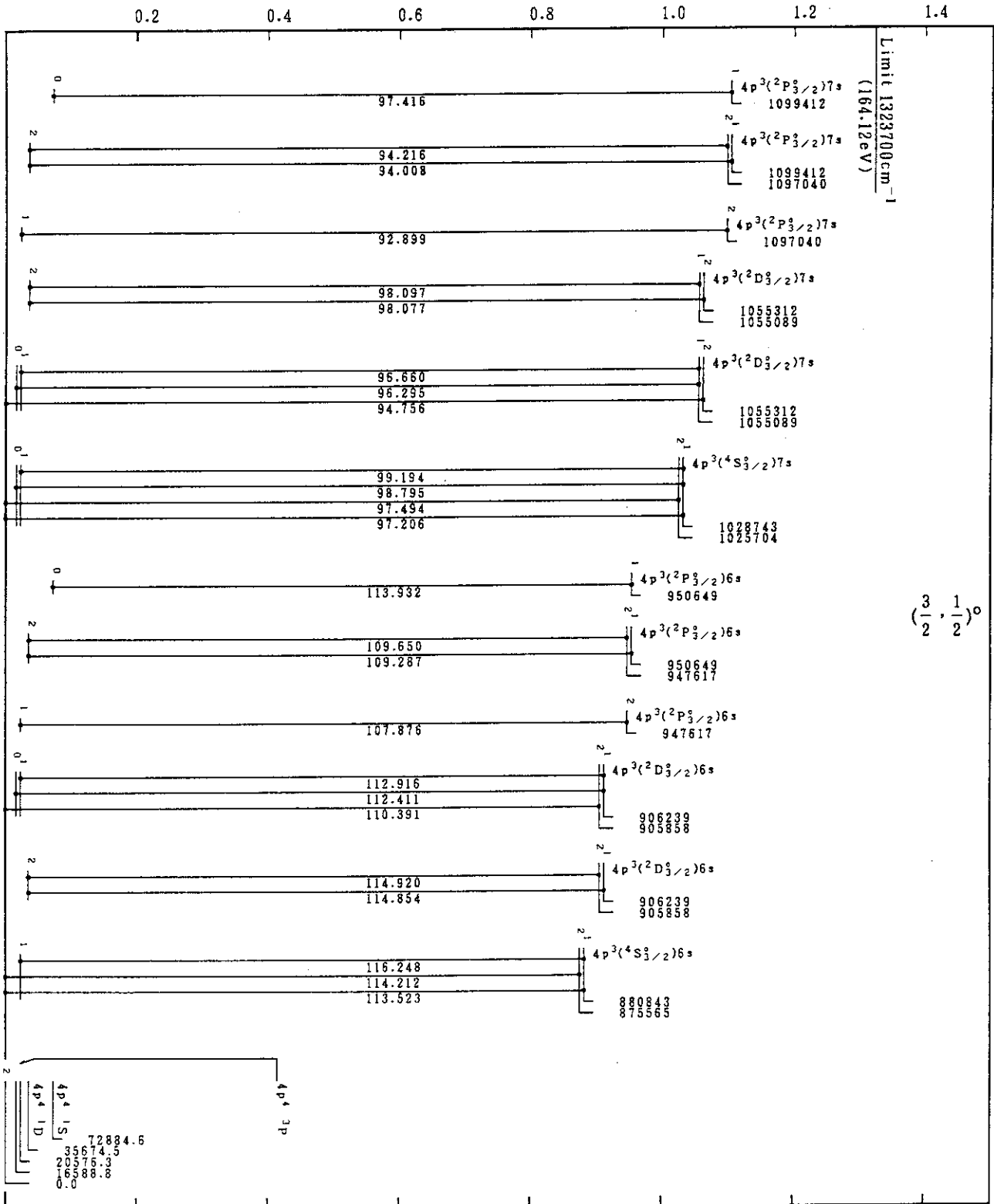
Mo IX(Se-Sequence)
