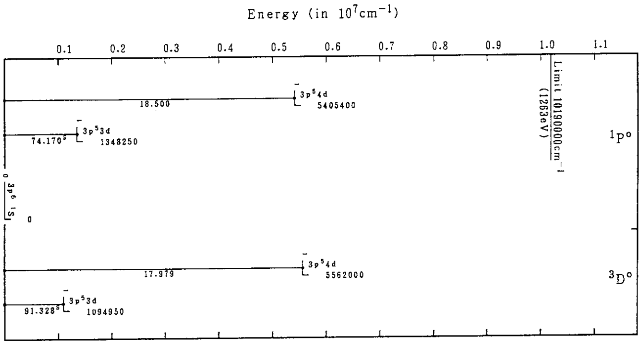
Mo XXV(Ar-Sequence)
