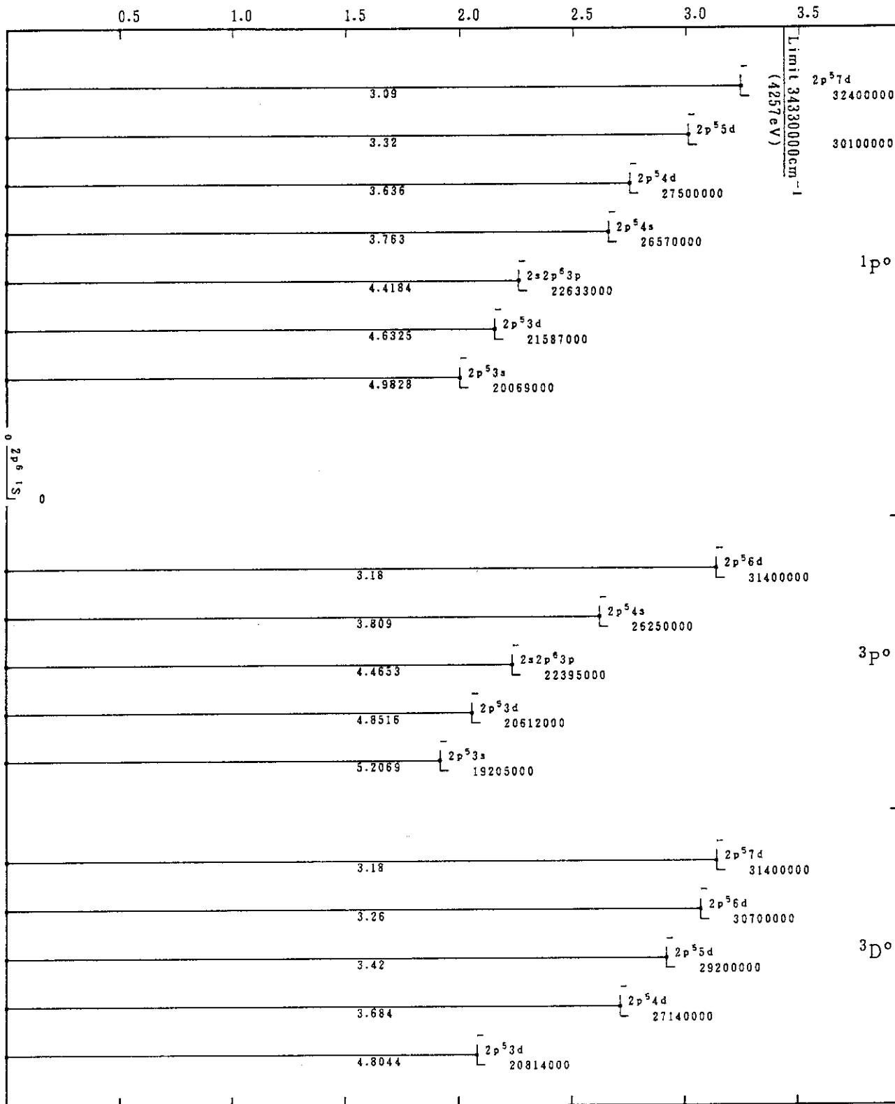
Mo XXXIII(Ne-Sequence)
