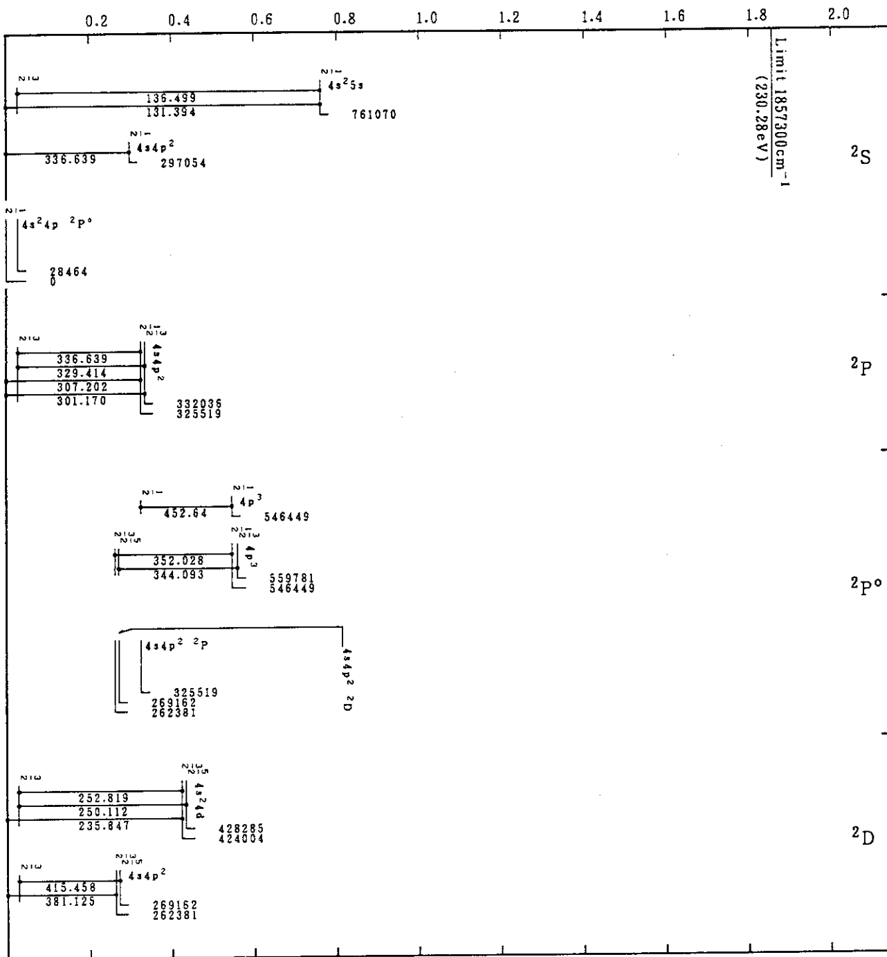
Mo XII(Ga-Sequence)
