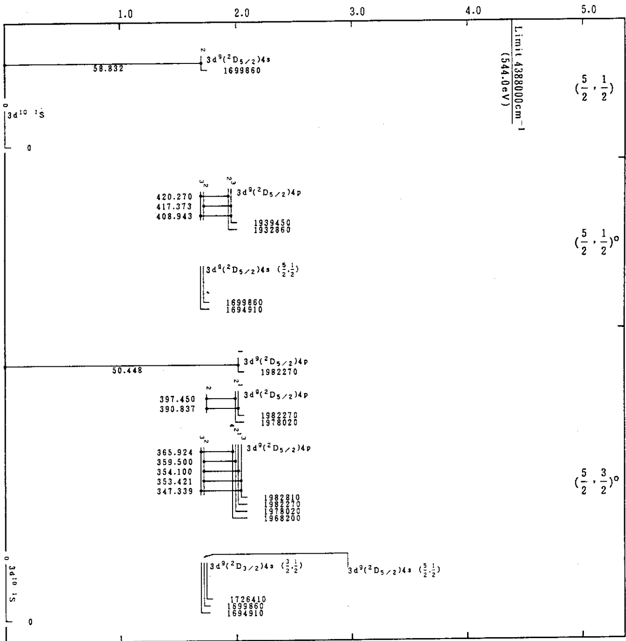
Mo XV(Ni-Sequence)
