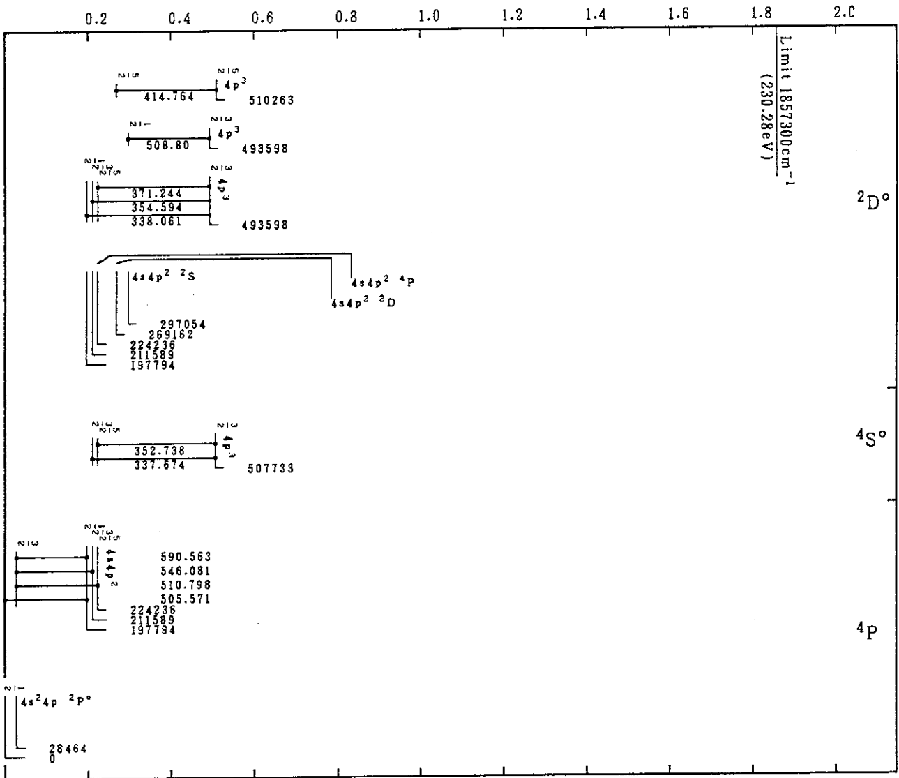
Mo XII(Ga-Sequence)
