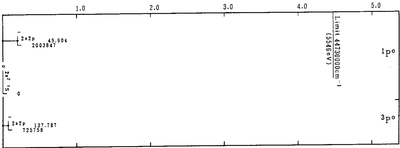
Mo XXXIX(Be-Sequence)
