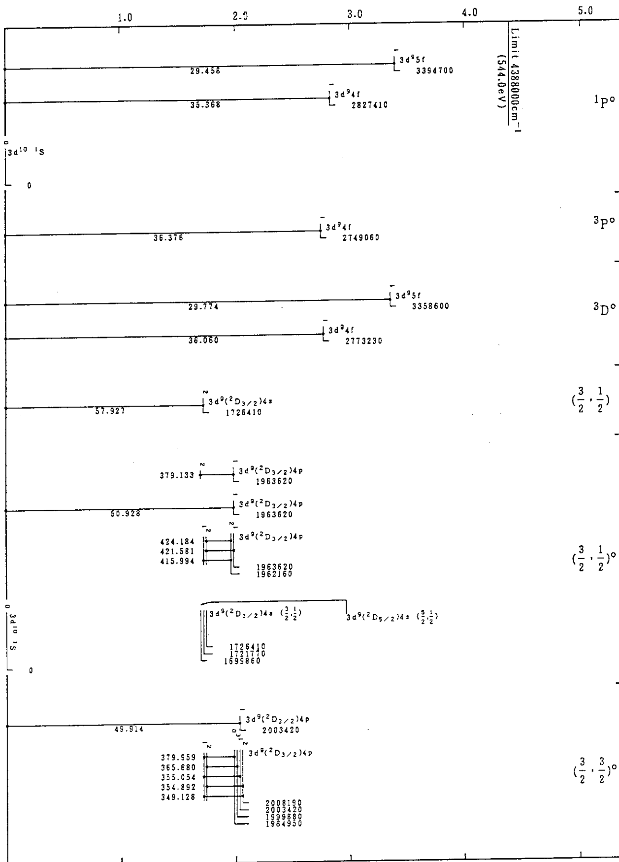
Mo XV(Ni-Sequence)
