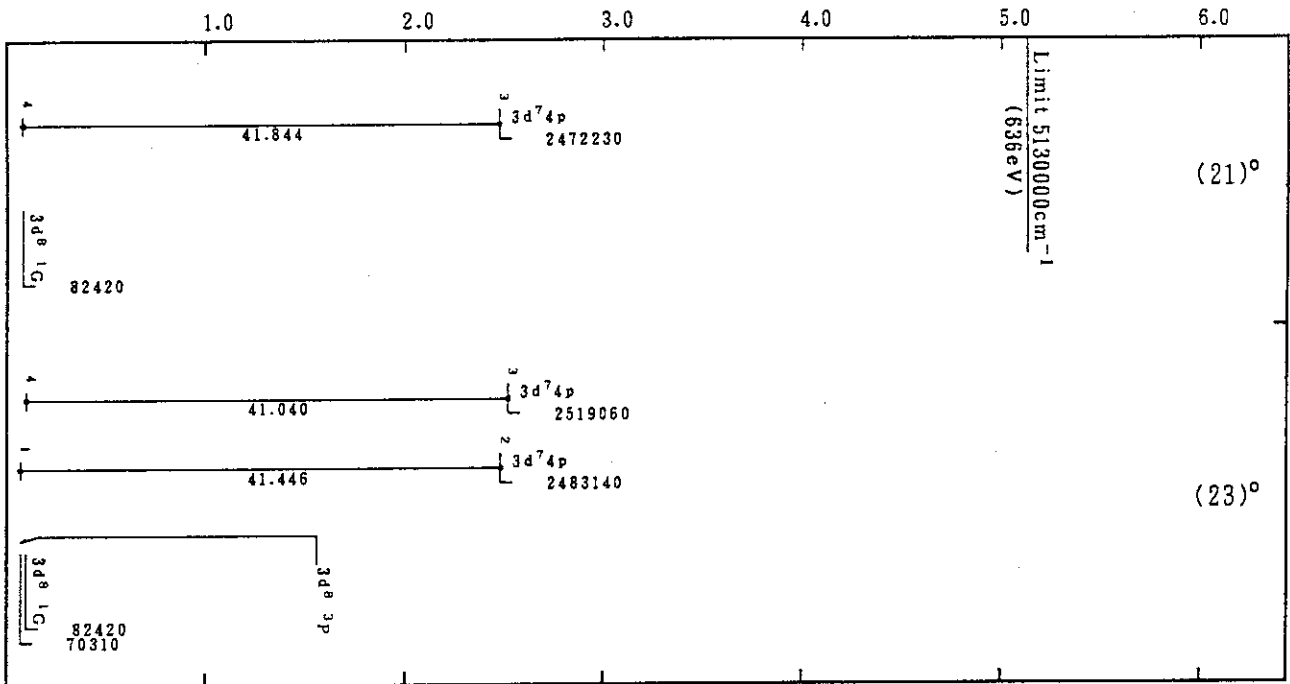
Mo XVII(Fe-Sequence)
