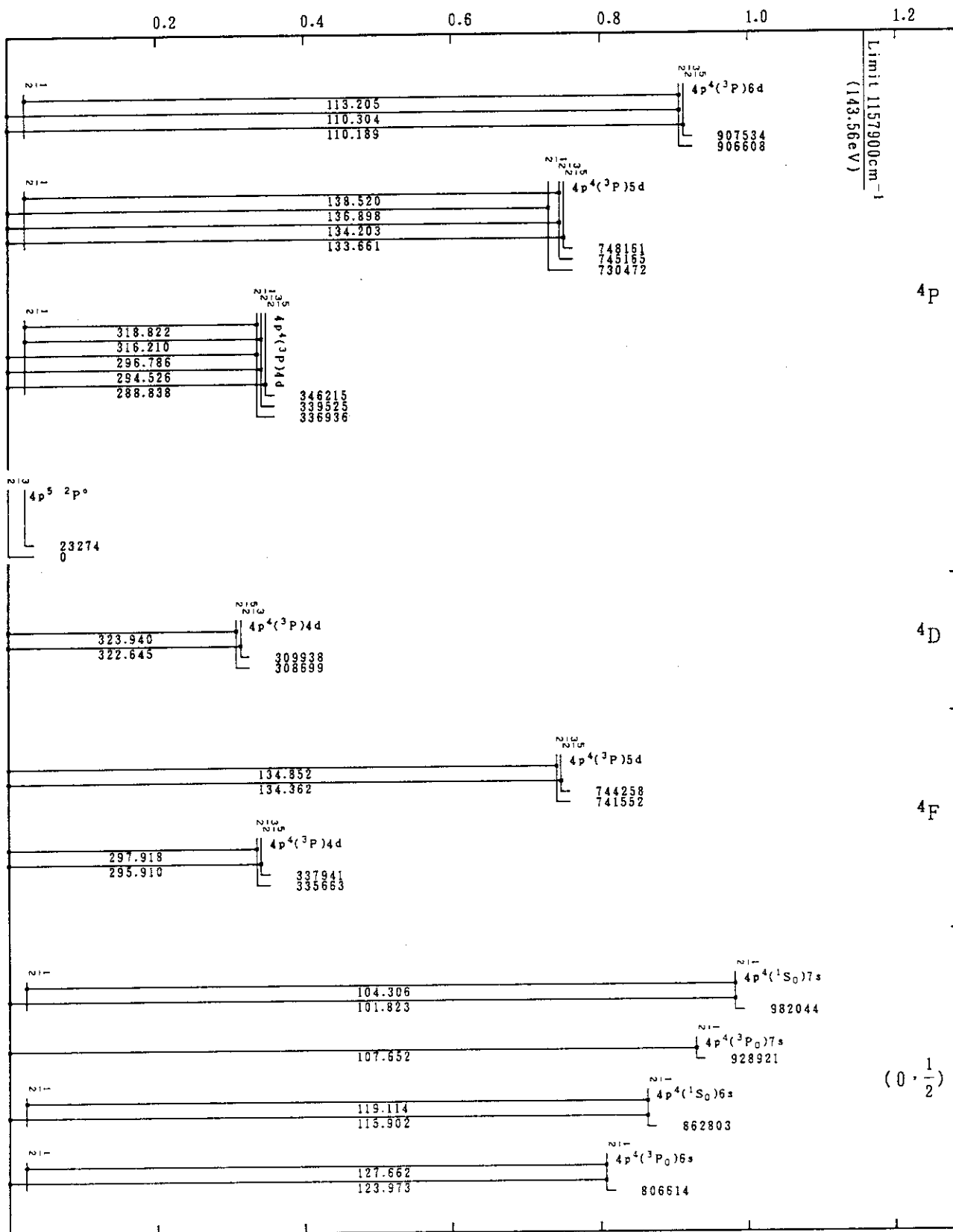
Mo VIII(Br-Sequence)
