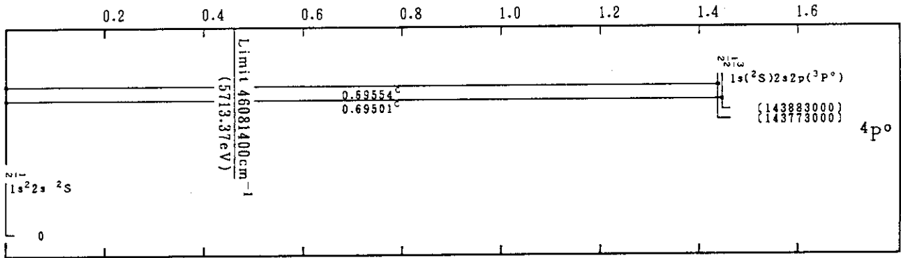
Mo XL(Li-Sequence)
