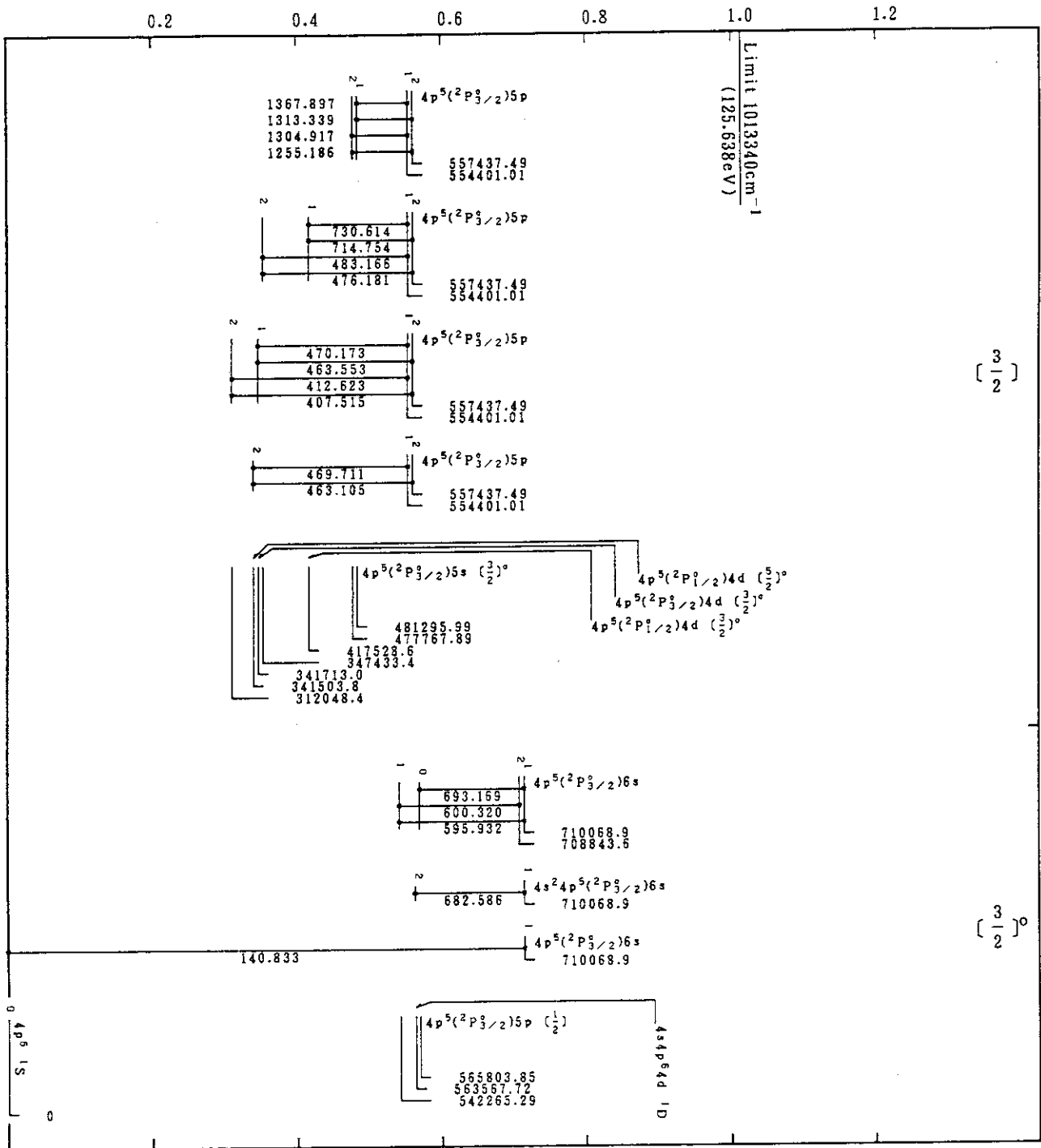
Mo VII(Kr-Sequence)
