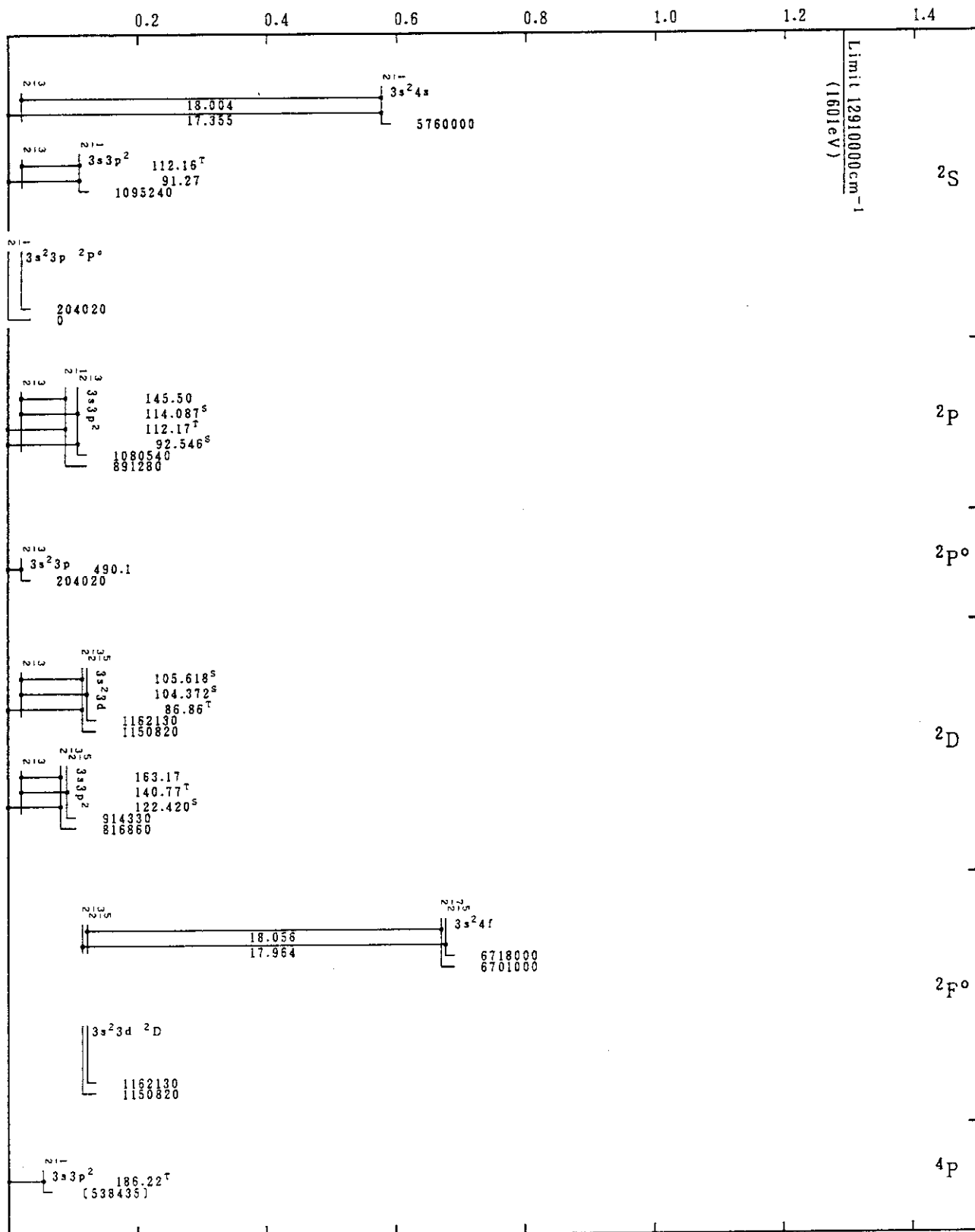
Mo XXX(AI-Sequence)
