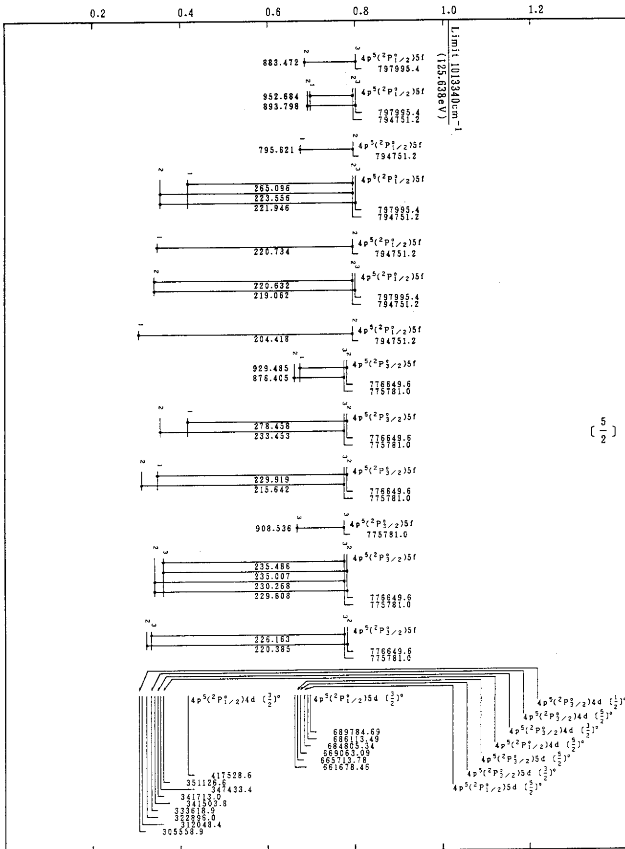
Mo VII(Kr-Sequence)
