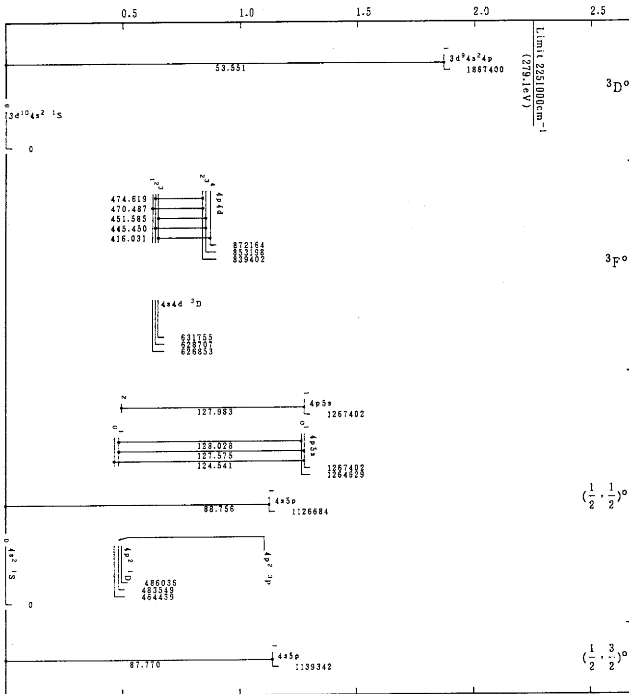
Mo XIII(Zn-Sequence)
