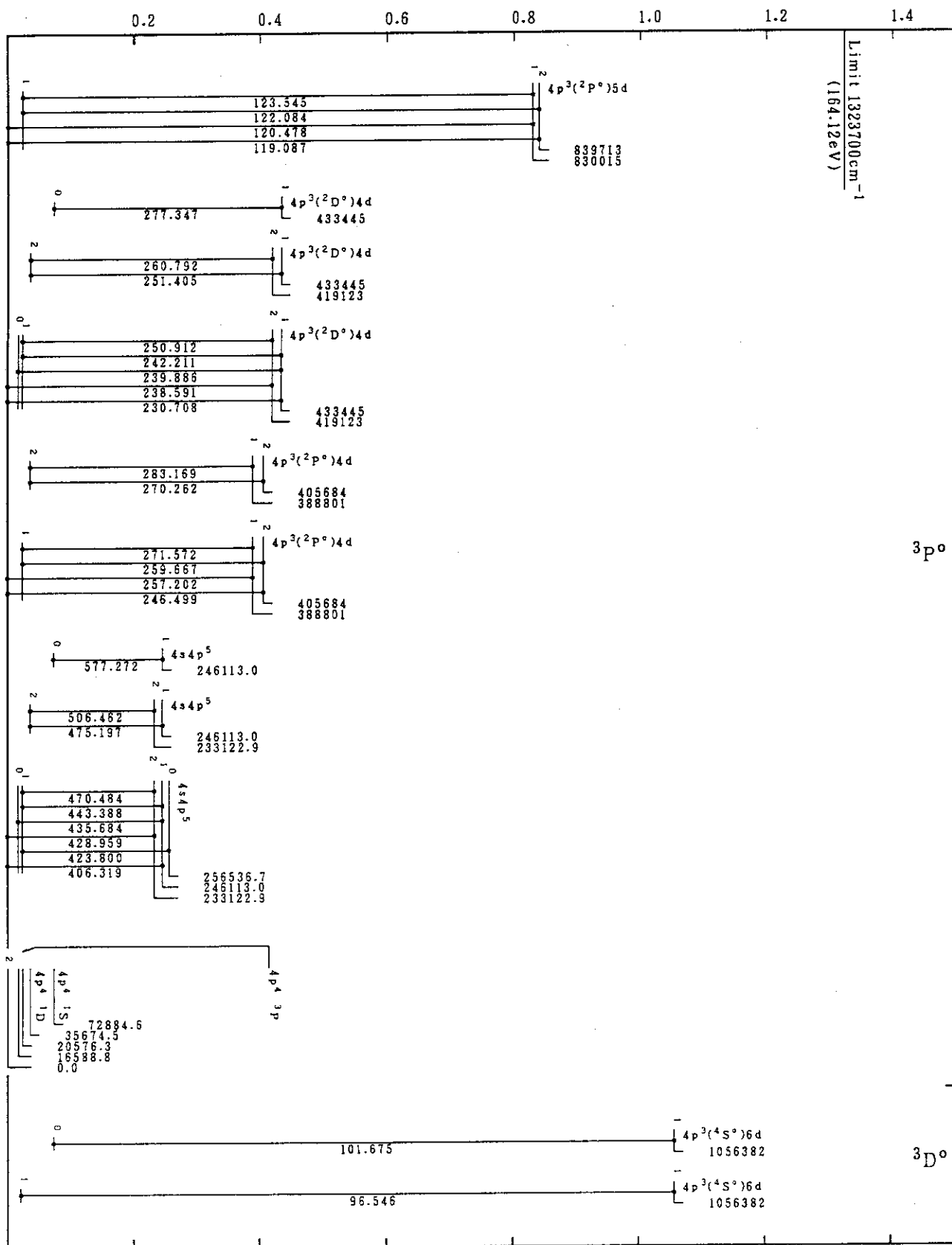
Mo IX(Se-Sequence)
