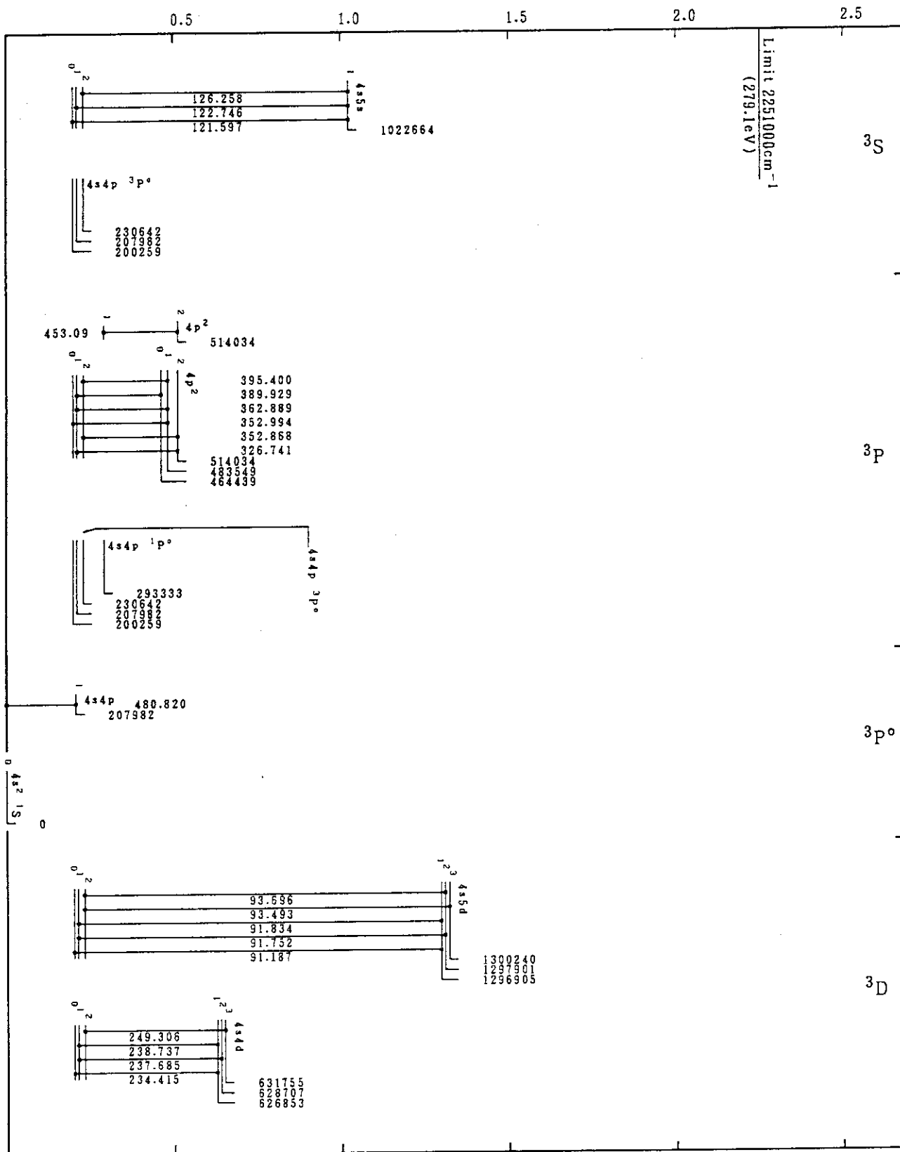
Mo XIII(Zn-Sequence)
