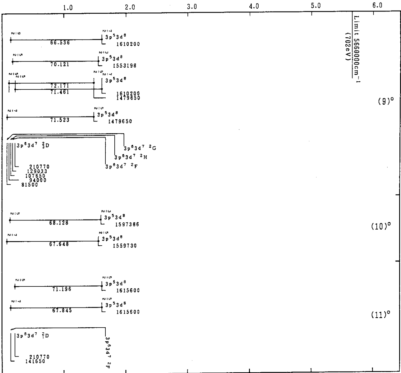
Mo XVIII(Mn-Sequence)
