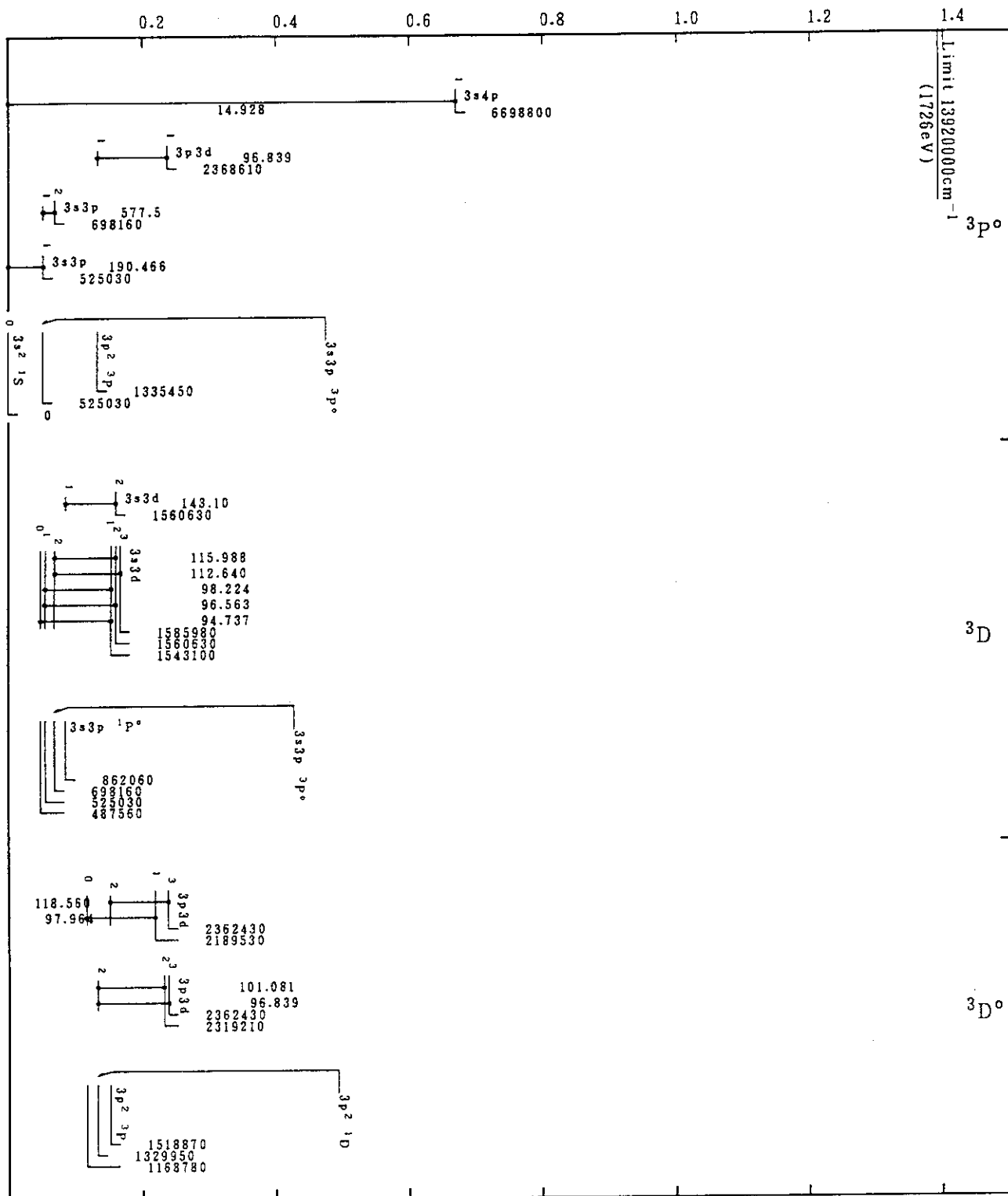
Mo XXXI(Mg-Sequence)
