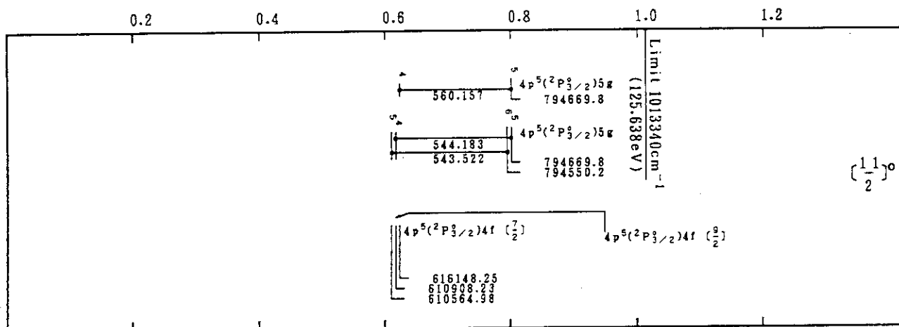
Mo VII(Kr-Sequence)
