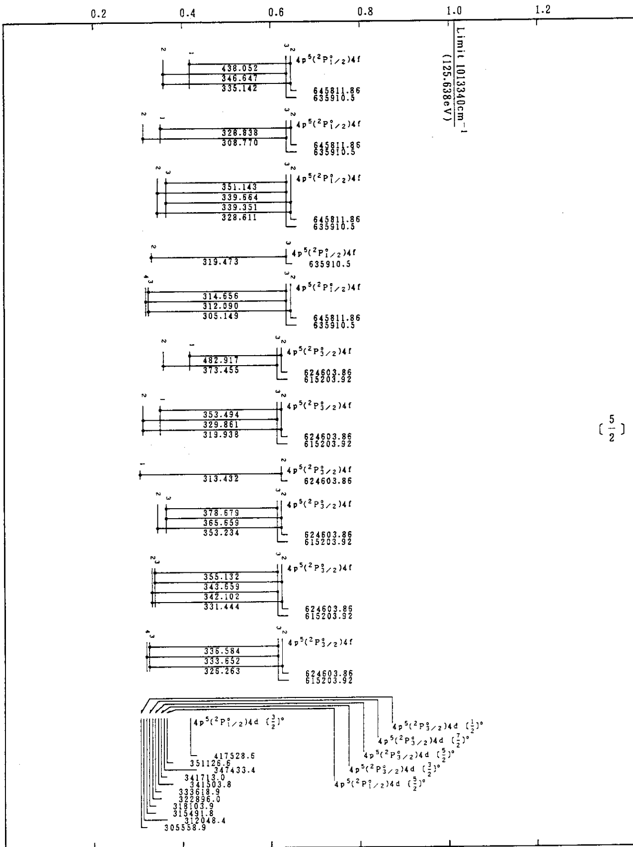
Mo VII(Kr-Sequence)
