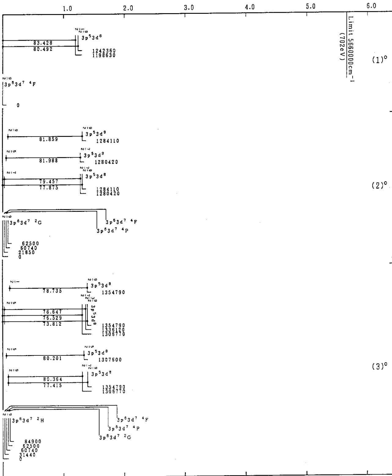
Mo XVIII(Mn-Sequence)
