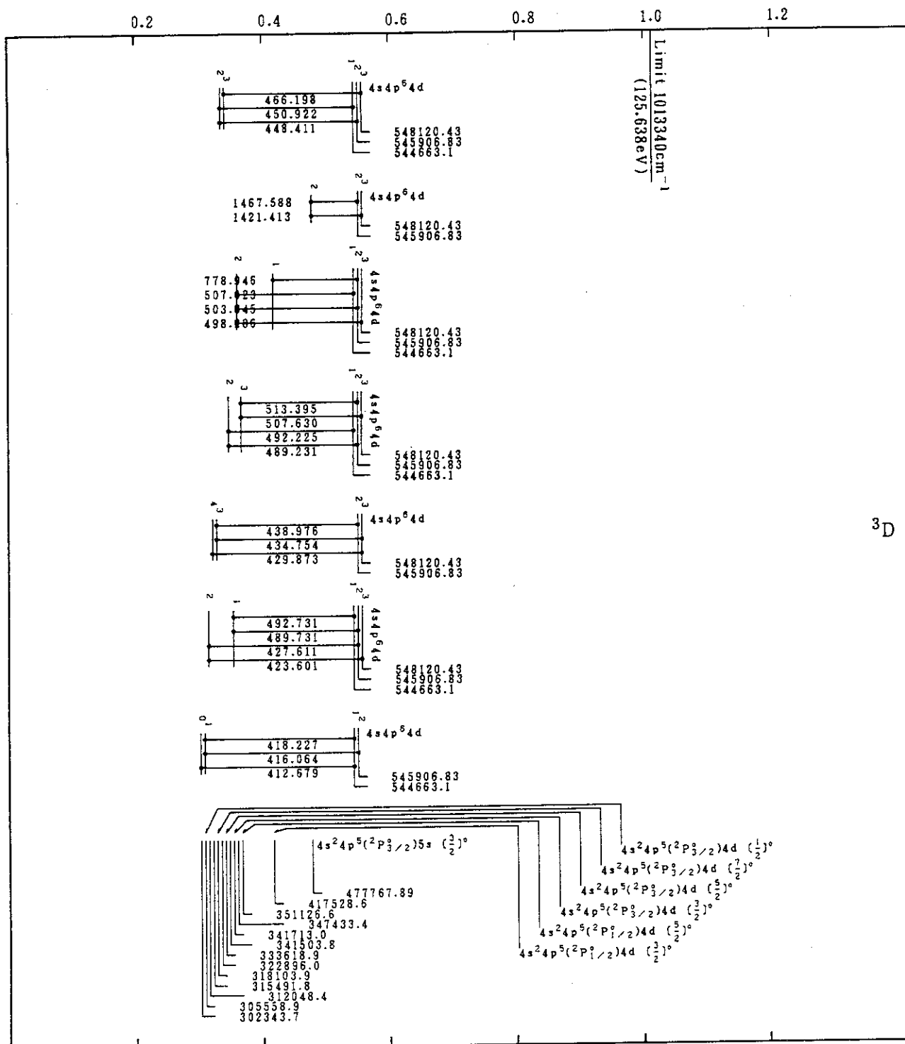
Mo VII(Kr-Sequence)
