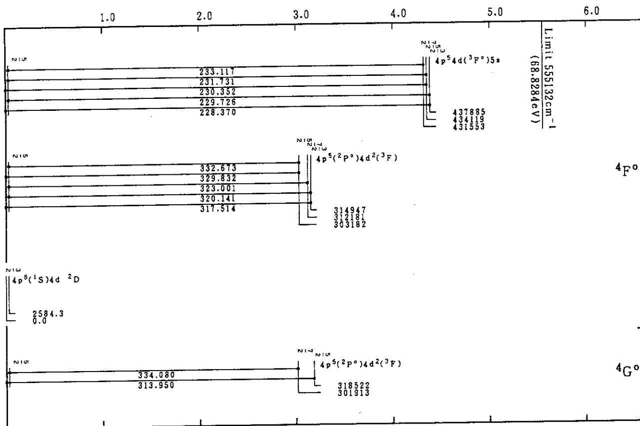
Mo VI(Rb-Sequence)
