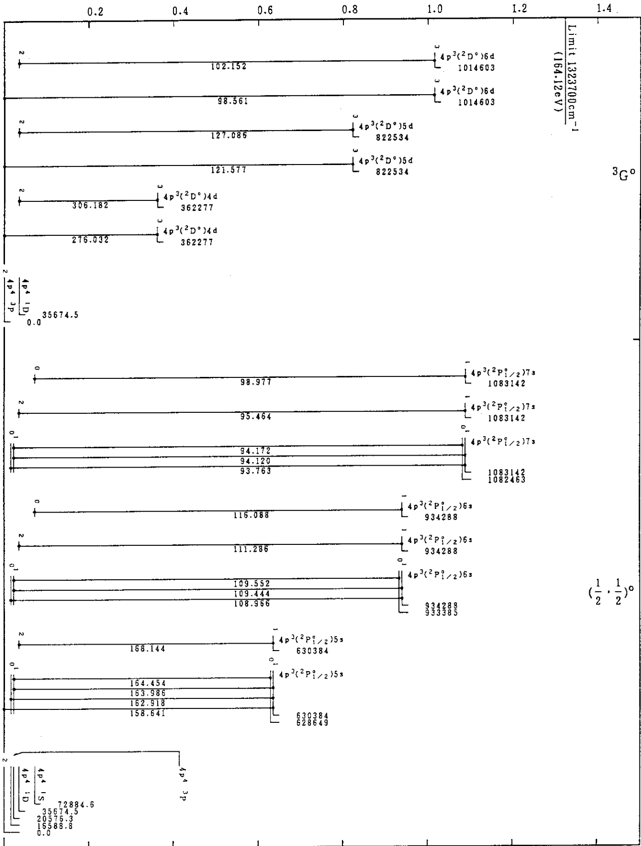
Mo IX(Se-Sequence)
