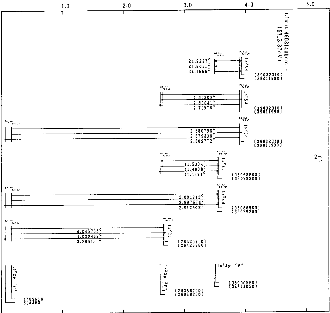
Mo XL(Li-Sequence)
