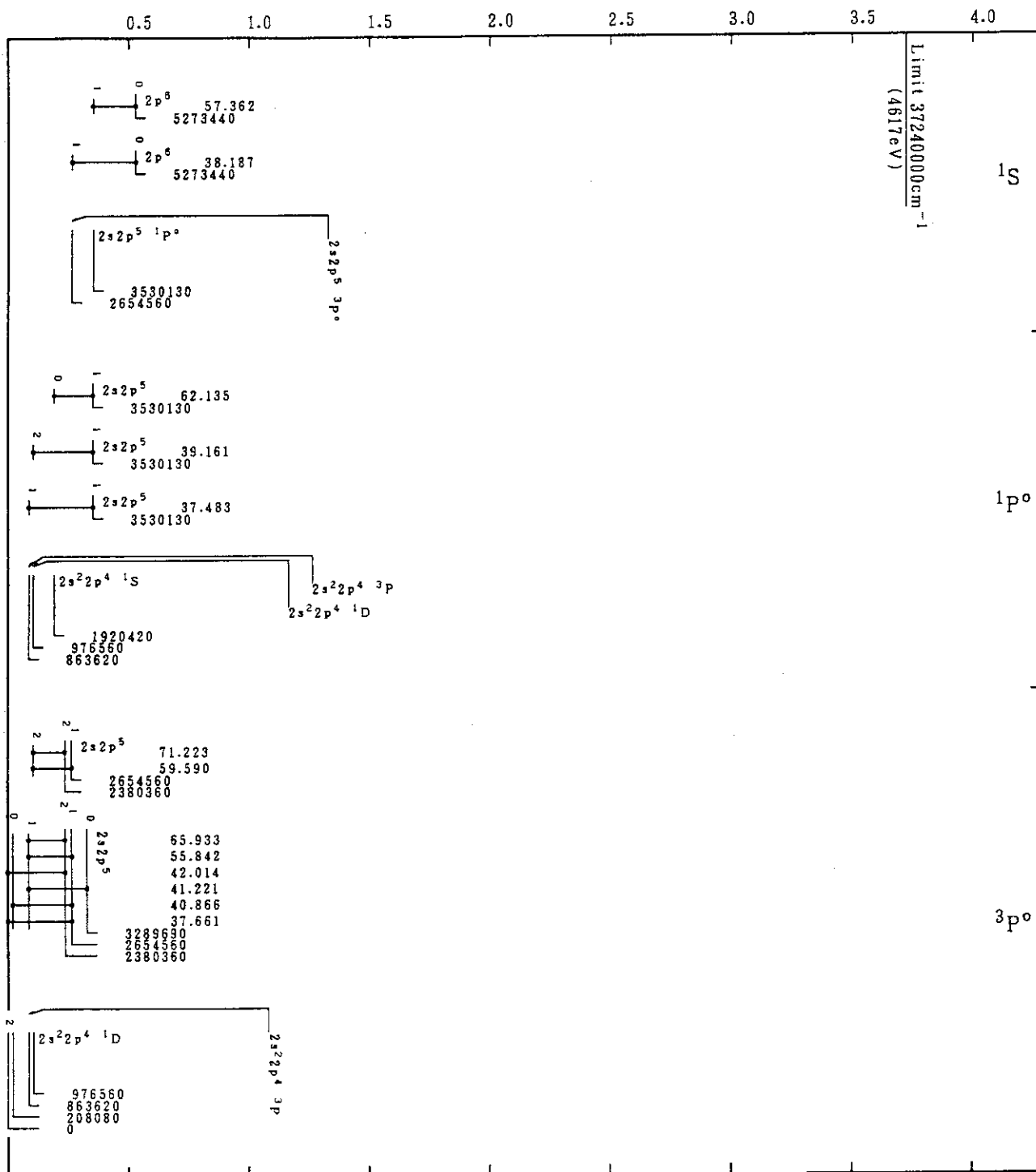
Mo XXXV(O-Sequence)
