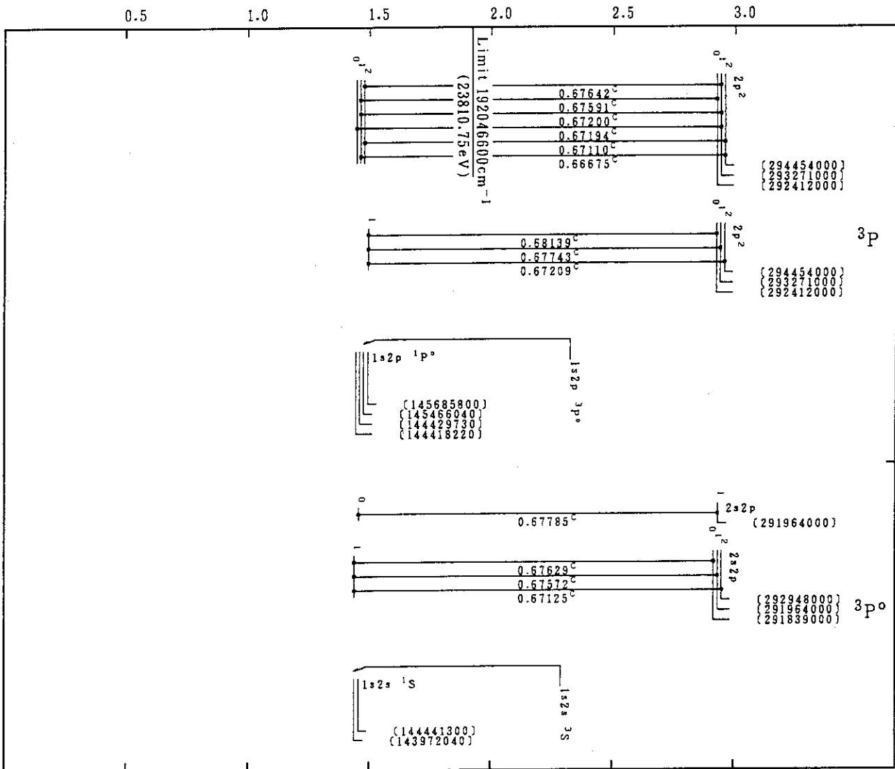
Mo XLI(He-Sequence)
