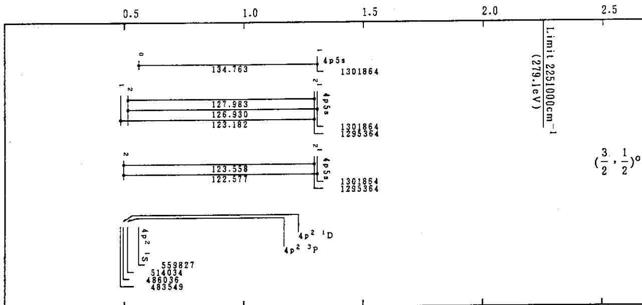
Mo XIII(Zn-Sequence)
