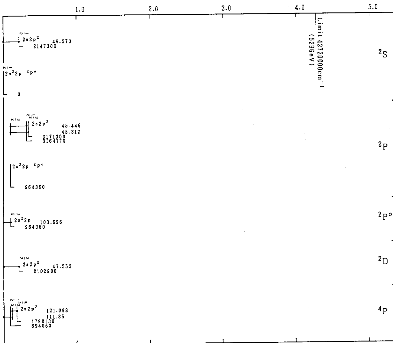
Mo XXXVIII(B-Sequence)
