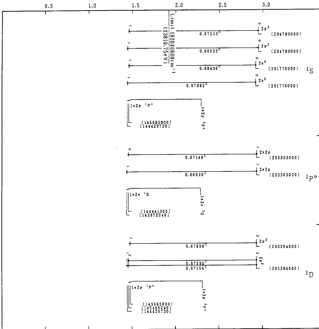
Mo XLI(He-Sequence)
