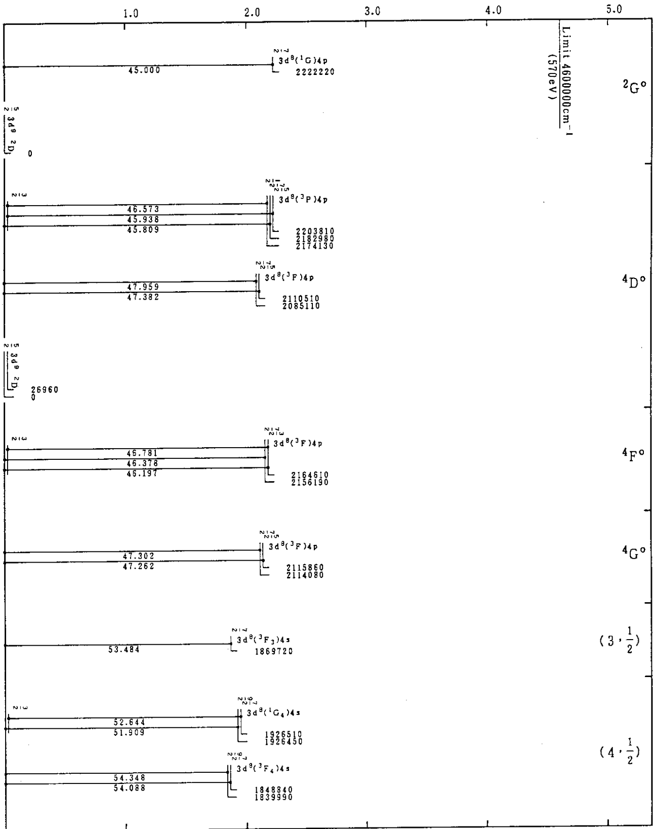
Mo XVI(Co-Sequence)
