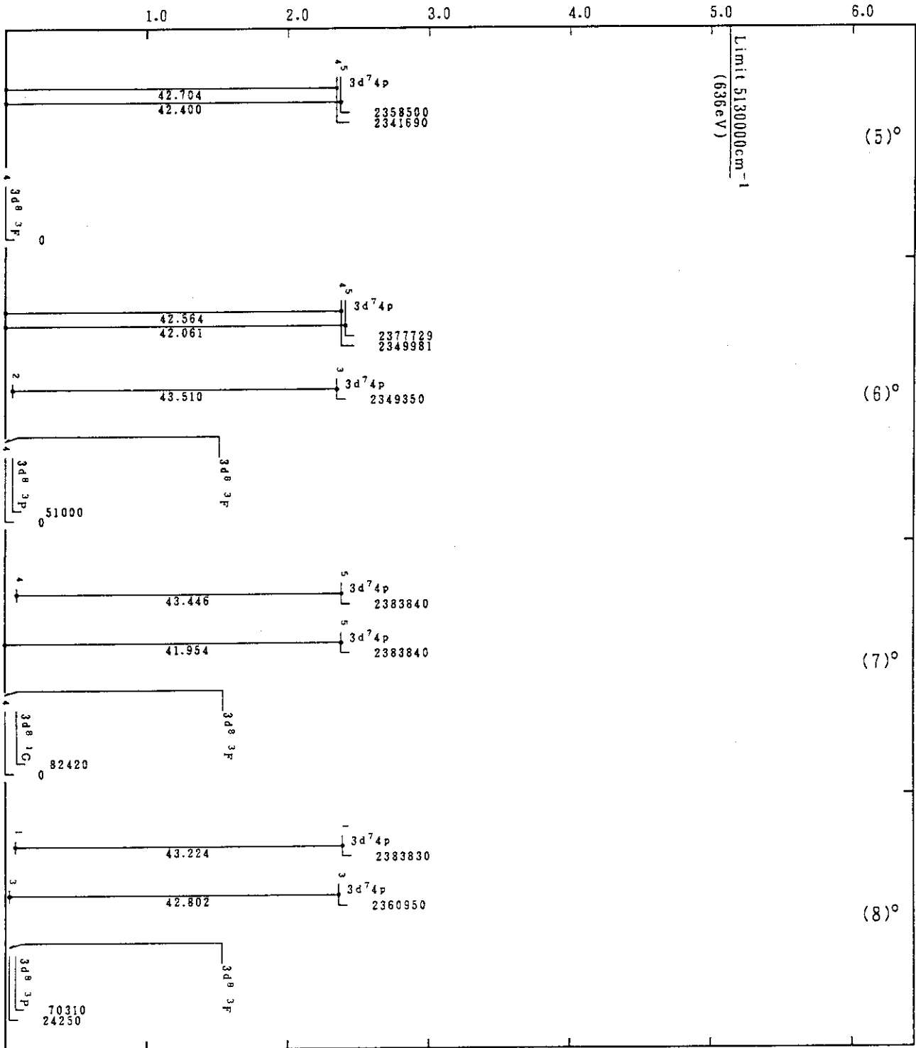
Mo XVII(Fe-Sequence)
