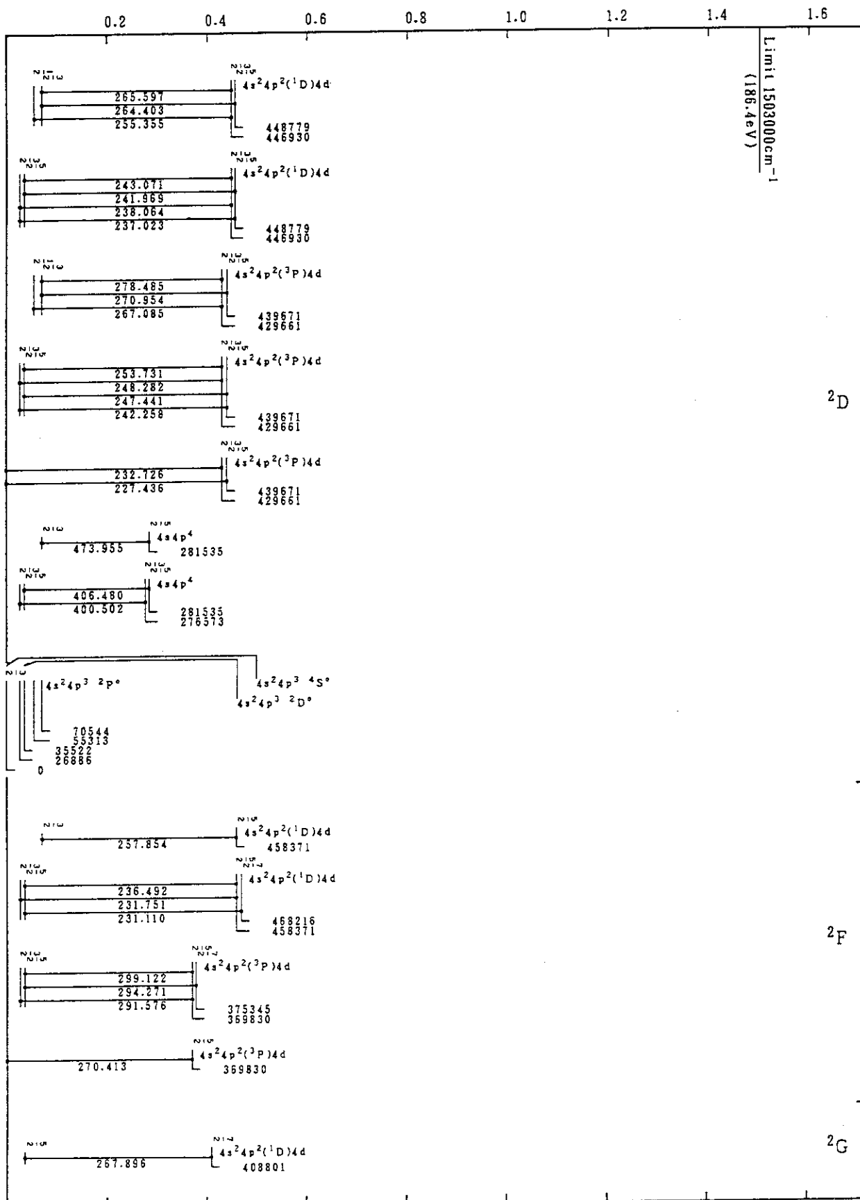
Mo X(As-Sequence)
