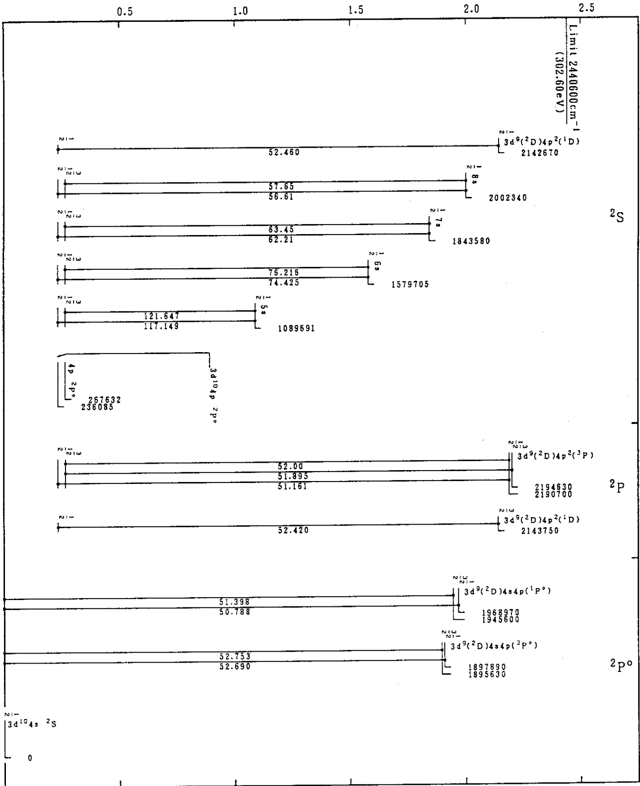
Mo XIV(Cu-Sequence)
