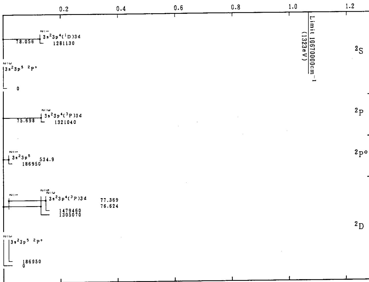
Mo XXVI(Cl-Sequence)
