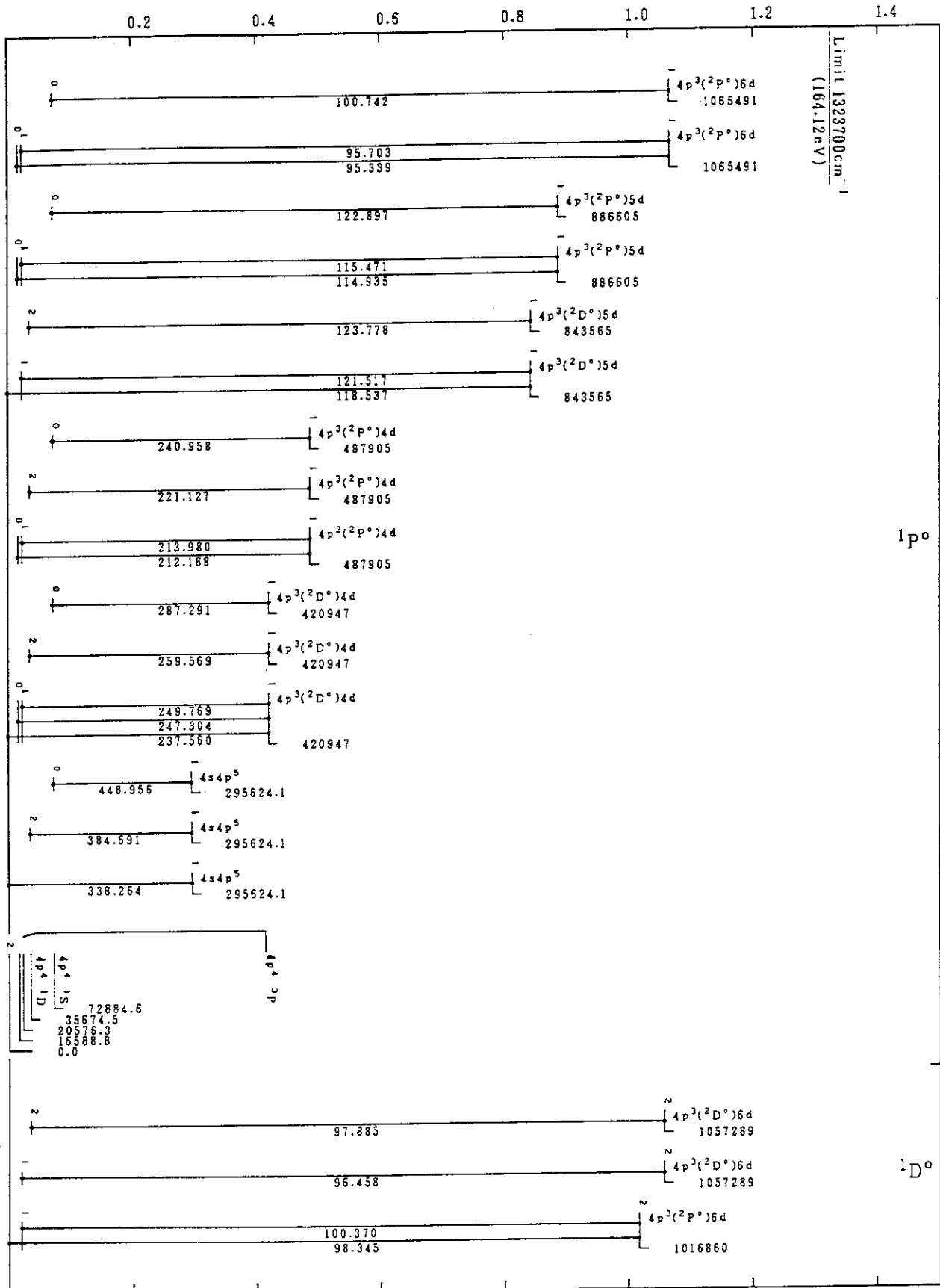
Mo IX(Se-Sequence)
