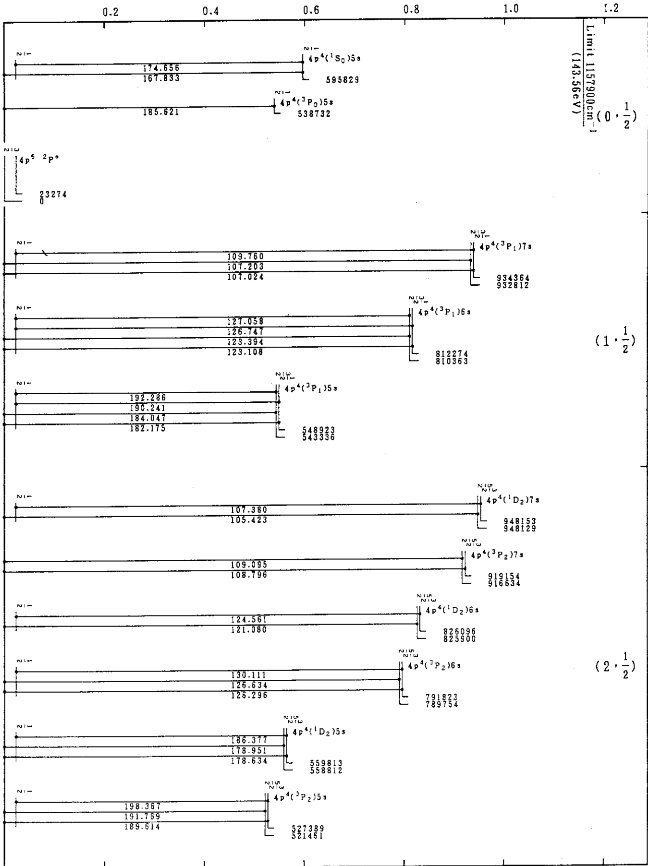
Mo VIII(Br-Sequence)
