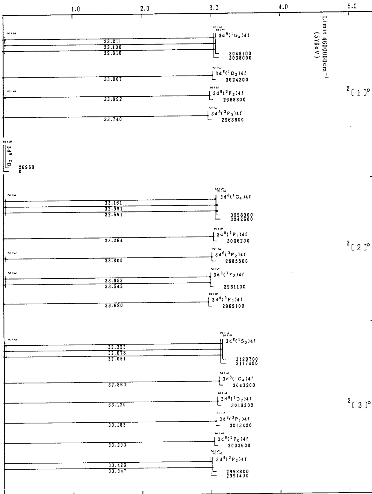
Mo XVI(Co-Sequence)
