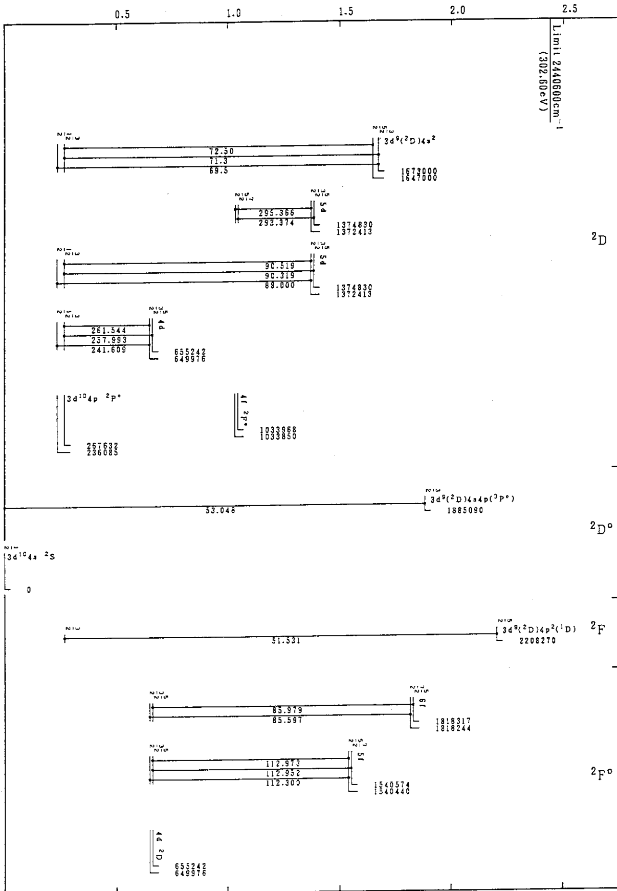
Mo XIV(Cu-Sequence)
