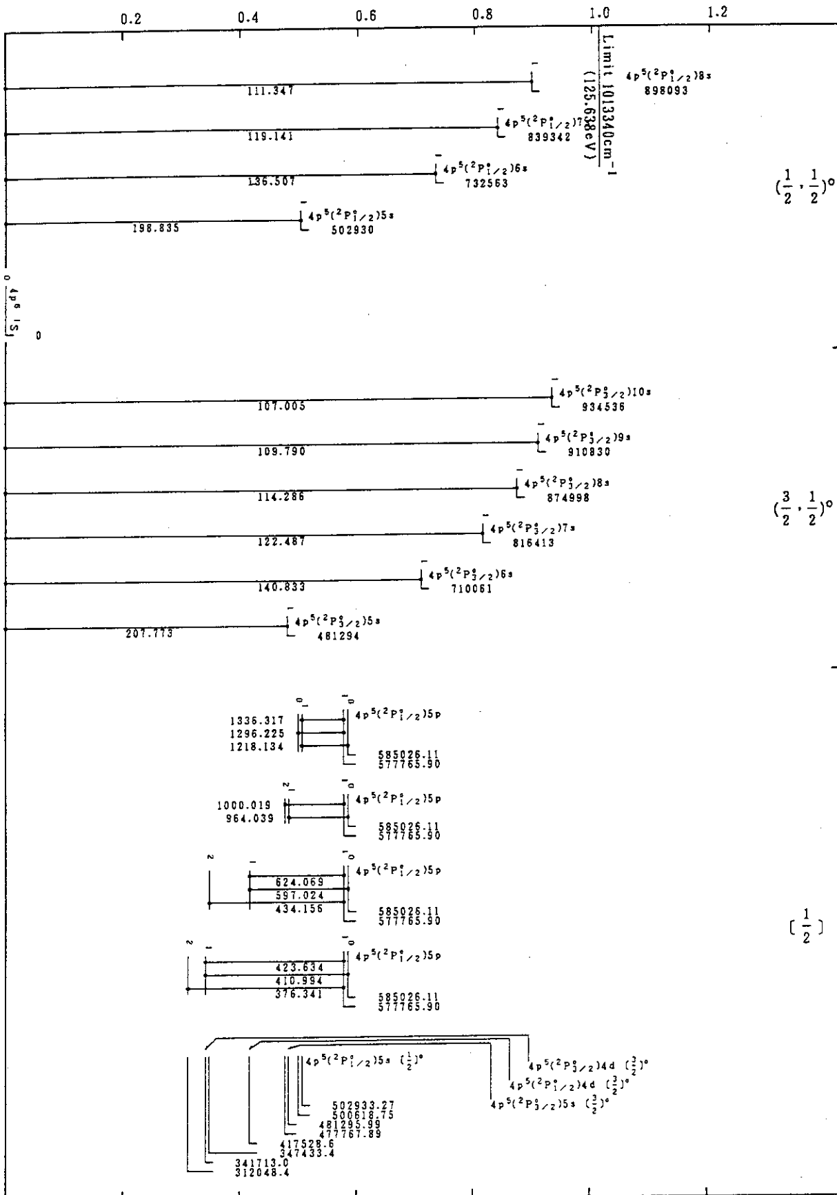
Mo VII(Kr-Sequence)
