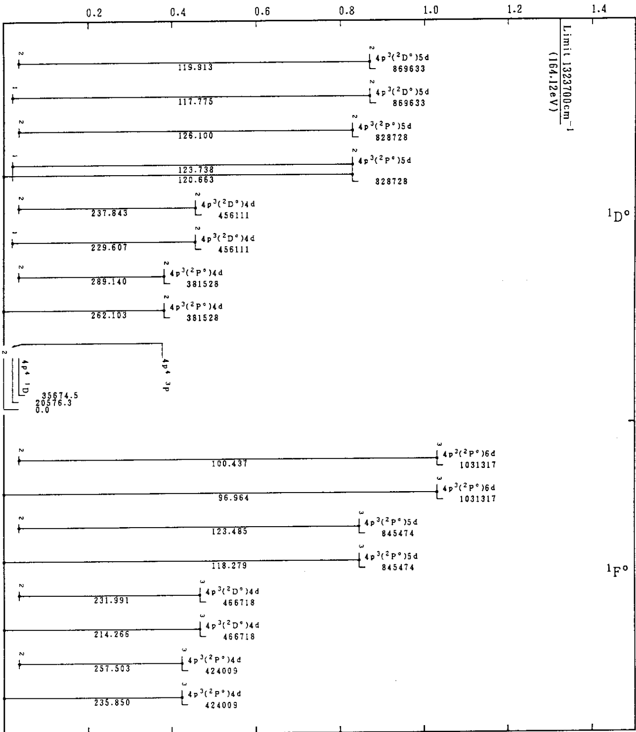
Mo IX(Se-Sequence)
