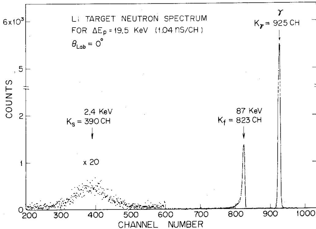
Fig. 11 Time-of-flight spectrum.
