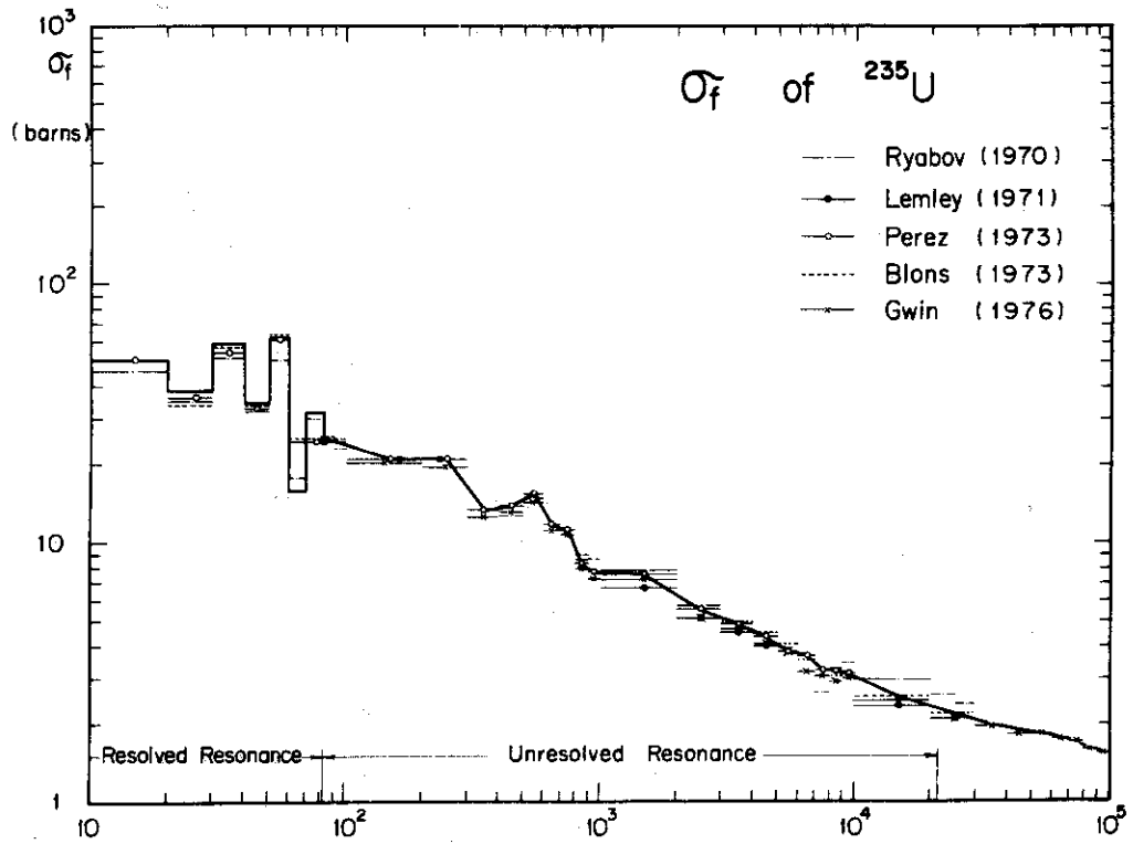
2.1.1. Fission cross section of ^{235}\text{U} in unresolved resonance region
