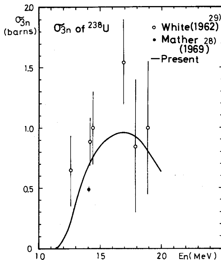
1.2.5 (n,3n) cross section of ^{238}\text{U} .
