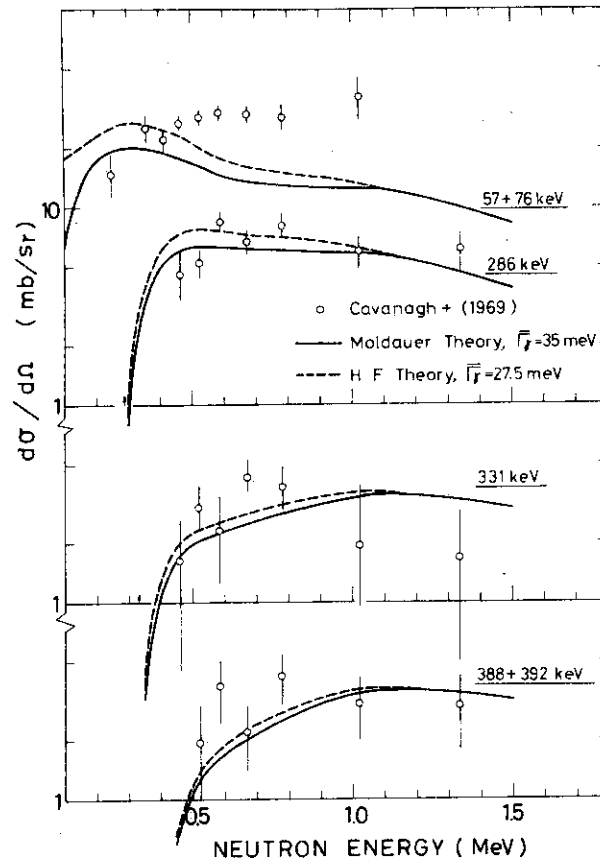
1.3.7. Partial inelastic scattering cross section of ^{239}\text{Pu} measured at 90^\circ
