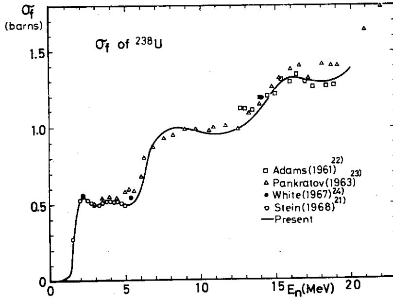
1.2.3 Fission cross sections of ^{238}\text{U} .
