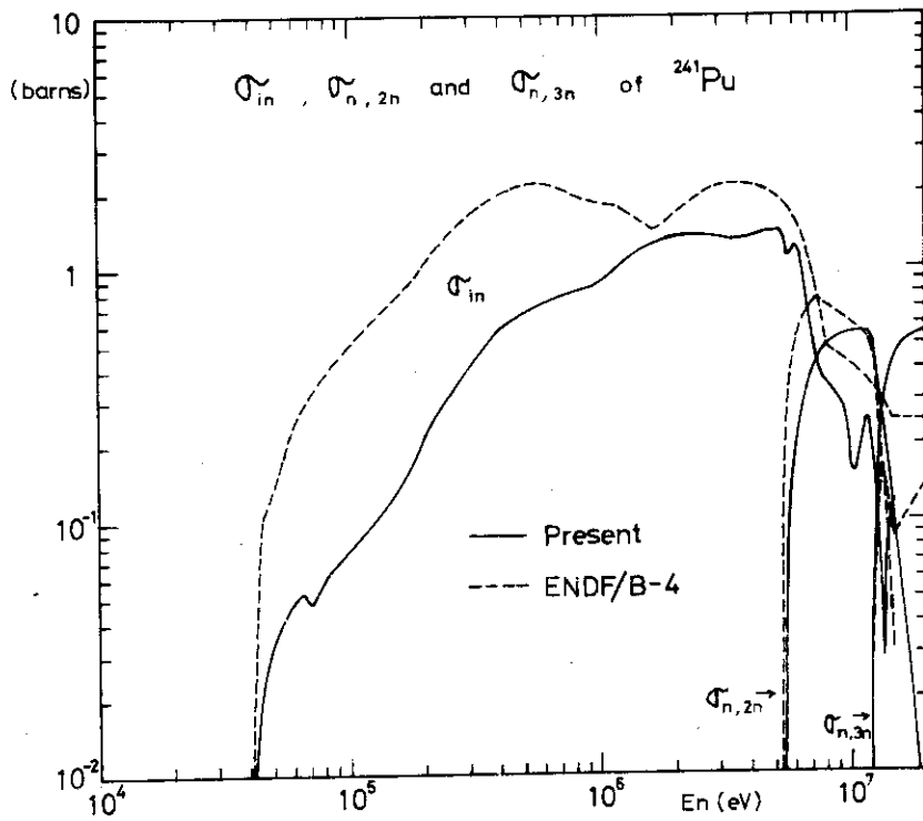
1.5.5. Inelastic scattering, (n,2n) and (n,3n) cross sections of ^{241}\text{Pu}
