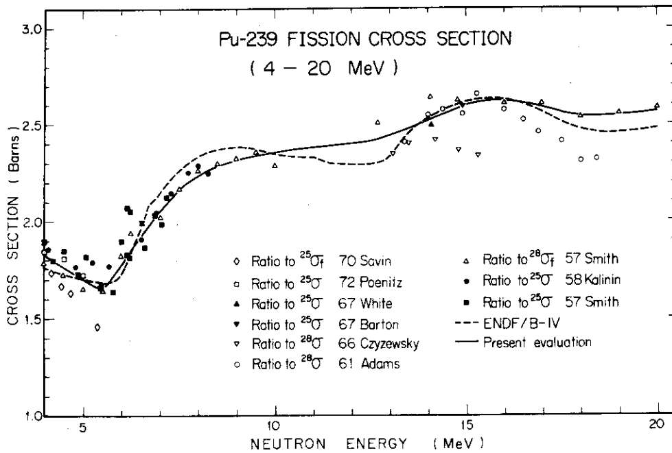
1.3.3. Fission cross section of ^{239}\text{Pu} from 4 MeV to 20 MeV
