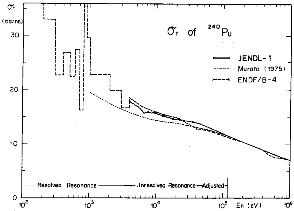
2.4.1. Total cross section of ^{240}\text{Pu}
