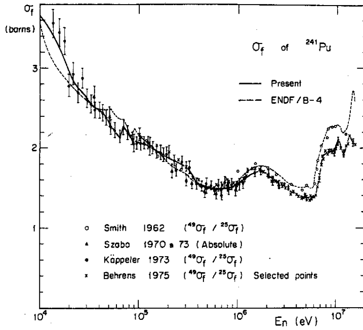
1.5.2. Fission cross section of ^{241}\text{Pu}
