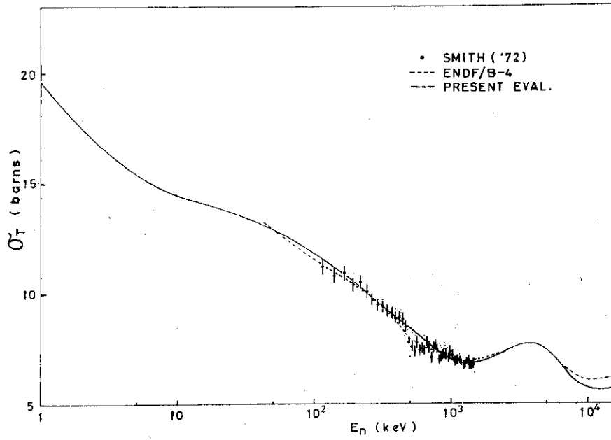
Fig. 1.4.1. Total cross section of ^{240}\text{Pu}
