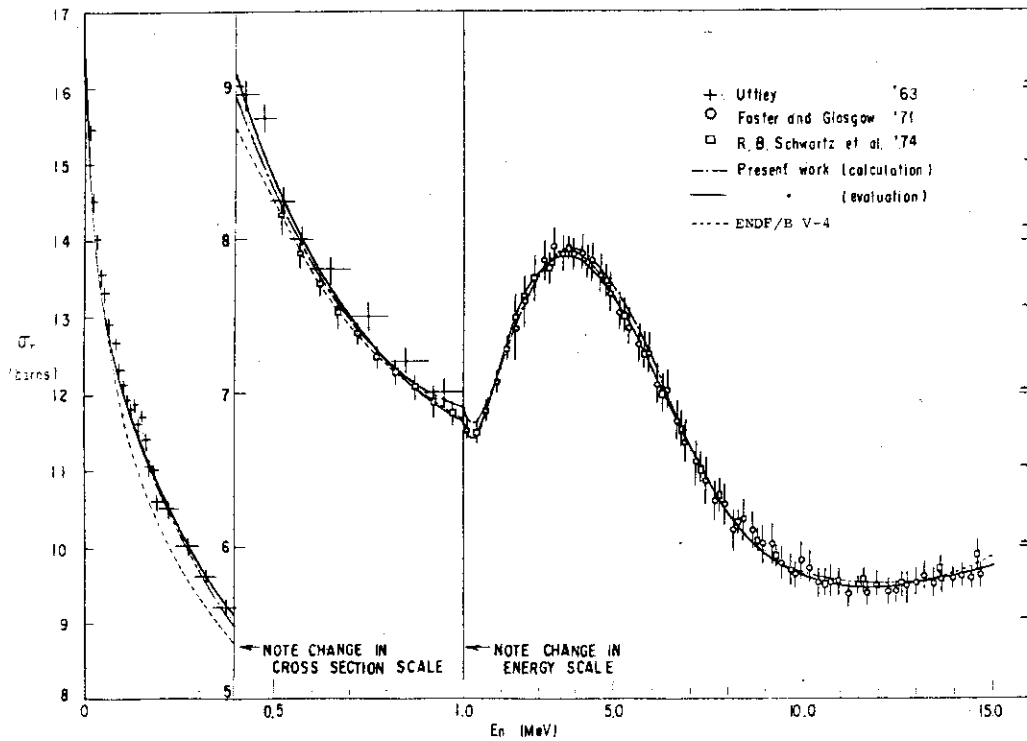
1.1.1. Total cross section of ^{235}\text{U}
