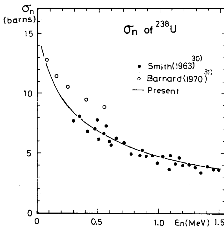
1.2.6 Elastic scattering cross sections of ^{238}\text{U} below 1.5 MeV.
