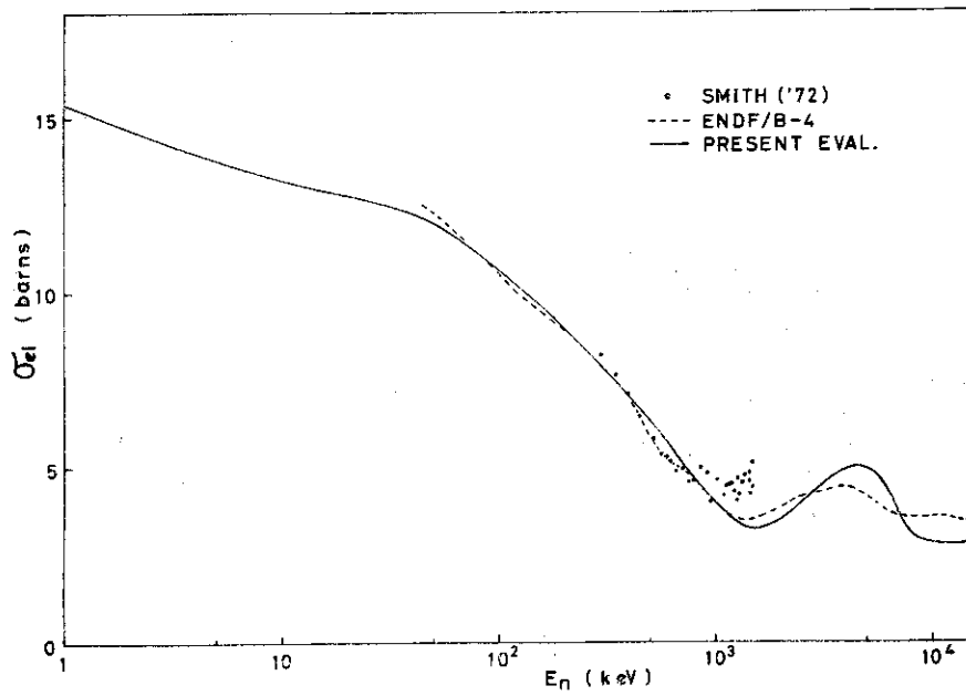
Fig. 1.4.2. Elastic scattering cross section of ^{240}\text{Pu}
