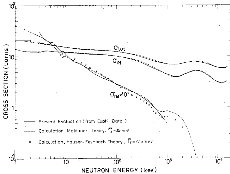
1.3.5. Comparison of present evaluation with statistical calculations for total, elastic scattering and capture cross sections of ^{239}\text{Pu}
