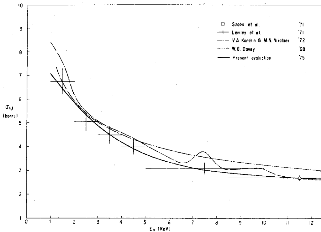
1.1.2. Fission cross section of ^{235}\text{U} from 1 to 12 keV
