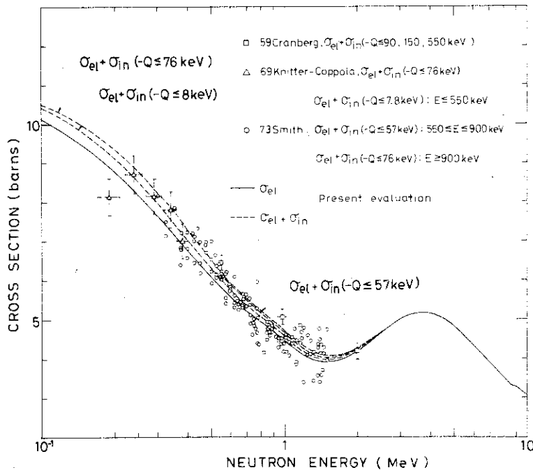
Fig.136 ELASTIC AND SOME INELASTIC SCATTERING CROSS SECTION OF Pu-239
