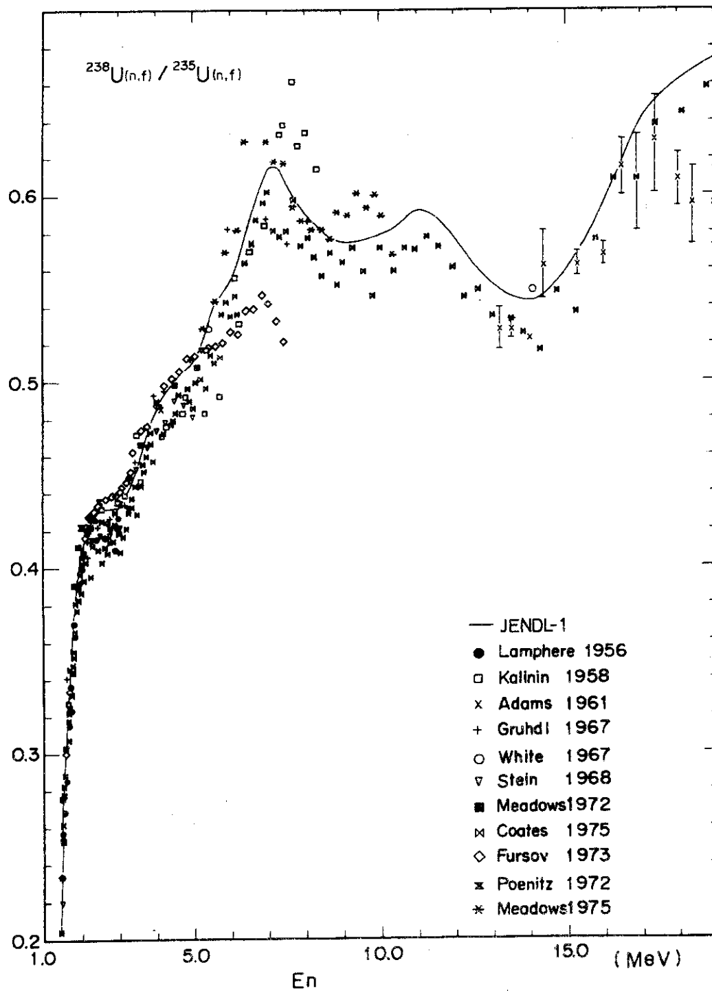
2.2.1. Ratio of fission cross section of ^{238}\text{U} to that of ^{235}\text{U}
