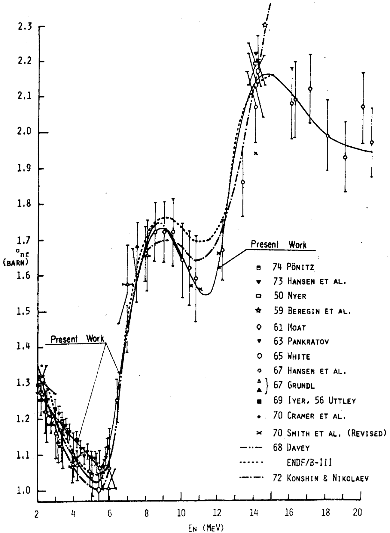
1.1.5. Fission cross section of ^{235}\text{U} from 2 to 20 MeV
