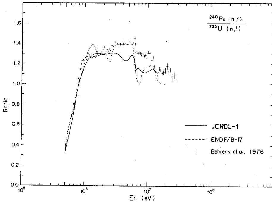
2.4.2. The ratio of ^{40}\sigma_f / ^{25}\sigma_f above 100 keV.
