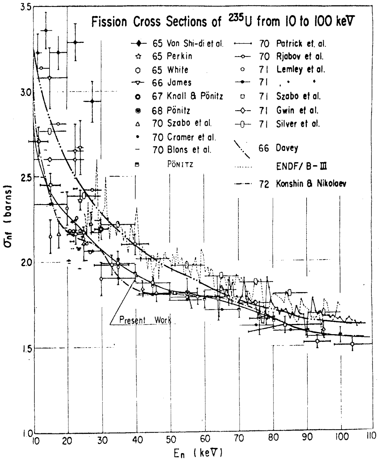
1.1.3. Fission cross section of ^{235}\text{U} from 10 to 100 keV
