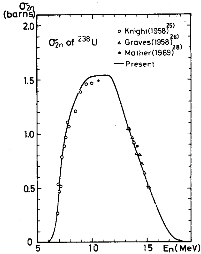
1.2.4 (n,2n) cross section of ^{238}\text{U} .
