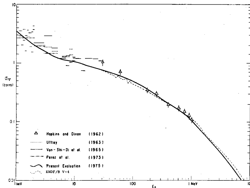
1.1.7. Capture cross section of ^{235}\text{U} from 1 keV to 1 MeV
