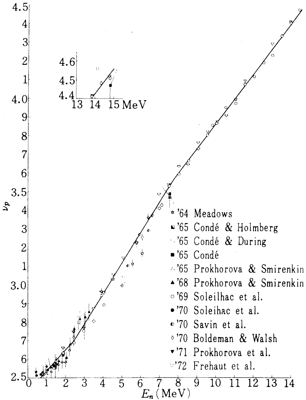
1.1.11 \nu_p of ^{235}\text{U} from 1 MeV to 10 MeV
