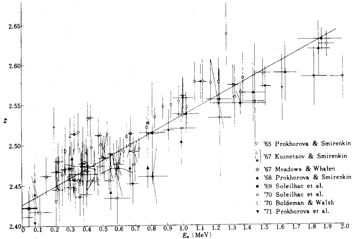
1.1.10 \nu_p of ^{235}\text{U} below 2 MeV
