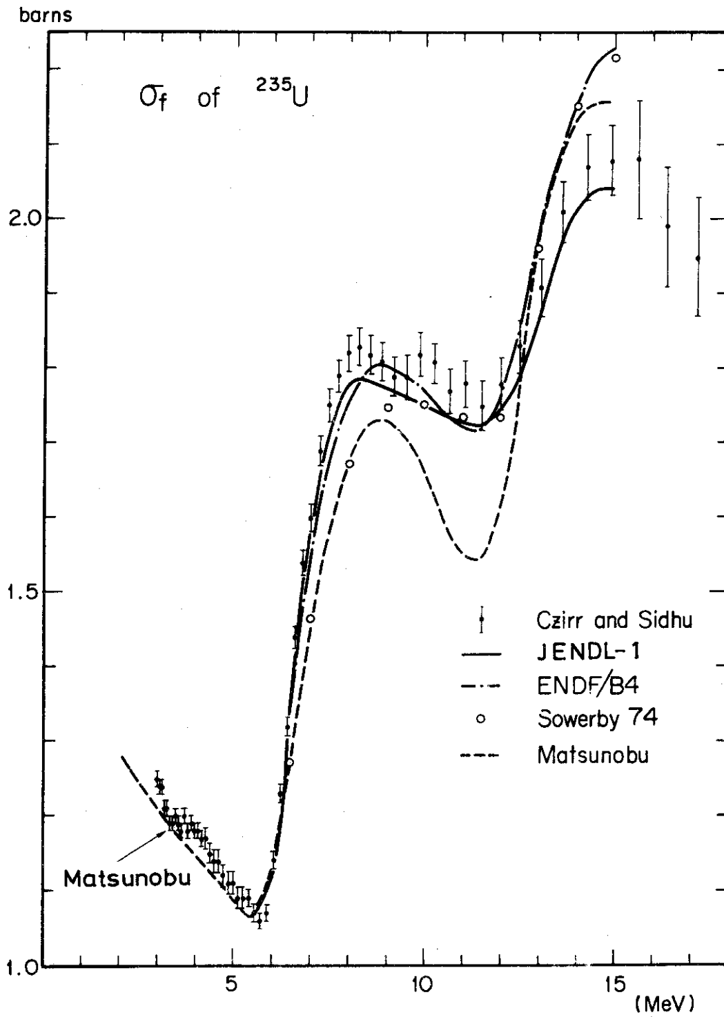
2.1.3. Fission cross section of ^{235}\text{U} in MeV region
