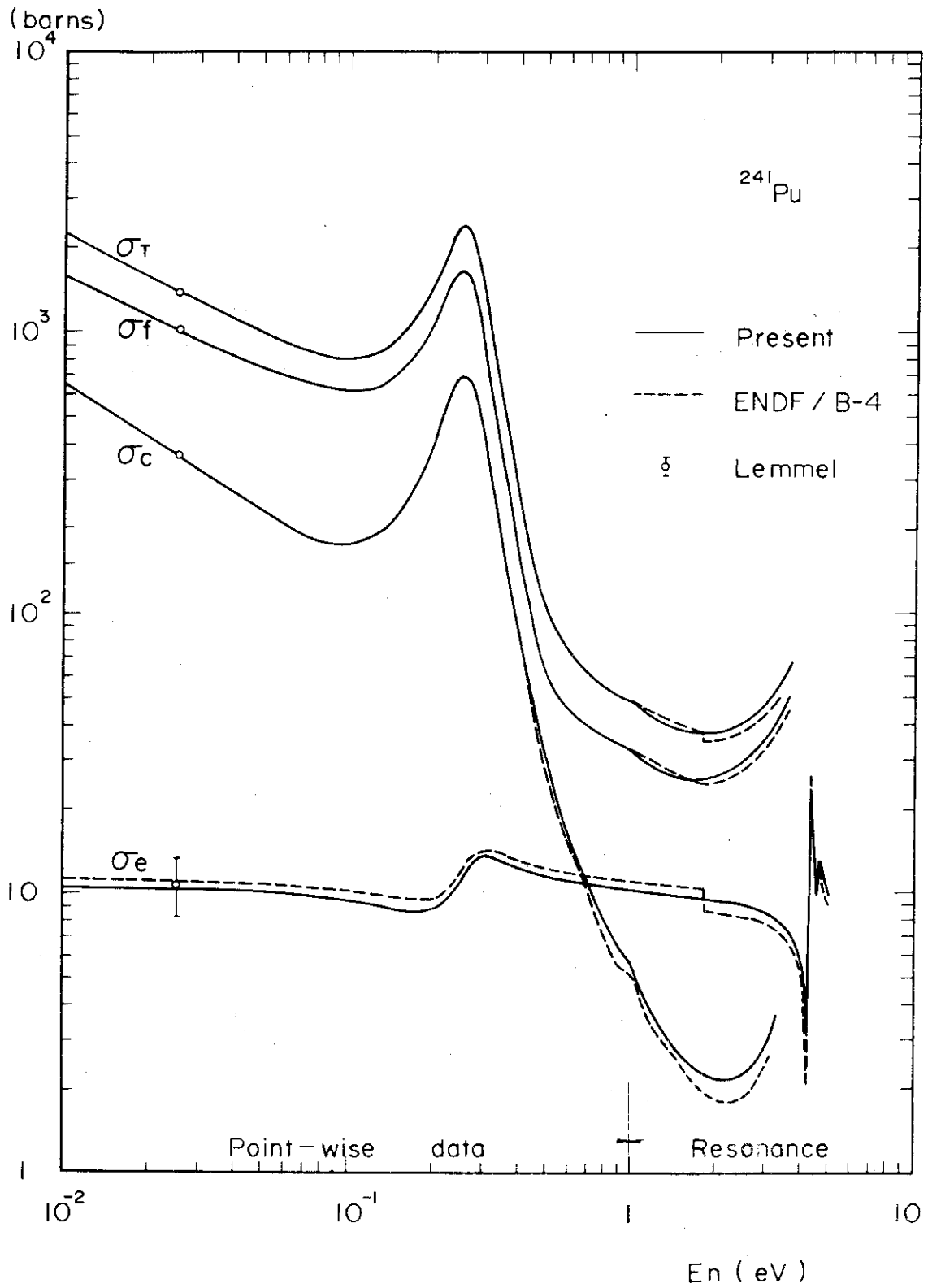
2.5.1. Cross sections of ^{241}\text{Pu} below a few eV
