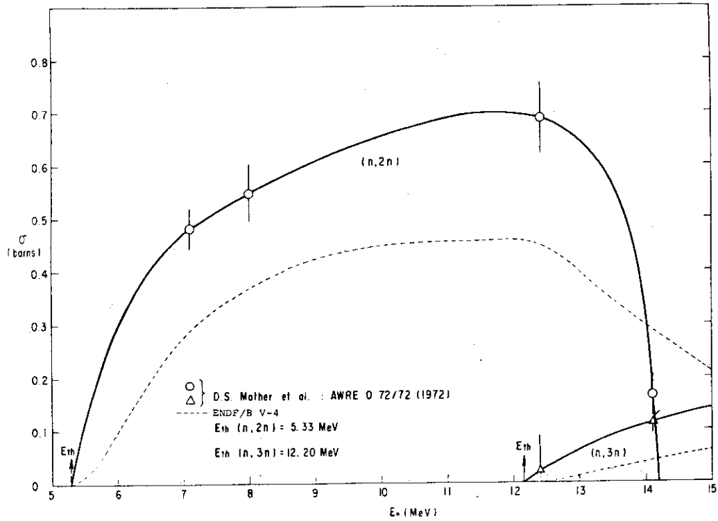
1.1.9. (n,2n) and (n,3n) cross sections of ^{235}\text{U}
