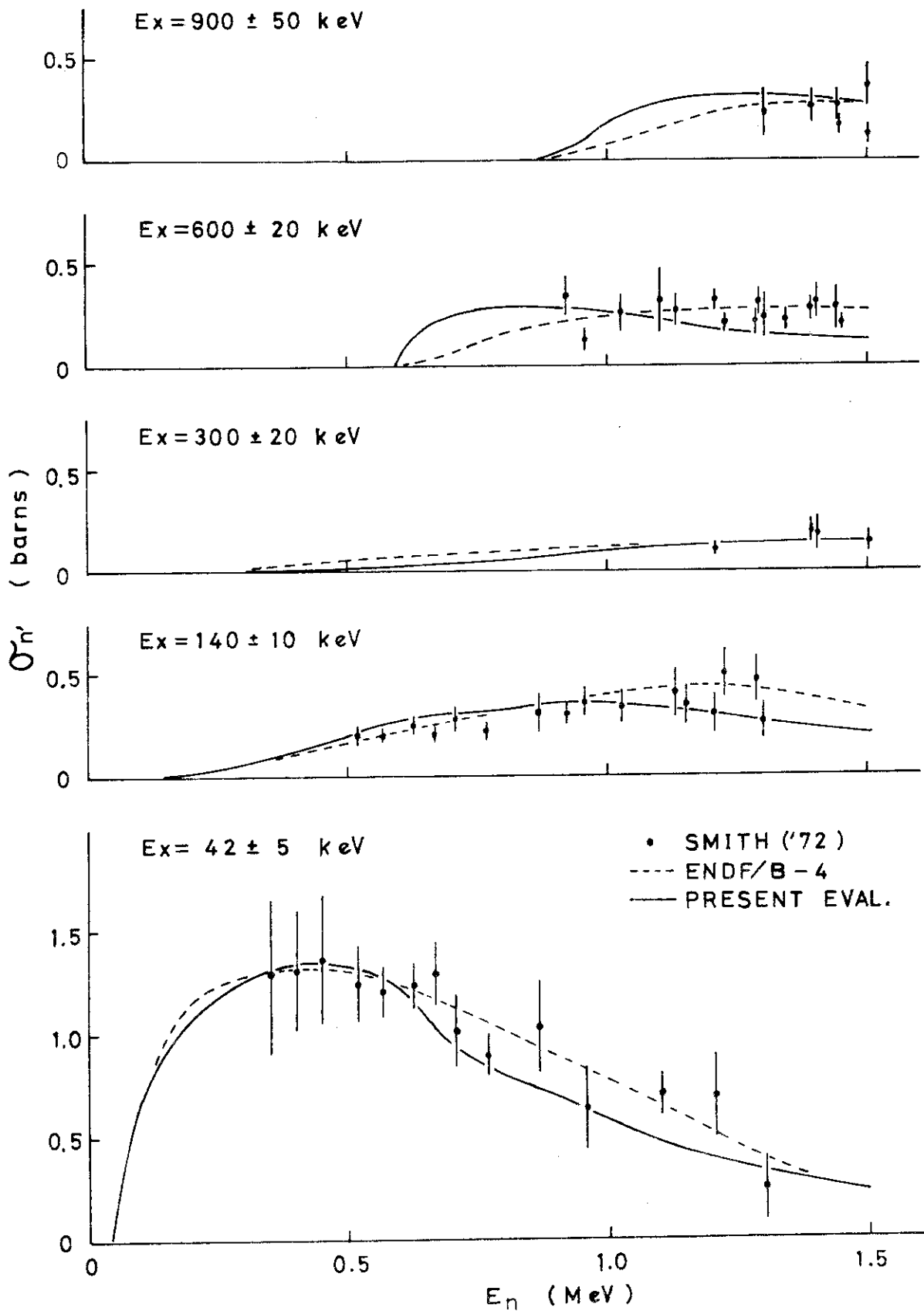
1.4.5. Partial inelastic scattering cross sections of ^{240}\text{Pu}
