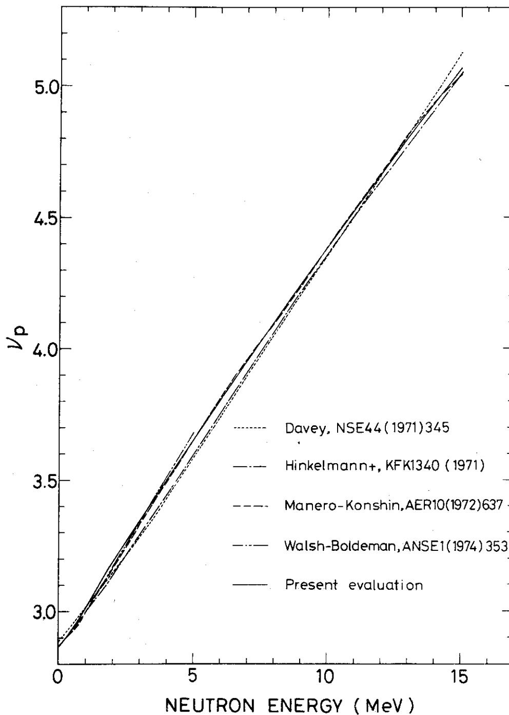
1.3.9. \nu_p of ^{239}\text{Pu}
