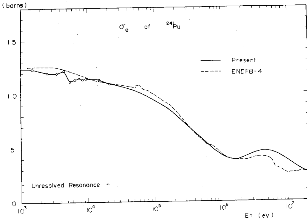
1.5.4. Elastic scattering cross section of ^{241}\text{Pu}
