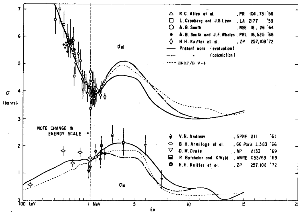
1.1.8. Total, elastic and inelastic scattering cross sections of ^{235}\text{U}
