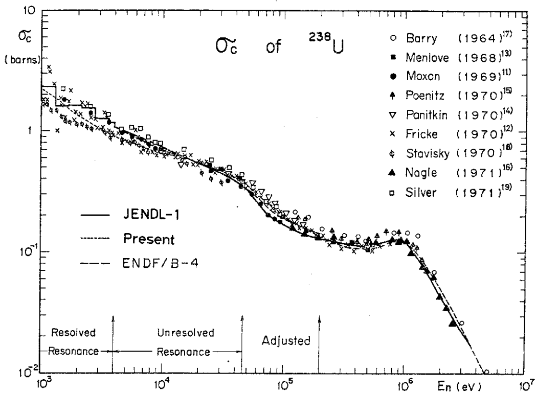
1.2.2 Capture cross sections of ^{238}\text{U} .
