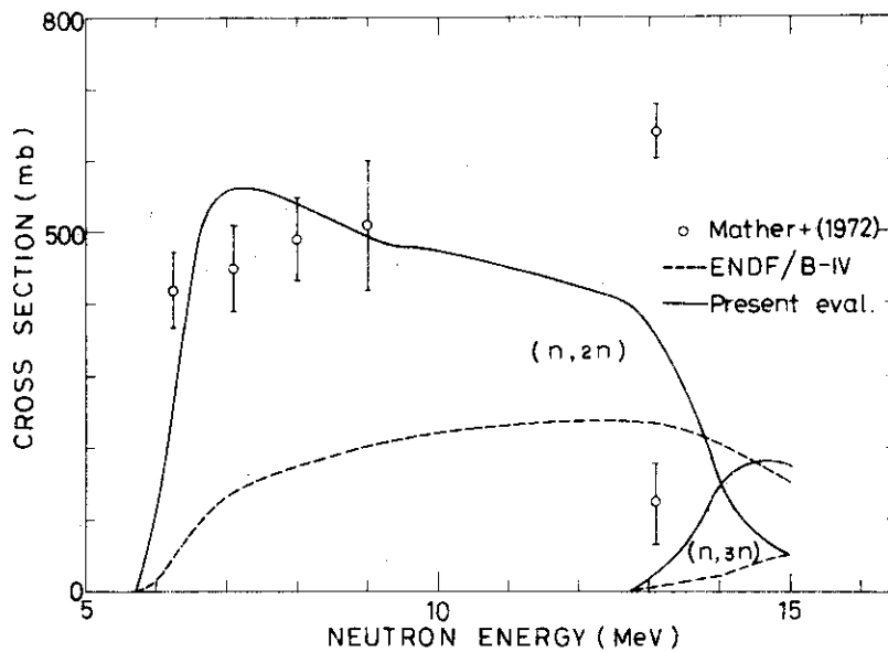
1.3.8. (n,2n) and (n,3n) cross sections of ^{239}\text{Pu}
