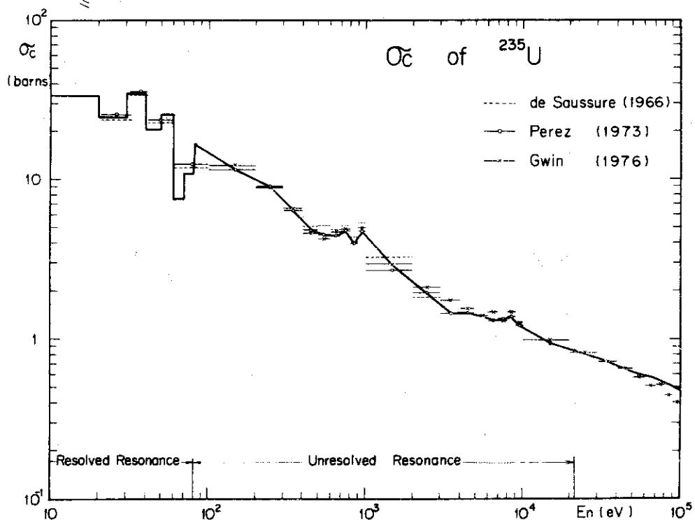
2.1.2. Capture cross section of ^{235}\text{U} in unresolved resonance region
