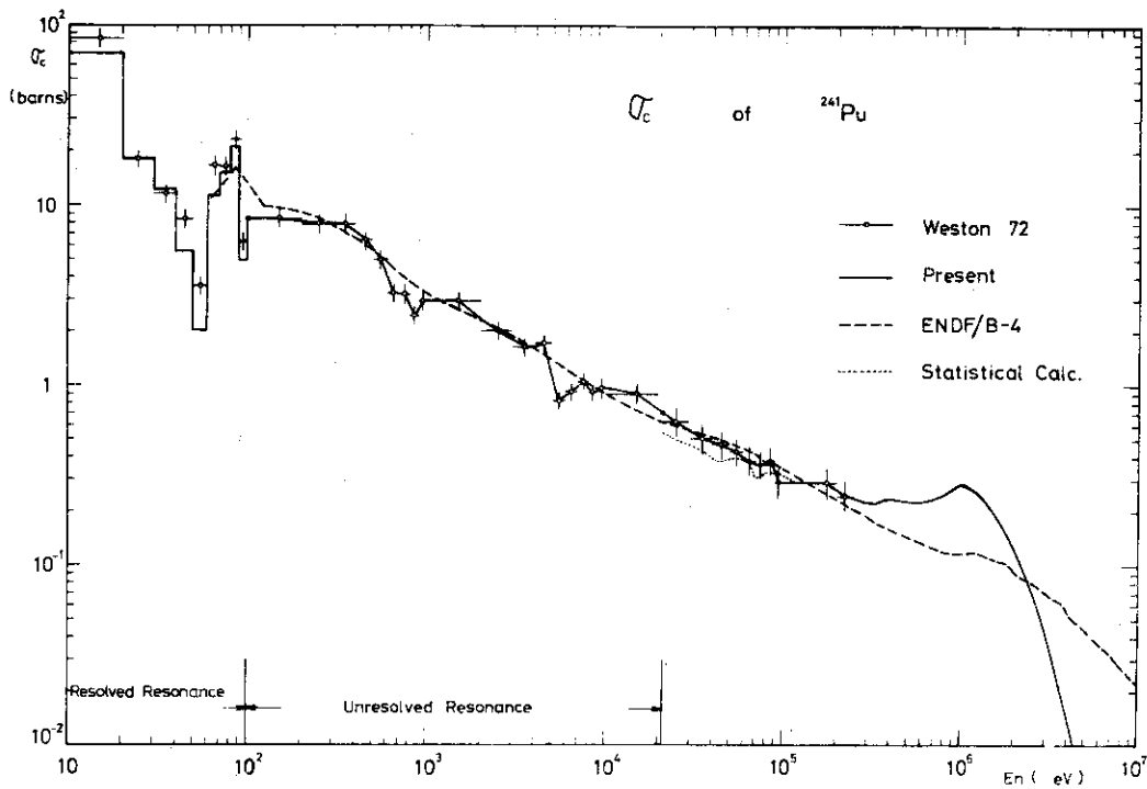
1.5.3. Capture cross section of ^{241}\text{Pu}
