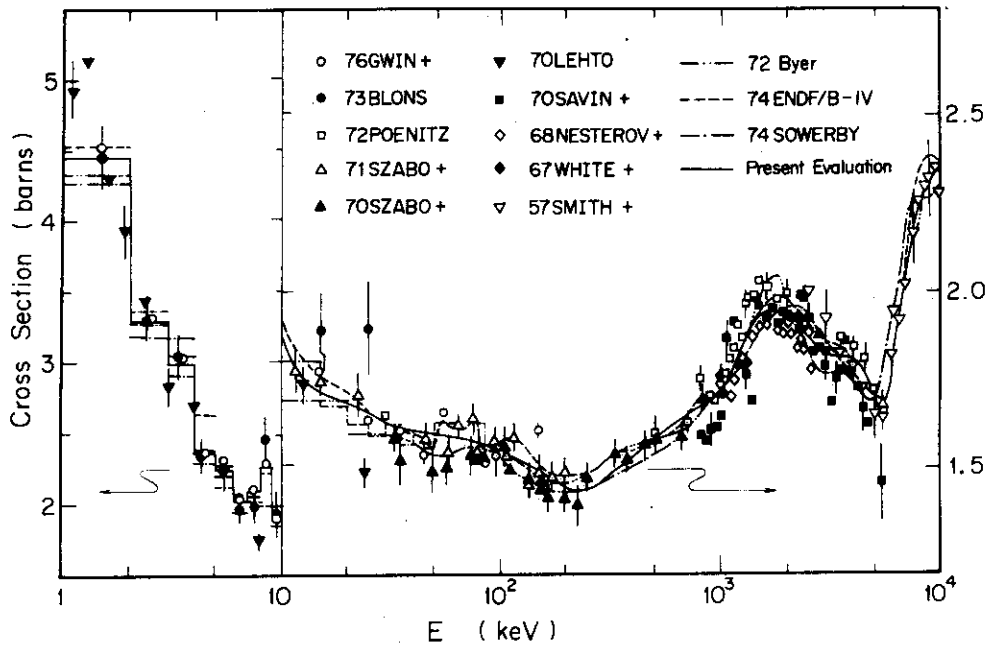
1.3.2. Fission cross section of ^{239}\text{Pu}
