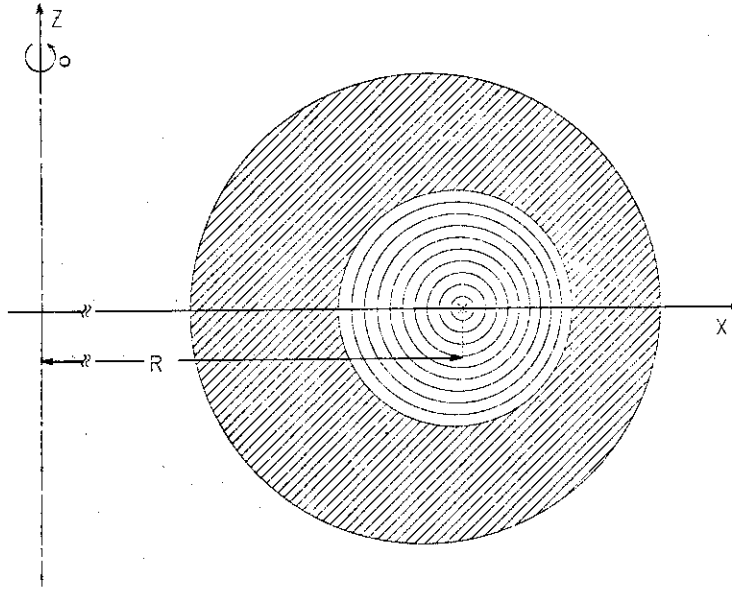
Fig.2.10 a) Equilibrium magnetic of a uniform current plasma with \epsilon^{-1}=10 , \beta_p=1 , b=2a .
