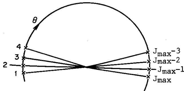
Fig.2.3 Grid points in the \theta direction. The grid points of J=2 and J=J_{\text{max}}^{-1} represent \theta=0 and \theta=\pi , respectively.
