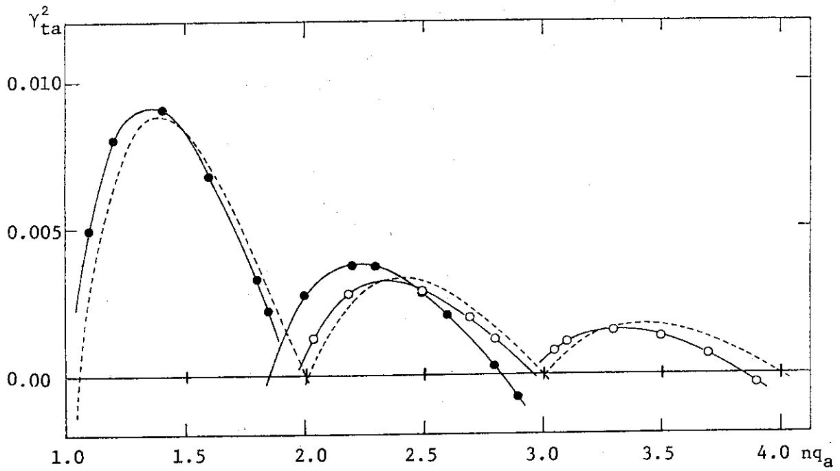
Fig.2.4 Growth rate as a function of safety factor at plasma surface r=a multiplied by the toroidal mode number n . Black and open circles denote the computed growth rate with the azimuthal mesh number J_{max}=19 and J_{max}=35 , respectively. The broken lines are analytical growth rate obtained by Eq.(2.27).
