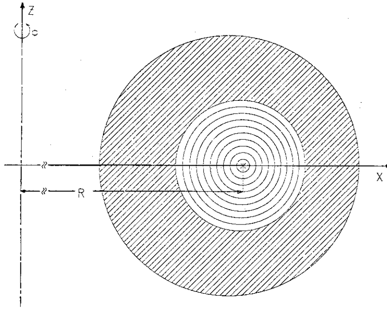
Fig.2.9 a) Equilibrium of a uniform current plasma with \epsilon^{-1}=15 , \beta_p=1 , b=2a . Shaded region is vacuum and the conducting shell is placed at the outer boundary of the region.
