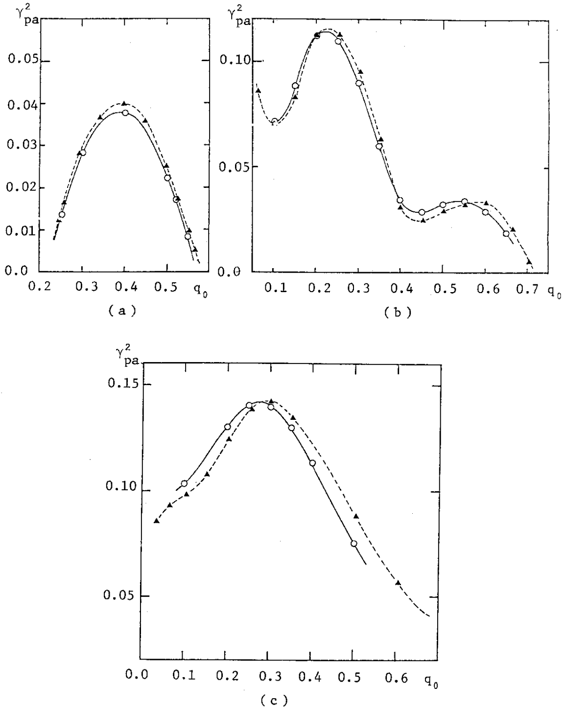
Fig.2.5 Comparison of growth rate by two codes vs. safety factor at magnetic axis. The solid and broken lines show the growth rates obtained by ZEPHYRUS and ERATO codes, respectively. The parameters in this calculation are: (a) E=1, n=2 , (b) E=1, n=3 and (c) E=2, n=2 . The aspect ratio \epsilon^{-1}=3 for all cases. The growth rates are normalized to the poloidal Alfvén transit time.
