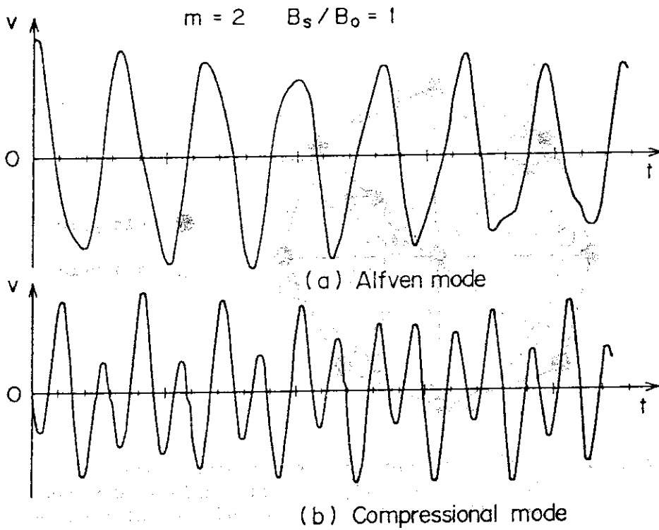
Fig. 3.6 Oscillations of the radial velocity at r=a/2 for (a) the m=2 Alfvén mode and (b) the m=2 compressional mode.
