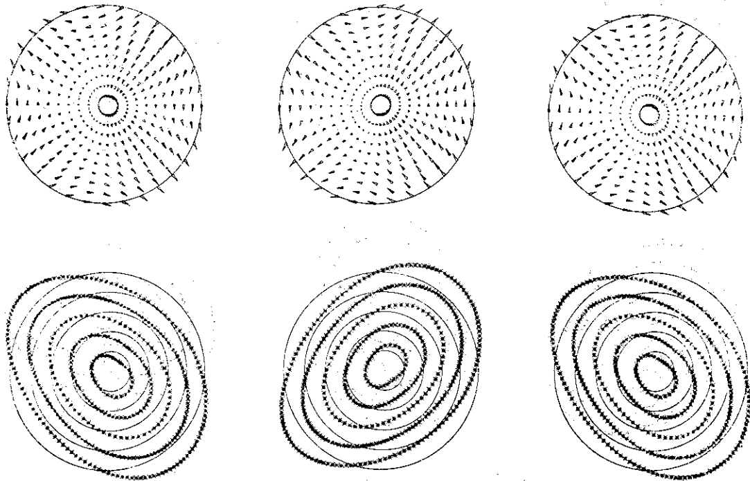
Fig.2.9 b) Eigenfunctions of the m=2 external mode for q_0=1.2 and n=3 at three different toroidal locations.
