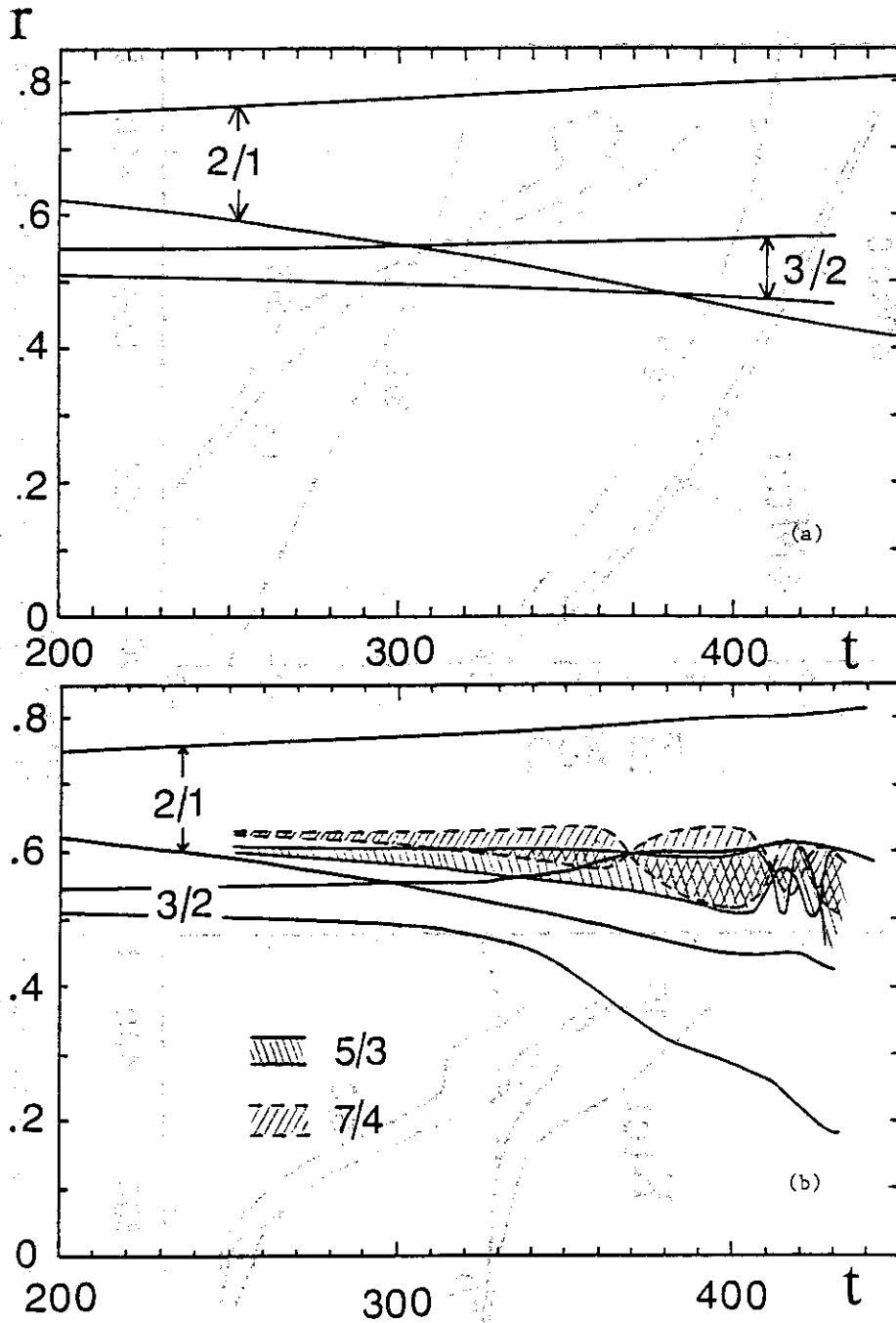
Fig.4.1. Time evolution of the m/n mode magnetic island width for the case of (a) single-helicity calculation and (b) multi-helicity calculation. The widths for both cases are the same before the island-overlapping time ( t = 300 ).
