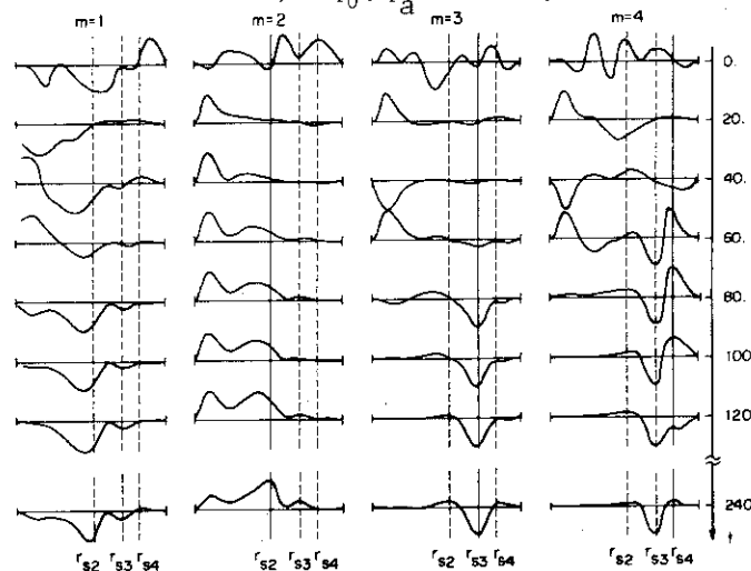
(c) Toroidal case, (q_0, q_a) = (0.46, 1.96) , n=3 .
