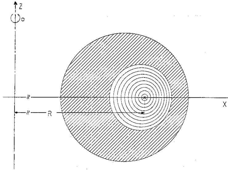
Fig.2.11 a) Equilibrium magnetic of a uniform current plasma with \epsilon^{-1}=5 , \beta_p=1 , b=2a .
