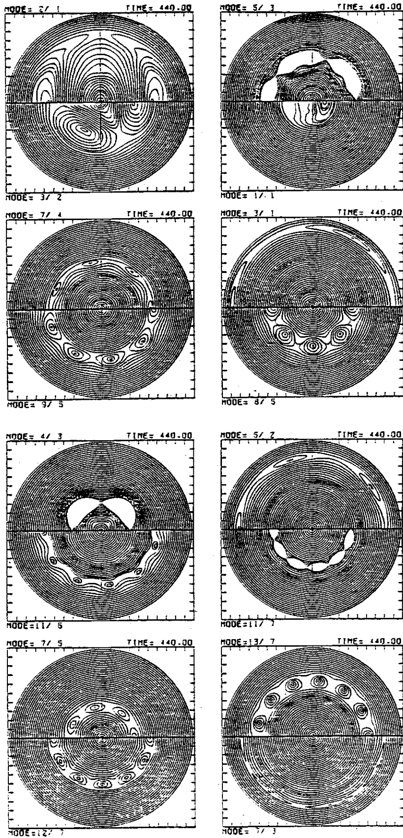
Fig.4.5 Helical flux contours of different helicities at the end of the calculation, t = 440 .
