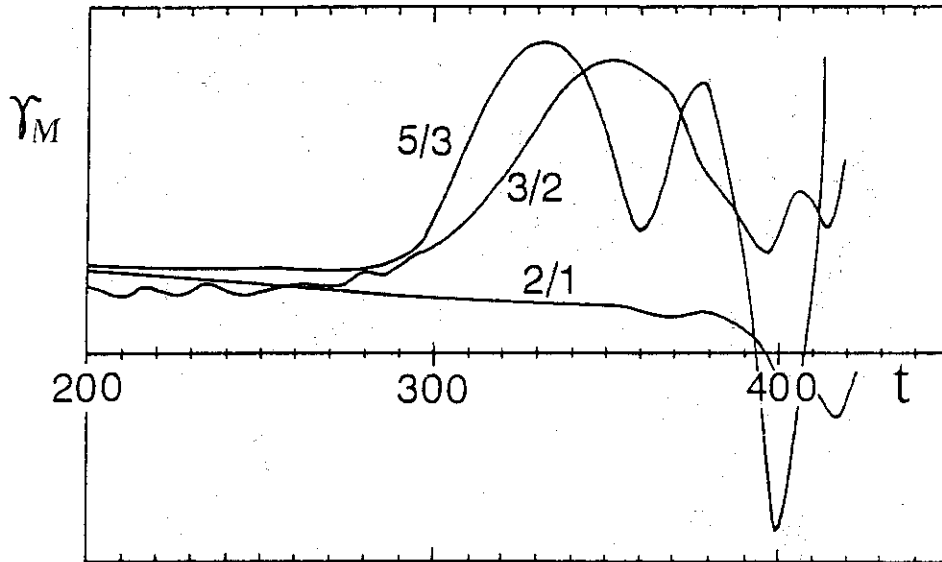
Fig.4.3 Instantaneous growth rates of the m/n magnetic energy. The growth rates of the 3/2 and 5/3 modes start to increase at the island-overlapping time ( t=300 ), while the 2/1 mode remains in the Rutherford regime.
