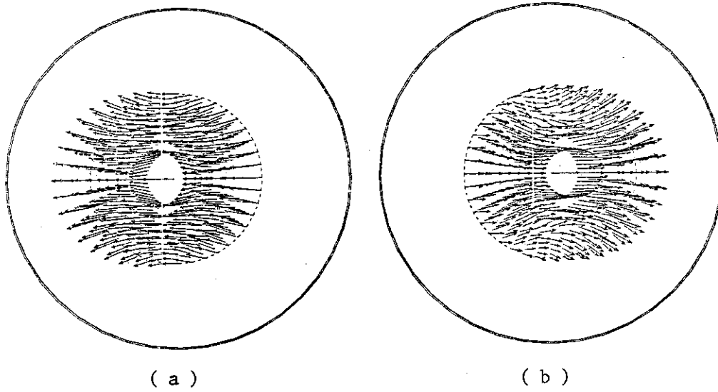
Fig. 3.12 Velocity vectors of m=1 Alfvén mode in the case of free boundary at (a) t=2.5 and (b) t=5.5 . The outer circles represent the shell.
