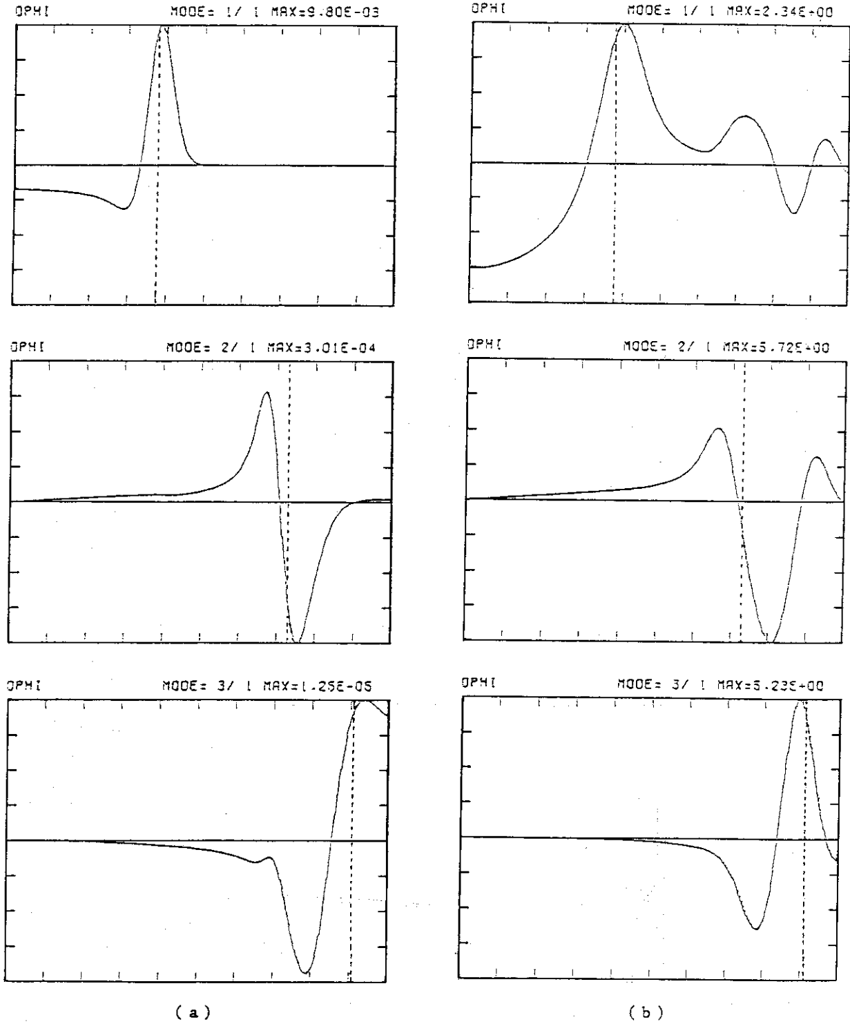
Fig. 5.3 Eigenfunctions of v^v of n=1 mode for (a) \beta_p=0 and (b) \beta_p=3 for fixed \varepsilon(=0.1) and S(=2 \times 10^4) . The poloidal mode numbers are m=1 , m=2 , and m=3 from the top to bottom. In each subfigure, the dotted line denotes the position of the singular surface of the mode.
