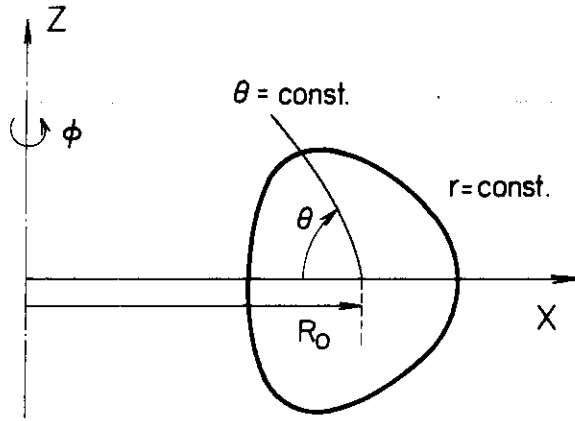
Fig.2.1 Curvilinear coordinate system (r, \theta, \phi) . The closed curve ( r = \text{const.} ) is the intersection of a magnetic surface.
