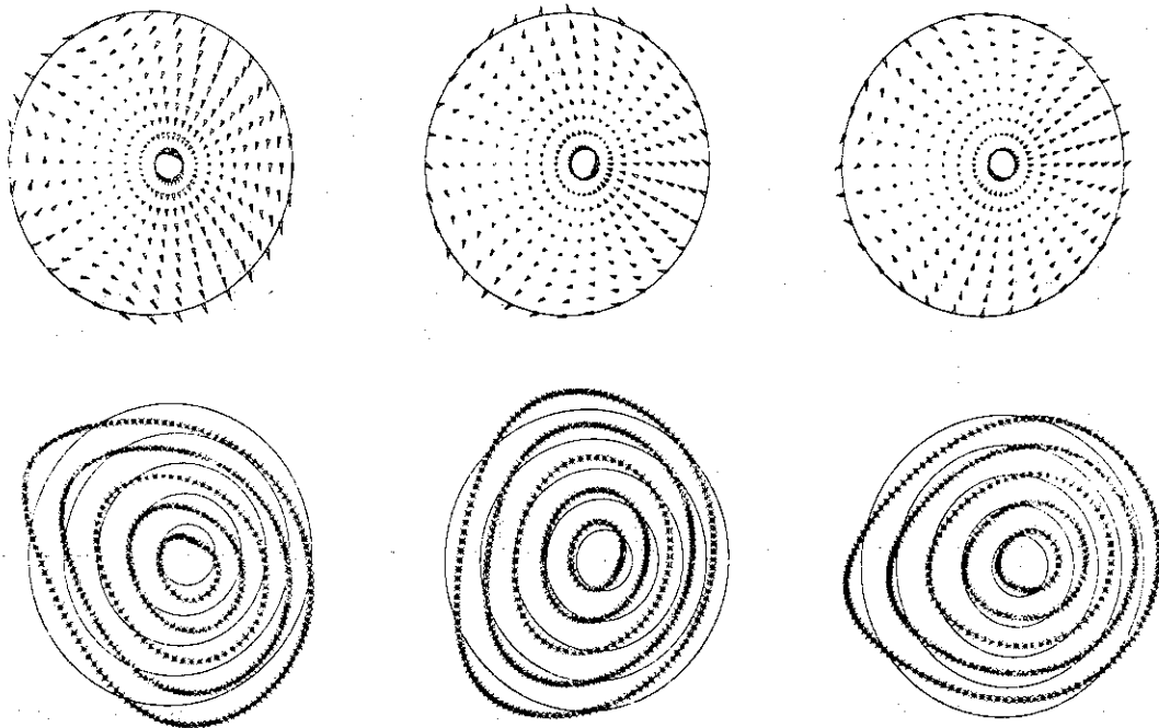
Fig.2.11 b) Eigenfunctions of the m=2 external mode for q_0=1.2 and n=1 at three different toroidal locations.
