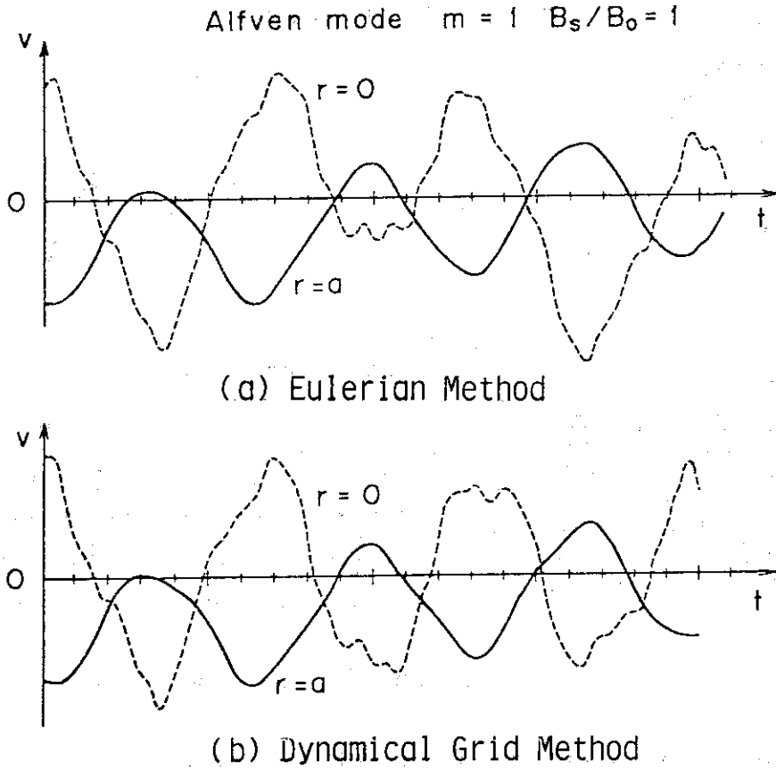
Fig. 3.9 Comparison of the result for the m=1 Alfvén mode obtained by (a) the Eulerian method with that by (b) the dynamical grid method. The solid curve corresponds to the total velocity at the plasma surface and the broken one corresponds to the velocity of the center grid.
