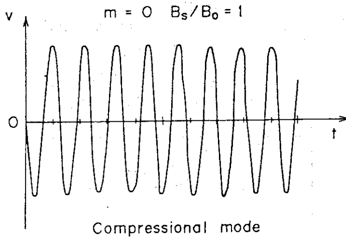
Fig. 3.5 Oscillation of the radial velocity at r=a/2 for the m=0 compressional mode in a fixed-boundary plasma with uniform mass and uniform current distributions ( B_s/B_0=1.0 ).
