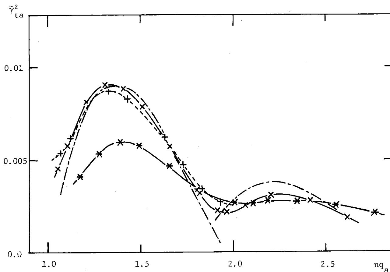
Fig.2.8 Growth rate vs. nq_a , for \epsilon n = 0.2 . Dotted solid curve is the growth rate in cylindrical case and other curves are toroidal cases in which the solid line with the mark \times , broken line with the mark + and solid line with the mark * denote the cases of \epsilon^{-1} = 15 , \epsilon^{-1} = 10 and \epsilon^{-1} = 5 , respectively, for \beta_p = 1 , b = 2a and uniform current distribution.
