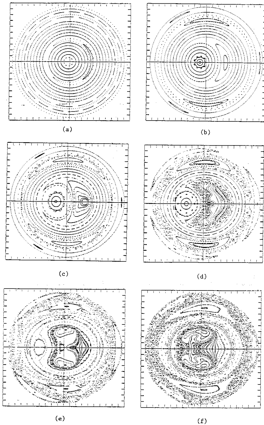
Fig. 5.7 Intersections of the trajectories of the magnetic field lines at the poloidal plane, \zeta=0 , for (a) t=50 , (b) t=100 , (c) t=125 , (d) t=150 , (e) t=165 , and (f) t=180 . In each subfigure several tens of trajectories with different starting points are demonstrated. Internal disruption occurs at t \approx 160 .
