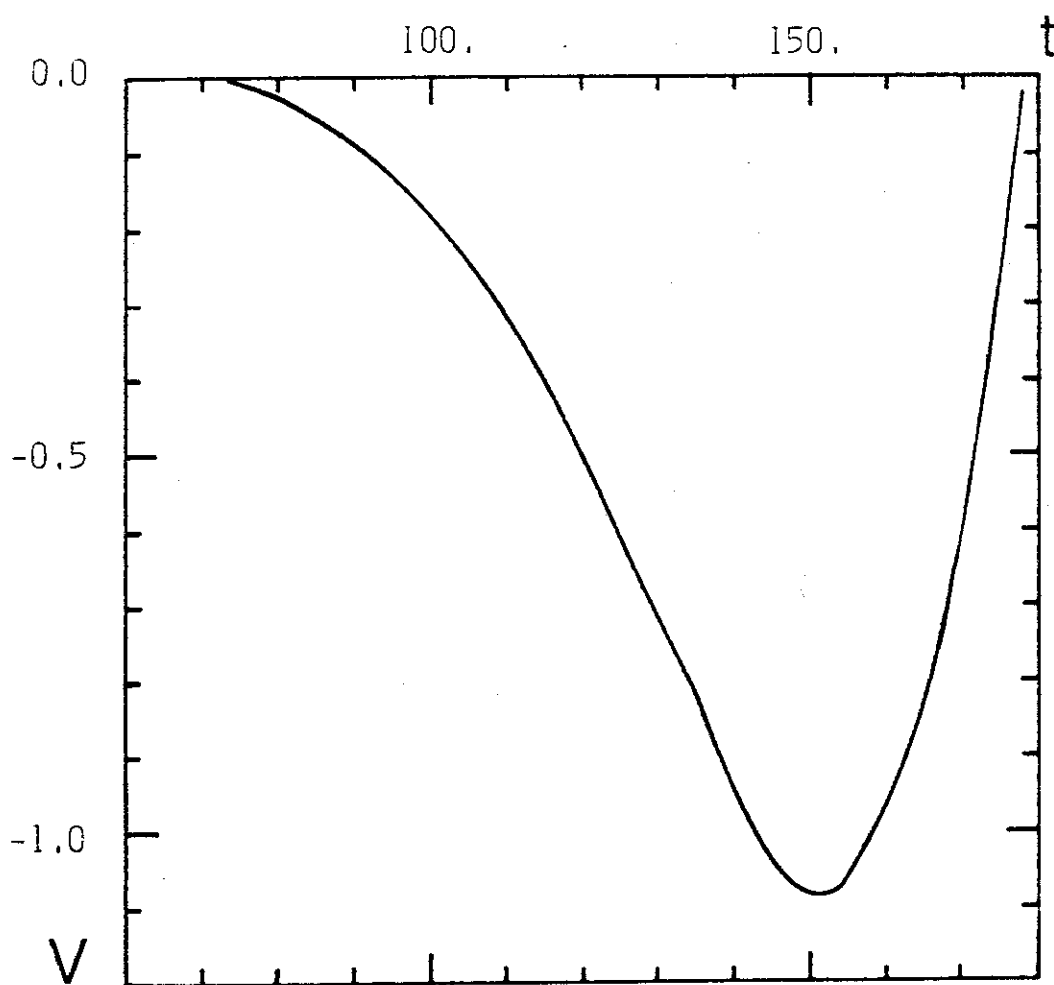
Fig. 5.8 Time evolution of the one-turn voltage at the limiter for the case \epsilon=0.1 , \beta_p=1.0 and S=2 \times 10^4 with pressure perturbation.
