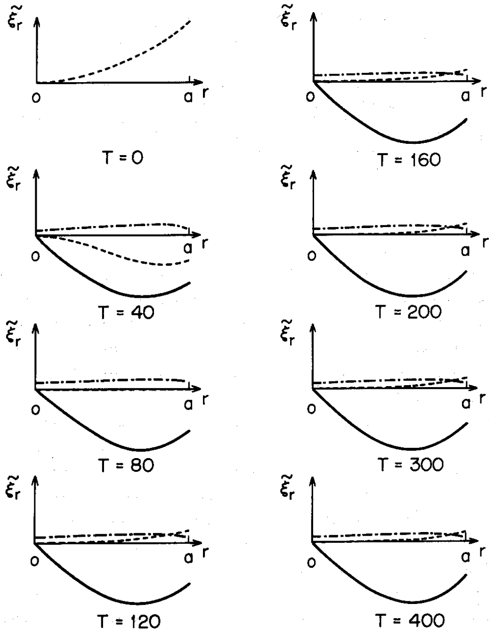
Fig.2.13 Time development of the Fourier component of \xi^r(r, \theta) expanded in \theta direction for \epsilon^{-1}=15 , q_a=2.0 and uniform current distribution. Solid, broken and dotted solid lines denote m=2 , m=3 and m=1 modes, respectively. They are normalized to its maximum value in each subfigure.
