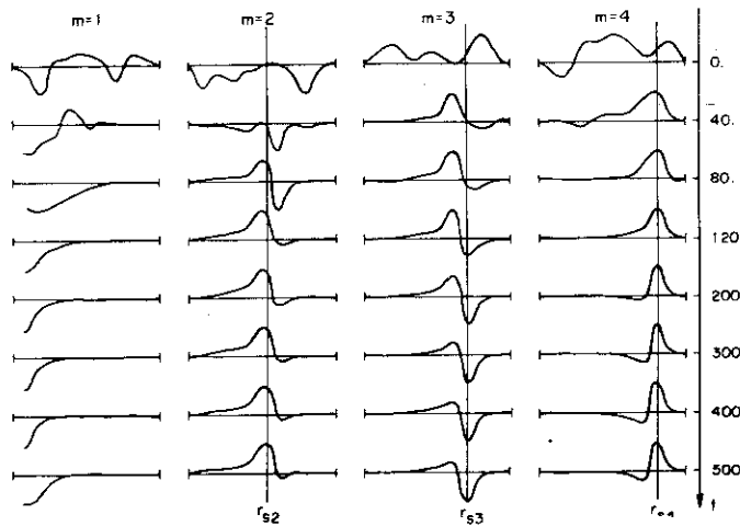
(a) Cylindrical case, (q_0, q_a) = (1.0, 6.0) , n=1 .
