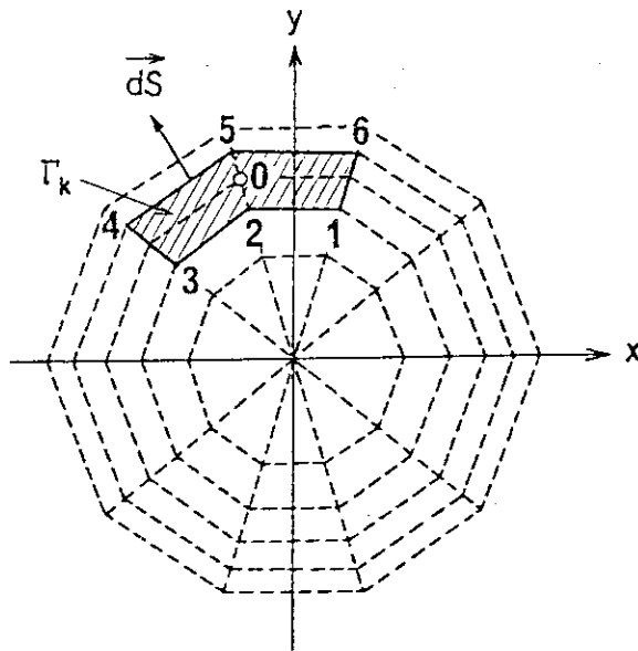
Fig. 3.2 Grid configuration in AEOLUS-P code for the analysis of the n=0 mode in a cylindrical plasma. All the physical quantities are integrated in the region \Gamma_k .
