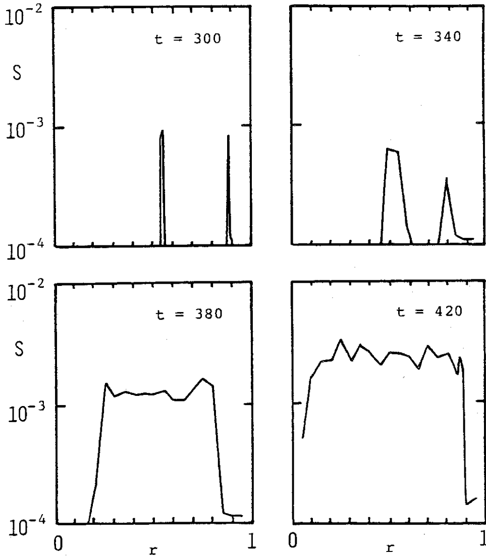
Fig.4.7 Space distribution of the K-S entropy of a magnetic field line at t=300, 340, 380 and 420 . The K-S entropy is defined by
