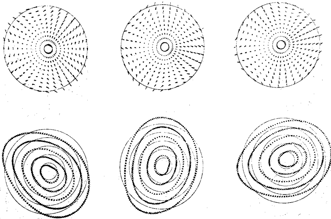
Fig.2.10 b) Eigenfunctions of the m=2 external mode for q_0=1.2 and n=2 at three different toroidal locations.
