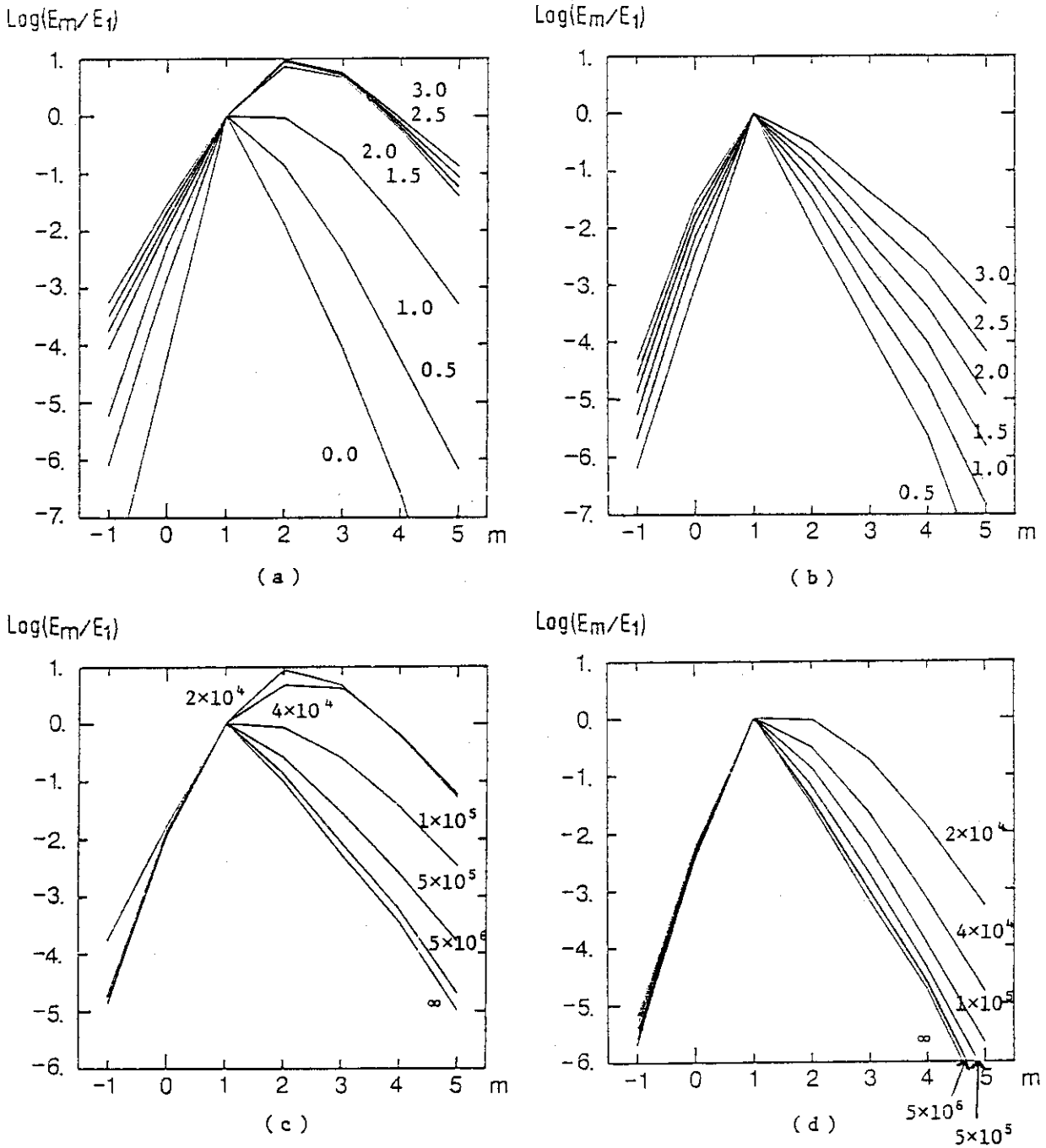
Fig. 5.2 Magnetic energy of the n=1 mode versus the Fourier mode number: (a) \beta_p dependence for fixed \epsilon (=0.1) and S (=2 \times 10^4) , (b) \beta_p dependence for fixed \epsilon (=0.1) and S (= \infty) , (c) S dependence for fixed \epsilon (=0.1) and \beta_p (=2.0) and (d) S dependence for fixed \epsilon (=0.1) and \beta_p (=1.0) .
