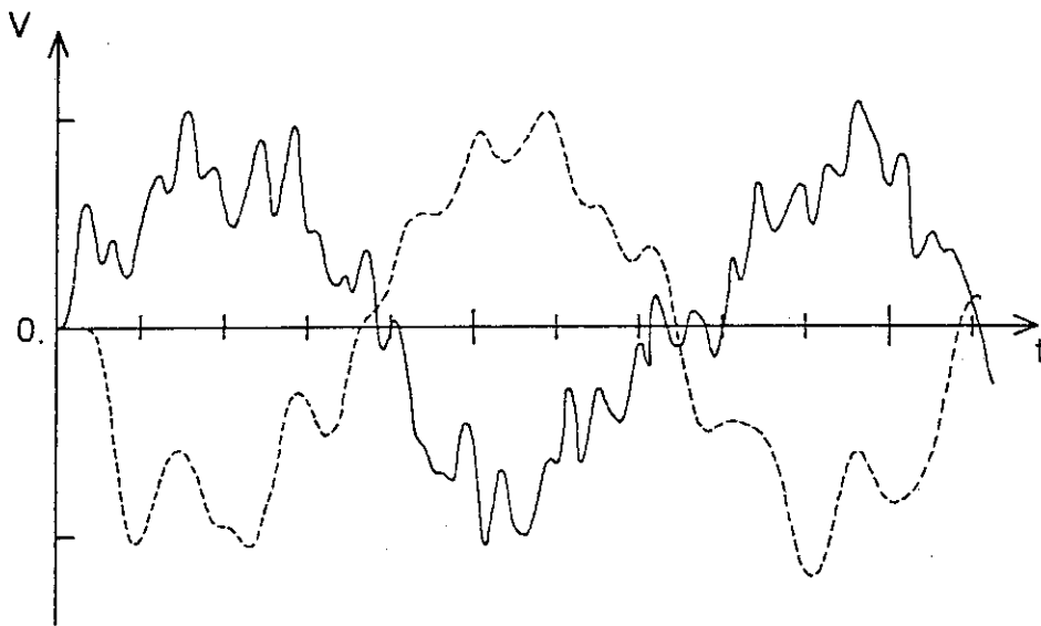
Fig. 3.11 Oscillations of radial velocity of m=1 Alfvén mode for B_s/B_0=1.0 . The shell is located at r=2a . The solid curve corresponds to the total velocity at r=a/2 and the broken one corresponds to the total velocity at r=0 .
