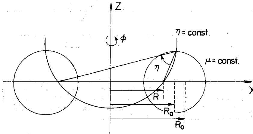
Fig.2.2 Toroidal coordinate system (\mu, \eta, \phi) used for the calculation of vacuum magnetic field. R_0 is the radius of the center of circular plasma surface and R , the singular point of toroidal coordinate, R = \sqrt{R_0^2 - a^2} .
