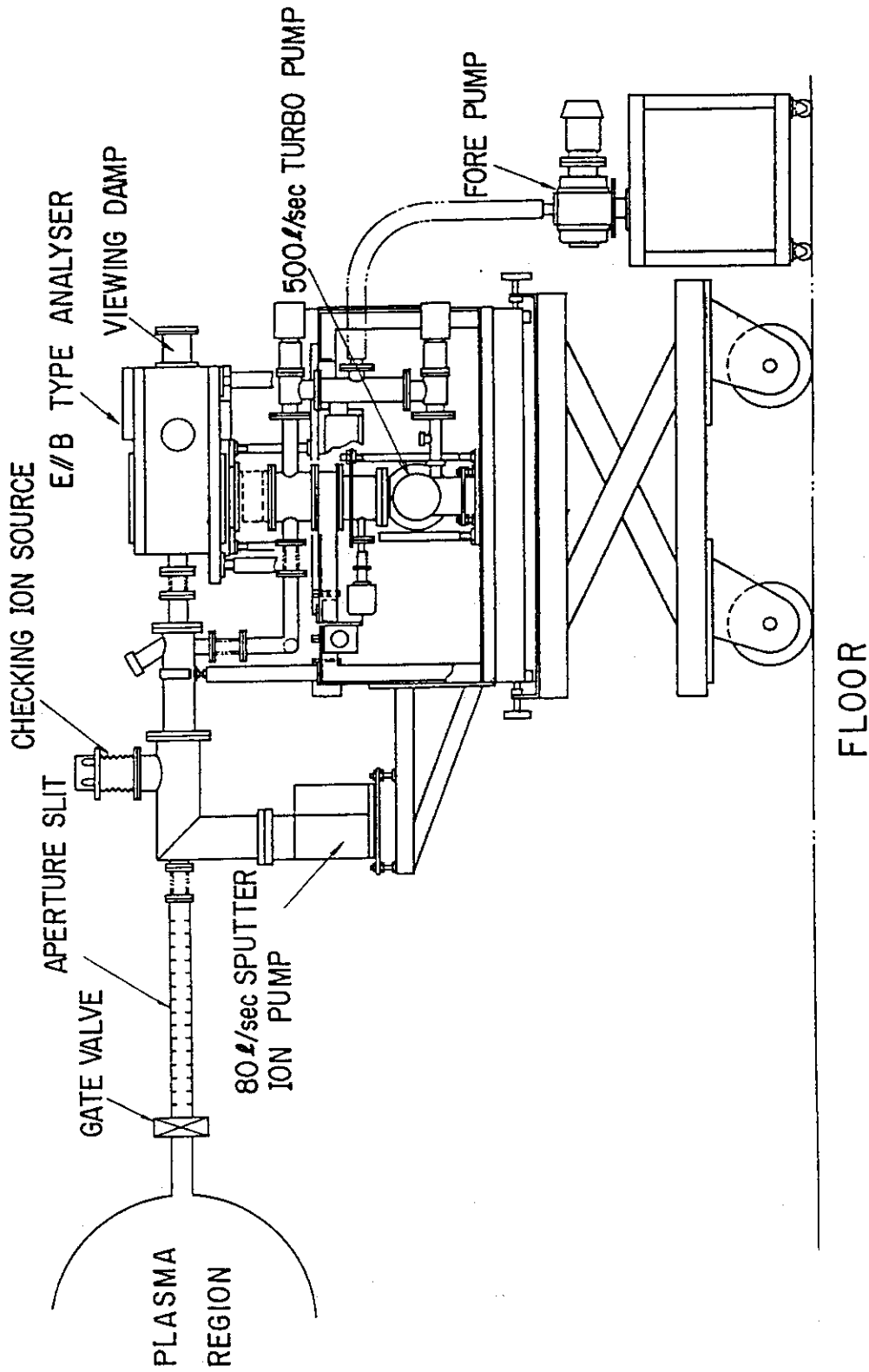
Fig. 12 Experimental set-up for measuring charge-exchanged neutral particle spectrum from the JFTI-2 tokamak plasma
