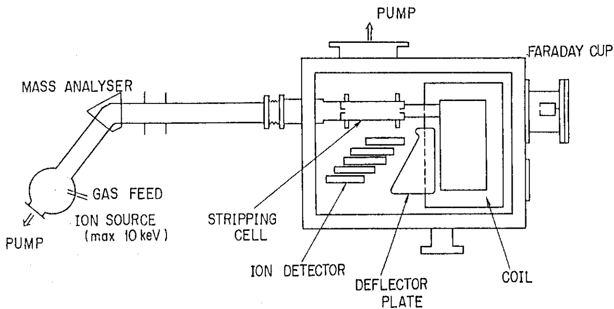
Fig. 5 Schematic diagram of set-up for calibration experiments
