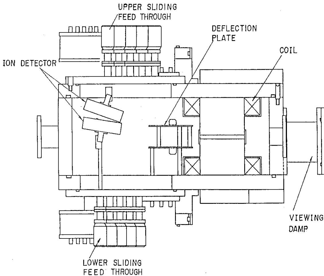
Fig. 3 Sectional side view of E//B type analyser
