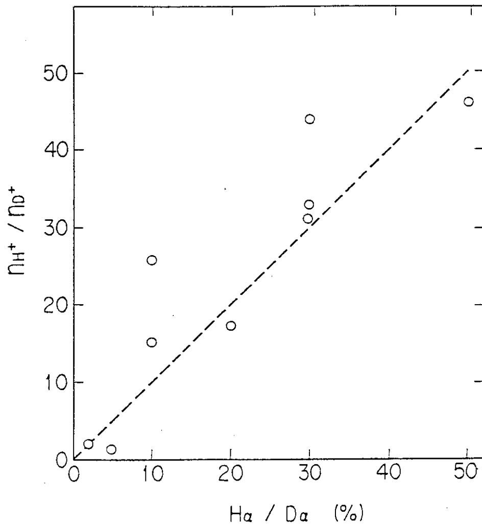
Fig. 18 Comparison of the ratio of deuterium and proton density determined by the energy spectrum with the ratio of hydrogen and deuterium density estimated by H\alpha and D\alpha line intensity respectively
