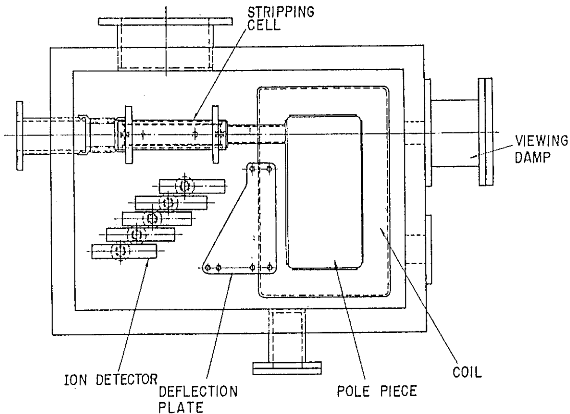
Fig. 2 Sectional plan view of E//B type analyser
