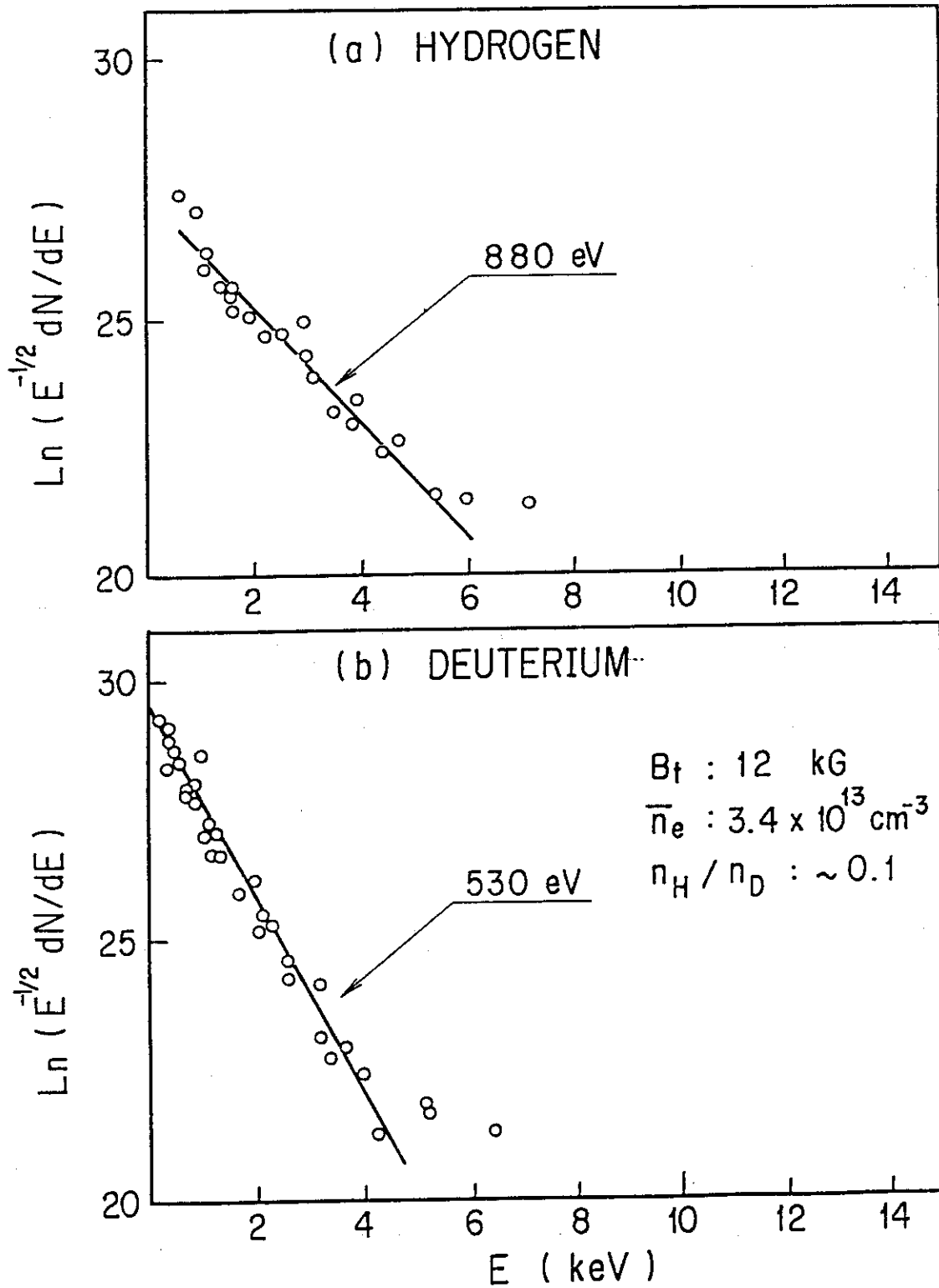
Fig. 15 The obtained energy spectra of (a) hydrogen and (b) deuterium in the discharge of the ratio of hydrogen to deuterium 1:10 which was heated by ion cyclotron wave power of 130 kW.
