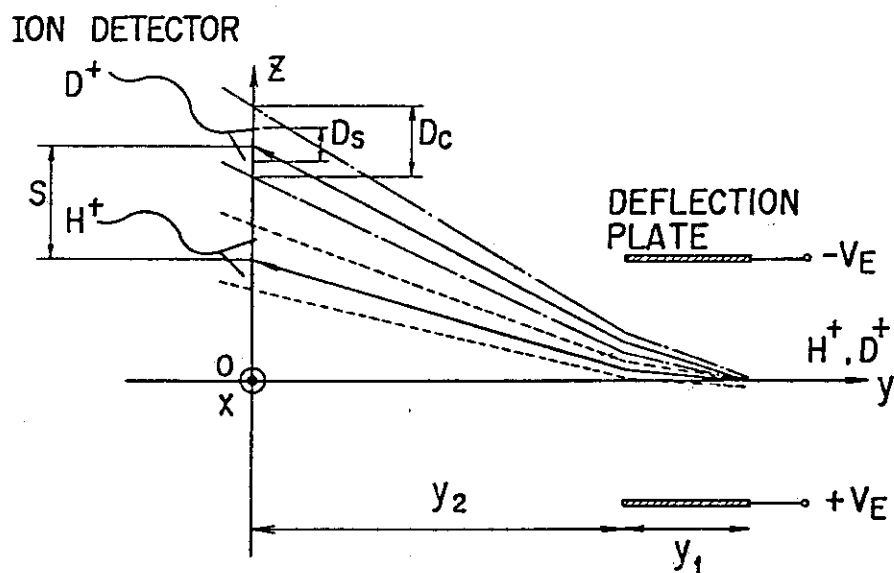
Fig. 4 Diagram explaining the condition of mass separation
