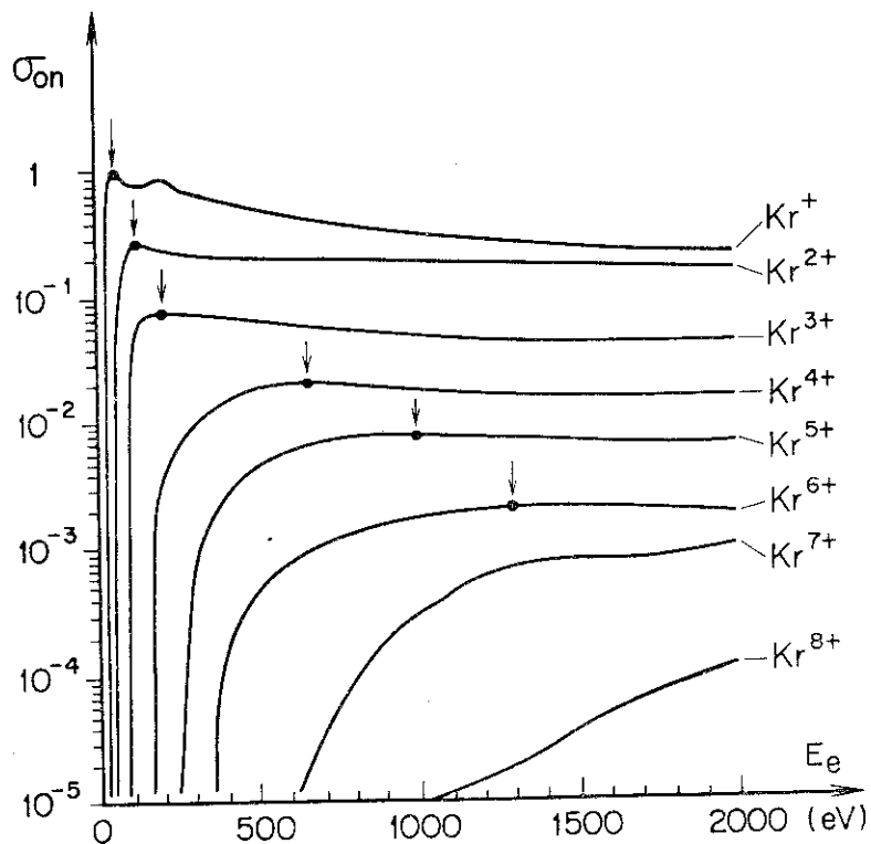
Fig. 4 Values of ionization cross section \sigma_{on} of krypton atoms as a function of impact energy E_e for different values of n
