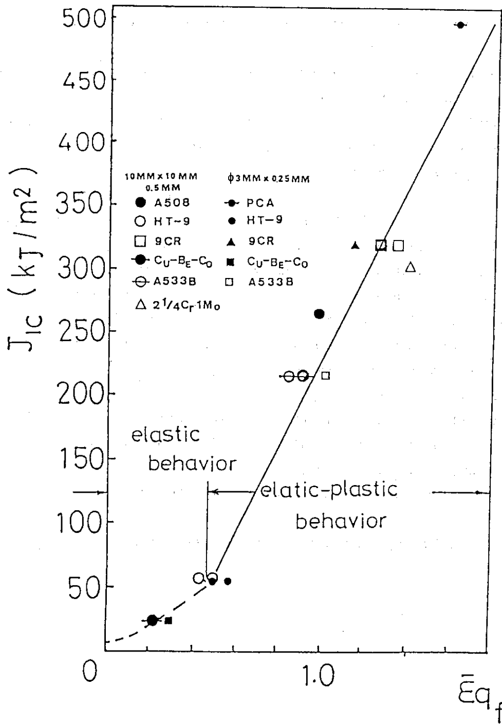
Fig. 8 Relation between \bar{\epsilon}_{qf} and J_{IC} .
