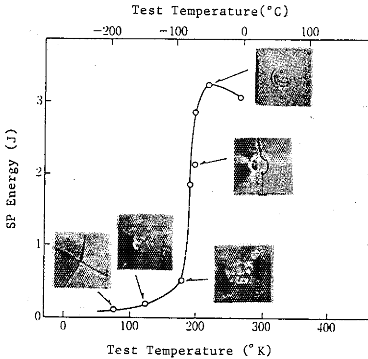
Fig. 5 Transition curve of SP energy and related fracture appearance. (J. Kameda et al.)
