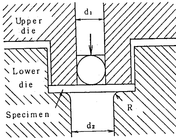
Small Punch Test (Bulge Test)
