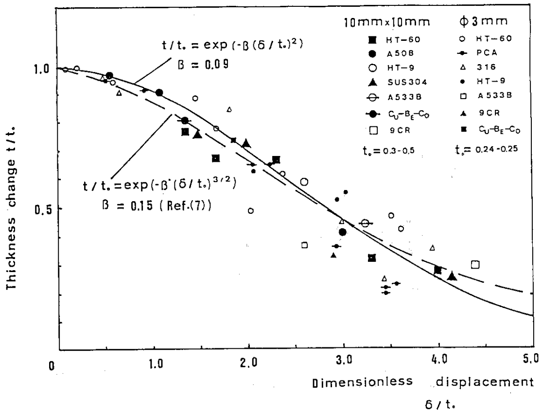
Fig. 7 Relation between t/t_0 and \delta/t in SP test.
