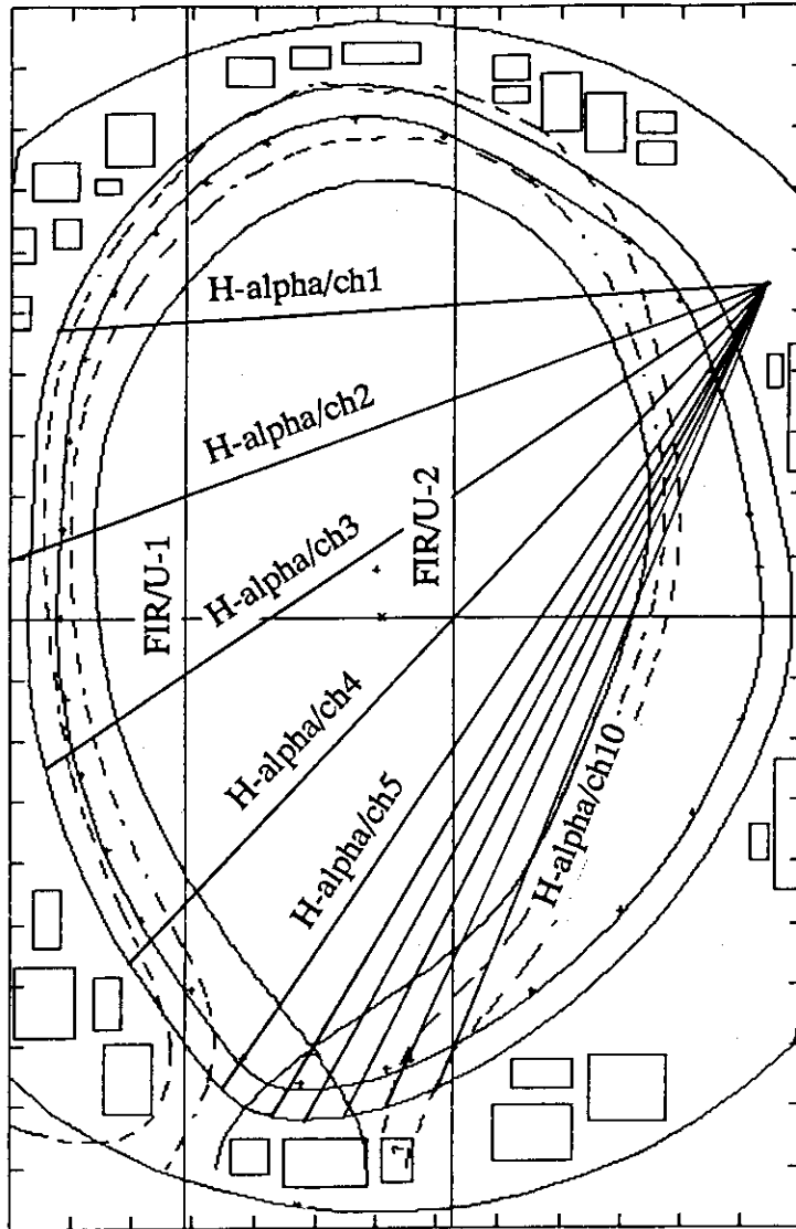
Fig.1 The plasma configuration and the measurement chords of FIR interferometer and H-alpha monitor.
