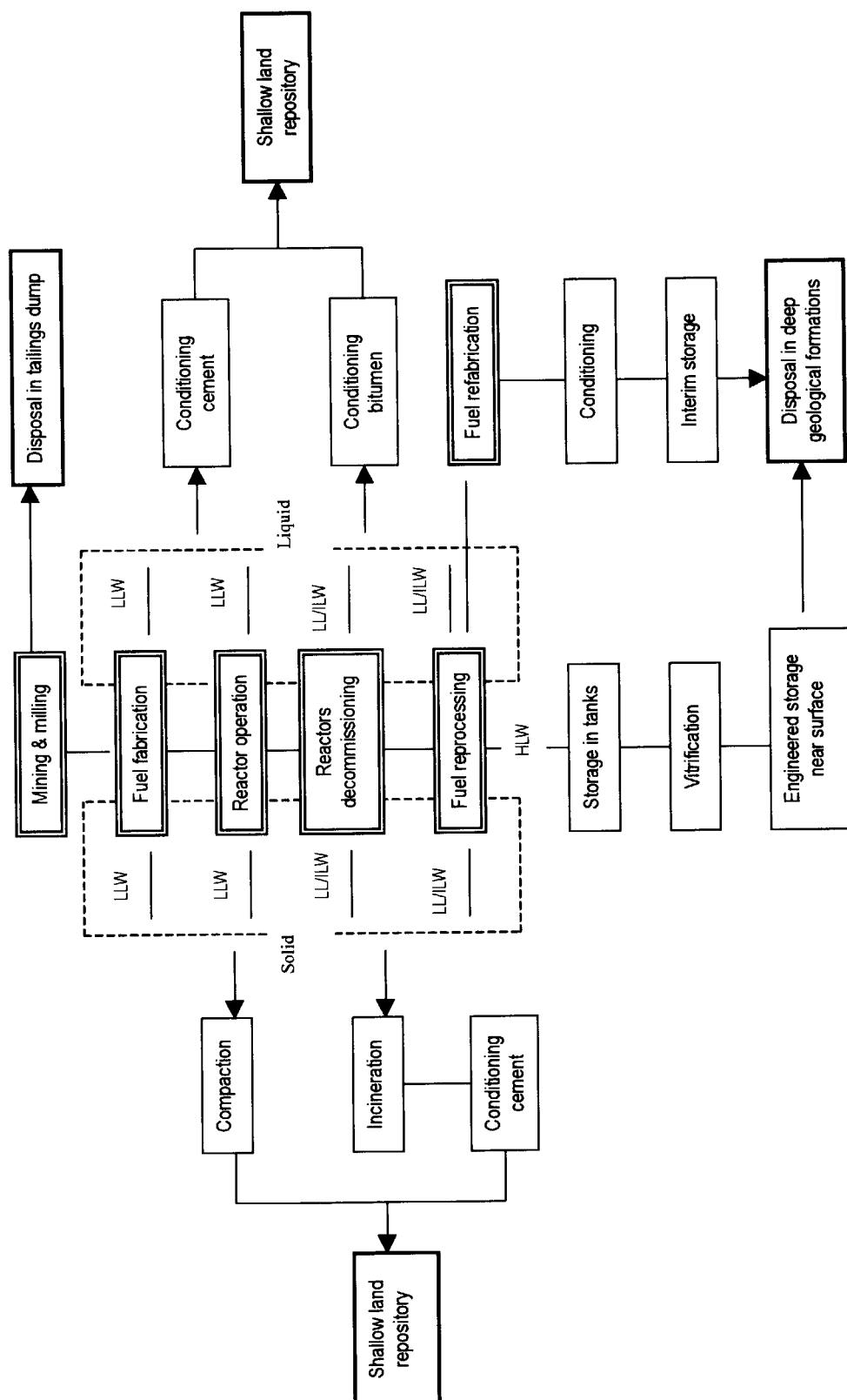
Fig. 7 Scheme of radioactive waste management program in China
