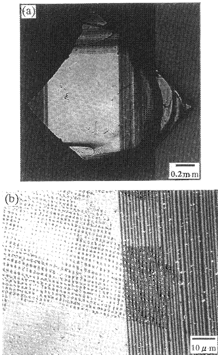
Fig. 5-3. Polarized optical micrographs of (a) an oxygen annealed \text{YBa}_2\text{Cu}_3\text{O}_x single crystal after the detwinning treatment and (b) its magnification of the boundary between twinned and perfectly detwinned domain.
