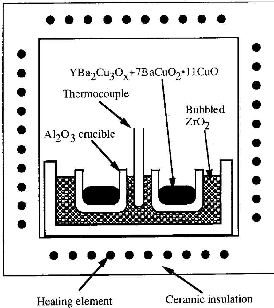
Fig. 3-1. Arrangement of the crucibles in a muffle furnace for preparation of solid-melt mixtures due to the peritectic reaction.
