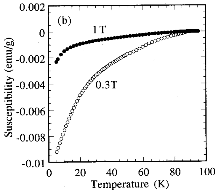
Fig. 2-15. Temperature dependence of the magnetic susceptibility of an O_2 -annealed YBa_2Cu_3O_x single crystal under magnetic fields of 0.3 and 1 T applied along or perpendicular to the c -axis in (a) and (b), respectively.
