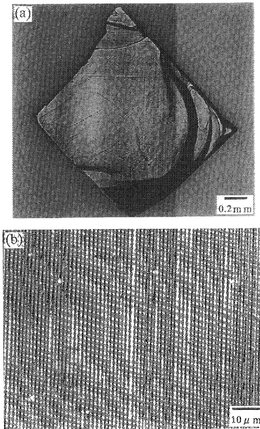
Fig. 5-2. Polarized optical micrographs of (a) an oxygen annealed \text{YBa}_2\text{Cu}_3\text{O}_x single crystal before the detwinning treatment and (b) its magnification of twinned domain.
