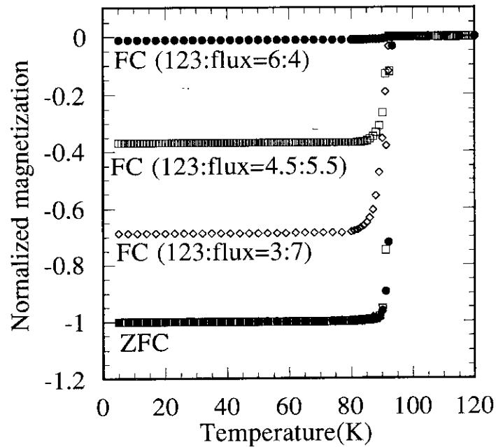
Fig. 4-4. Zero-field-cooled (ZFC) and field-cooled (FC) susceptibility of the three kinds of \text{YBa}_2\text{Cu}_3\text{O}_x single crystals which were grown from the mixtures whose compositional ratios of the solid 1/6 (123) to the melt 1/25 ( 7\text{BaCuO}_2 \cdot 11\text{CuO} ) were 3:7, 4.5:5.5 and 6:4. Magnetic field of 1.0 \times 10^{-3} T was applied along the c -axis.
