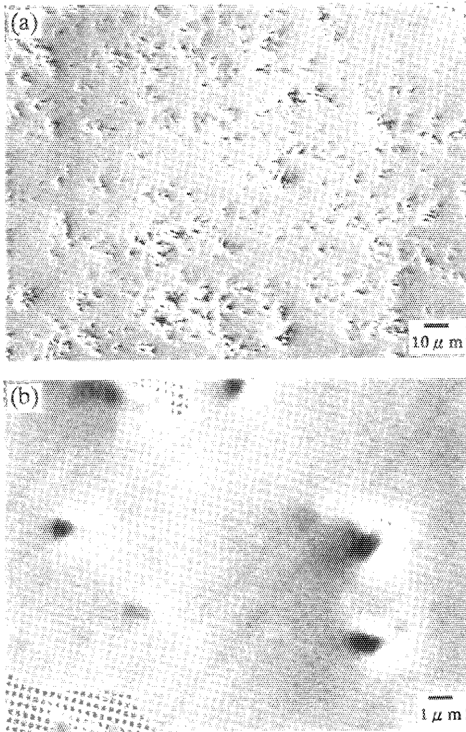
Fig. 4-2. (a) Cross sections perpendicular to the c -axis of a YBa 2 Cu 3 O x single crystal which was grown from the mixture whose compositional ratio of the solid 1/6 (123) to the melt 1/25 (7BaCuO 2 •11CuO) was 4.5:5.5 and (b) its magnification.
