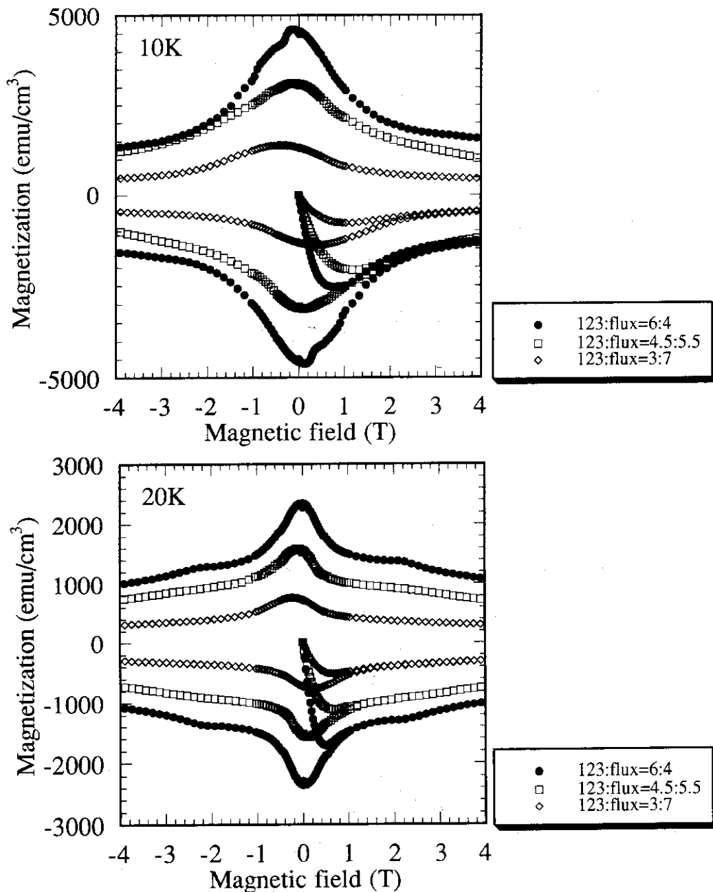
Fig. 4-5. Magnetization hysteresis loops of the three kinds of \text{YBa}_2\text{Cu}_3\text{O}_x single crystals which were grown from the mixtures whose compositional ratios of the solid 1/6 (123) to the melt 1/25 ( 7\text{BaCuO}_2 \cdot 11\text{CuO} ) were 3:7, 4.5:5.5 and 6:4. Magnetic fields up to 5.5 T were applied along the c -axis in the temperature range 10~80 K.
