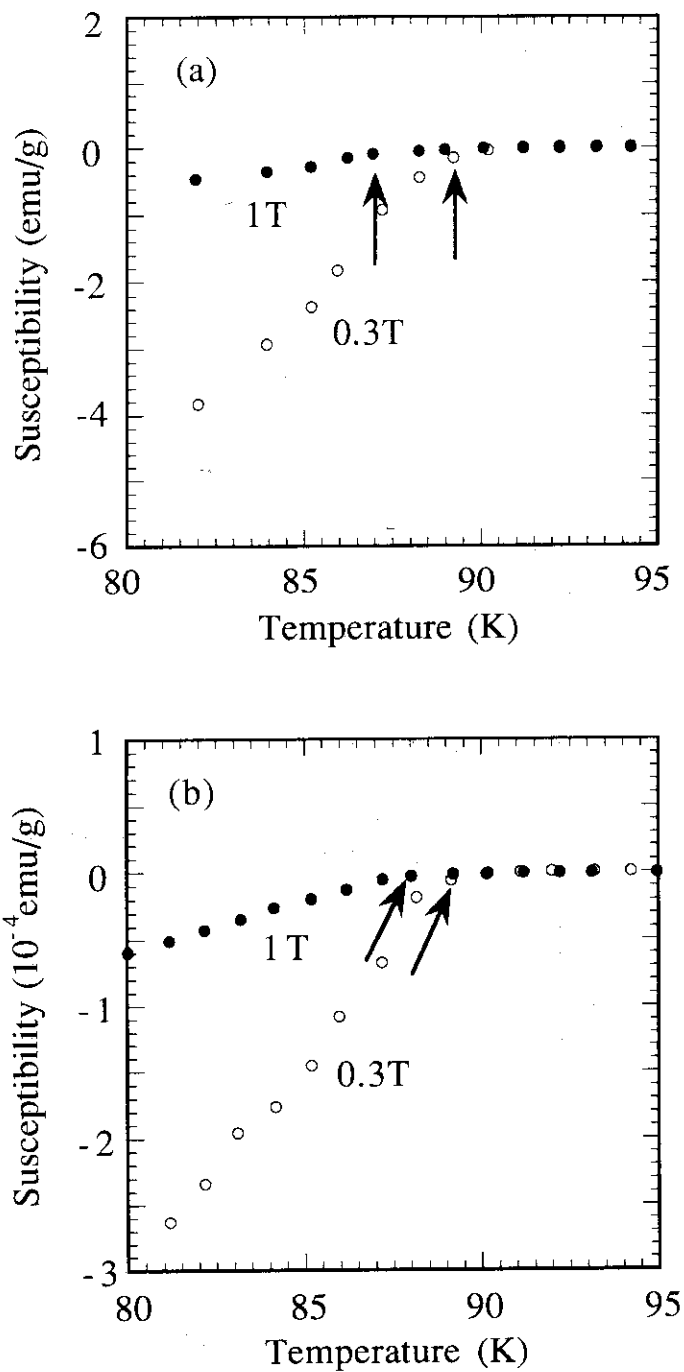
Fig. 2-16. Temperature dependence of the magnetic susceptibility of an O_2^- annealed YBa_2Cu_3O_x single crystal around the transition range under magnetic fields of 0.3 and 1 T applied along or perpendicular to the c -axis in (a) and (b), respectively.
