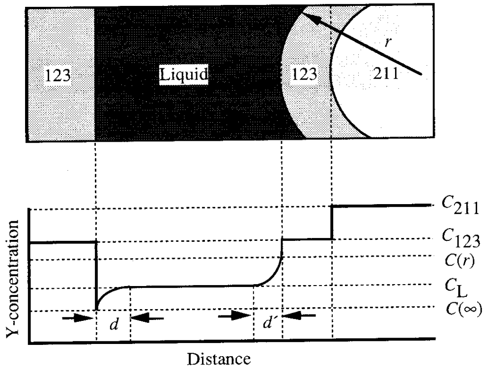
Fig. 3-8. Illustration of the dissolution of the curved \text{YBa}_2\text{Cu}_3\text{O}_x phase formed on \text{Y}_2\text{BaCuO}_5 phase due to the peritectic reaction and the growth of \text{YBa}_2\text{Cu}_3\text{O}_x single crystal having sharp flat surface. The phases are labeled as follows: 123: \text{YBa}_2\text{Cu}_3\text{O}_x , 211: \text{Y}_2\text{BaCuO}_5
