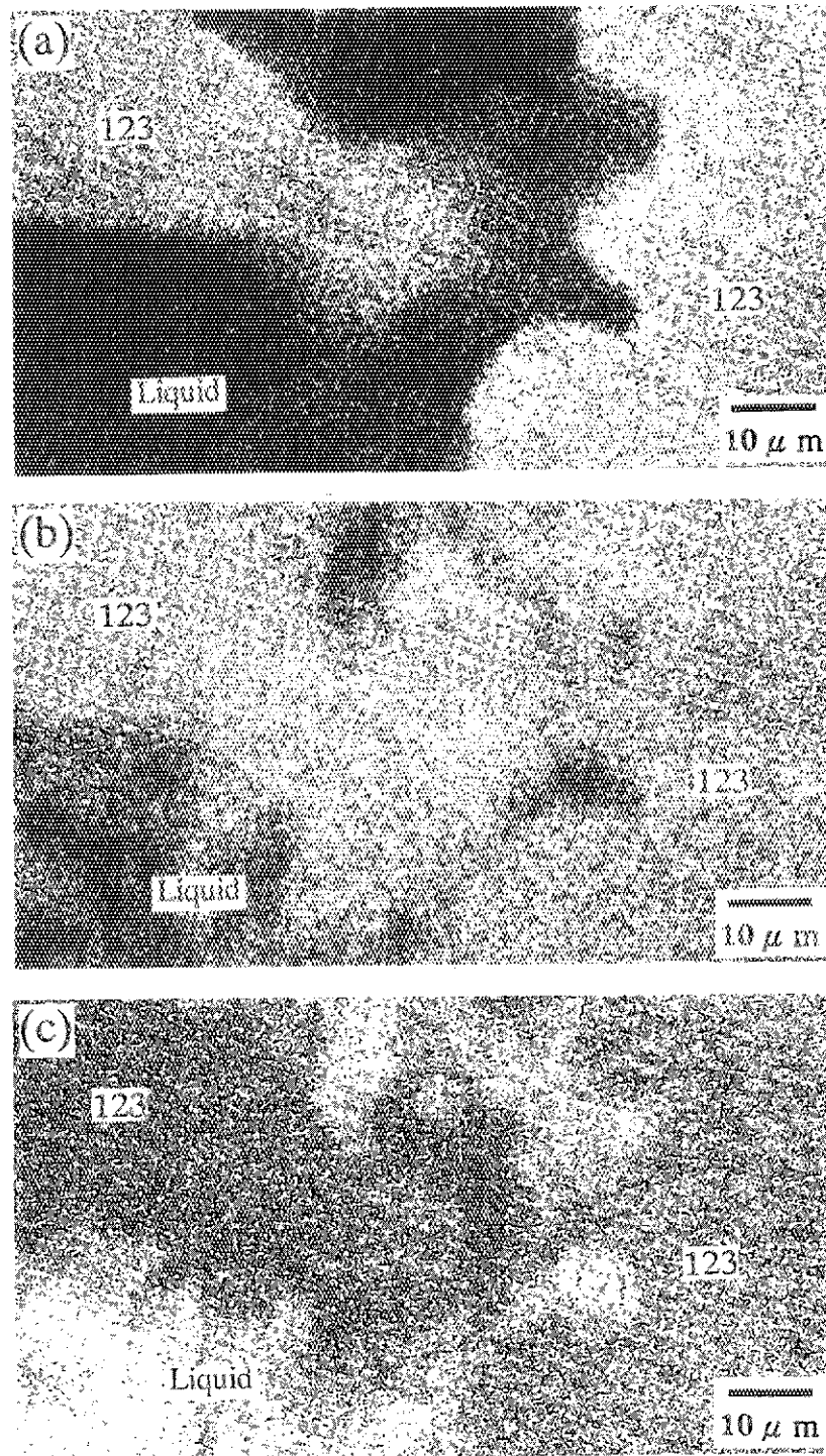
Fig. 3-5. Diffusion features of (a) yttrium, (b) barium and (c) copper contents from the top of the \text{YBa}_2\text{Cu}_3\text{O}_x phase to the ambient melt. The phases are labeled as follows: 123: \text{YBa}_2\text{Cu}_3\text{O}_x , 211: \text{Y}_2\text{BaCuO}_5
