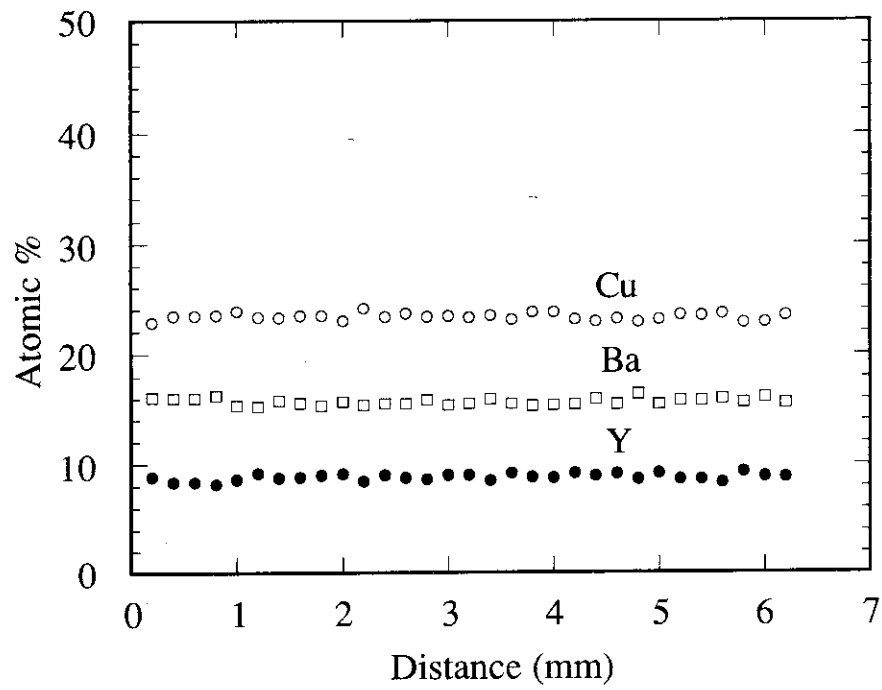
Fig. 2-10. Compositional distribution of Y, Ba and Cu atoms in the cross section along the c -axis. The data were determined using EPMA.
