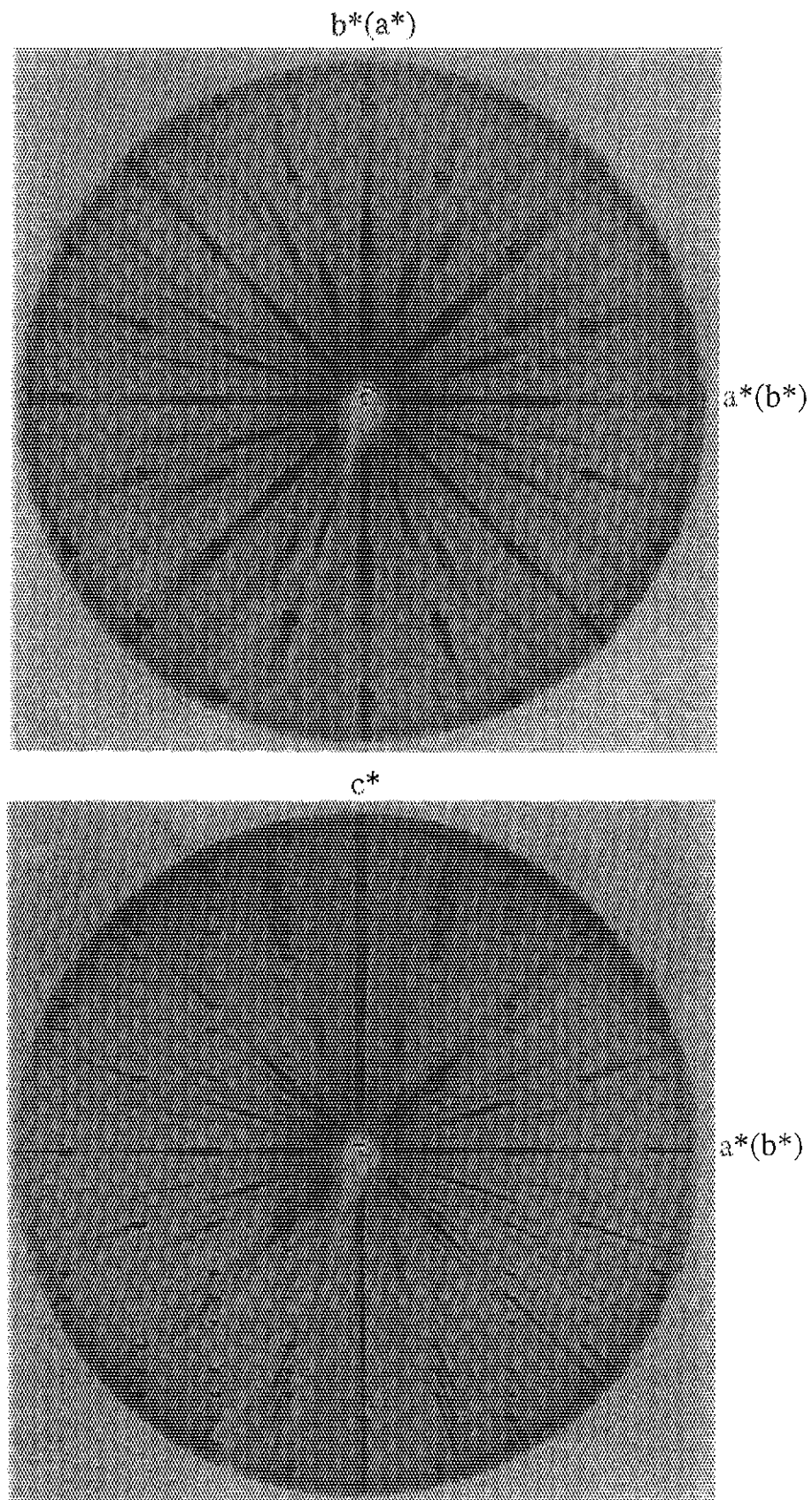
Fig. 5-5. X-ray precession photographs of a twinned \text{YBa}_2\text{Cu}_3\text{O}_x single crystal on the (a) (hk0) and (b) (0kl) plane.
