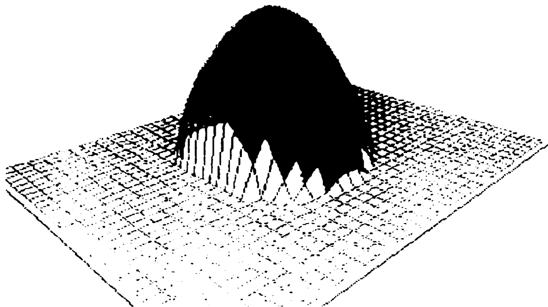
(a) Wavefront measured by Shearing interferometer
