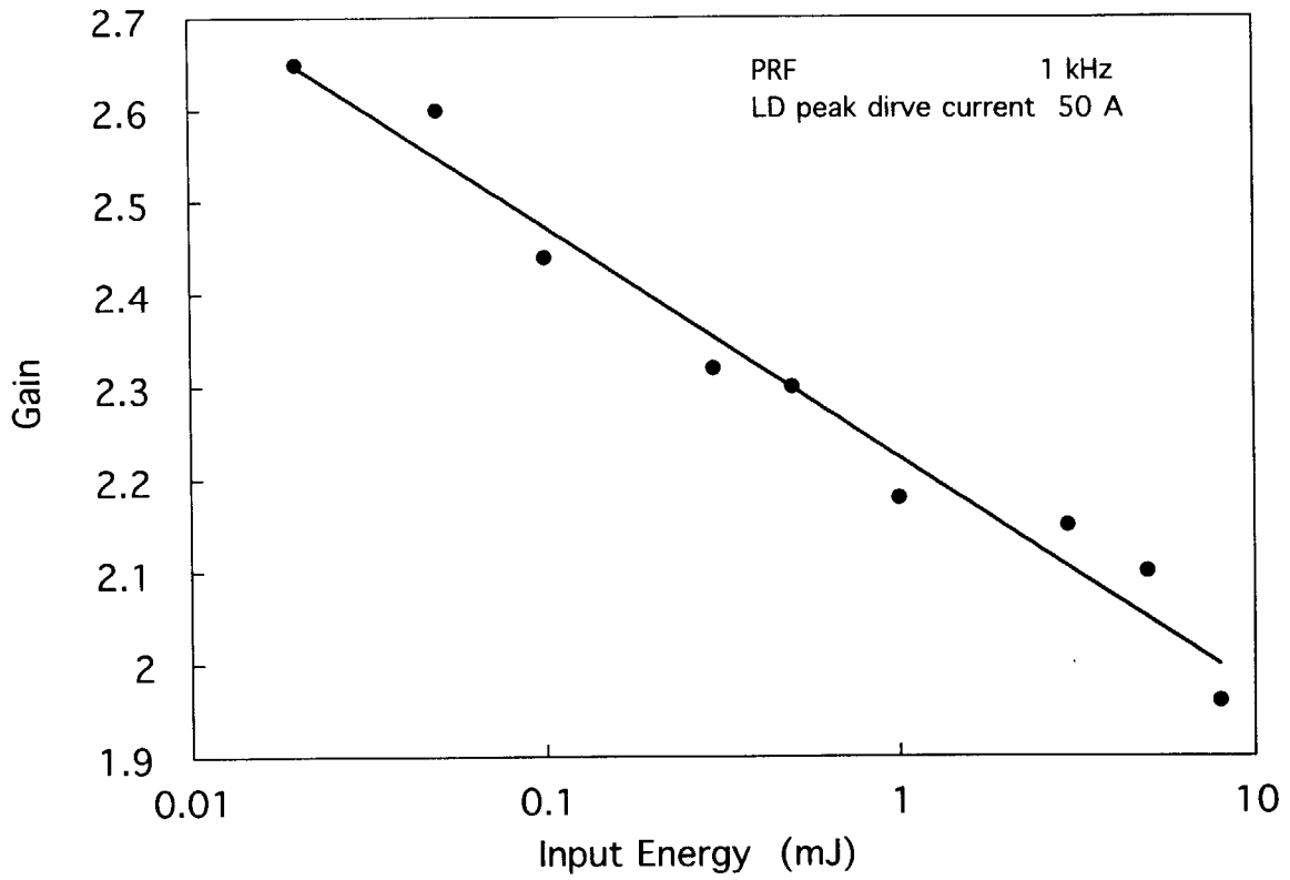
Fig.17 Gain of Nd:YAG amplifier
