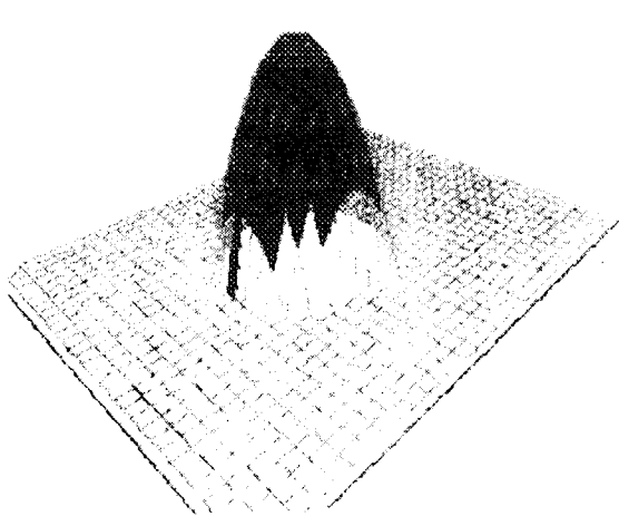
Wavefront ( 3\lambda )
