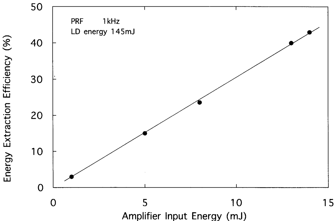
Fig.20 Energy extraction efficiency of YAG laser amplifier
