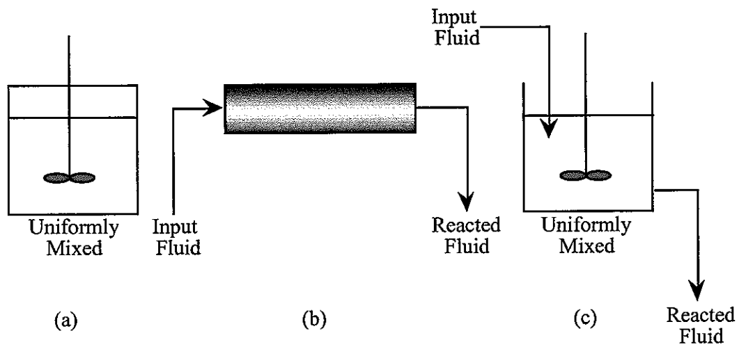
Figure 4 The three types of reactors: (a) batch reactor, (b) columns and (c) continuously stirred tank reactor (adapted from Levenspiel, 1972)
