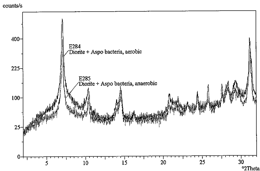
Figure 10 XRD traces (air-dried) obtained from orientated fine fraction ( <5\ \mu\text{m} ) material from CSTR experimental residues: (a) comparison of residues from biotic experiments run under aerobic and anaerobic conditions; (b) comparison of residues from abiotic experiments run under aerobic and anaerobic conditions.
