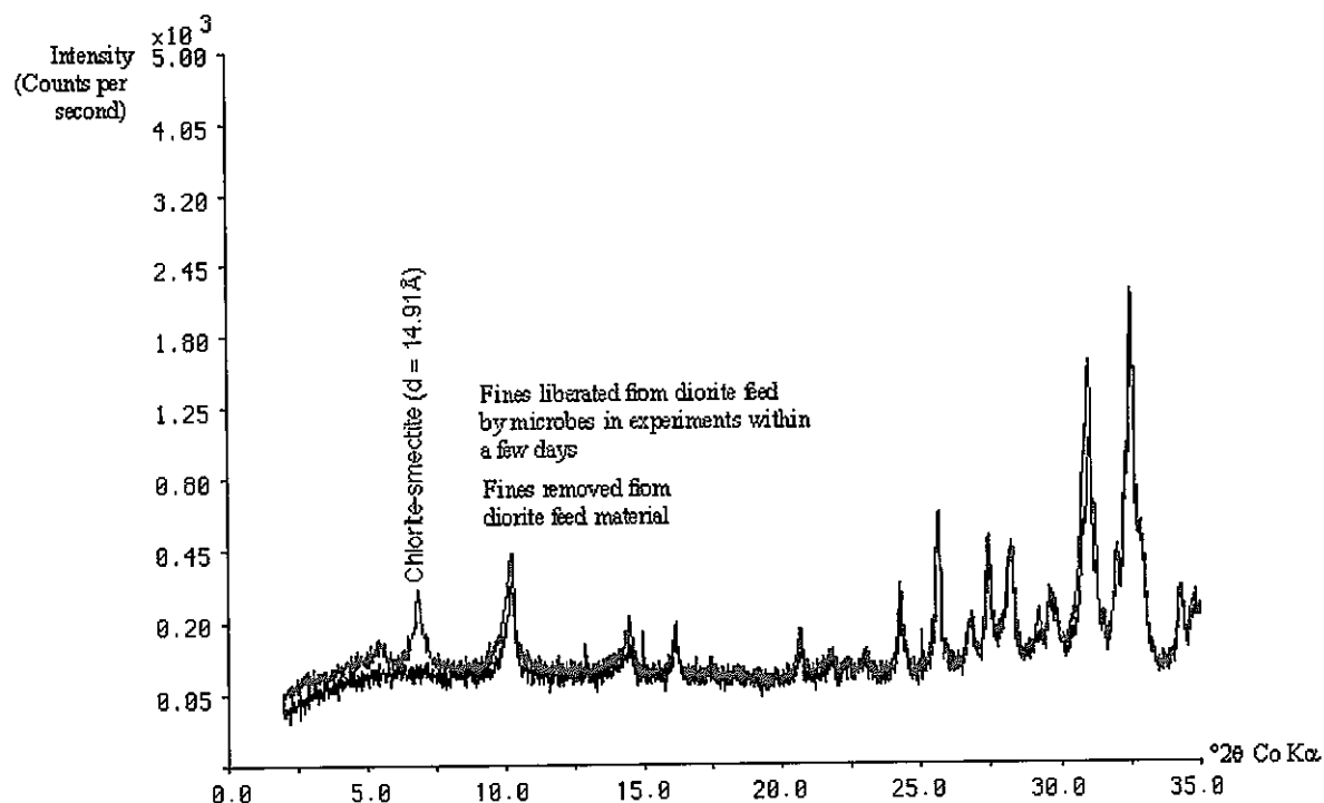
Figure 8 Comparison of the XRD traces (air-dried) obtained from the orientated fine fraction ( <5\ \mu\text{m} ) material separated from the crushed Äspö Diorite starting material and the experimental residue from Column 2.
