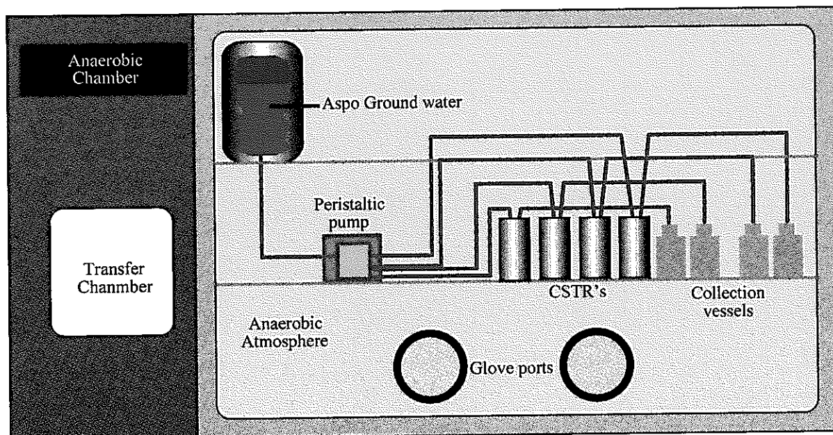
Figure 6 Schematic of CSTR set up
