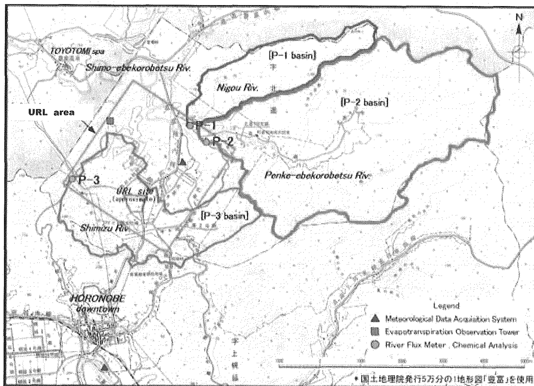
Figure 1 Location of the equipment for the surface hydrogeological investigations.
