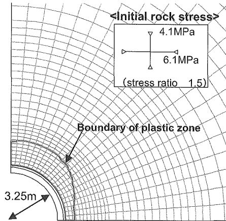
Figure 3. Results of analyses (Boundary of plastic zone).
