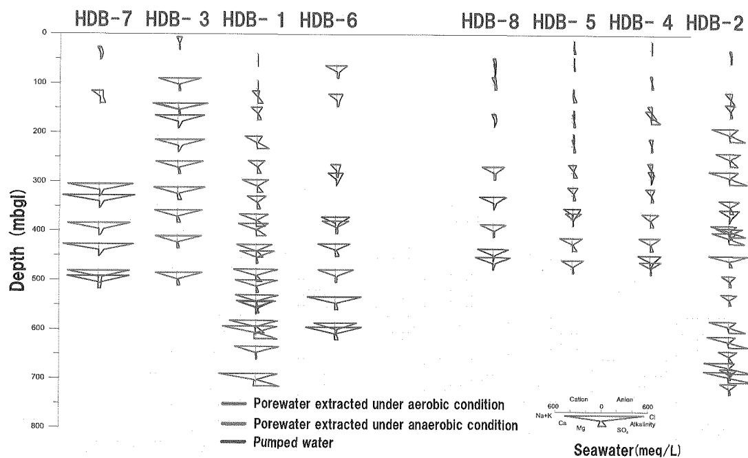
Figure 5 Depth profile of hydrochemistry of groundwater
