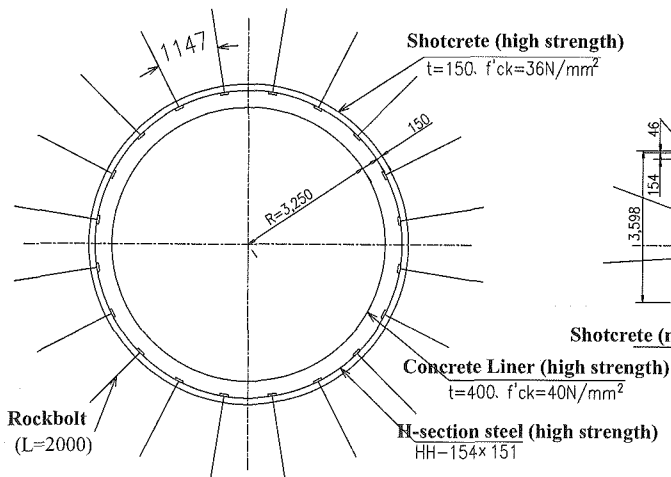
Figure 4. Standard support patterns (Samples).
