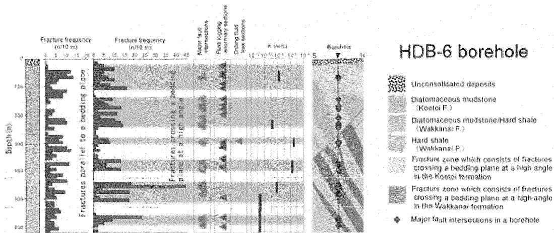
Figure 3 Result of the borehole investigations
