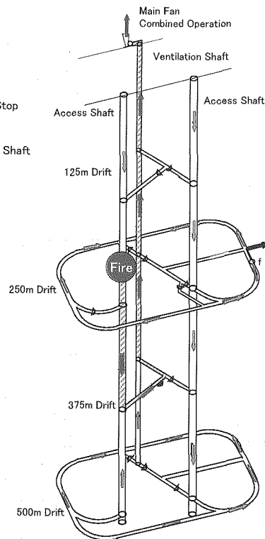
Figure 5. Results of ventilation network analysis under fire condition.
