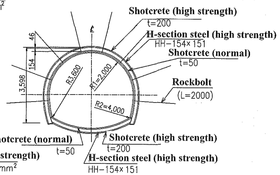
Figure 4. Standard support patterns (Samples).
