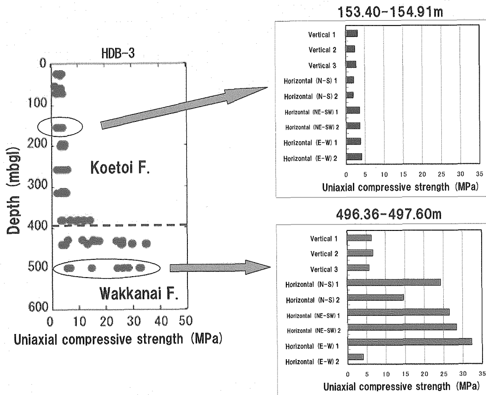
Fig.3 Heterogeneity of rock mechanical property
