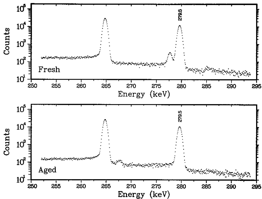
Fig. 8. The upper sixth of the ^{75}\text{Se} spectra, obtained in 1000-second counting periods with fresh and aged product solution samples, which includes the ^{75}\text{Se} gamma ray at 279.5 keV.
