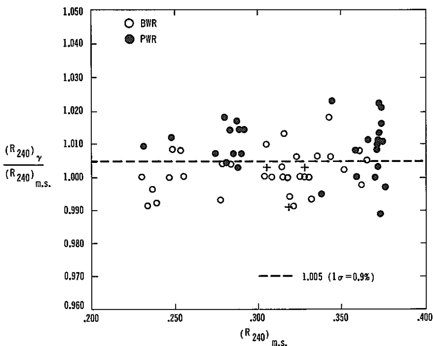
Fig. 18. Ratio of the ^{240}\text{Pu} isotopic ratio (relative to ^{239}\text{Pu} ) obtained from the passive gamma-ray assay to that obtained from mass spectrometry, plotted vs the ^{240}\text{Pu} isotopic ratio (relative to ^{239}\text{Pu} ). The open symbols distinguish the BWR from the PWR samples. The dashed line corresponds to the average result. The 1\text{-}\sigma value is the percentage standard deviation of the data.
