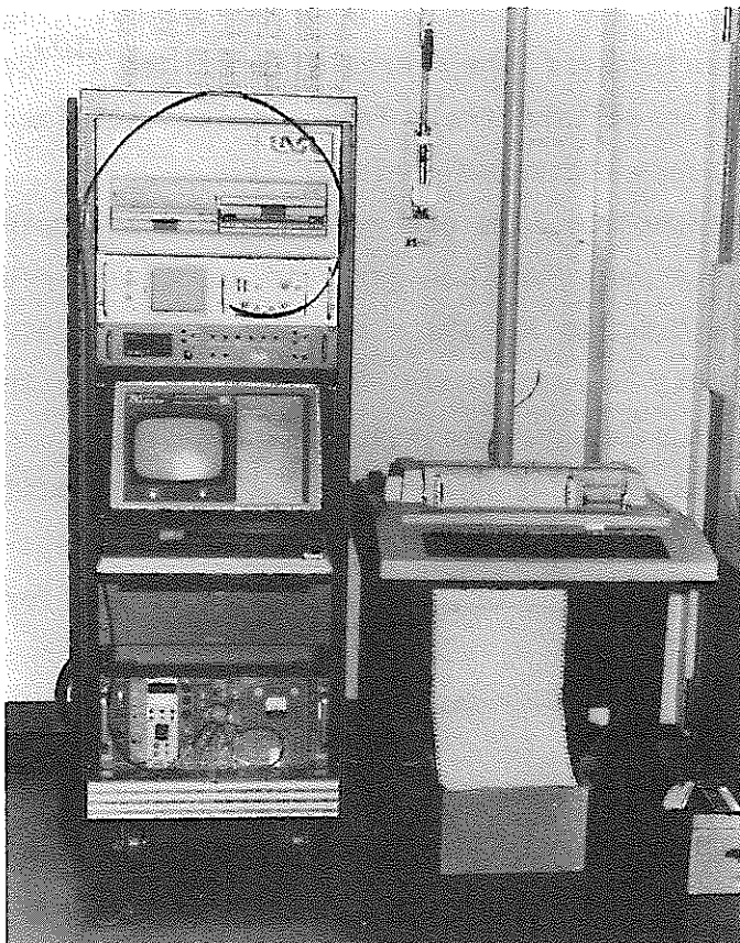
Fig. 5. Photograph of the electronics and the hardcopy terminal at the Tokai plant. The electronics rack includes (top to bottom) a dual floppy disk drive, an oscilloscope, the control unit for the mechanical system, the multichannel analyzer with CRT terminal, the minicomputer, and NIM modular electronics.
