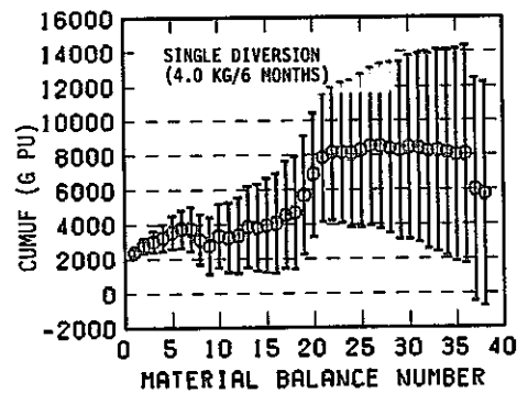
Fig. 5.16 CUMUF and uniform diversion tests for different n.r.t. material balance periods with S.S.1-5-1 (single diversion (↓) of 4.0 kgs Pu per 6 months).
