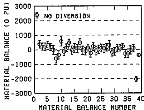
Fig. 5.13 CUMUF and uniform diversion tests for different n.r.t. material balance periods with S.S.1-5-1 (no diversion); Simulation period; 6 months.
