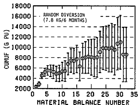
Fig. 5.25 CUMUF and uniform diversion tests for different n.r.t. material balance periods with S.S.1-8 (random diversion (↓) 7.8 kgs Pu per 6 months).
