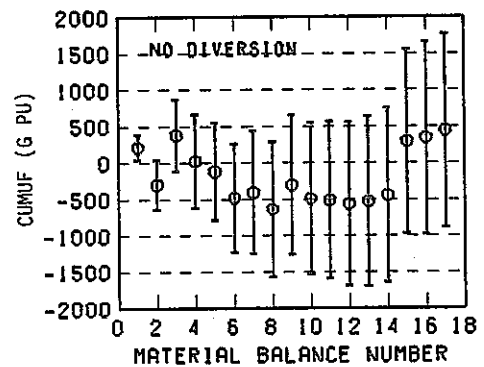
Fig. 5.41 Comparison of detection sensitivities in terms of different in-process PIT models for S.S.4 (no diversion).
