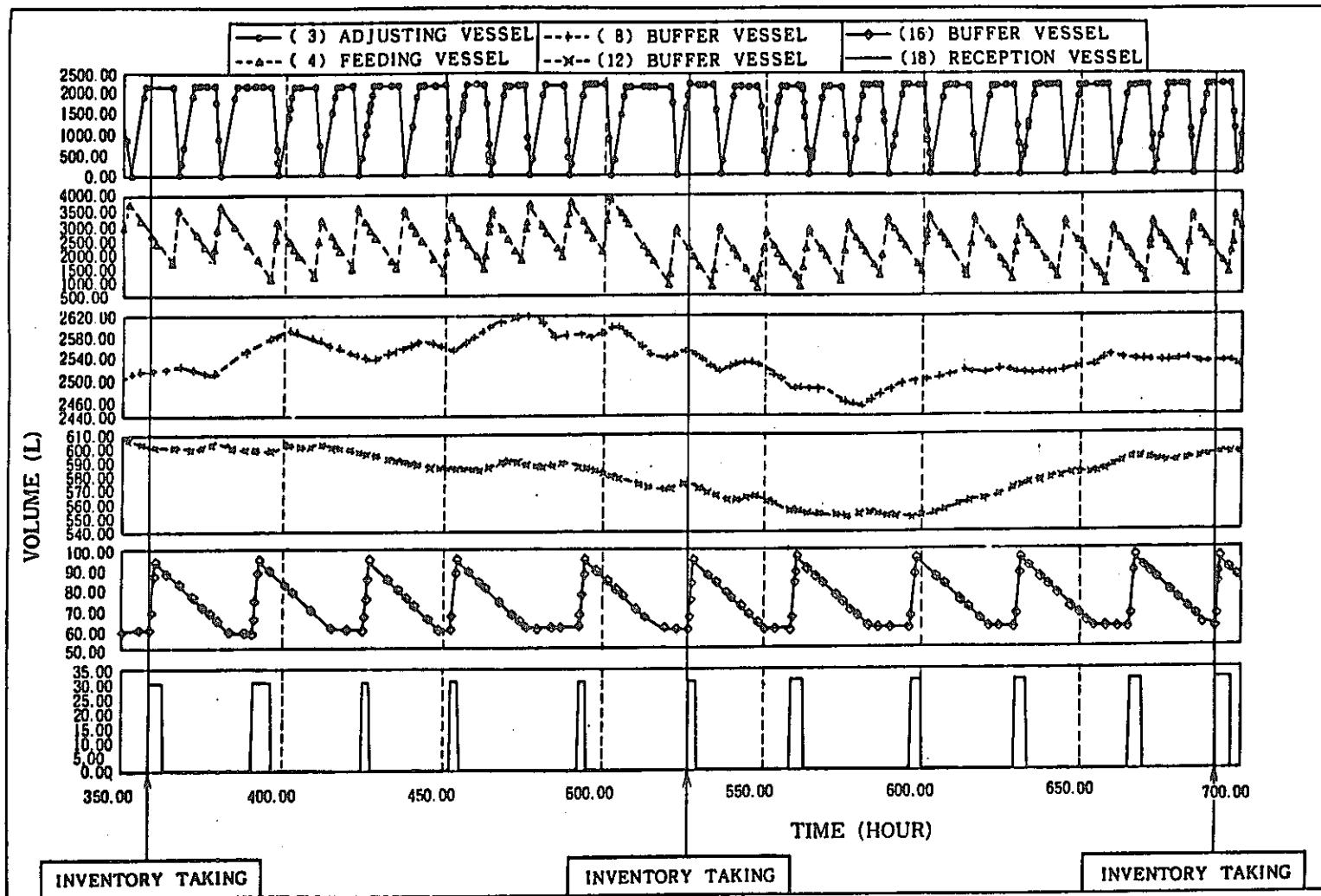
Fig. 4.1 Graphic representation of variations in volume of solution in the major measurement points. Three inventory cut-off points are also indicated. Each point is chosen at a particular point of time immediately after the evaporator become empty and before evaporator feed is resumed
