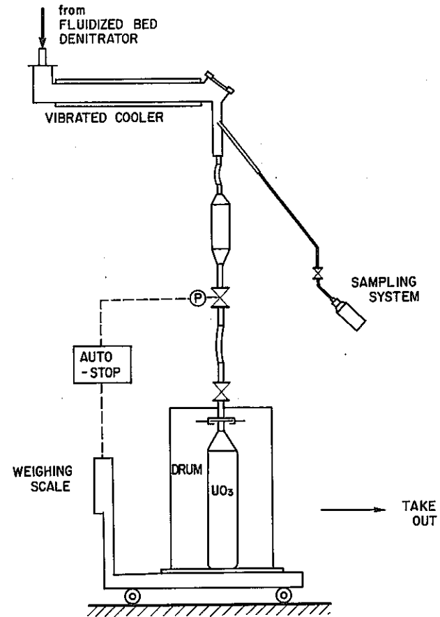
Fig. 3.10 Weighing and Sampling System for U-product (UO 3 -powder)
