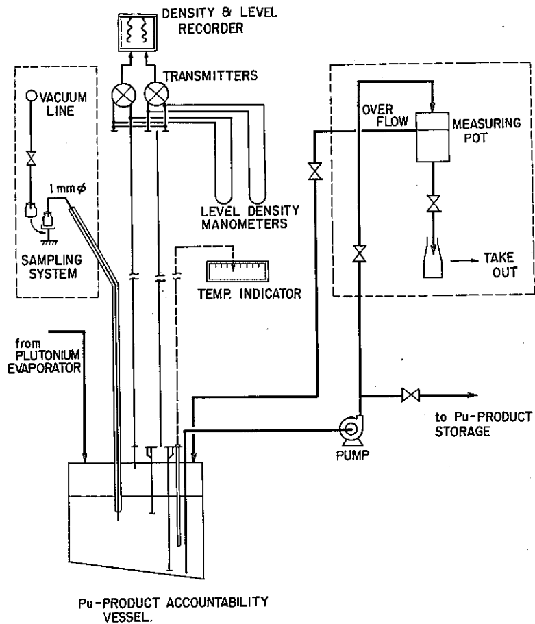
Fig. 3.9 Volume Measurement and Sampling System for Pu-product
