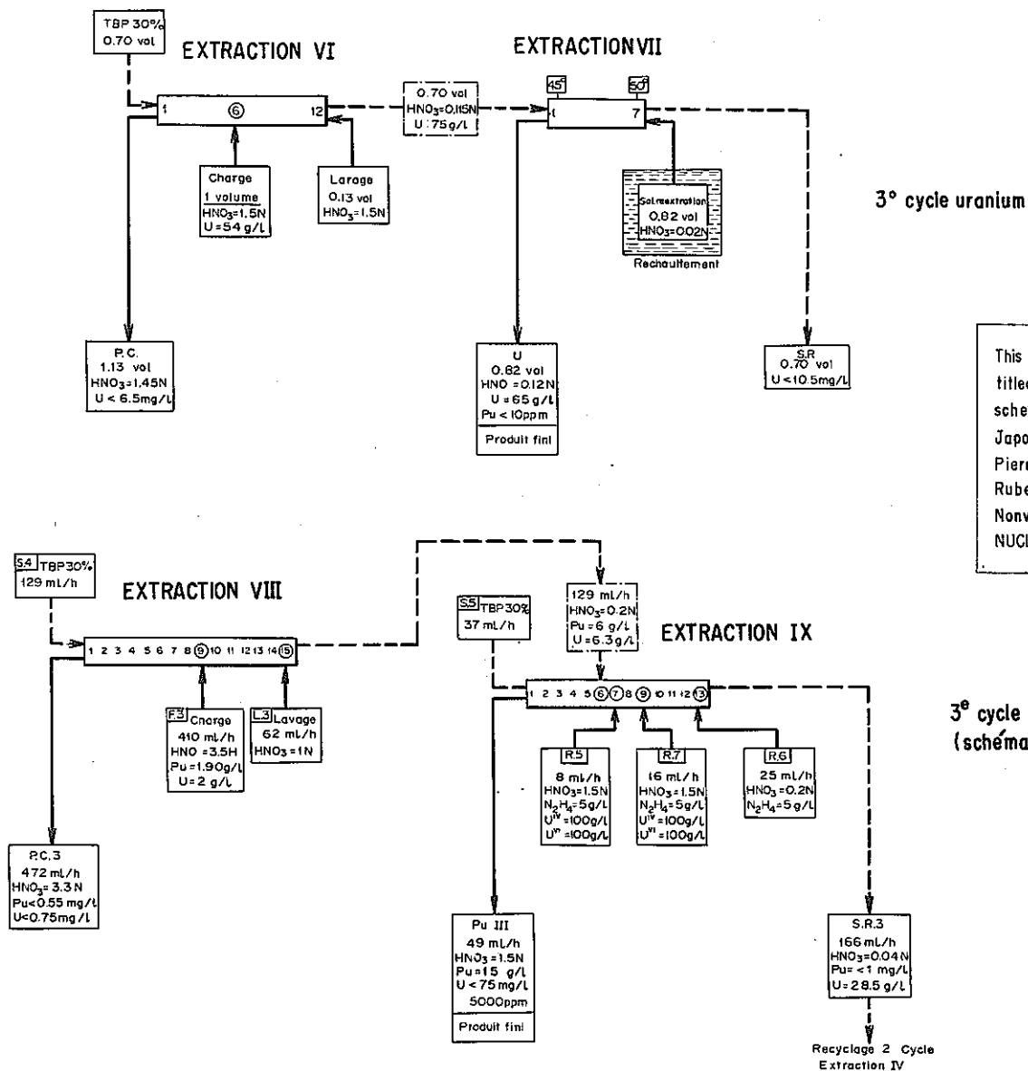
Fig. 3.4 Flowsheet of Purification Processes of Uranium and Plutonium
