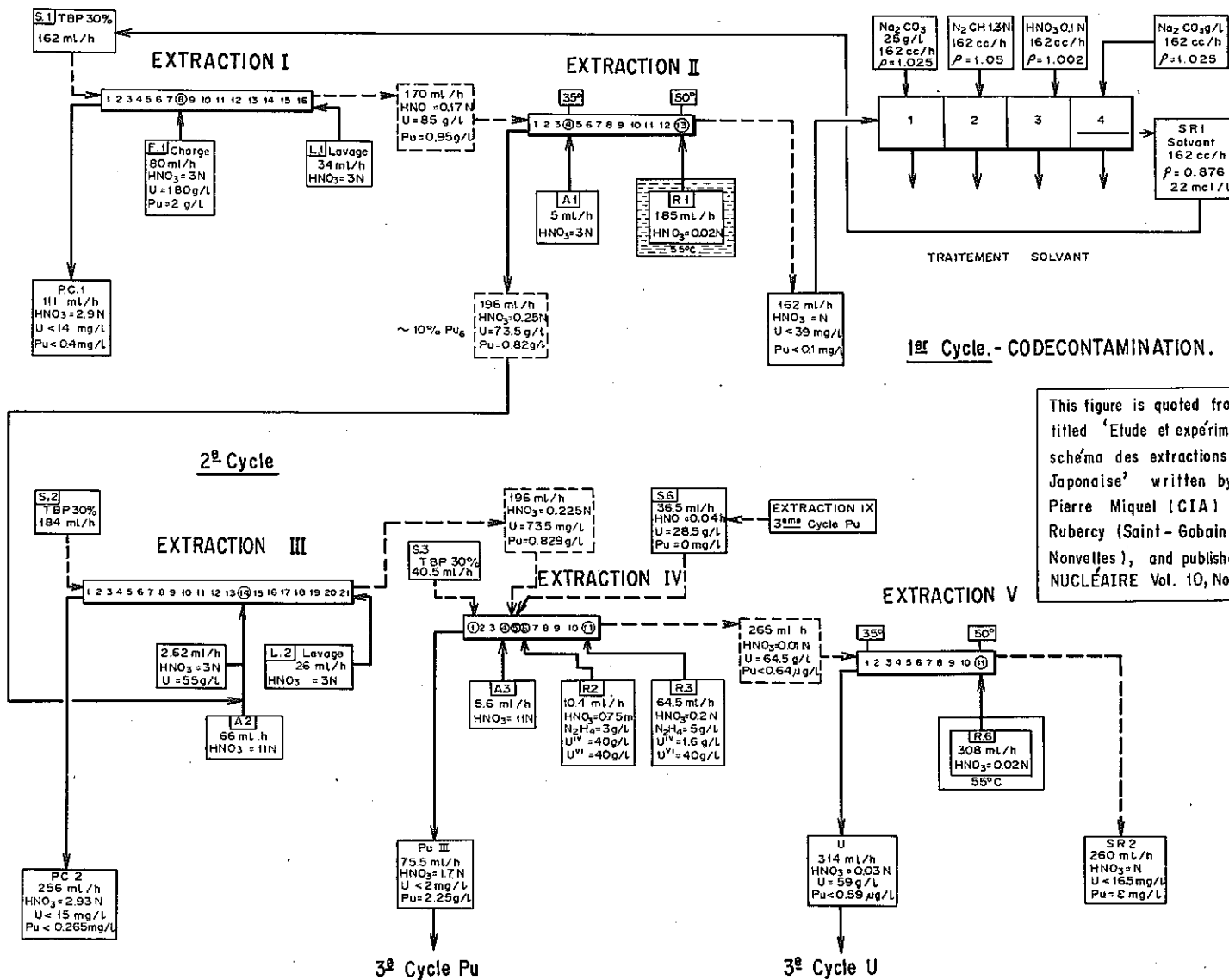
Fig. 3.3 Flowsheet of Co-decontamination and Partition Process
