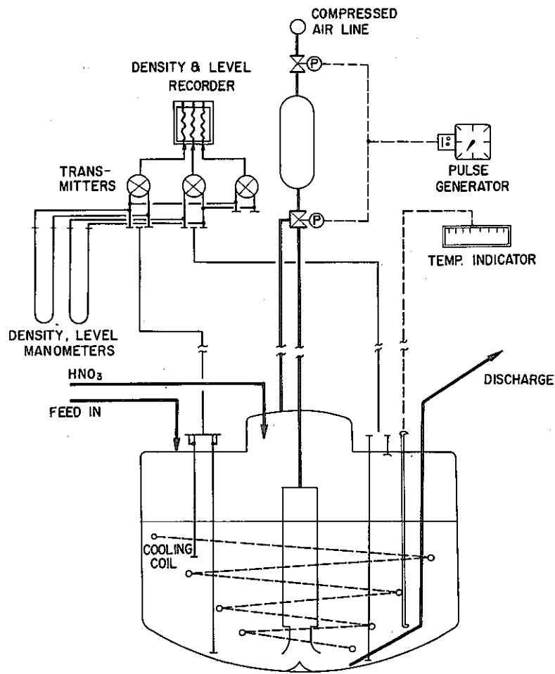
Fig. 3.7 Volume Measurement System of Input Accountability Vessel
