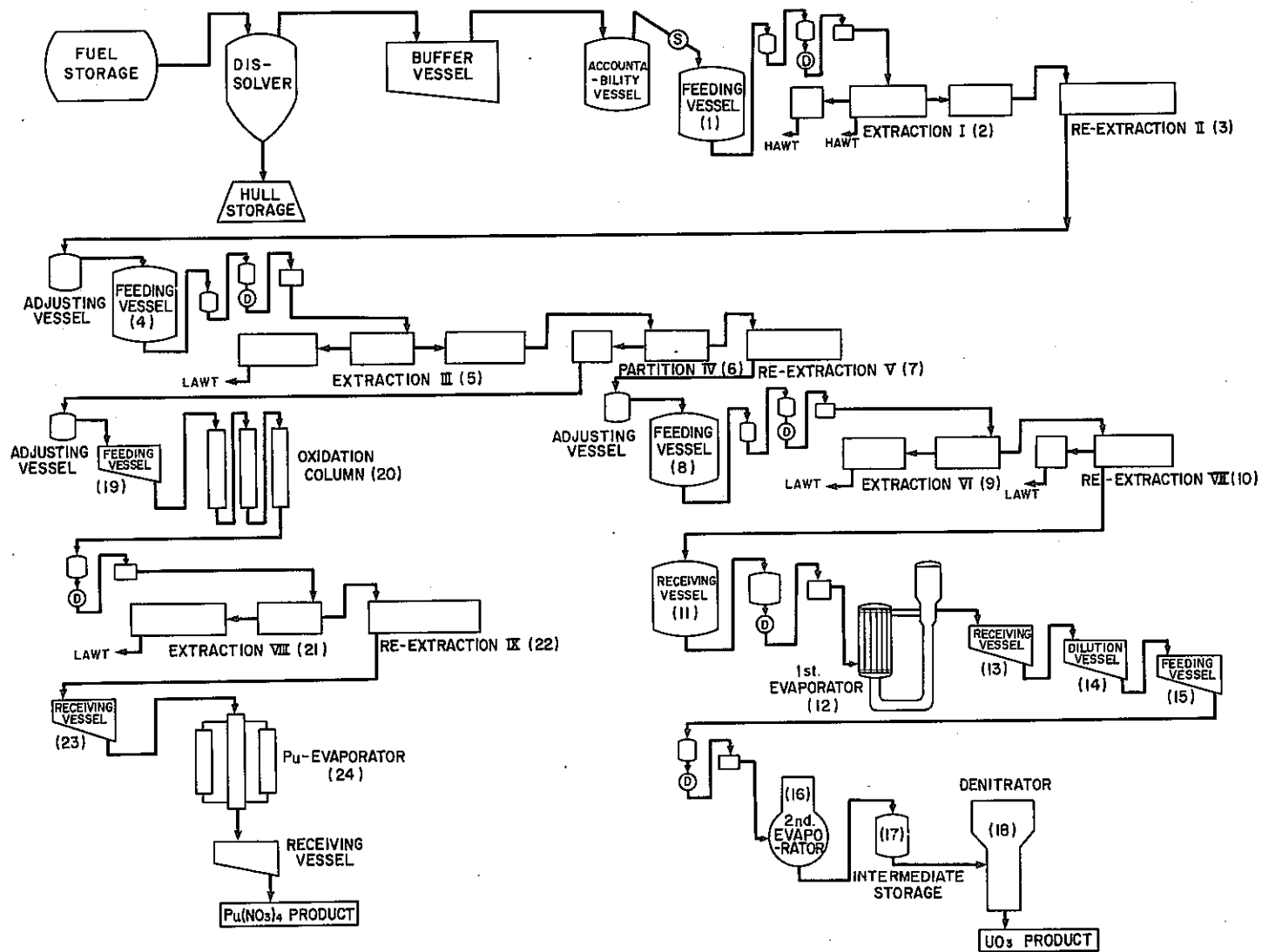
Fig. 3.2 Schematic Flowsheet of the Model Reprocessing Plant
