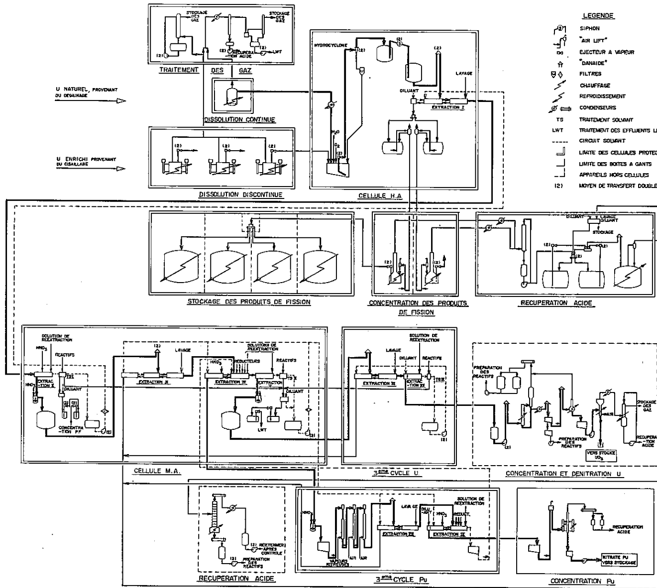
Fig. 3.1 General Scheme of Chemical Treatment
