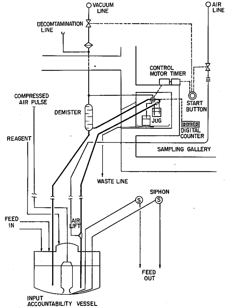
Fig. 3.8 Sampling System of Input Accountability Vessel
