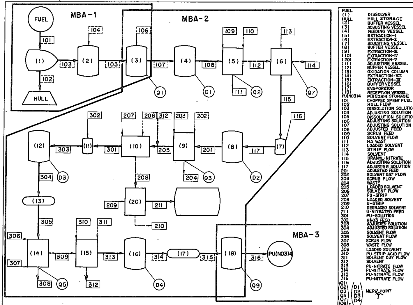
Fig. 3.5 MODEL REPROCESSING PLANT PROCESS FLOW
