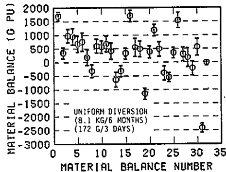
Fig. 5.31 CUMUF and uniform diversion tests for different n.r.t. material balance periods with S.S.4 (uniform diversion of 8.1 kgs Pu per 6 months).
