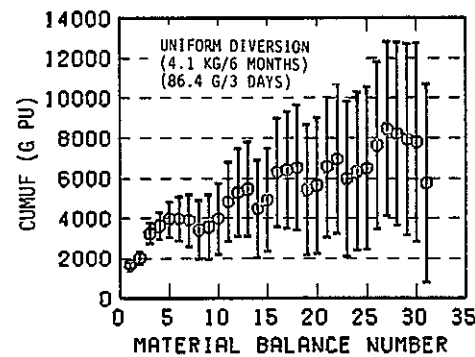
Fig. 5.28 CUMUF and uniform diversion tests for different n.r.t. material balance periods with S.S.4 (uniform diversion of 4.1 kgs Pu per 6 months).
