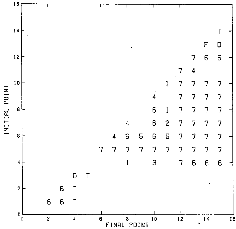
Fig. 7.4 Alarm-Sequence Chart based on CUMUF Tests
