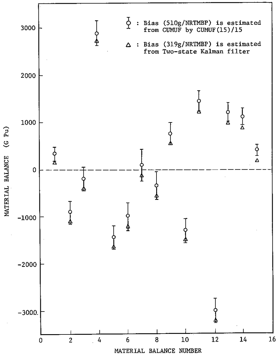
Fig. 7.6 MUF d Corrected for Biases of Different Estimates.
