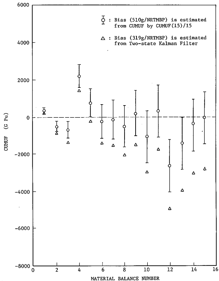
Fig. 7.7 CUMUF Based on MUF d Corrected for Biases of Different Estimates.
