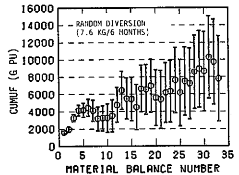
Fig. 5.32 CUMUF and uniform diversion tests for different n.r.t. material balance periods with S.S.4 (random diversion ( \downarrow ) of 7.6 kgs Pu per 6 months).
