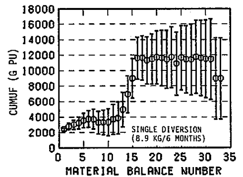
Fig. 5.26 CUMUF and uniform diversion tests for different n.r.t. material balance periods with S.S.1-8 (single diversion (↓) of 8.9 kgs Pu per 6 months).
