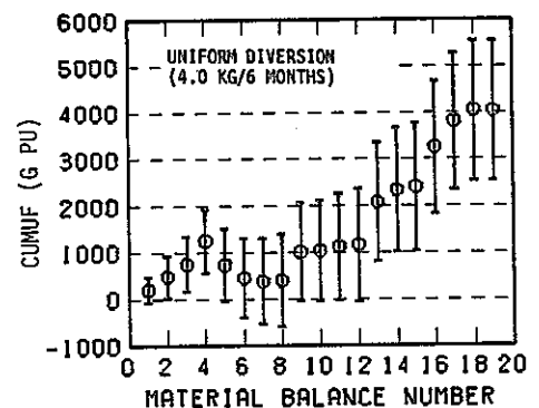
Fig. 5.36 Comparison of detection sensitivities in terms of different in-process PIT models for S.S.1-7 (uniform diversion of 4.0 kgs Pu per 6 months).
