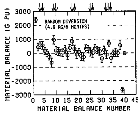
Fig. 5.15 CUMUF and uniform diversion tests for different n.r.t. material balance periods with S.S.1-5-1 (random diversion ( \psi ) of 4 kgs Pu per 6 months).
