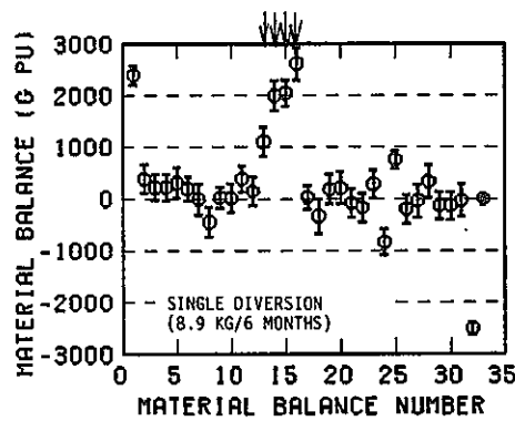
Fig. 5.26 CUMUF and uniform diversion tests for different n.r.t. material balance periods with S.S.1-8 (single diversion (↓) of 8.9 kgs Pu per 6 months).
