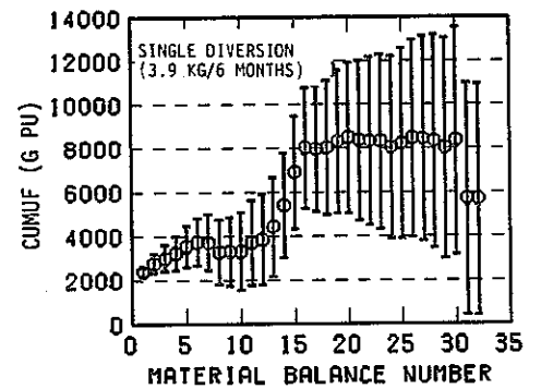
Fig. 5.23 CUMUF and uniform diversion tests for different n.r.t. material balance periods with S.S.1-8 (single diversion ( \psi ) of 3.9 kgs Pu per 6 months).
