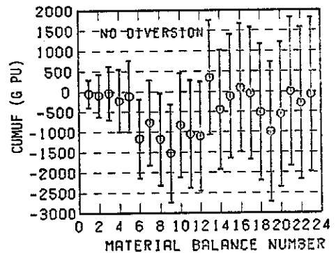
Fig. 5.49 CUMUF and uniform diversion tests for different estimation methods for unmeasured inventories with S.S.1-9-2 (no diversion); Simulation period: 8 months.
