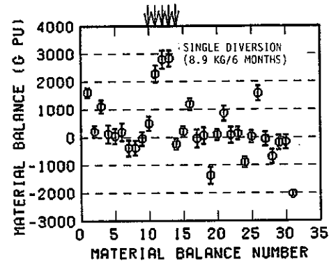
Fig. 5.33 CUMUF and uniform diversion tests for different n.r.t. material balance periods with S.S.4 (single diversion ( \psi ) of 8.9 kgs Pu per 6 months).
