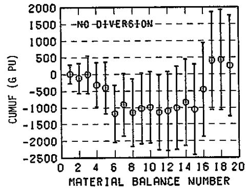
Fig. 5.35 Comparison of detection sensitivities in terms of different in-process PIT models for S.S.1-7 (no diversion).
