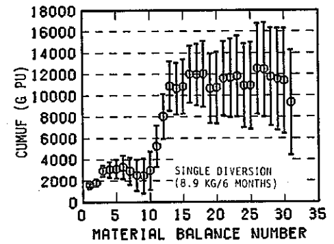
Fig. 5.33 CUMUF and uniform diversion tests for different n.r.t. material balance periods with S.S.4 (single diversion ( \psi ) of 8.9 kgs Pu per 6 months).
