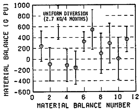
Fig. 5.40 Comparison of detection sensitivities in terms of different in-process PIT models for S.S.1-10 (uniform diversion of 2.7 kgs Pu per 4 months).
