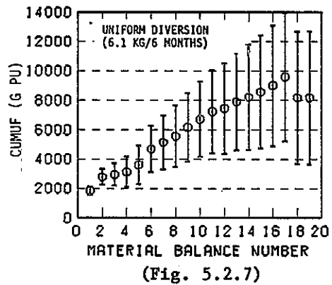
Fig. 5.2 CUMUF and uniform diversion tests for S.S.1-1 and S.S.1-2; Simulation period; 6 months.
