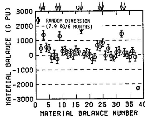
Fig. 5.18 CUMUF and uniform diversion tests for different n.r.t. material balance periods with S.S.1-5-1 (random diversion ( \psi ) 7.9 kgs Pu per 6 months).
