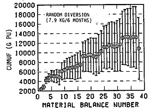
Fig. 5.18 CUMUF and uniform diversion tests for different n.r.t. material balance periods with S.S.1-5-1 (random diversion ( \psi ) 7.9 kgs Pu per 6 months).
