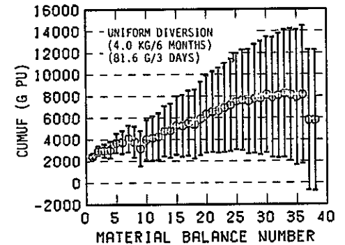
Fig. 5.14 CUMUF and uniform diversion tests for different n.r.t. material balance periods with S.S.1-5-1 (uniform diversion of 4 kgs Pu per 6 months).
