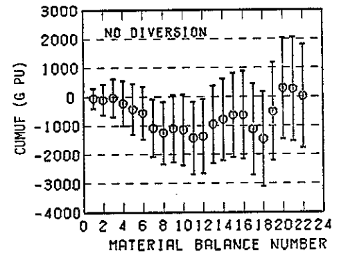
Fig. 5.51 CUMUF and uniform diversion tests for different estimation methods for unmeasured inventories with S.S.1-10-2 (no diversion); Simulation period: 8 months.
