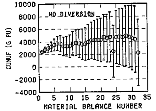
Fig. 5.20 CUMUF and uniform diversion tests for different n.r.t. material balance periods with S.S.1-8 (no diversion); Simulation period; 6 months.
