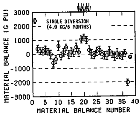
Fig. 5.16 CUMUF and uniform diversion tests for different n.r.t. material balance periods with S.S.1-5-1 (single diversion (↓) of 4.0 kgs Pu per 6 months).
