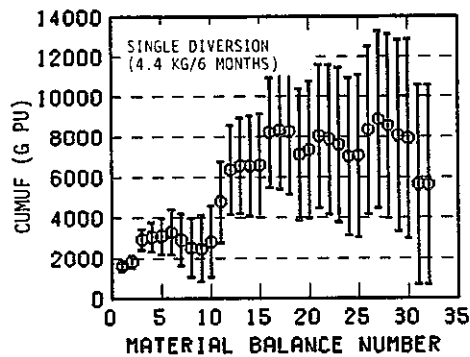
Fig. 5.30 CUMUF and uniform diversion tests for different n.r.t. material balance periods with S.S.4 (single diversion ( \psi ) of 4.4 kgs Pu per 6 months).
