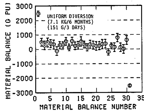
Fig. 5.24 CUMUF and uniform diversion tests for different n.r.t. material balance periods with S.S.1-8 (uniform diversion of 7.1 kgs Pu per 6 months).
