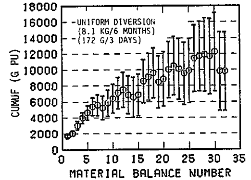
Fig. 5.31 CUMUF and uniform diversion tests for different n.r.t. material balance periods with S.S.4 (uniform diversion of 8.1 kgs Pu per 6 months).
