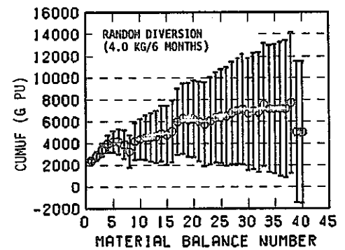
Fig. 5.15 CUMUF and uniform diversion tests for different n.r.t. material balance periods with S.S.1-5-1 (random diversion ( \psi ) of 4 kgs Pu per 6 months).
