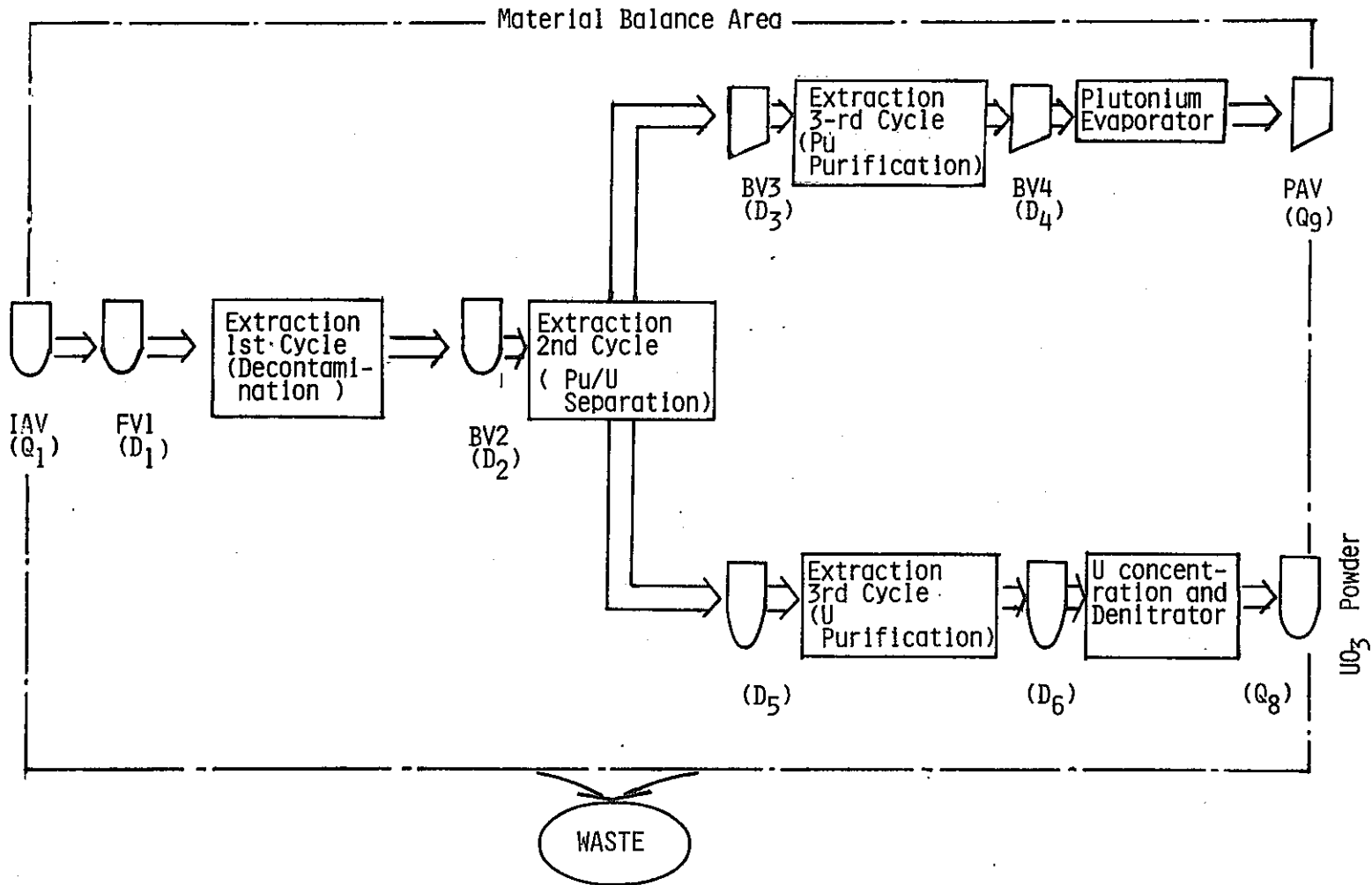
Fig. 6.1 Measurement Points for the In-process Inventory
